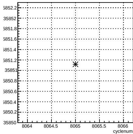
usl_coil6:cyclenum {run == 7120}
