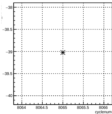
usl_11X12X:cyclenum {run == 7120}
