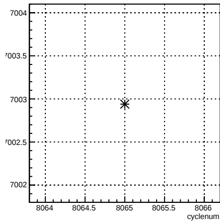
usl_coil7:cyclenum {run == 7120}
