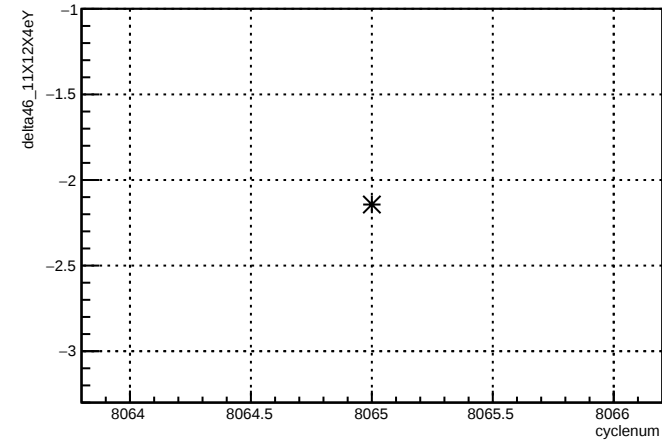
delta46_11X12X4eY:cyclenum {run == 7120}
