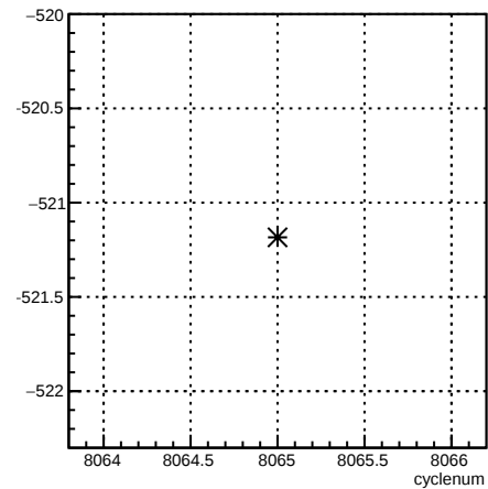
4eX_coil1:cyclenum {run == 7120}
