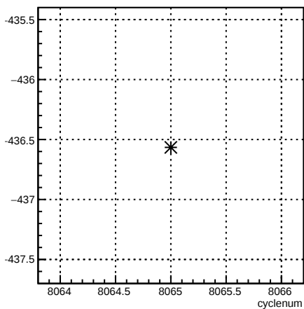
11X12X_coil7:cyclenum {run == 7120}
