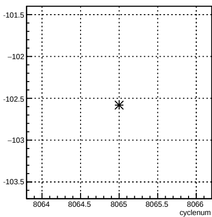
4eX_coil3:cyclenum {run == 7120}
