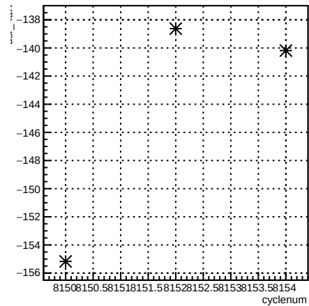
usr_4eY:cyclenum {run == 7151}
