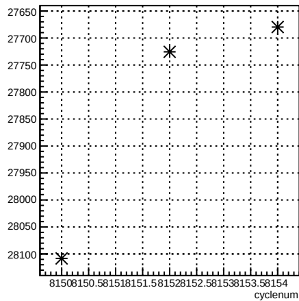
usr_coil6:cyclenum {run == 7151}
