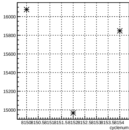
usl_coil7:cyclenum {run == 7151}
