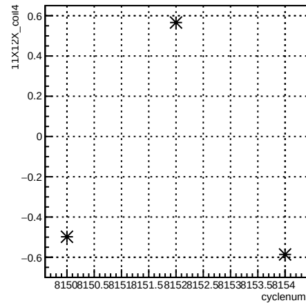
11X12X_coil4:cyclenum {run == 7151}
