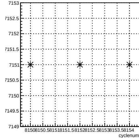
run:cyclenum {run == 7151}
