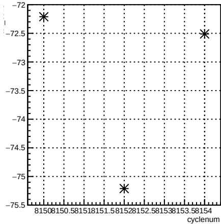
4eX_coil3:cyclenum {run == 7151}
