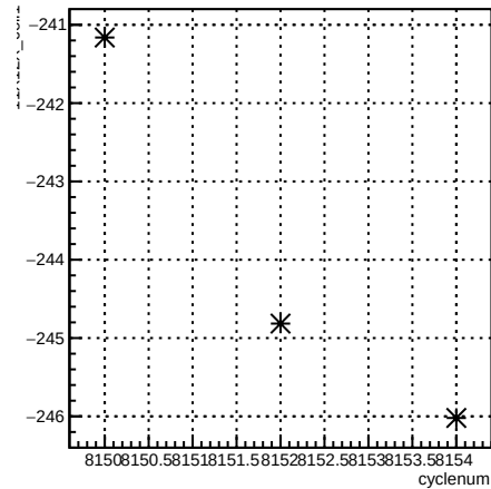
11X12X_coil1:cyclenum {run == 7151}
