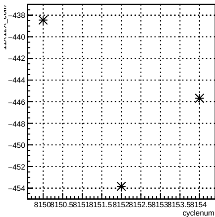
11X12X_coil7:cyclenum {run == 7151}
