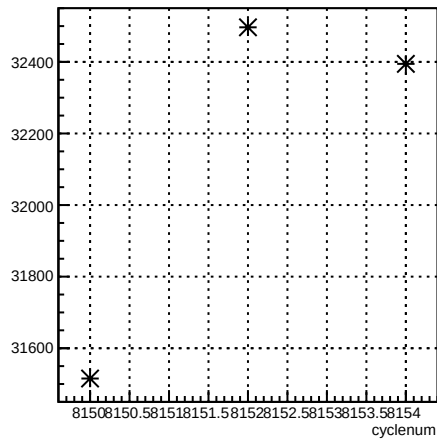
usl_coil6:cyclenum {run == 7151}
