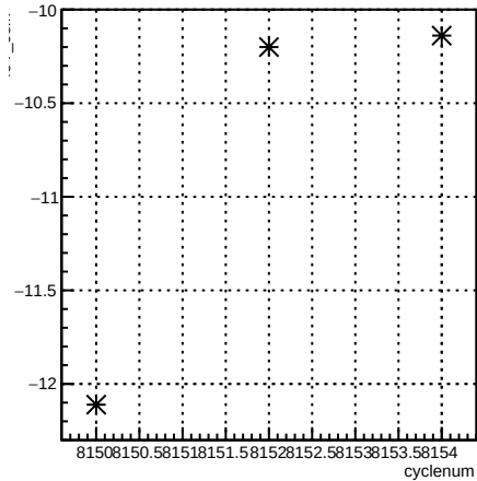
4eY_coil7:cyclenum {run == 7151}
