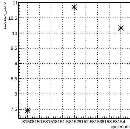
11X12X_coil6:cyclenum {run == 7151}
