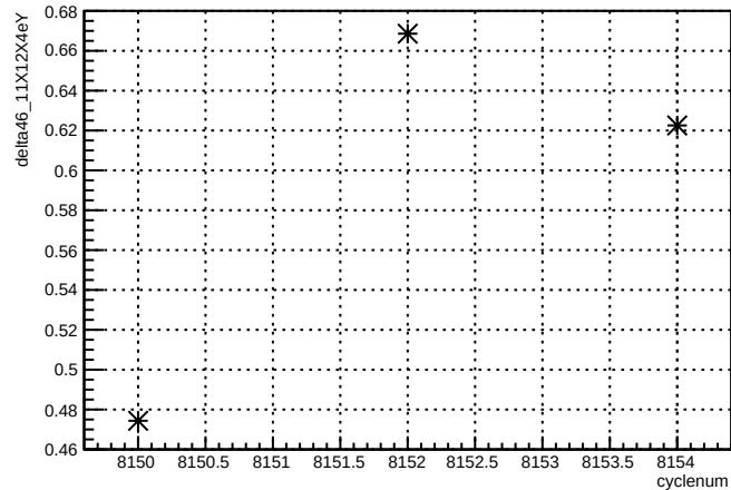
delta46_11X12X4eY:cyclenum {run == 7151}
