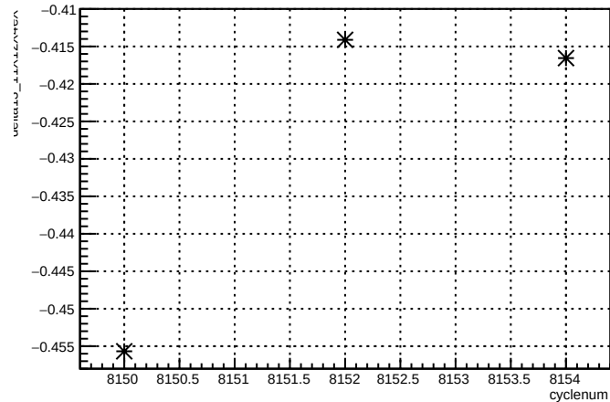
delta13_11X12X4eX:cyclenum {run == 7151}
