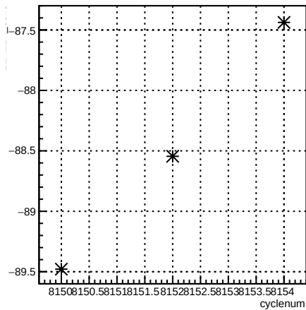
11X12X_coil3:cyclenum {run == 7151}
