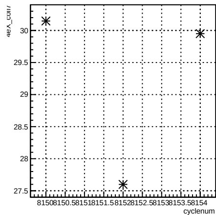
4eX_coil7:cyclenum {run == 7151}
