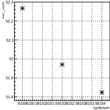
4eY_coil6:cyclenum {run == 7151}
