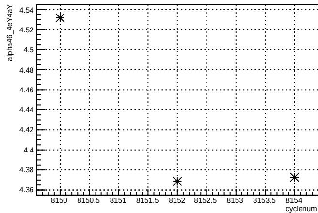
alpha46_4eY4aY:cyclenum {run == 7151}
