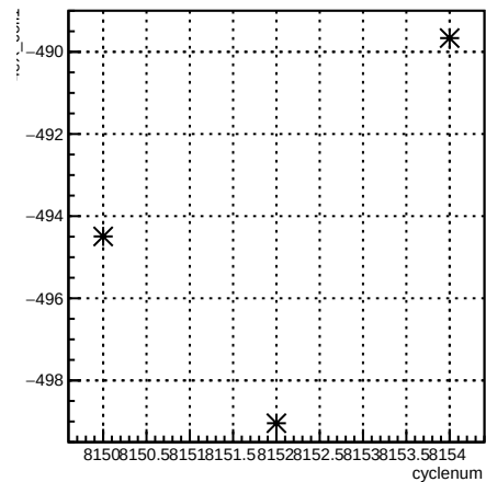
4eX_coil1:cyclenum {run == 7151}
