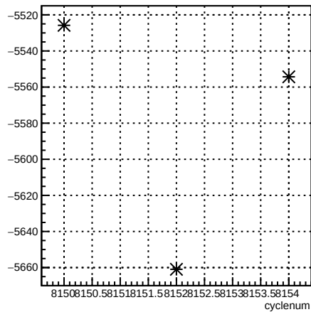
usr_coil7:cyclenum {run == 7151}
