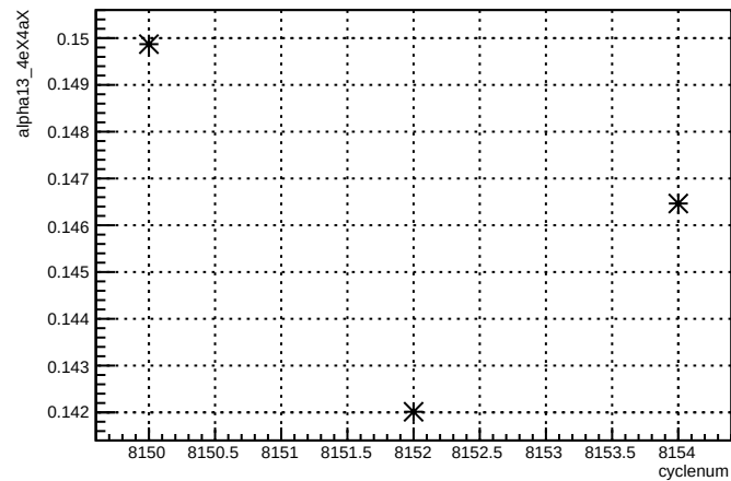
alpha13_4eX4aX:cyclenum {run == 7151}
