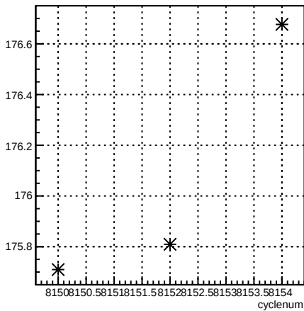
4eY_coil4:cyclenum {run == 7151}
