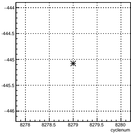
4eX_coil1:cyclenum {run == 7180}
