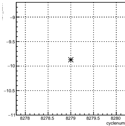
4eY_coil7:cyclenum {run == 7180}
