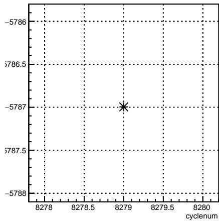
usr_coil7:cyclenum {run == 7180}
