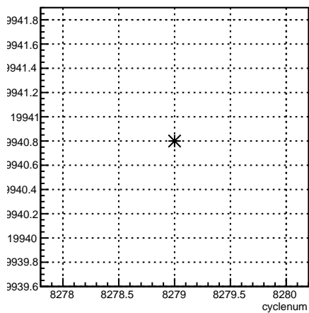
usr_coil7:cyclenum {run == 7180}
