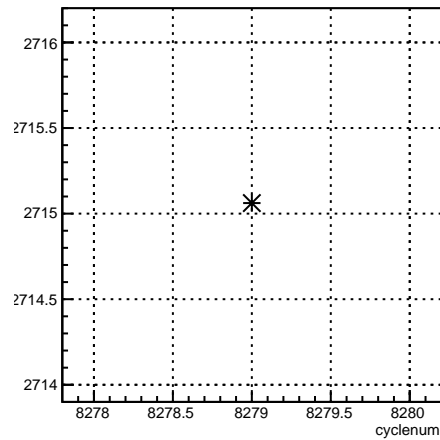
run:cyclenum {run == 7180}
