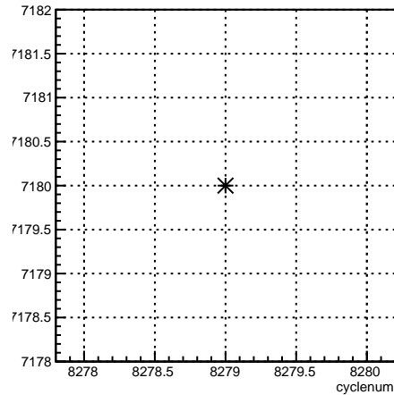
run:cyclenum {run == 7180}
