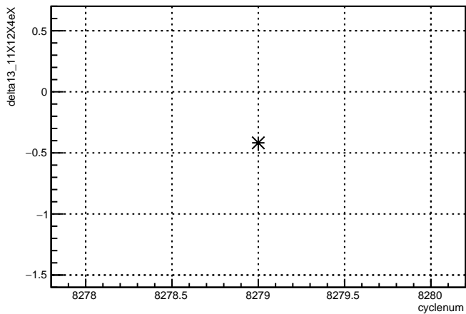
delta13_11X12X4eX:cyclenum {run == 7180}
