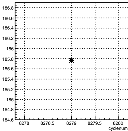
4eY_coil4:cyclenum {run == 7180}
