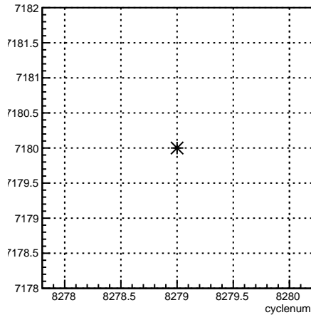
run:cyclenum {run == 7180}
