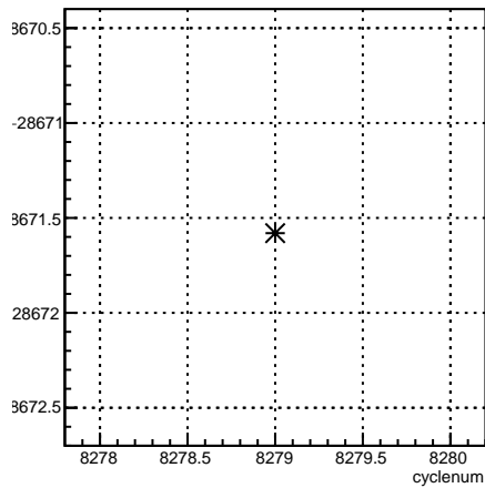
usr_coil6:cyclenum {run == 7180}
