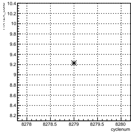
11X12X_coil6:cyclenum {run == 7180}
