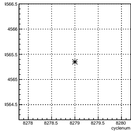
usl_coil4:cyclenum {run == 7180}
