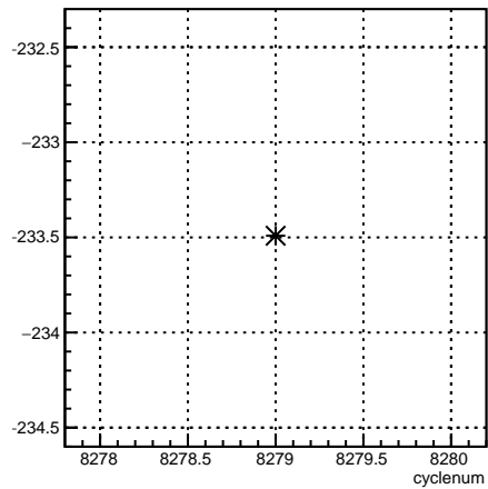
11X12X_coil6:cyclenum {run == 7180}
