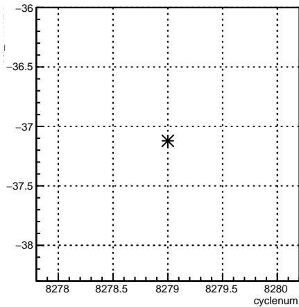
usl_11X12X:cyclenum {run == 7180}
