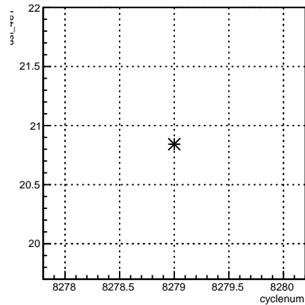
usl_4eY:cyclenum {run == 7180}
