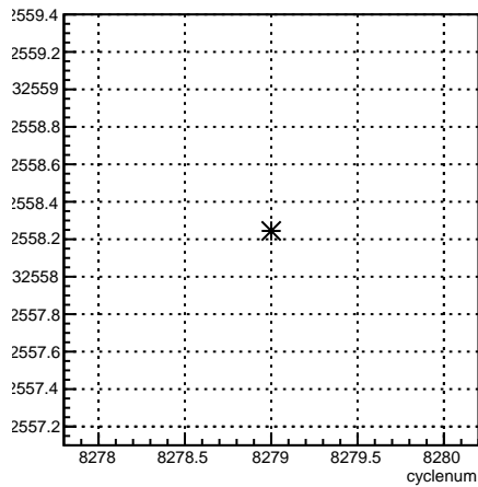
usl_coil1:cyclenum {run == 7180}
