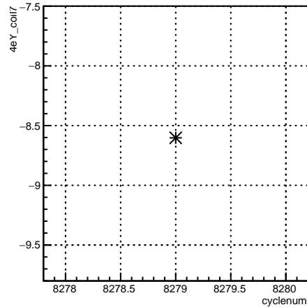
4eY_coil7:cyclenum {run == 7180}
