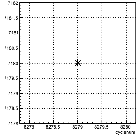
run:cyclenum {run == 7180}
