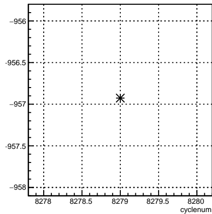
usl_coil6:cyclenum {run == 7180}
