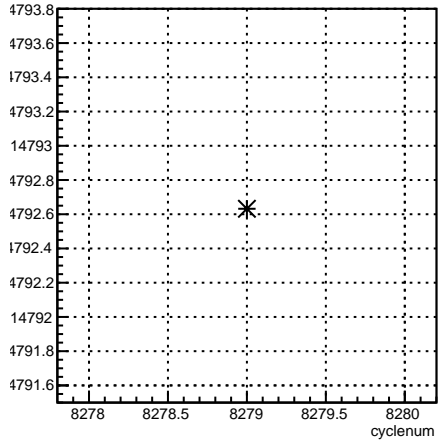
usl_coil7:cyclenum {run == 7180}
