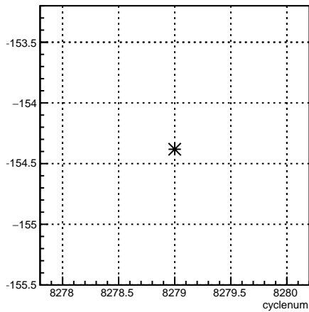
usr_4eY:cyclenum {run == 7180}
