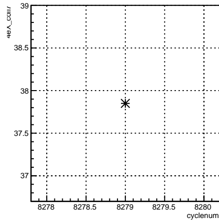
4eX_coil7:cyclenum {run == 7180}
