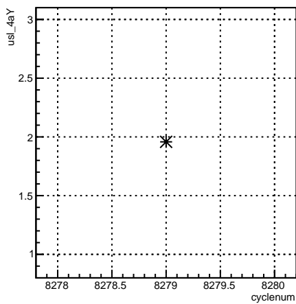
usl_4aY:cyclenum {run == 7180}
