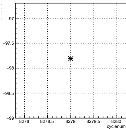
4eX_coil3:cyclenum {run == 7180}
