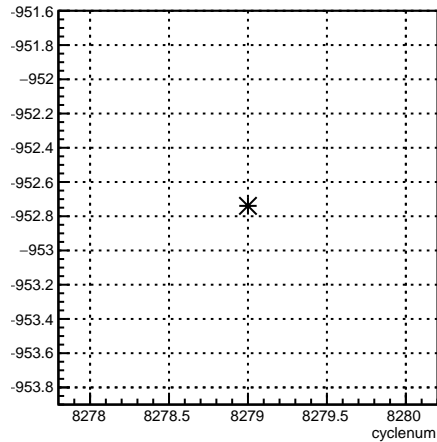
usr_coil6:cyclenum {run == 7180}
