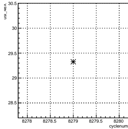
usl_4eX:cyclenum {run == 7180}
