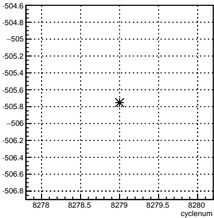
4eX_coil1:cyclenum {run == 7180}
