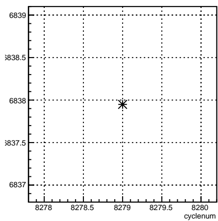
usl_coil3:cyclenum {run == 7180}
