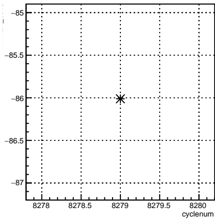
11X12X_coil7:cyclenum {run == 7180}
