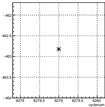
11X12X_coil7:cyclenum {run == 7180}
