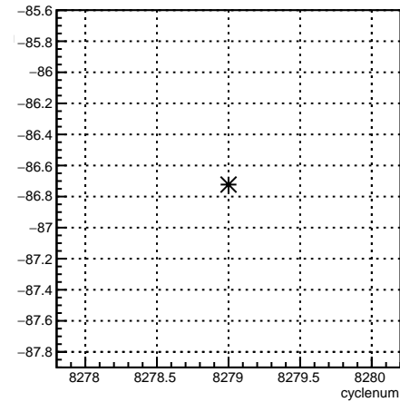
usl_4aX:cyclenum {run == 7180}
