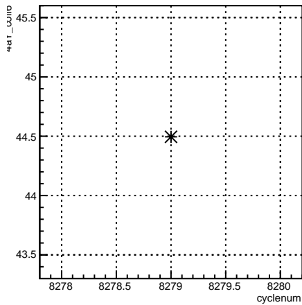
4eY_coil6:cyclenum {run == 7180}
