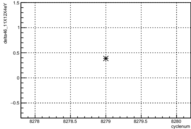
delta46_11X12X4eY:cyclenum {run == 7180}
