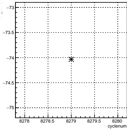
4eX_coil3:cyclenum {run == 7180}
