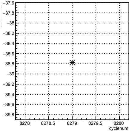
usr_11X12X:cyclenum {run == 7180}
