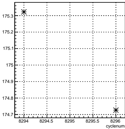
4eY_coil4:cyclenum {run == 7185}
