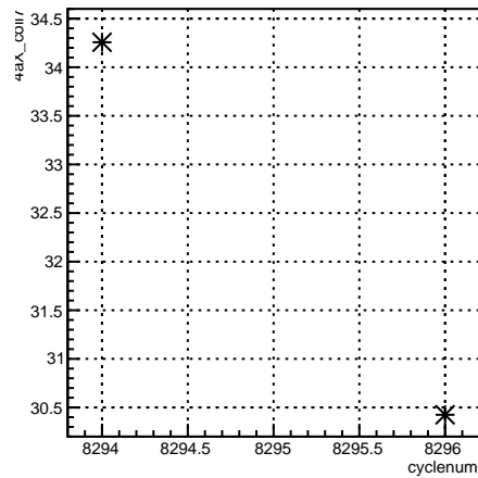
4eX_coil7:cyclenum {run == 7185}
