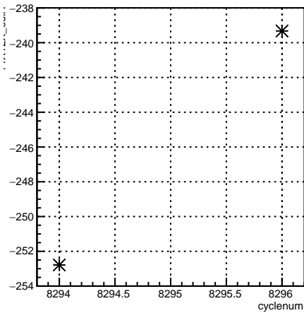
11X12X_coil1:cyclenum {run == 7185}
