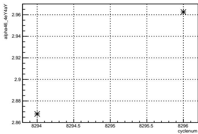
alpha46_4eY4aY:cyclenum {run == 7185}
