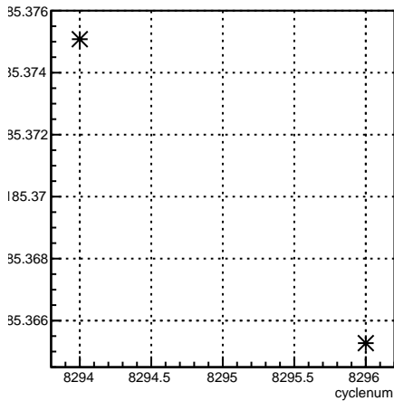
4eY_coil4:cyclenum {run == 7185}
