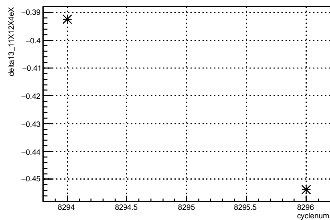
delta13_11X12X4eX:cyclenum {run == 7185}
