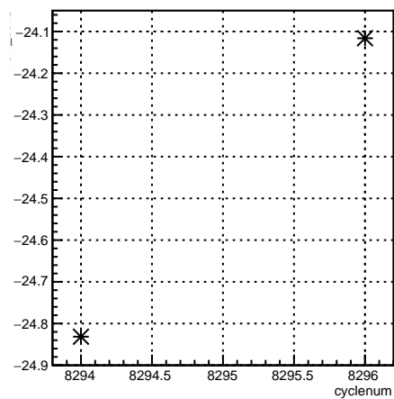
4eY_coil6:cyclenum {run == 7185}
