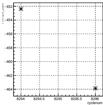
11X12X_coil7:cyclenum {run == 7185}
