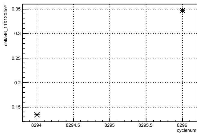
delta46_11X12X4eY:cyclenum {run == 7185}
