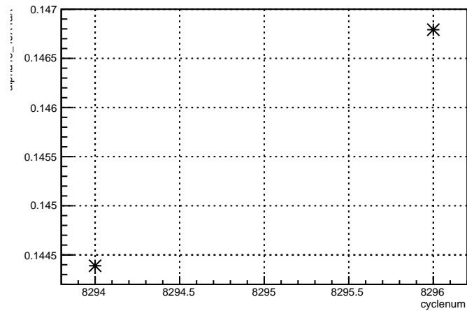
alpha13_4eX4aX:cyclenum {run == 7185}
