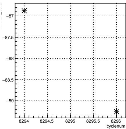
11X12X_coil3:cyclenum {run == 7185}
