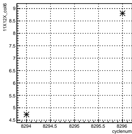
11X12X_coil6:cyclenum {run == 7185}
