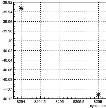
usr_11X12X:cyclenum {run == 7185}
