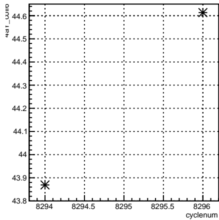
4eY_coil6:cyclenum {run == 7185}
