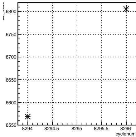
usl_coil7:cyclenum {run == 7185}
