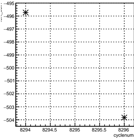
4eX_coil1:cyclenum {run == 7185}
