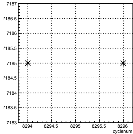
run:cyclenum {run == 7185}
