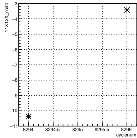
11X12X_coil4:cyclenum {run == 7185}
