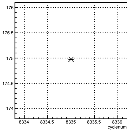
4eY_coil4:cyclenum {run == 7196}
