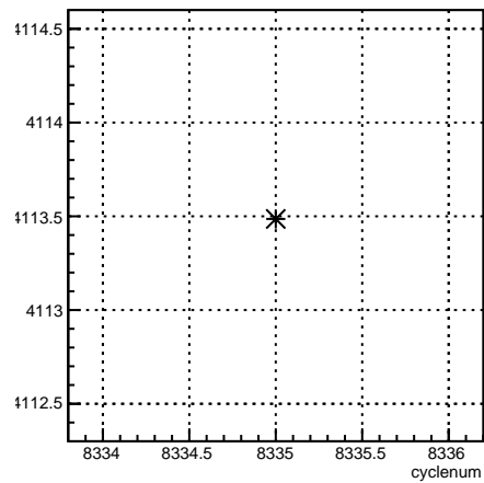
run:cyclenum {run == 7196}
