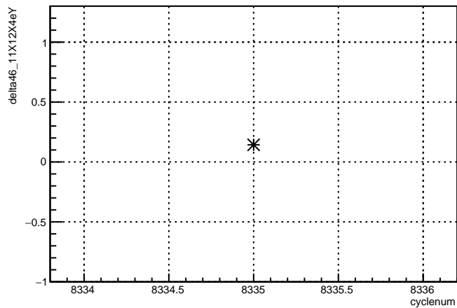
delta46_11X12X4eY:cyclenum {run == 7196}
