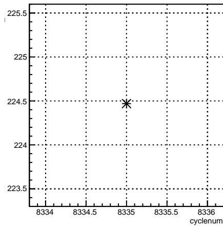
run:cyclenum {run == 7196}
