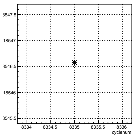
usl_coil7:cyclenum {run == 7196}
