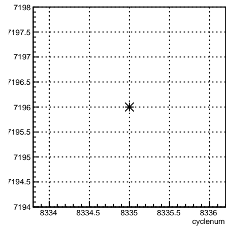
run:cyclenum {run == 7196}
