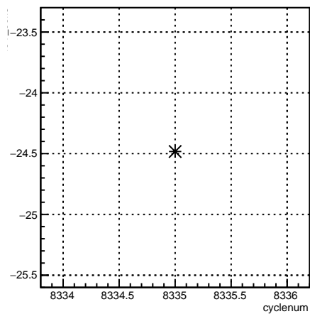
4eY_coil6:cyclenum {run == 7196}
