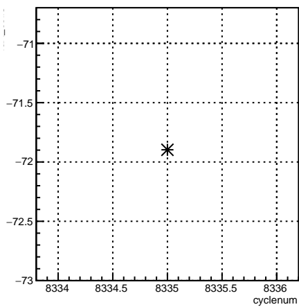
4aX_coil3:cyclenum {run == 7196}
