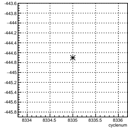
4aX_coil1:cyclenum {run == 7196}
