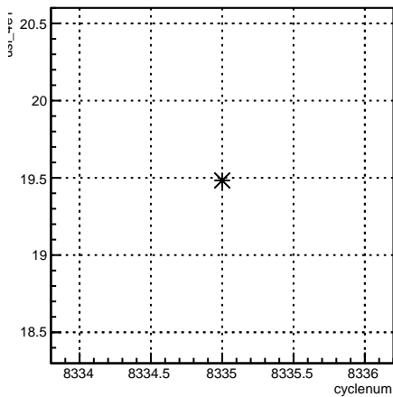
usl_4eY:cyclenum {run == 7196}
