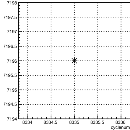
run:cyclenum {run == 7196}
