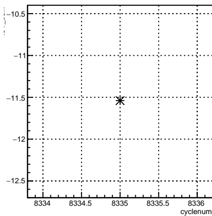
4eY_coil7:cyclenum {run == 7196}
