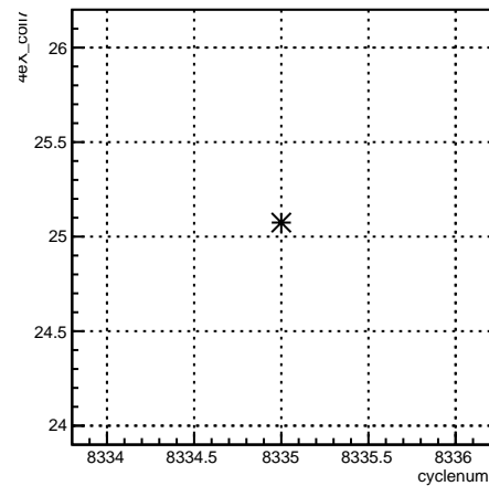
4eX_coil7:cyclenum {run == 7196}
