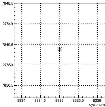
usr_coil1:cyclenum {run == 7196}
