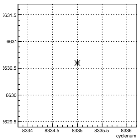
usl_coil3:cyclenum {run == 7196}
