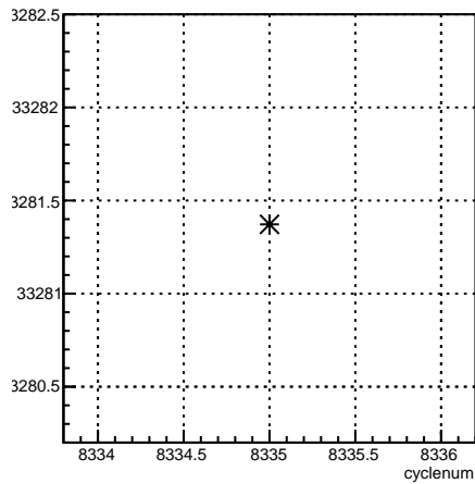
usl_coil1:cyclenum {run == 7196}
