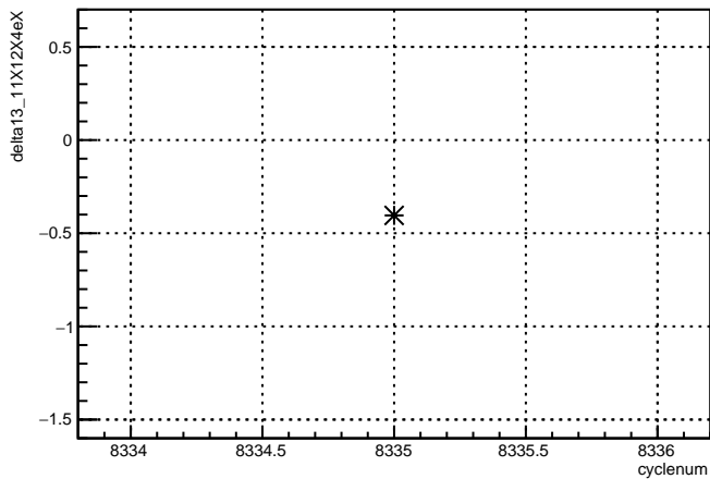
delta13_11X12X4eX:cyclenum {run == 7196}
