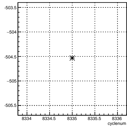
4eX_coil1:cyclenum {run == 7196}
