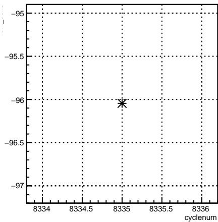
4eX_coil3:cyclenum {run == 7196}
