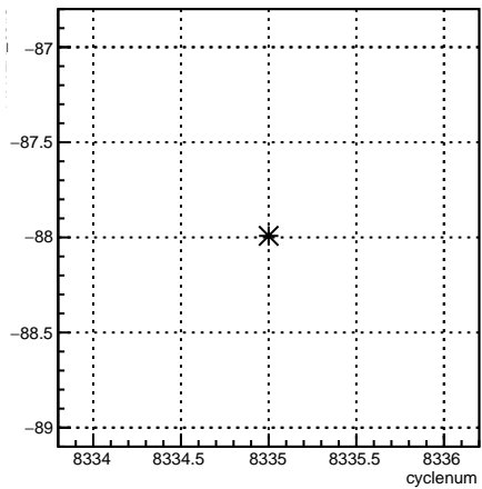
11X12X_coil7:cyclenum {run == 7196}
