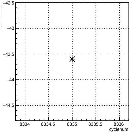
usr_11X12X:cyclenum {run == 7196}
