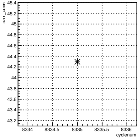
4eY_coil6:cyclenum {run == 7196}
