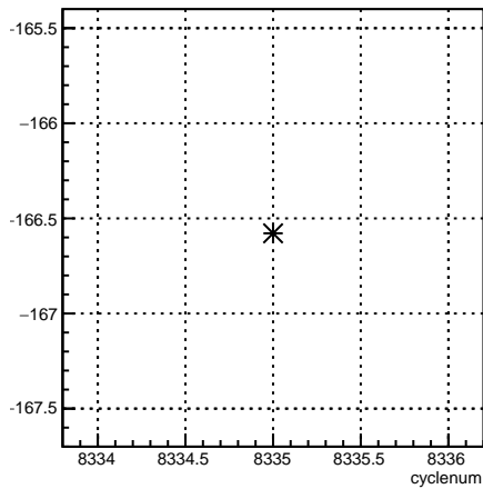
usr_4eY:cyclenum {run == 7196}
