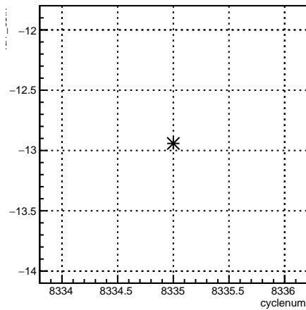
4eY_coil7:cyclenum {run == 7196}
