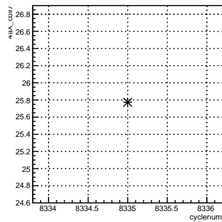
4aX_coil7:cyclenum {run == 7196}
