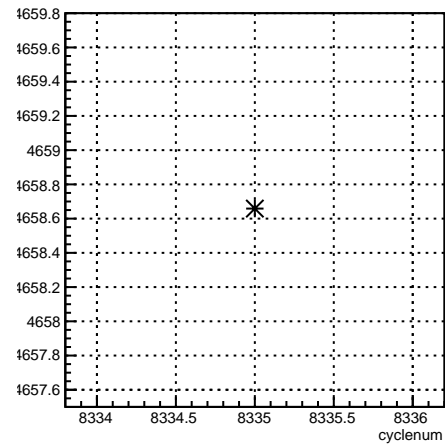
usl_coil4:cyclenum {run == 7196}
