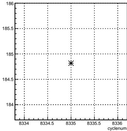
4eY_coil4:cyclenum {run == 7196}
