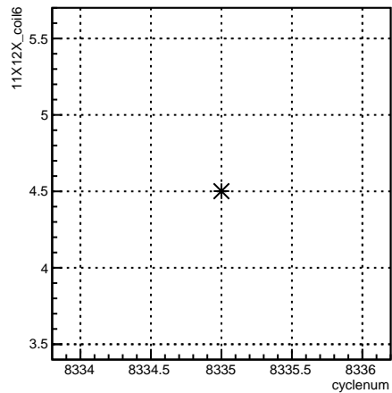
11X12X_coil6:cyclenum {run == 7196}
