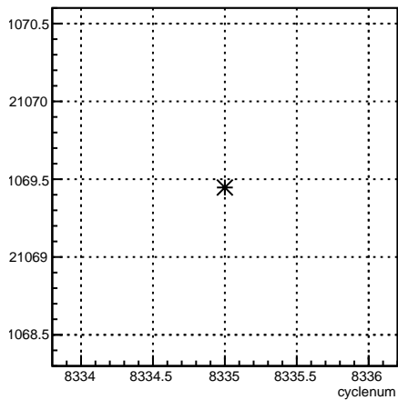
usr_coil7:cyclenum {run == 7196}
