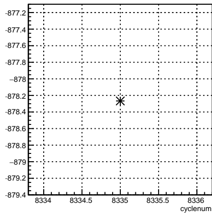
usr_coil6:cyclenum {run == 7196}
