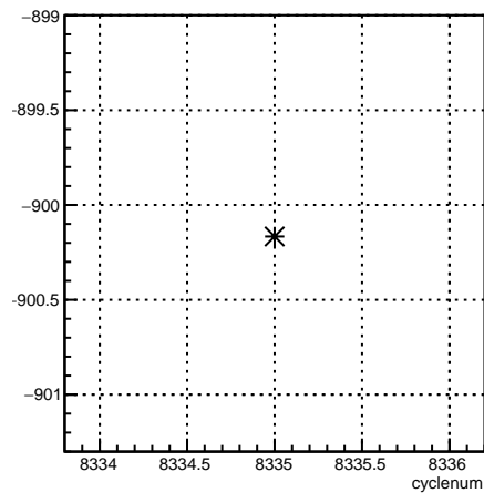
usl_coil6:cyclenum {run == 7196}
