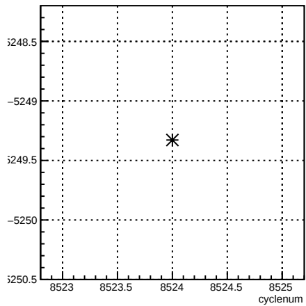
usr_coil7:cyclenum {run == 7260}
