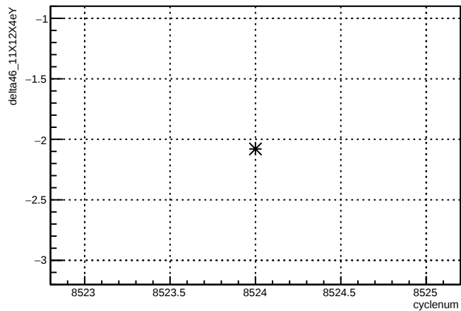
delta46_11X12X4eY:cyclenum {run == 7260}
