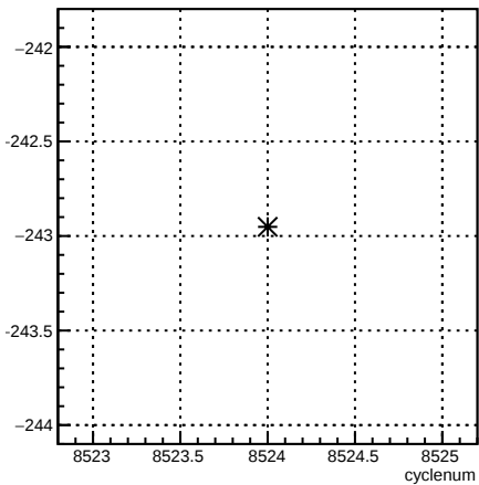
11X12X_coil1:cyclenum {run == 7260}
