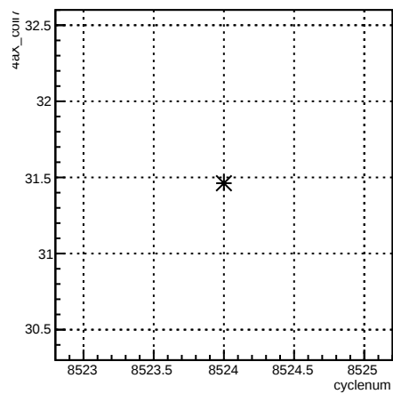
4aX_coil7:cyclenum {run == 7260}
