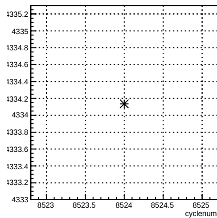
usl_coil4:cyclenum {run == 7260}
