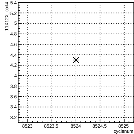
11X12X_coil4:cyclenum {run == 7260}
