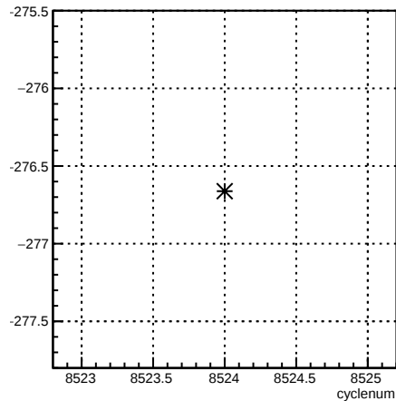
usl_coil6:cyclenum {run == 7260}
