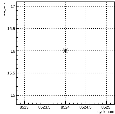
usl_4eY:cyclenum {run == 7260}
