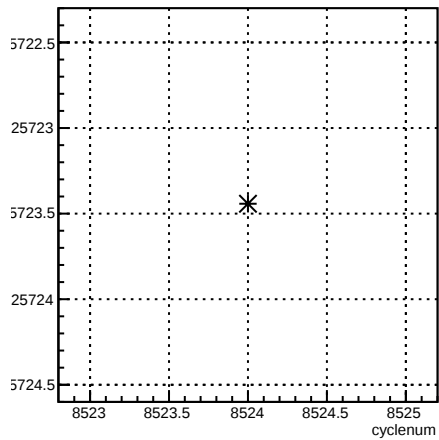
usr_coil6:cyclenum {run == 7260}
