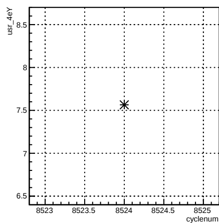
usr_4eY:cyclenum {run == 7260}
