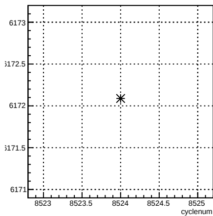
usl_coil3:cyclenum {run == 7260}
