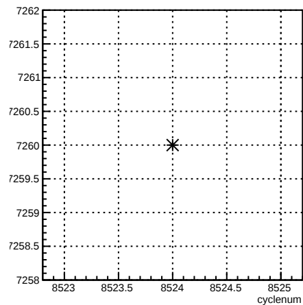
run:cyclenum {run == 7260}
