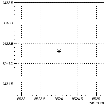
usl_coil1:cyclenum {run == 7260}
