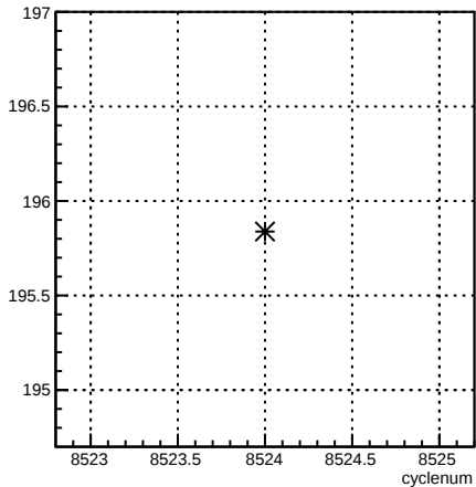
4eY_coil4:cyclenum {run == 7260}
