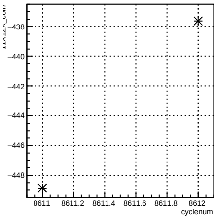
11X12X_coil7:cyclenum {run == 7296}
