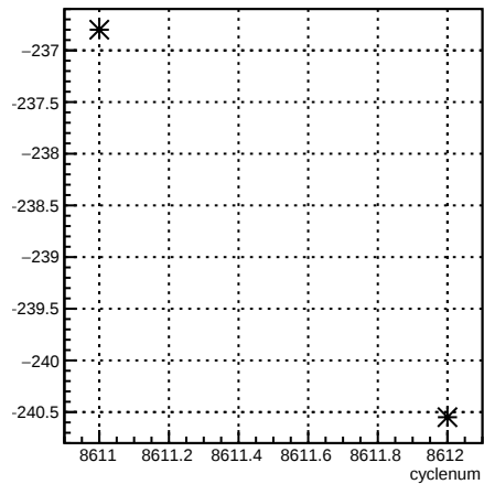
11X12X_coil1:cyclenum {run == 7296}
