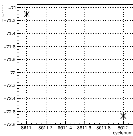
4aX_coil3:cyclenum {run == 7296}
