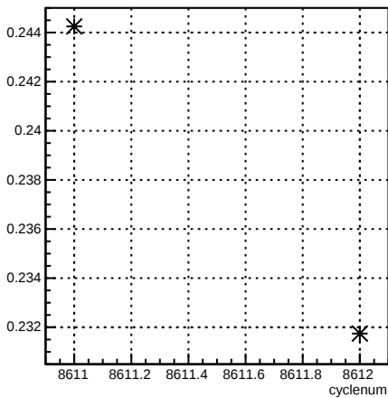
delta46_11X12X4eY:cyclenum {run == 7296}
