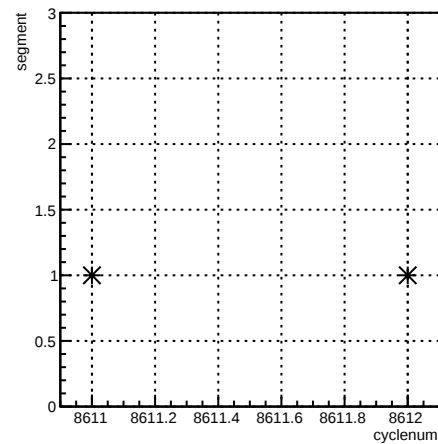
segment:cyclenum {run == 7296}
