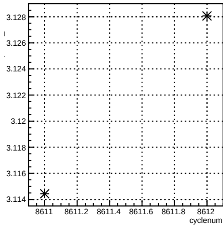
alpha46_4eY4aY:cyclenum {run == 7296}
