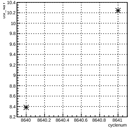
usr_11X12X:cyclenum {run == 7306}
