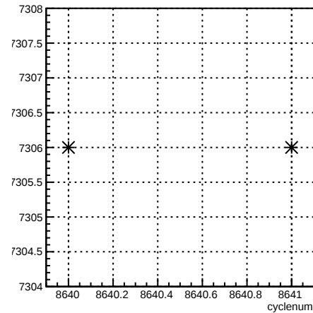
run:cyclenum {run == 7306}
