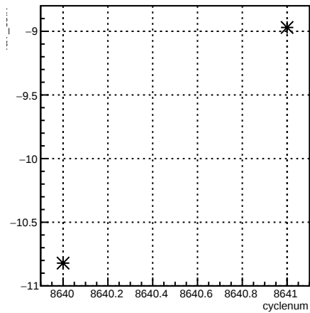
4eY_coil7:cyclenum {run == 7306}
