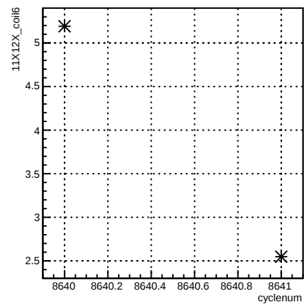
11X12X_coil6:cyclenum {run == 7306}
