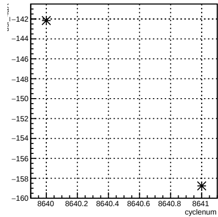
usr_4eY:cyclenum {run == 7306}
