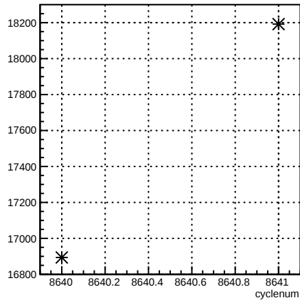
usr_coil7:cyclenum {run == 7306}
