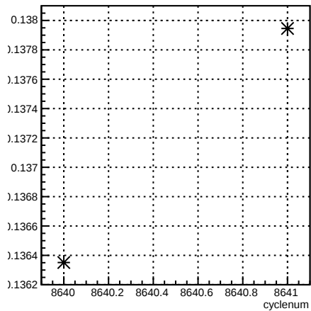
alpha13_4eX4aX:cyclenum {run == 7306}
