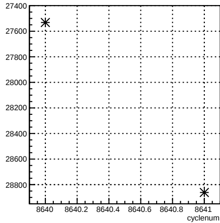
usr_coil1:cyclenum {run == 7306}
