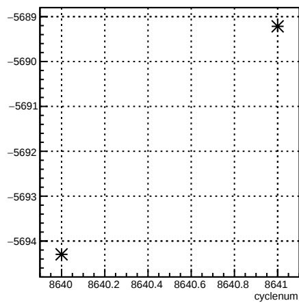
usr_coil3:cyclenum {run == 7306}
