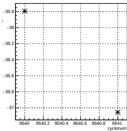
usl_11X12X:cyclenum {run == 7306}
