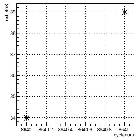
usl_4eX:cyclenum {run == 7306}
