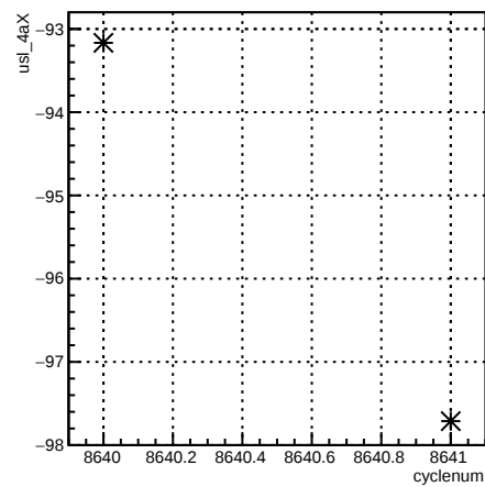
usl_4aX:cyclenum {run == 7306}
