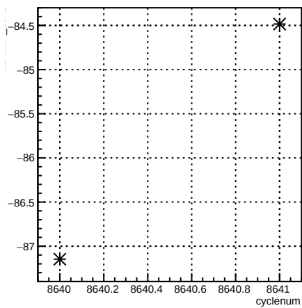
11X12X_coil3:cyclenum {run == 7306}
