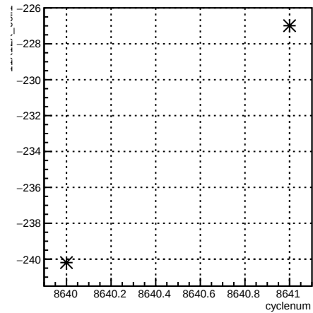
11X12X_coil1:cyclenum {run == 7306}
