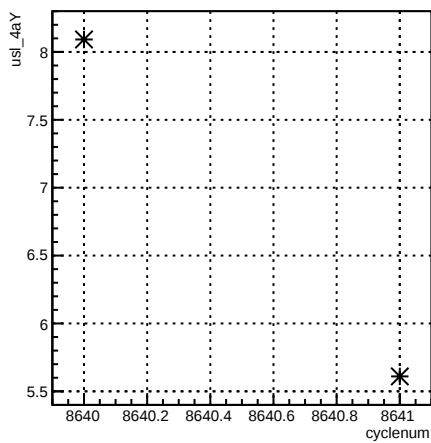
usl_4aY:cyclenum {run == 7306}
