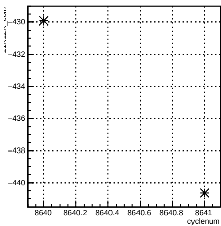
11X12X_coil7:cyclenum {run == 7306}
