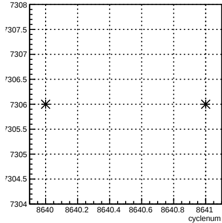
run:cyclenum {run == 7306}
