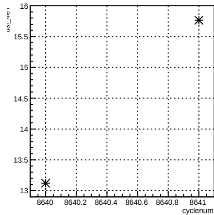
usl_4eY:cyclenum {run == 7306}
