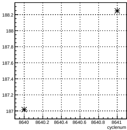
4eY_coil4:cyclenum {run == 7306}
