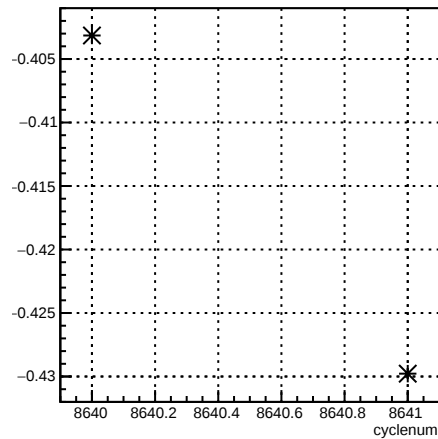
delta13_11X12X4eX:cyclenum {run == 7306}
