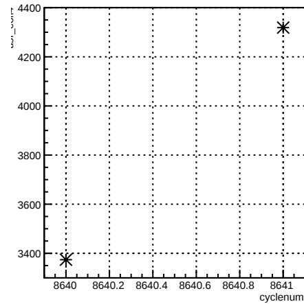
usr_coil4:cyclenum {run == 7306}
