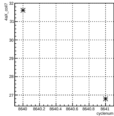
4aX_coil7:cyclenum {run == 7306}
