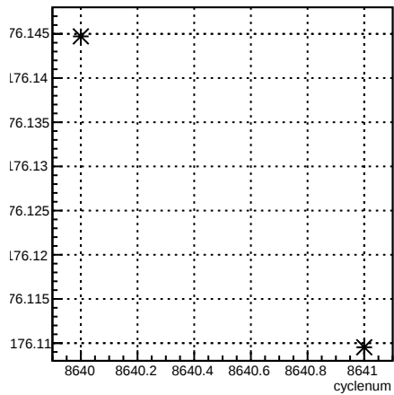
4eY_coil4:cyclenum {run == 7306}
