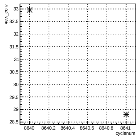
4eX_coil7:cyclenum {run == 7306}
