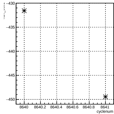
4aX_coil1:cyclenum {run == 7306}
