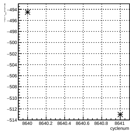
4eX_coil1:cyclenum {run == 7306}
