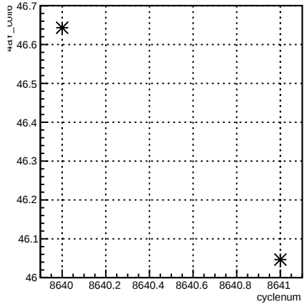
4eY_coil6:cyclenum {run == 7306}
