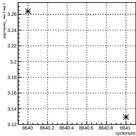
alpha46_4eY4aY:cyclenum {run == 7306}
