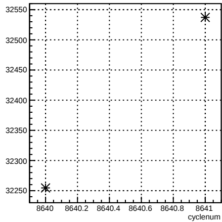
usl_coil6:cyclenum {run == 7306}
