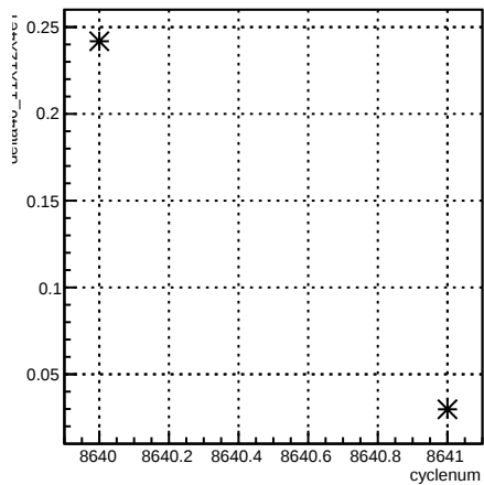
delta46_11X12X4eY:cyclenum {run == 7306}
