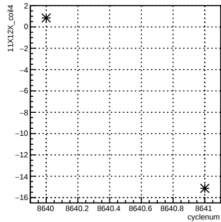
11X12X_coil4:cyclenum {run == 7306}
