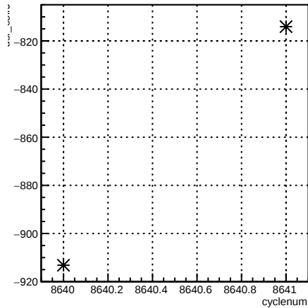
usr_coil6:cyclenum {run == 7306}
