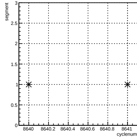
segment:cyclenum {run == 7306}
