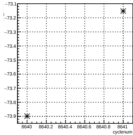
4aX_coil3:cyclenum {run == 7306}
