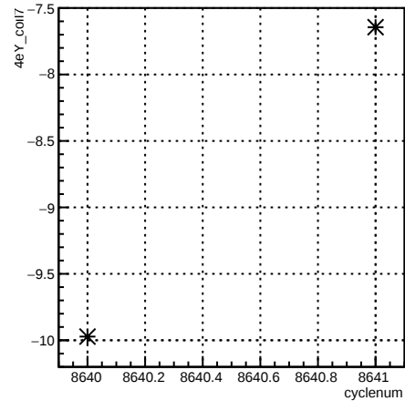
4eY_coil7:cyclenum {run == 7306}
