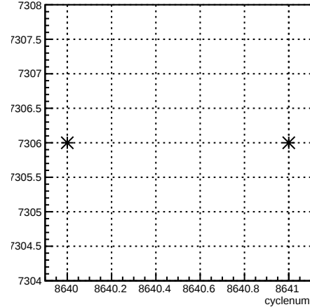
run:cyclenum {run == 7306}
