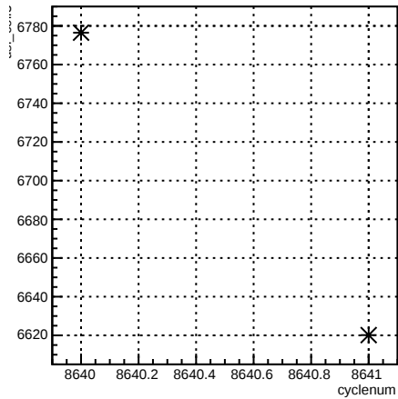
usl_coil7:cyclenum {run == 7306}
