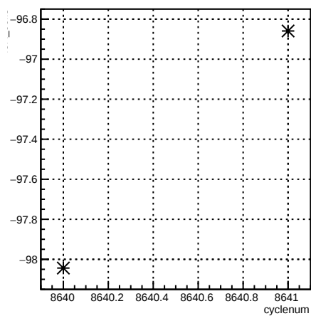
4eX_coil3:cyclenum {run == 7306}
