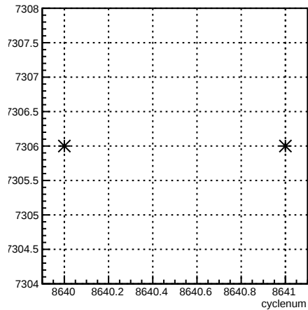
run:cyclenum {run == 7306}
