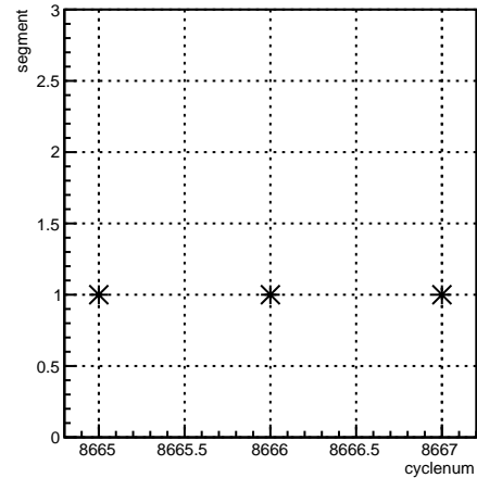
segment:cyclenum {run == 7313}
