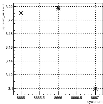
alpha46_4eY4aY:cyclenum {run == 7313}
