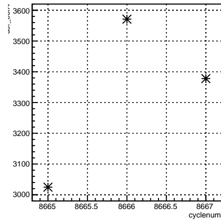
run:cyclenum {run == 7313}
