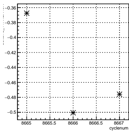
delta13_11X12X4eX:cyclenum {run == 7313}
