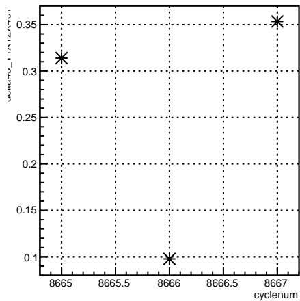
delta46_11X12X4eY:cyclenum {run == 7313}
