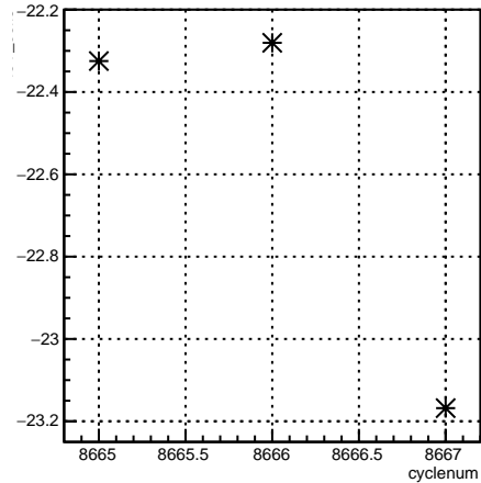
4eY_coil6:cyclenum {run == 7313}
