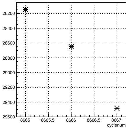
usr_coil6:cyclenum {run == 7313}
