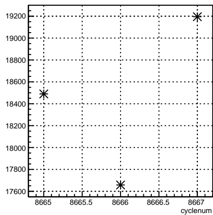
usr_coil7:cyclenum {run == 7313}
