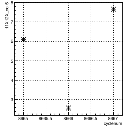
11X12X_coil6:cyclenum {run == 7313}
