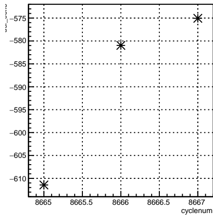
usl_coil6:cyclenum {run == 7313}
