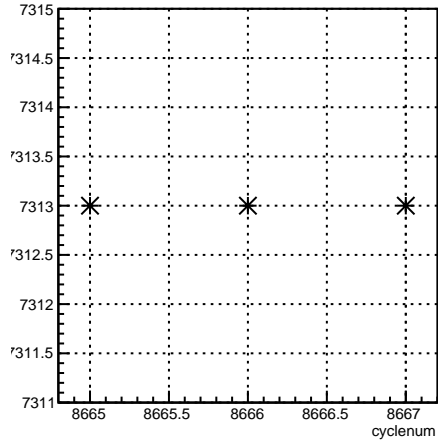
run:cyclenum {run == 7313}
