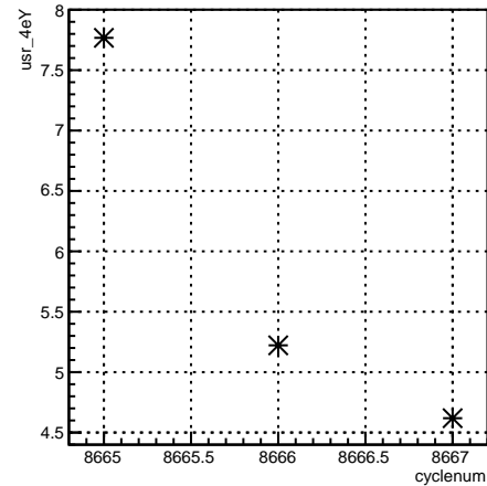
usr_4eY:cyclenum {run == 7313}
