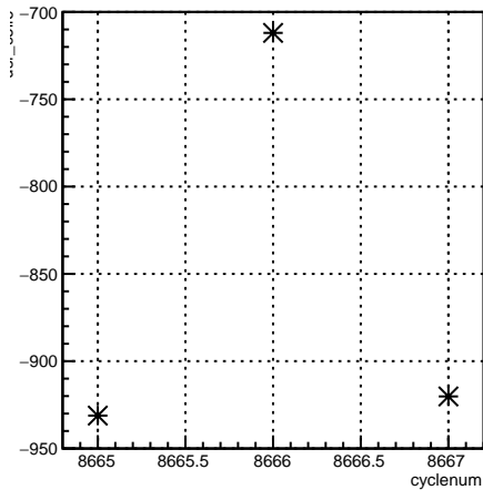
usr_coil6:cyclenum {run == 7313}
