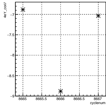
4eY_coil7:cyclenum {run == 7313}
