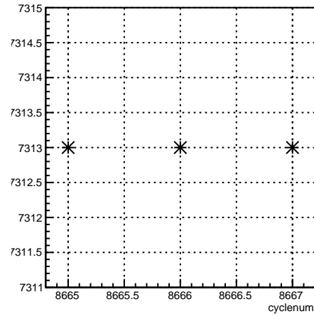
run:cyclenum {run == 7313}
