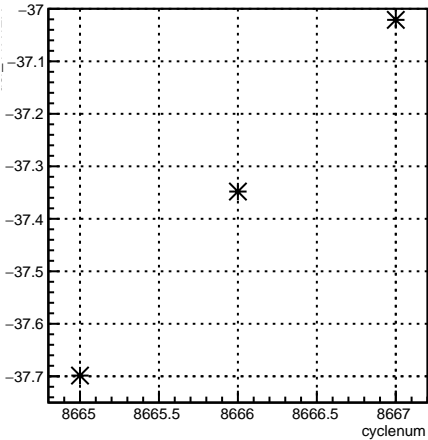
usr_11X12X:cyclenum {run == 7313}
