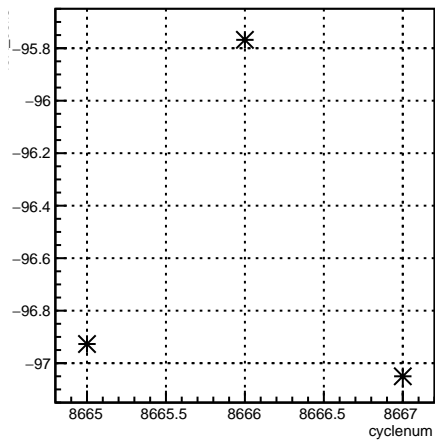
4eX_coil3:cyclenum {run == 7313}
