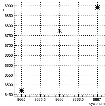
usl_coil7:cyclenum {run == 7313}
