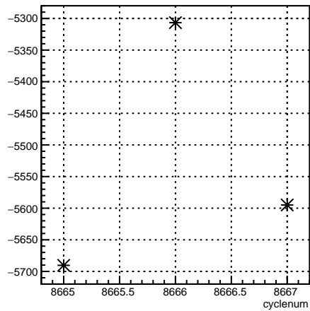
usr_coil7:cyclenum {run == 7313}
