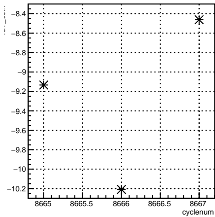
4eY_coil7:cyclenum {run == 7313}
