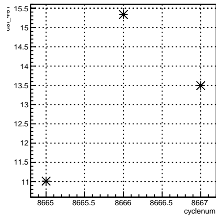
usl_4eY:cyclenum {run == 7313}
