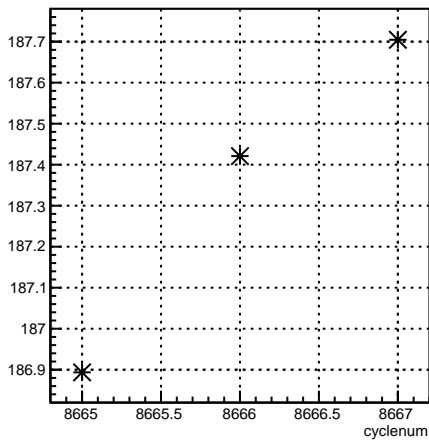
4eY_coil4:cyclenum {run == 7313}
