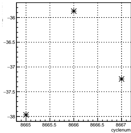
usl_11X12X:cyclenum {run == 7313}
