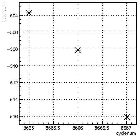
4eX_coil1:cyclenum {run == 7313}
