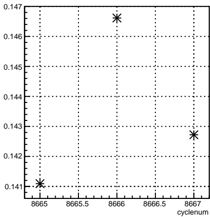
alpha13_4eX4aX:cyclenum {run == 7313}
