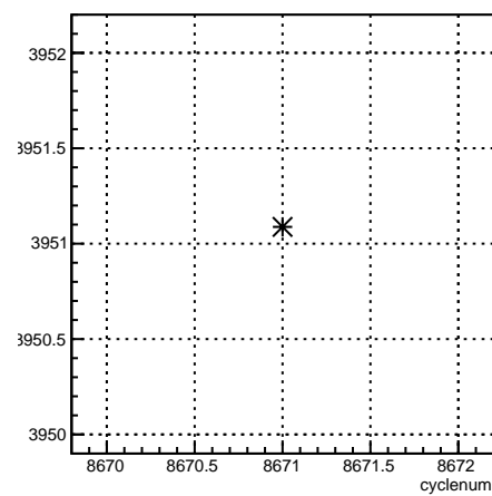
usl_coil4:cyclenum {run == 7314}
