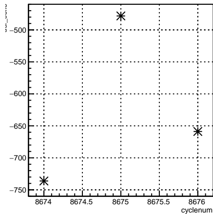
usl_coil6:cyclenum {run == 7315}
