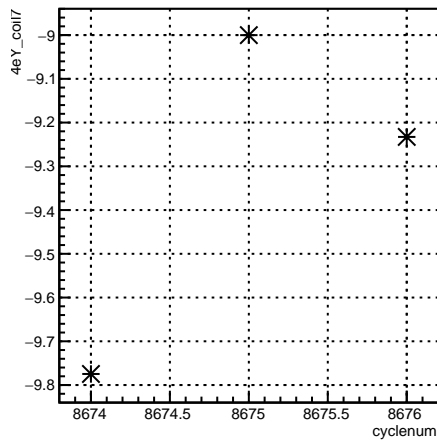
4eY_coil7:cyclenum {run == 7315}
