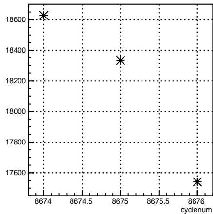
usr_coil7:cyclenum {run == 7315}
