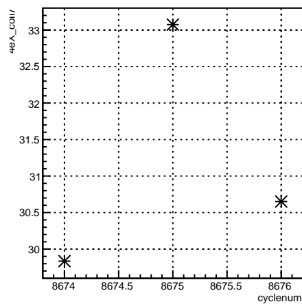
4eX_coil7:cyclenum {run == 7315}
