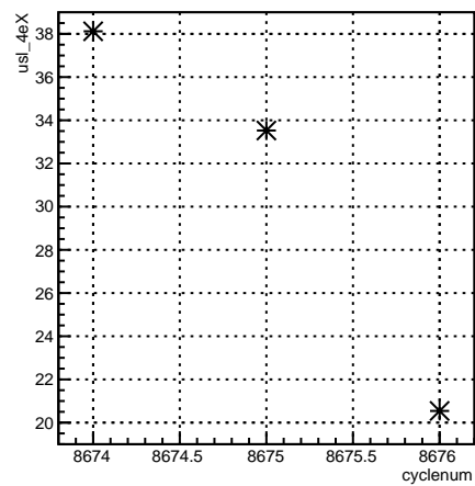
usl_4eX:cyclenum {run == 7315}
