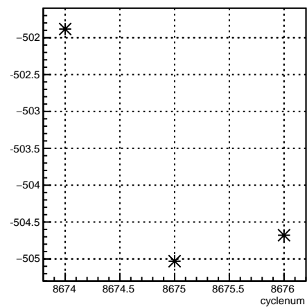
4eX_coil1:cyclenum {run == 7315}
