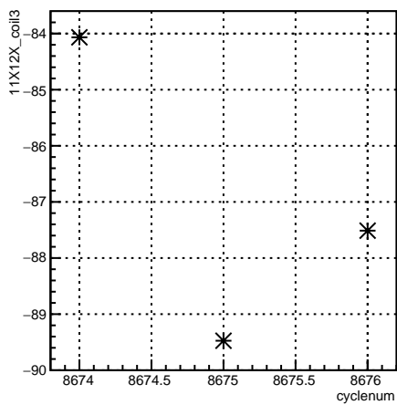
11X12X_coil3:cyclenum {run == 7315}
