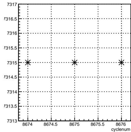
run:cyclenum {run == 7315}
