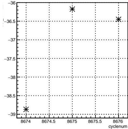
usr_11X12X:cyclenum {run == 7315}
