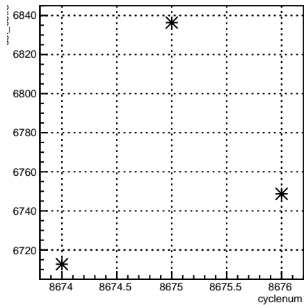
usl_coil7:cyclenum {run == 7315}
