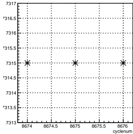
run:cyclenum {run == 7315}
