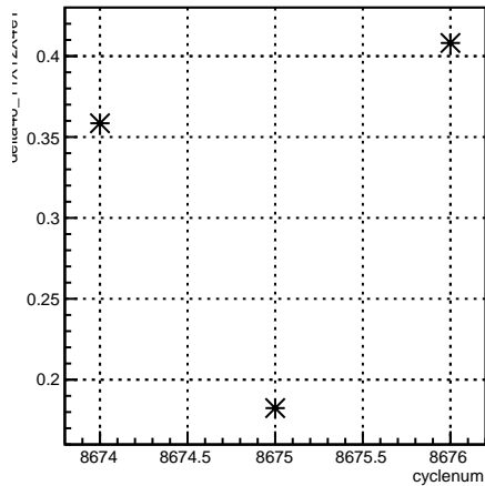
delta46_11X12X4eY:cyclenum {run == 7315}
