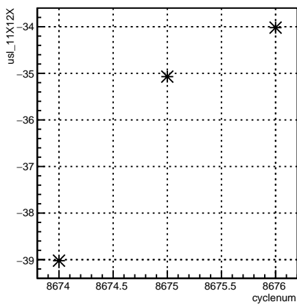
usl_11X12X:cyclenum {run == 7315}
