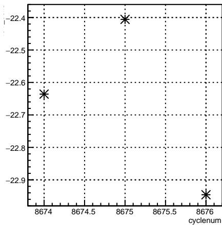
4eY_coil6:cyclenum {run == 7315}
