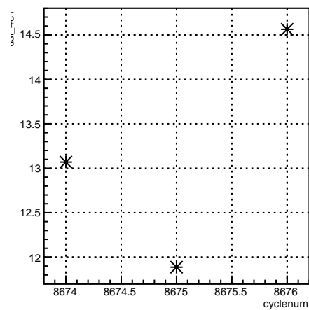
usl_4eY:cyclenum {run == 7315}
