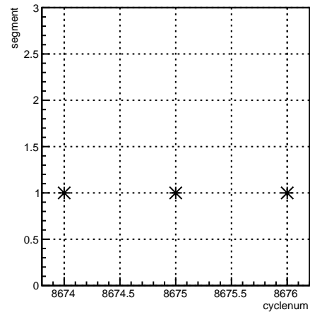
segment:cyclenum {run == 7315}
