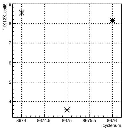
11X12X_coil6:cyclenum {run == 7315}
