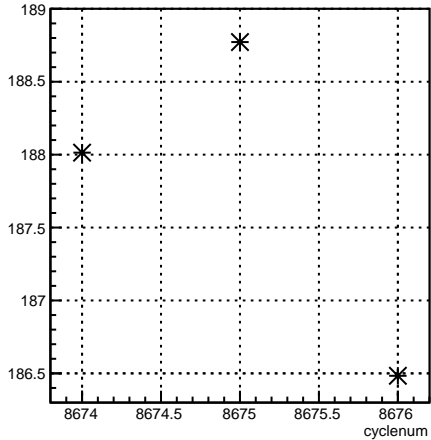
4eY_coil4:cyclenum {run == 7315}
