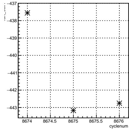
4aX_coil1:cyclenum {run == 7315}
