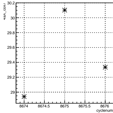
4aX_coil7:cyclenum {run == 7315}
