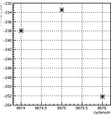
11X12X_coil1:cyclenum {run == 7315}
