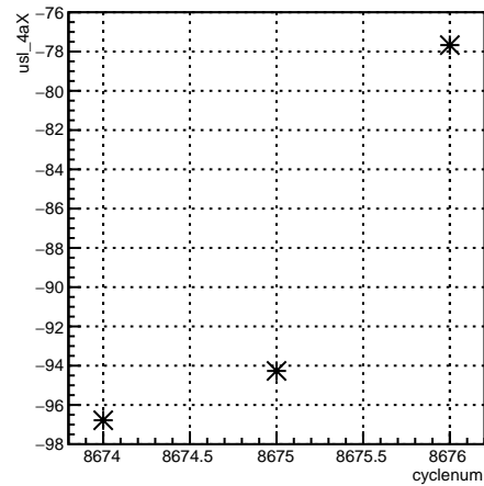
usl_4aX:cyclenum {run == 7315}
