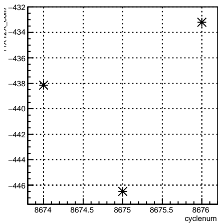
11X12X_coil7:cyclenum {run == 7315}
