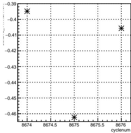
delta13_11X12X4eX:cyclenum {run == 7315}
