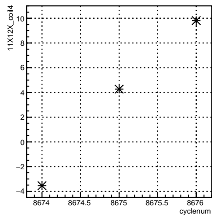
11X12X_coil4:cyclenum {run == 7315}
