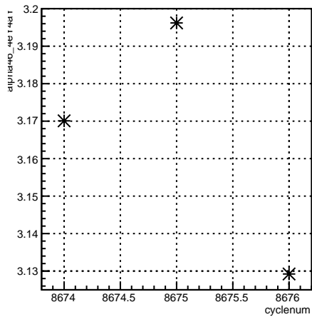
alpha46_4eY4aY:cyclenum {run == 7315}
