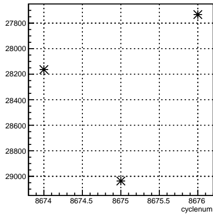
usr_coil6:cyclenum {run == 7315}
