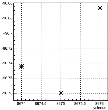
4eX_coil3:cyclenum {run == 7315}
