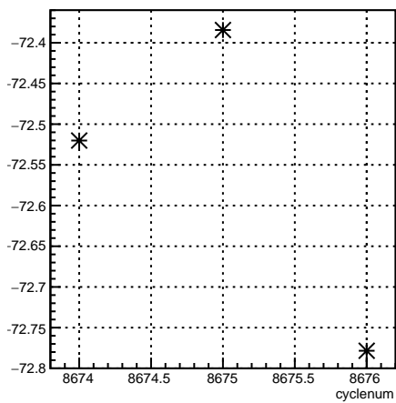
4aX_coil3:cyclenum {run == 7315}
