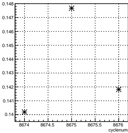
alpha13_4eX4aX:cyclenum {run == 7315}
