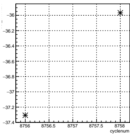
usr_11X12X:cyclenum {run == 7339}
