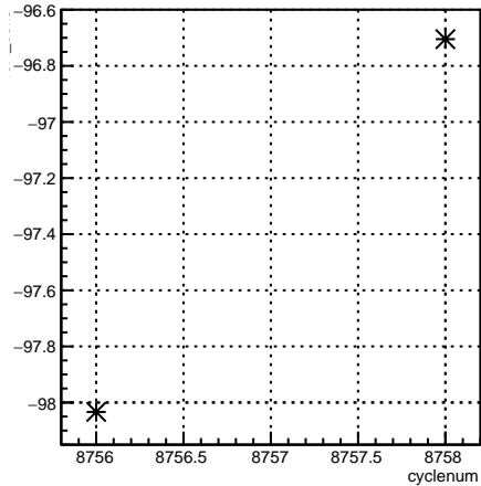
4eX_coil3:cyclenum {run == 7339}
