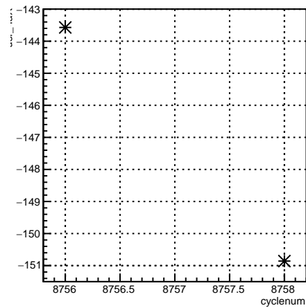
usr_4aX:cyclenum {run == 7339}
