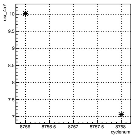
usr_4aY:cyclenum {run == 7339}
