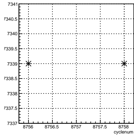
run:cyclenum {run == 7339}
