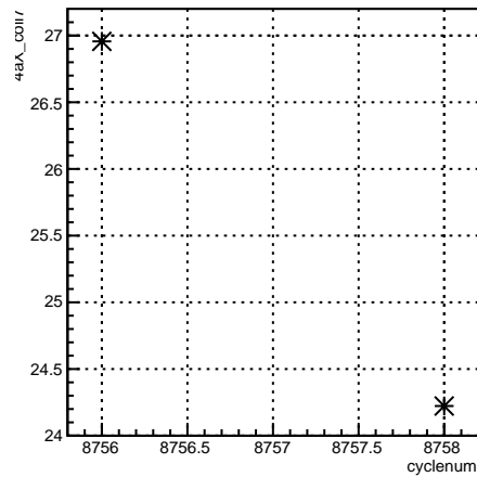
4eX_coil7:cyclenum {run == 7339}
