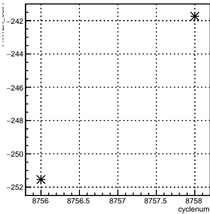
11X12X_coil1:cyclenum {run == 7339}
