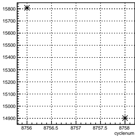
usl_coil7:cyclenum {run == 7339}
