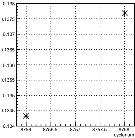
alpha13_4eX4aX:cyclenum {run == 7339}
