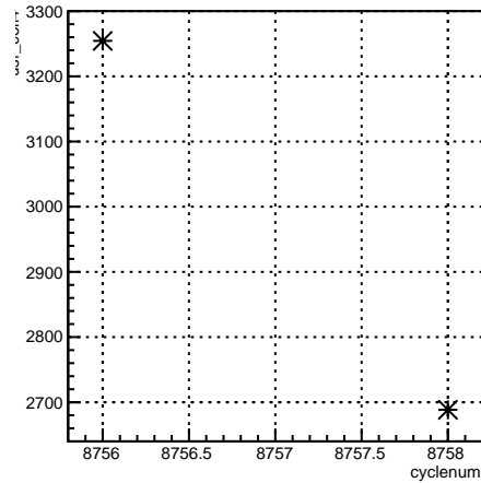
usr_coil4:cyclenum {run == 7339}
