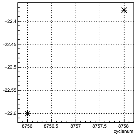
4eY_coil6:cyclenum {run == 7339}
