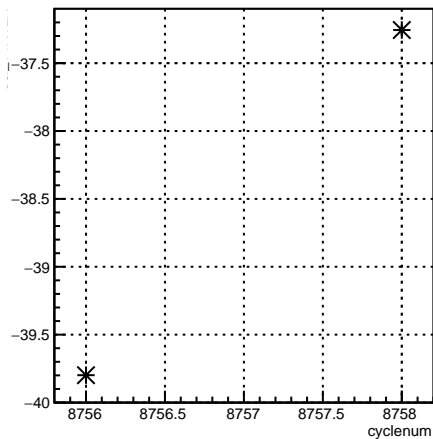
usl_11X12X:cyclenum {run == 7339}
