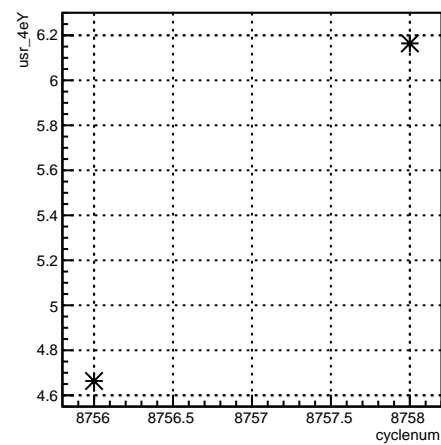
usr_4eY:cyclenum {run == 7339}
