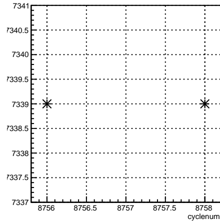
run:cyclenum {run == 7339}
