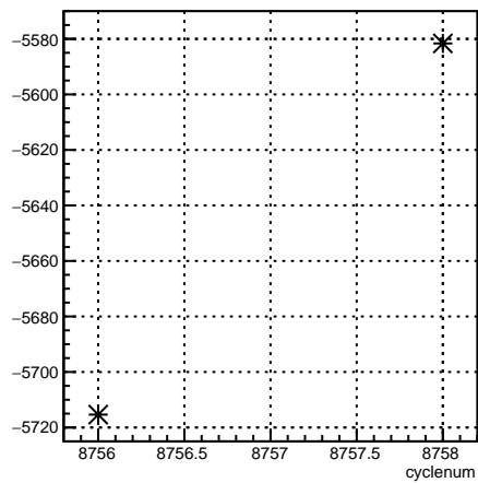
usr_coil3:cyclenum {run == 7339}
