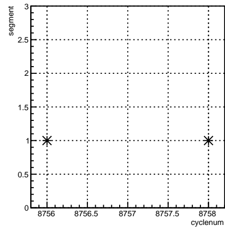
segment:cyclenum {run == 7339}
