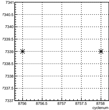
run:cyclenum {run == 7339}
