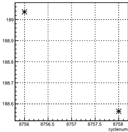
4eY_coil4:cyclenum {run == 7339}
