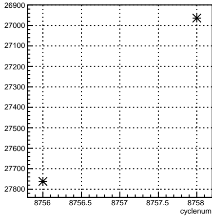
usr_coil1:cyclenum {run == 7339}
