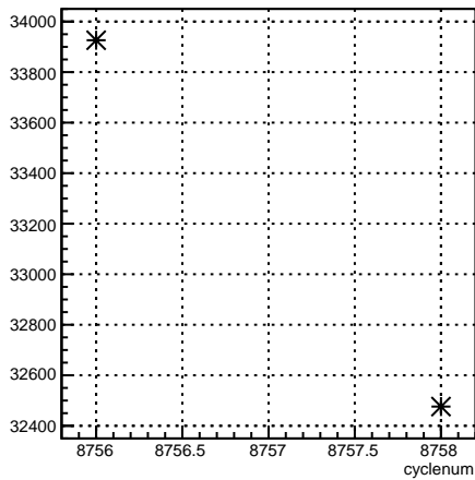
usl_coil6:cyclenum {run == 7339}
