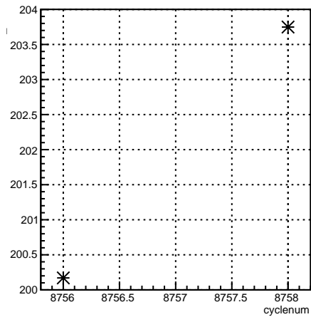
usr_4eX:cyclenum {run == 7339}
