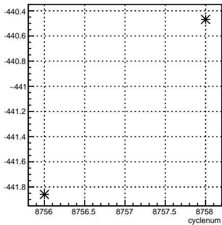
11X12X_coil7:cyclenum {run == 7339}
