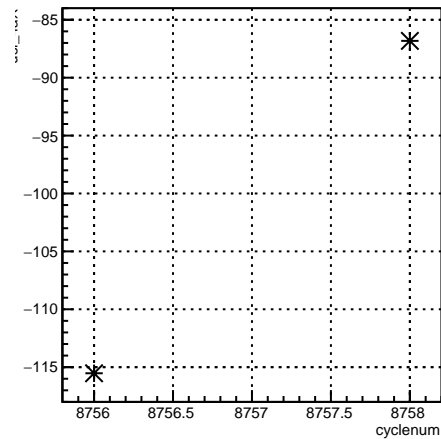
usl_4eY:cyclenum {run == 7339}
