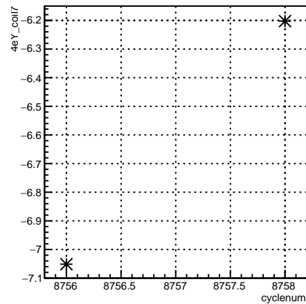
4eY_coil7:cyclenum {run == 7339}
