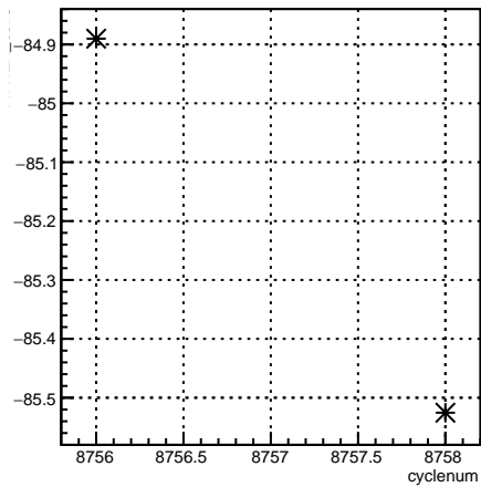
11X12X_coil3:cyclenum {run == 7339}
