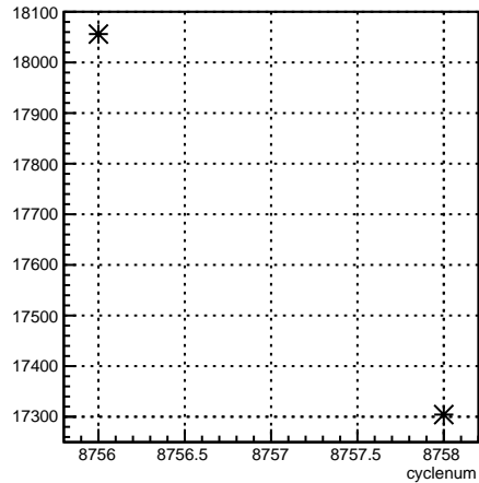
usr_coil7:cyclenum {run == 7339}
