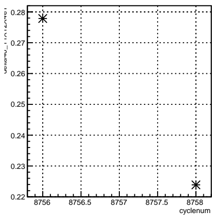
delta46_11X12X4eY:cyclenum {run == 7339}
