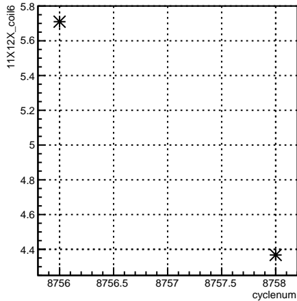
11X12X_coil6:cyclenum {run == 7339}
