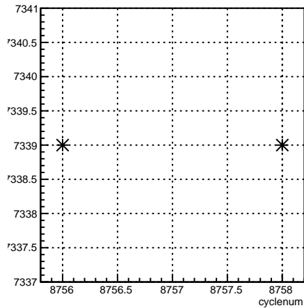
run:cyclenum {run == 7339}
