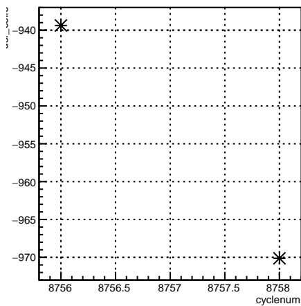
usr_coil6:cyclenum {run == 7339}
