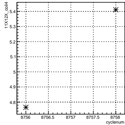
11X12X_coil4:cyclenum {run == 7339}
