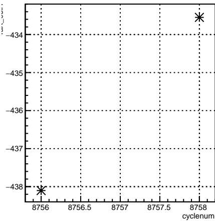
4eX_coil1:cyclenum {run == 7339}
