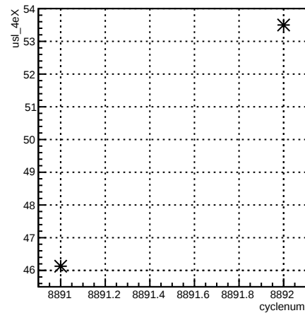
usl_4eX:cyclenum {run == 7373}
