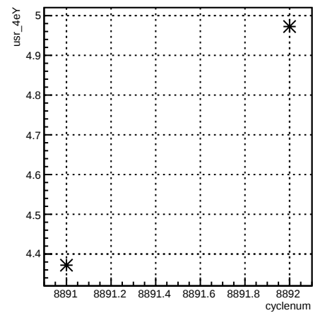
usr_4eY:cyclenum {run == 7373}
