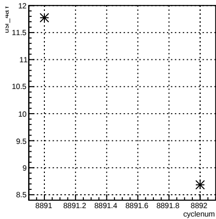
usr_4aY:cyclenum {run == 7373}
