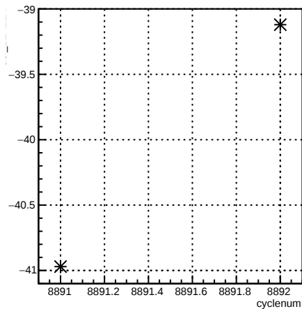
usl_11X12X:cyclenum {run == 7373}
