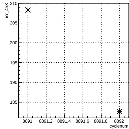
usr_4eX:cyclenum {run == 7373}
