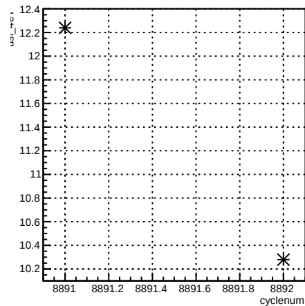
usl_4eY:cyclenum {run == 7373}
