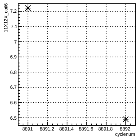
11X12X_coil6:cyclenum {run == 7373}
