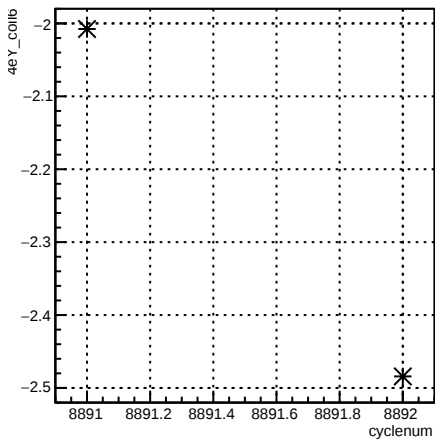
4eY_coil6:cyclenum {run == 7373}
