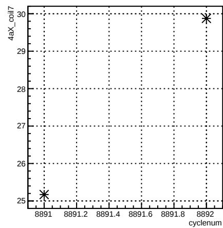
4aX_coil7:cyclenum {run == 7373}
