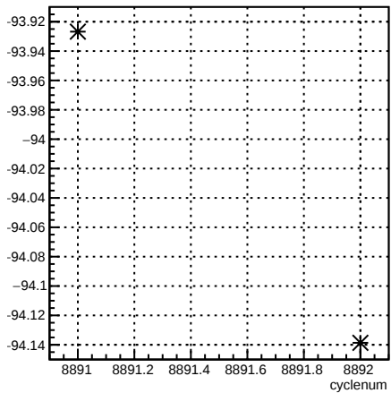
4eX_coil3:cyclenum {run == 7373}
