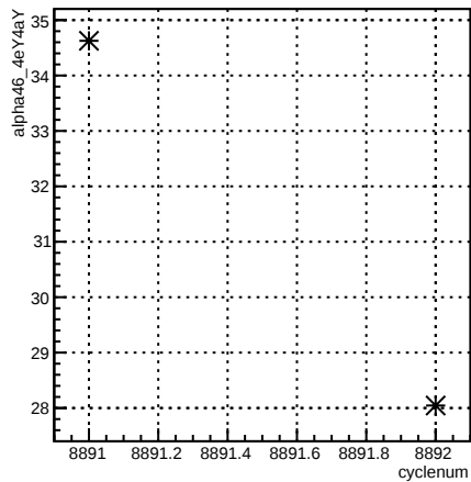
alpha46_4eY4aY:cyclenum {run == 7373}
