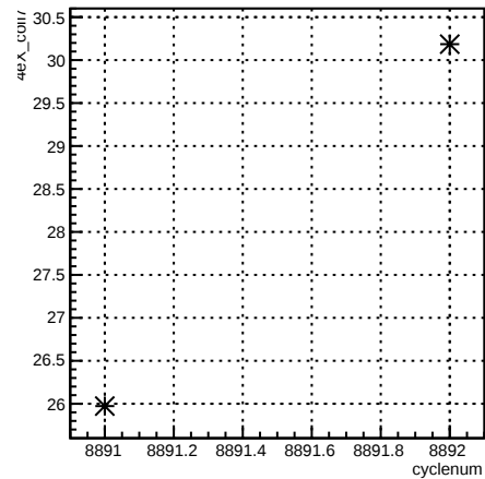
4eX_coil7:cyclenum {run == 7373}
