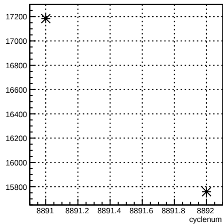
usl_coil7:cyclenum {run == 7373}
