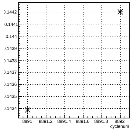
alpha13_4eX4aX:cyclenum {run == 7373}
