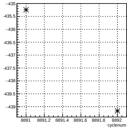
4aX_coil1:cyclenum {run == 7373}
