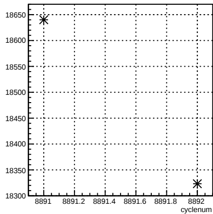
usr_coil7:cyclenum {run == 7373}
