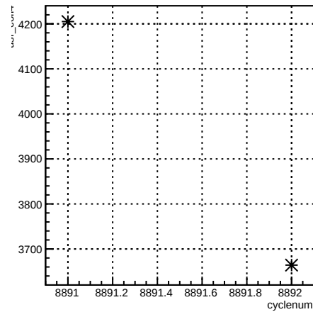
run:cyclenum {run == 7373}
