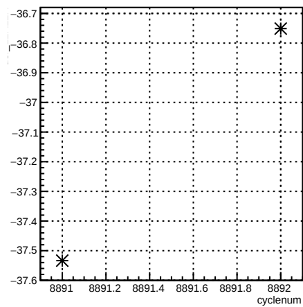
usr_11X12X:cyclenum {run == 7373}
