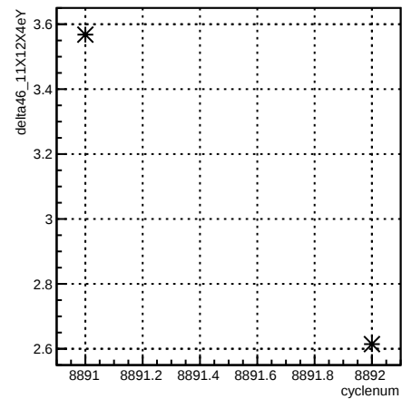
delta46_11X12X4eY:cyclenum {run == 7373}
