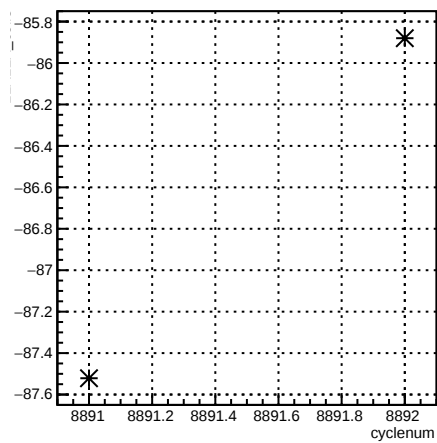
11X12X_coil3:cyclenum {run == 7373}
