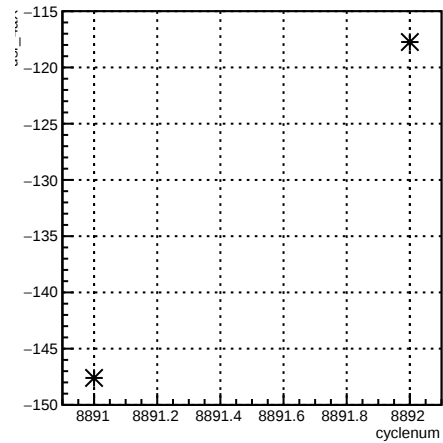
usr_4aX:cyclenum {run == 7373}
