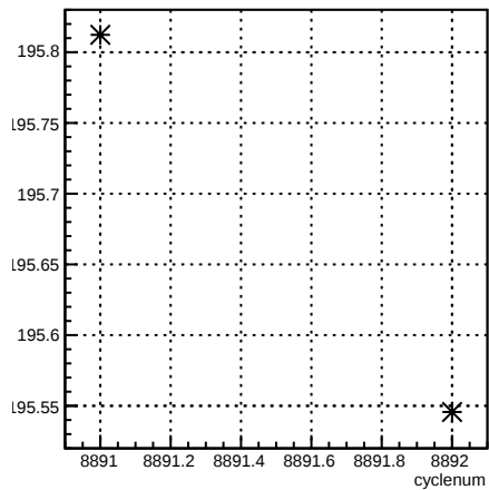
4eY_coil4:cyclenum {run == 7373}
