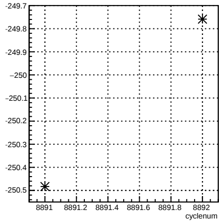
11X12X_coil1:cyclenum {run == 7373}
