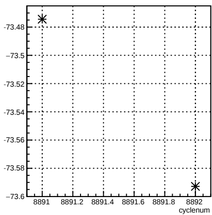
4aX_coil3:cyclenum {run == 7373}
