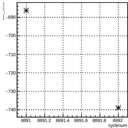
usr_coil6:cyclenum {run == 7373}
