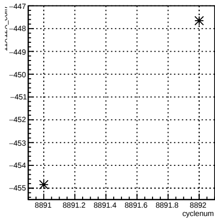
11X12X_coil7:cyclenum {run == 7373}
