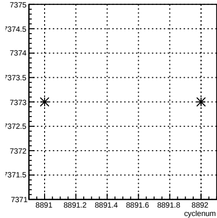
run:cyclenum {run == 7373}
