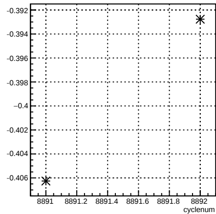
delta13_11X12X4eX:cyclenum {run == 7373}
