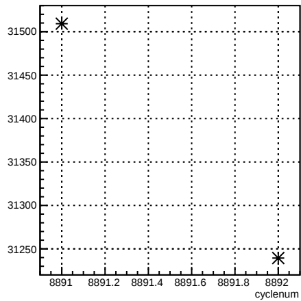
usl_coil6:cyclenum {run == 7373}
