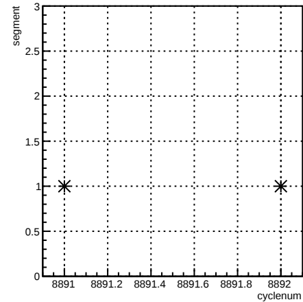
segment:cyclenum {run == 7373}
