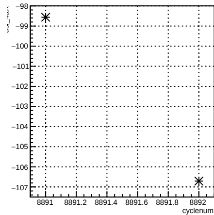
usl_4aX:cyclenum {run == 7373}
