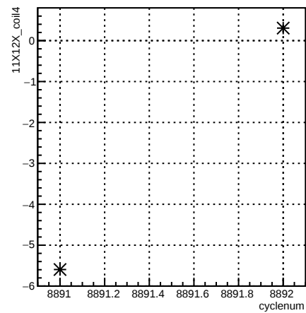
11X12X_coil4:cyclenum {run == 7373}
