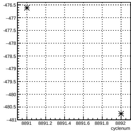
4eX_coil1:cyclenum {run == 7373}
