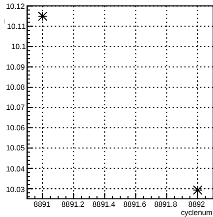
usl_4aY:cyclenum {run == 7373}
