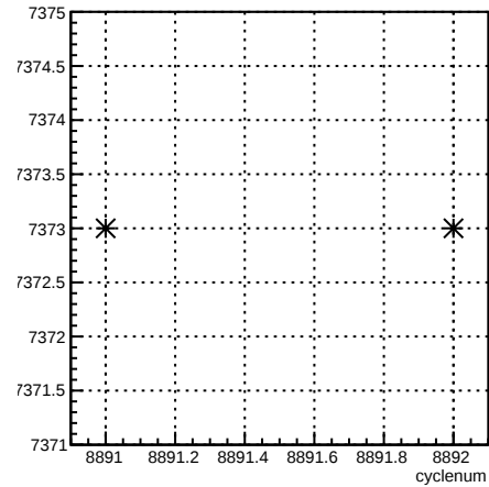
run:cyclenum {run == 7373}
