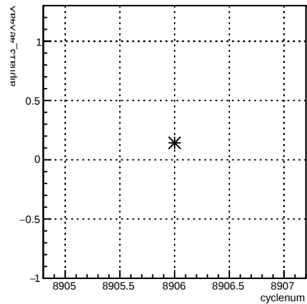
alpha13_4eX4aX:cyclenum {run == 7376}
