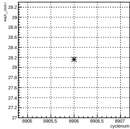
4eX_coil7:cyclenum {run == 7376}
