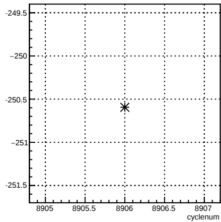
11X12X_coil6:cyclenum {run == 7376}
