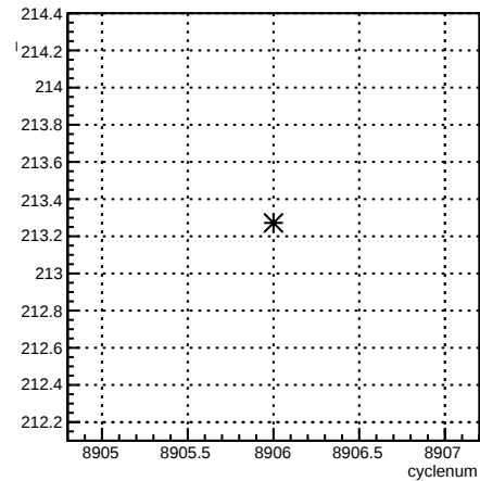
usr_4eX:cyclenum {run == 7376}
