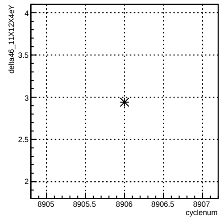
delta46_11X12X4eY:cyclenum {run == 7376}
