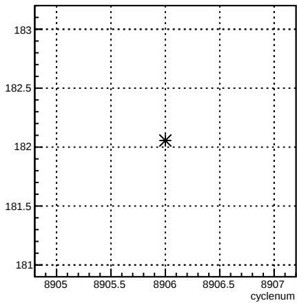
4eY_coil4:cyclenum {run == 7376}
