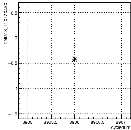
segment:cyclenum {run == 7376}
