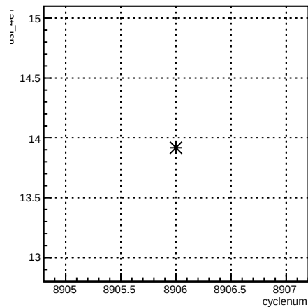
usl_4eY:cyclenum {run == 7376}
