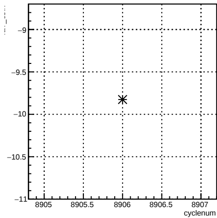
4eY_coil7:cyclenum {run == 7376}
