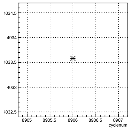
usr_coil4:cyclenum {run == 7376}
