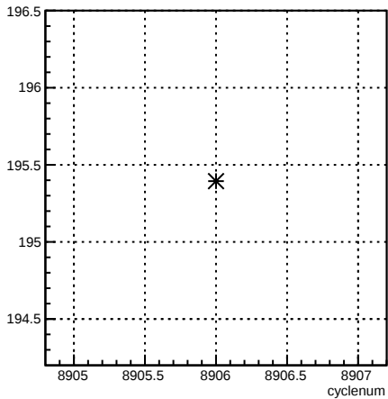
4eY_coil4:cyclenum {run == 7376}
