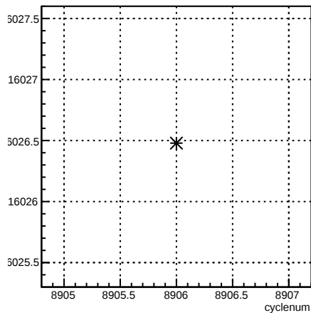
usl_coil7:cyclenum {run == 7376}
