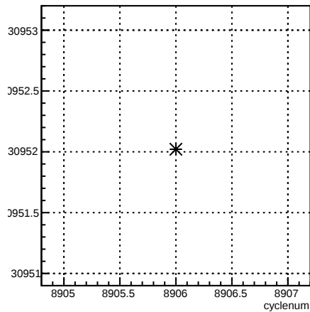
usl_coil6:cyclenum {run == 7376}
