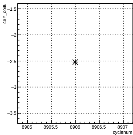
4eY_coil6:cyclenum {run == 7376}
