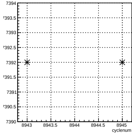
run:cyclenum {run == 7392}
