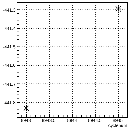
4eX_coil1:cyclenum {run == 7392}
