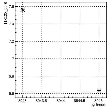
11X12X_coil6:cyclenum {run == 7392}
