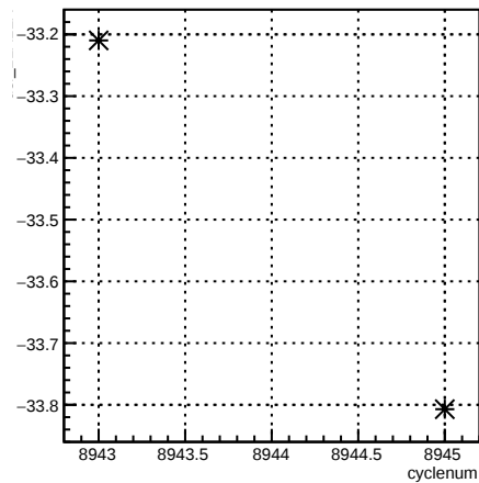
usl_11X12X:cyclenum {run == 7392}
