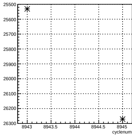
usr_coil1:cyclenum {run == 7392}
