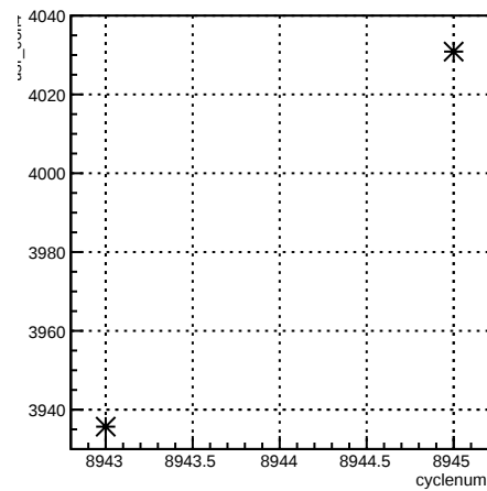
usr_coil4:cyclenum {run == 7392}
