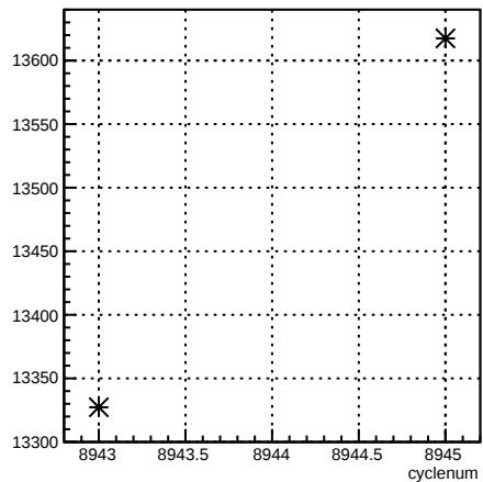
usl_coil7:cyclenum {run == 7392}
