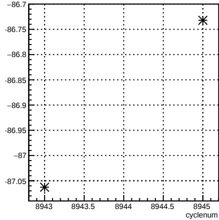
11X12X_coil3:cyclenum {run == 7392}
