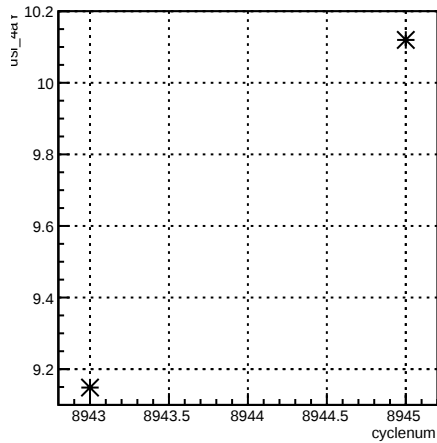
usl_4aY:cyclenum {run == 7392}
