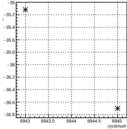
usr_11X12X:cyclenum {run == 7392}
