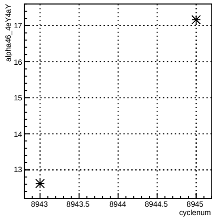
run:cyclenum {run == 7392}
