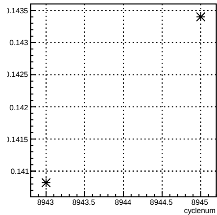
alpha13_4eX4aX:cyclenum {run == 7392}
