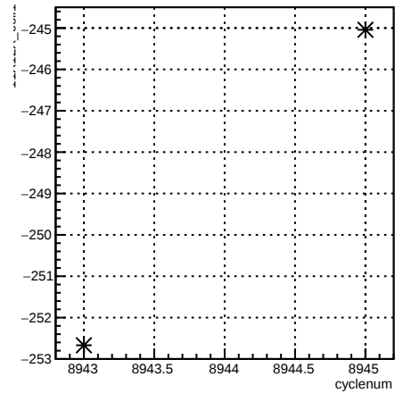
11X12X_coil1:cyclenum {run == 7392}
