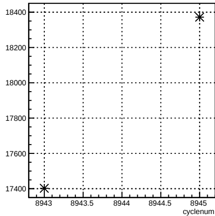
usr_coil7:cyclenum {run == 7392}
