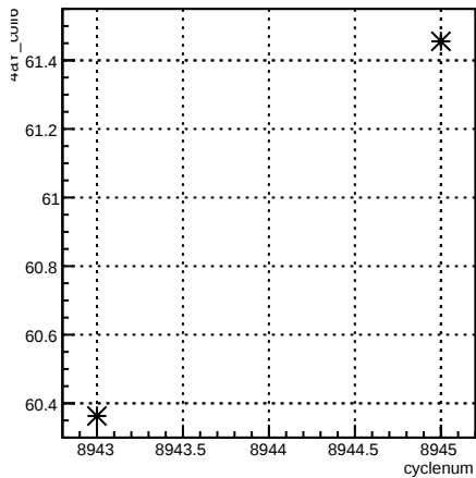
4eY_coil6:cyclenum {run == 7392}
