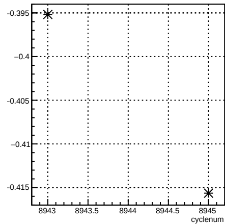
segment:cyclenum {run == 7392}
