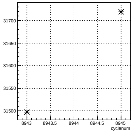
usl_coil6:cyclenum {run == 7392}
