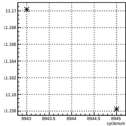
usl_4eY:cyclenum {run == 7392}
