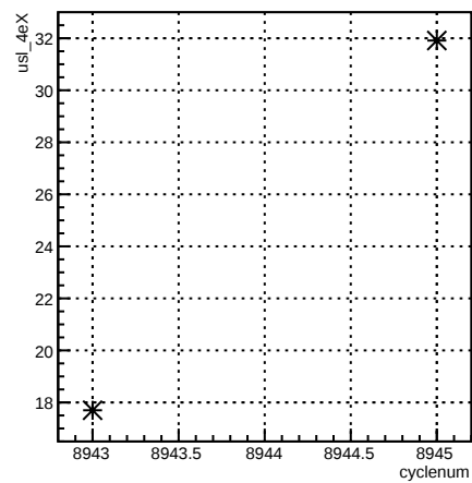
usl_4eX:cyclenum {run == 7392}
