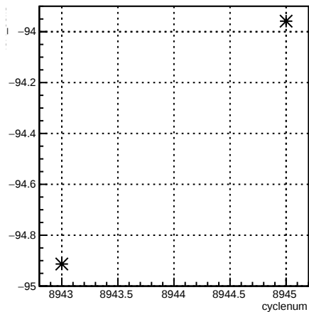
4eX_coil3:cyclenum {run == 7392}
