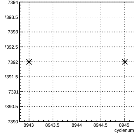
run:cyclenum {run == 7392}
