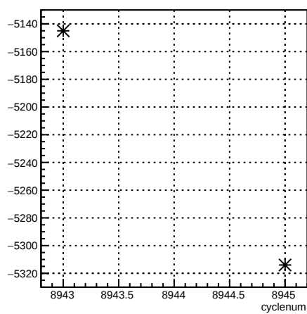
usr_coil3:cyclenum {run == 7392}
