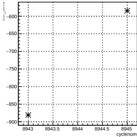
usr_coil6:cyclenum {run == 7392}
