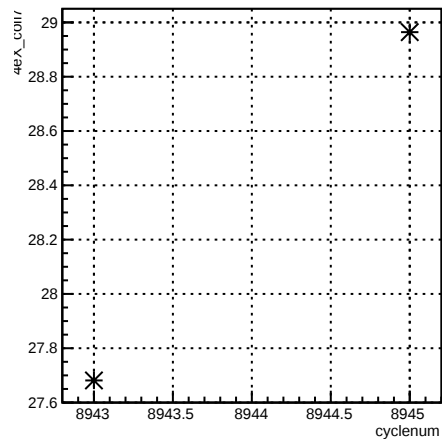
4eX_coil7:cyclenum {run == 7392}
