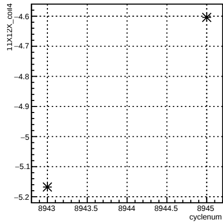
11X12X_coil4:cyclenum {run == 7392}
