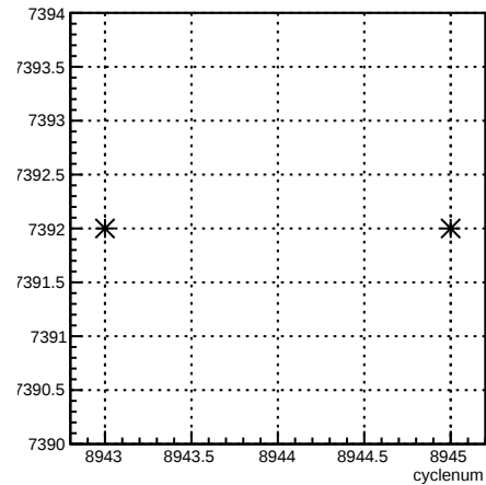
run:cyclenum {run == 7392}
