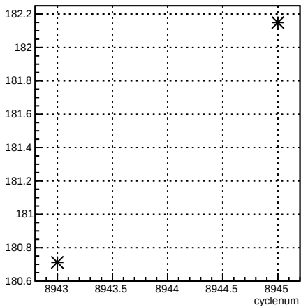
4eY_coil4:cyclenum {run == 7392}
