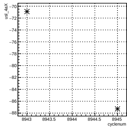
usl_4aX:cyclenum {run == 7392}
