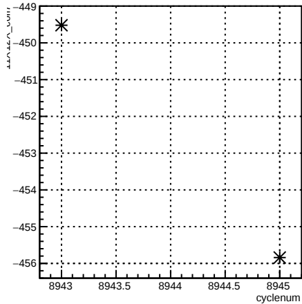
11X12X_coil7:cyclenum {run == 7392}
