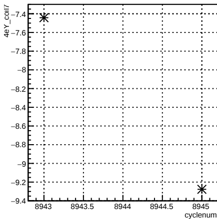
4eY_coil7:cyclenum {run == 7392}
