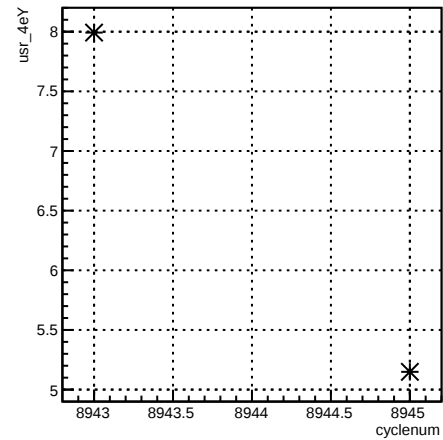
usr_4eY:cyclenum {run == 7392}
