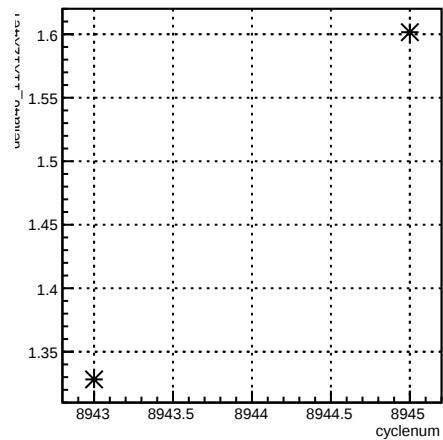
delta46_11X12X4eY:cyclenum {run == 7392}
