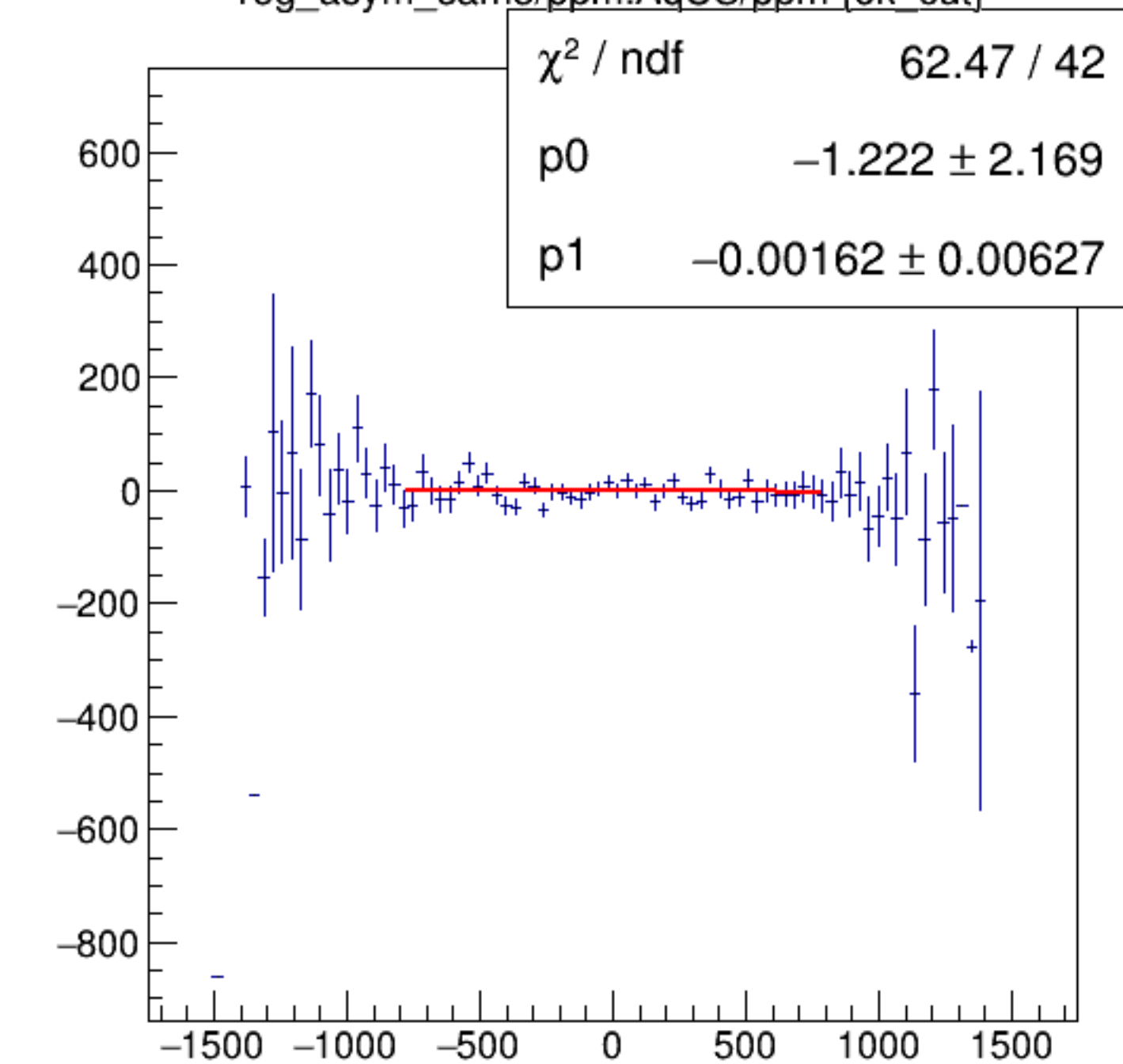
reg_asym_sam3/ppm:AqUS/ppm {ok_cut}
