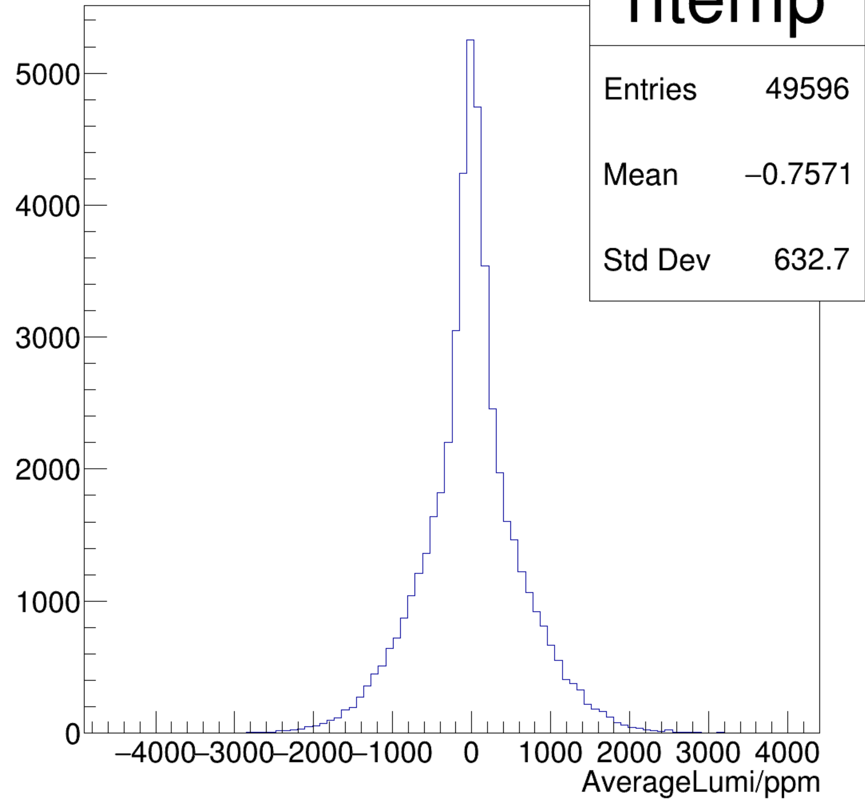
AverageLumi/ppm {ok_cut}
