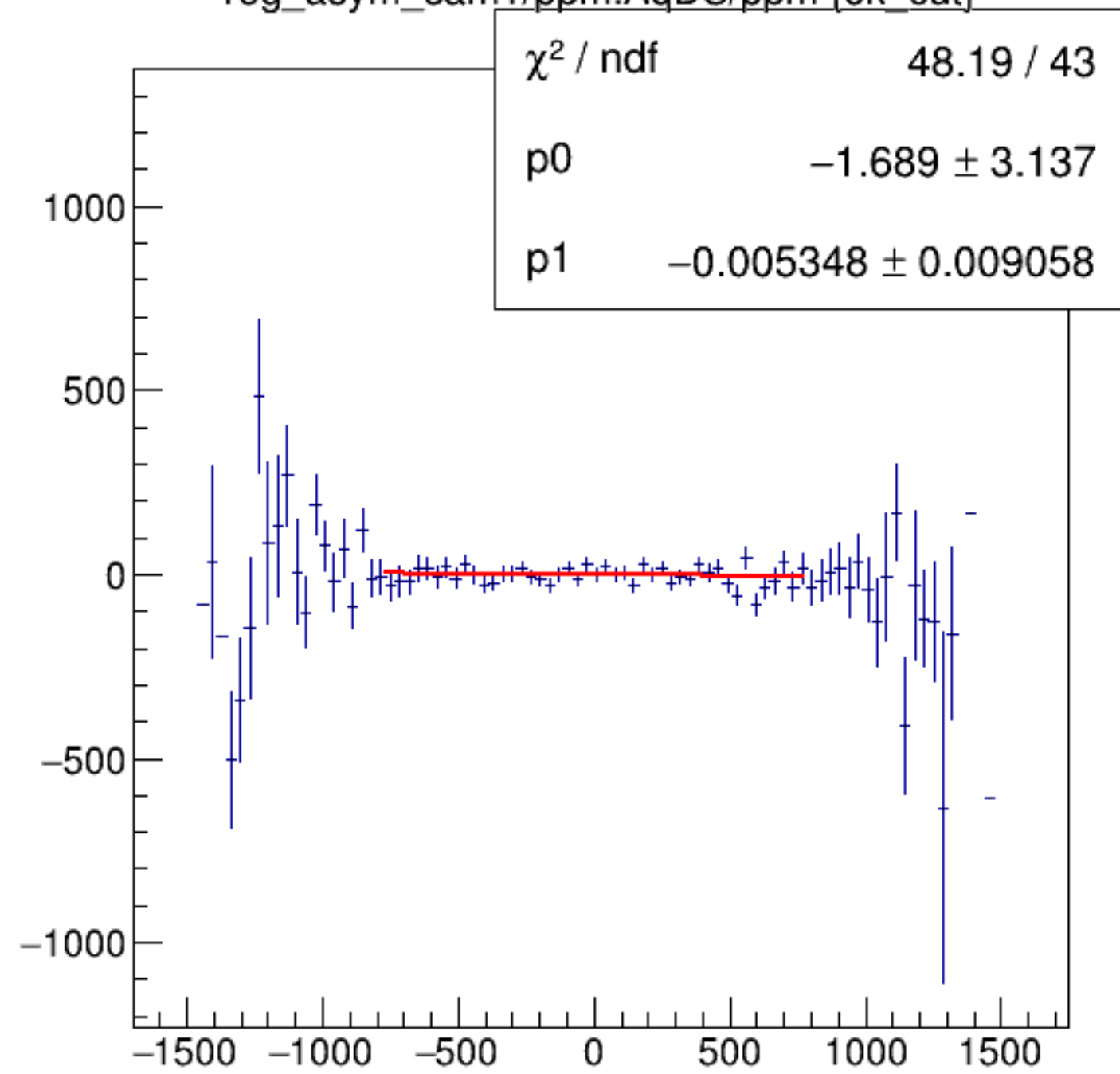
reg_asym_sam1/ppm:AqDS/ppm {ok_cut}
