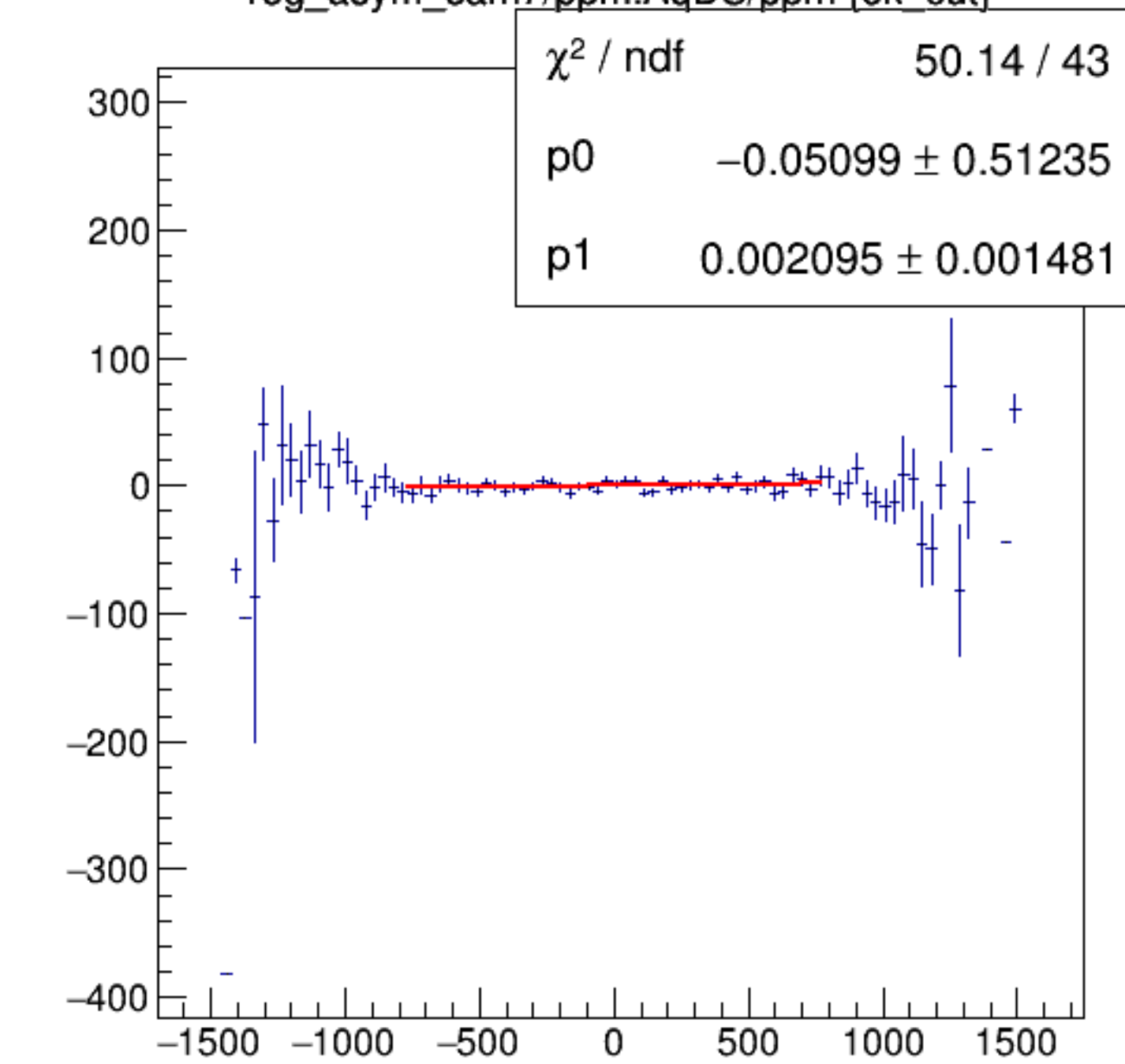
reg_asym_sam7/ppm:AqDS/ppm {ok_cut}
