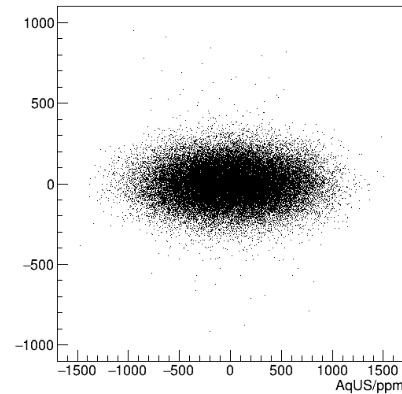
reg_asym_sam7/ppm:AqUS/ppm {ok_cut}
