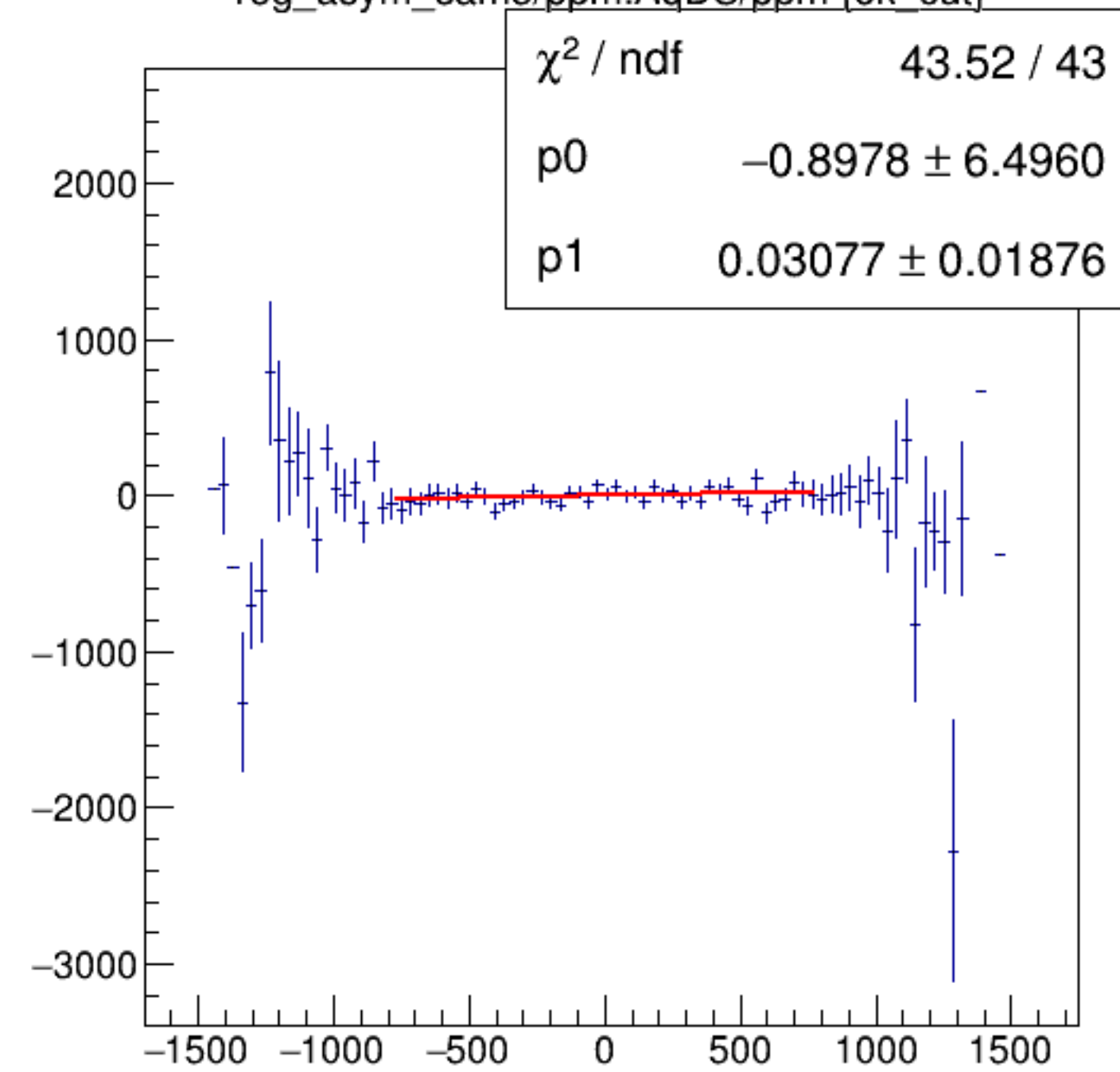
reg_asym_sam5/ppm:AqDS/ppm {ok_cut}
