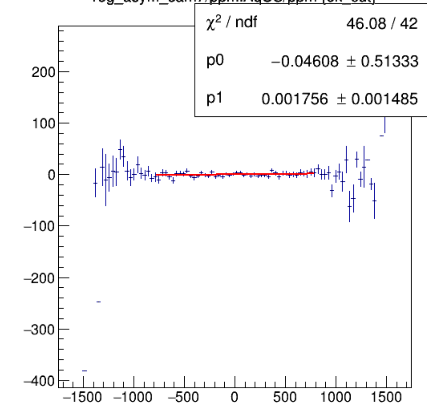
reg_asym_sam7/ppm:AqUS/ppm {ok_cut}
