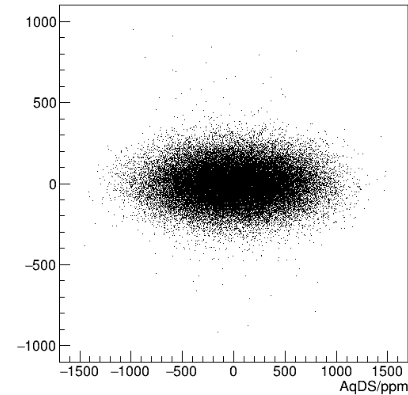
reg_asym_sam7/ppm:AqDS/ppm {ok_cut}
