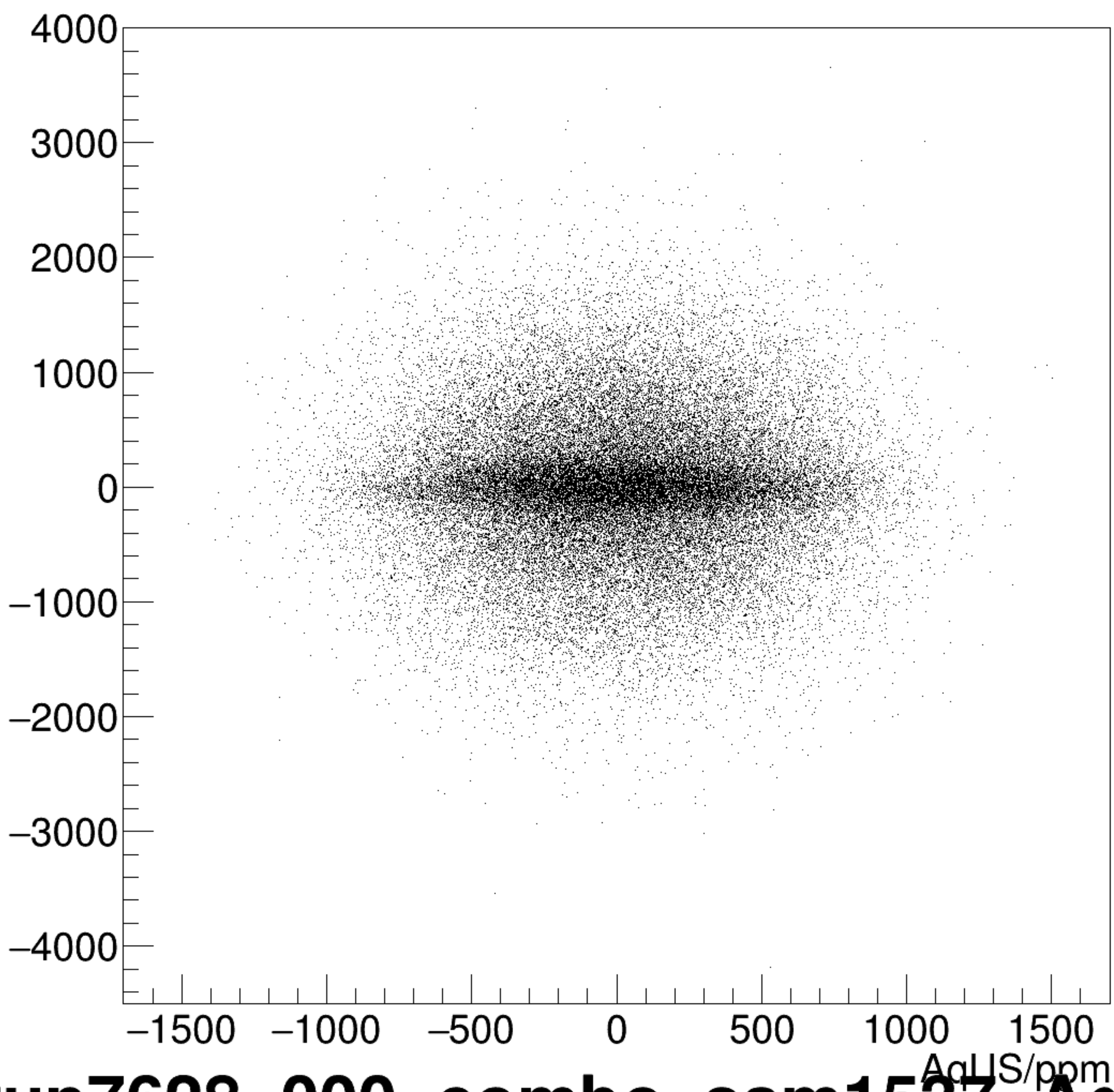
AverageLumi/ppm:AqUS/ppm {ok_cut}
