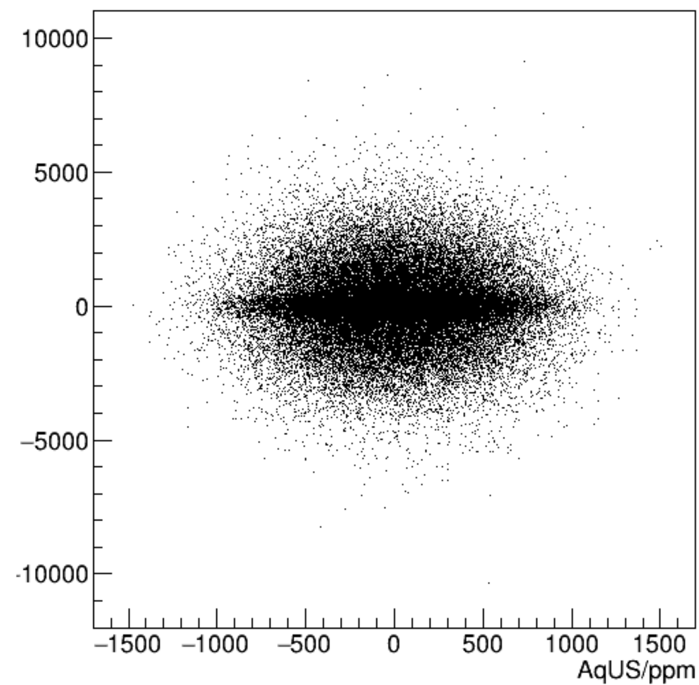
reg_asym_sam5/ppm:AqUS/ppm {ok_cut}
