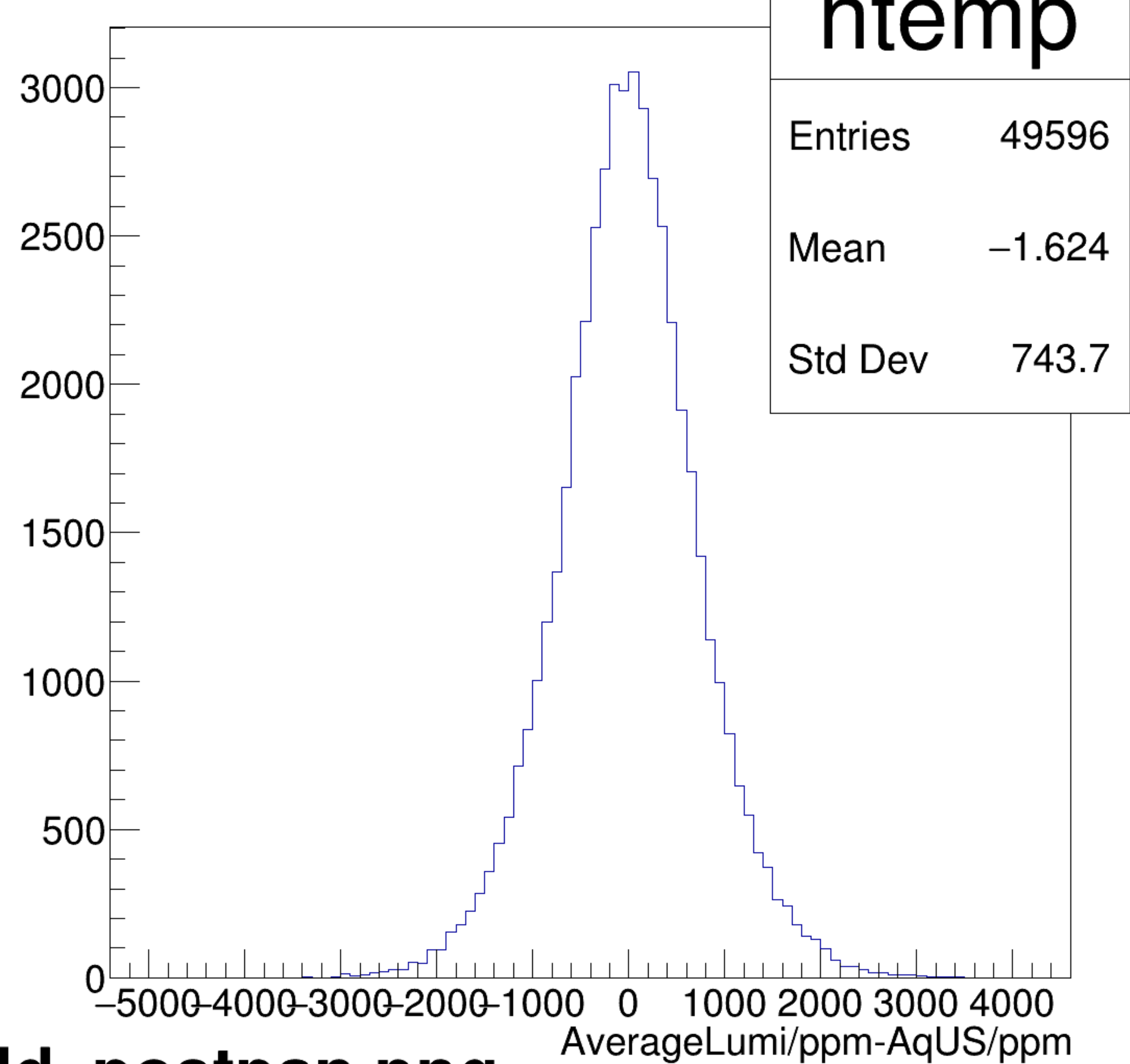
AverageLumi/ppm-AqUS/ppm {ok_cut}
