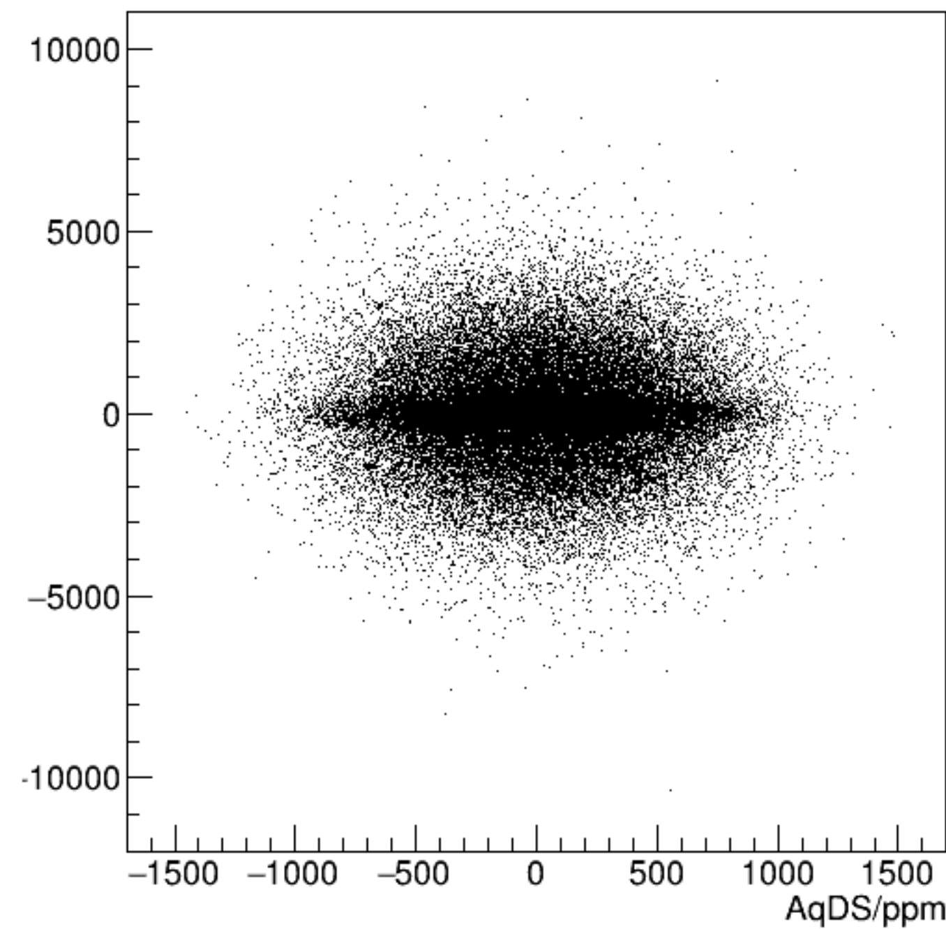
reg_asym_sam5/ppm:AqDS/ppm {ok_cut}
