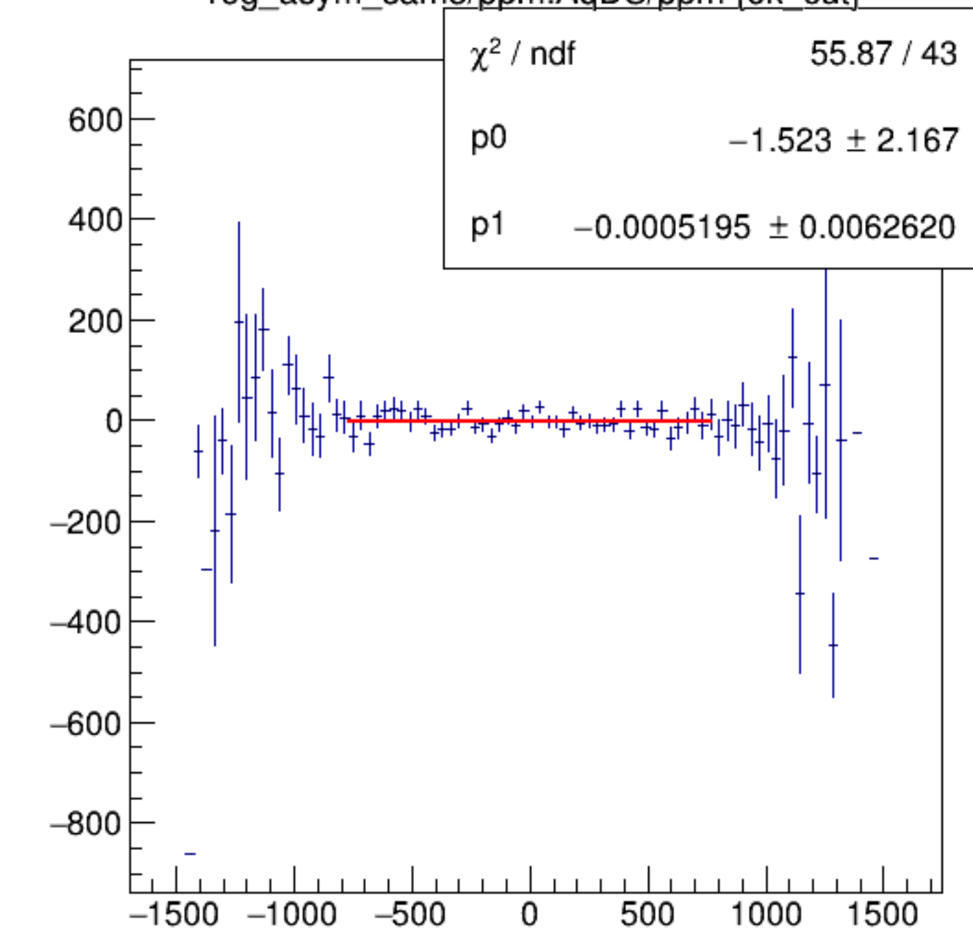
reg_asym_sam3/ppm:AqDS/ppm {ok_cut}
