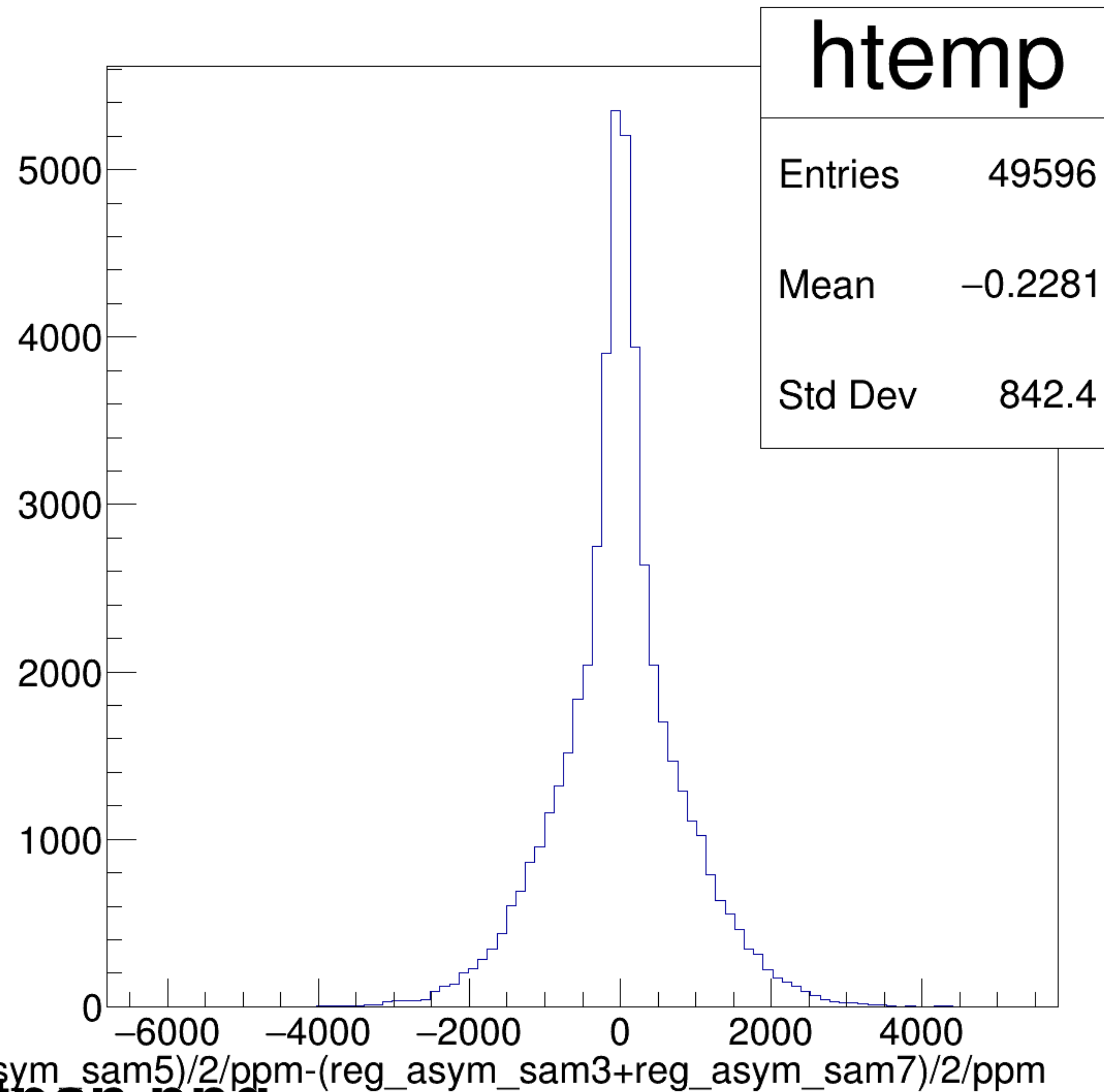
(reg_asym_sam1+reg_asym_sam5)/2/ppm-(reg_asym_sam3+reg_asym_sam7)/2/ppm {ok_cut}
