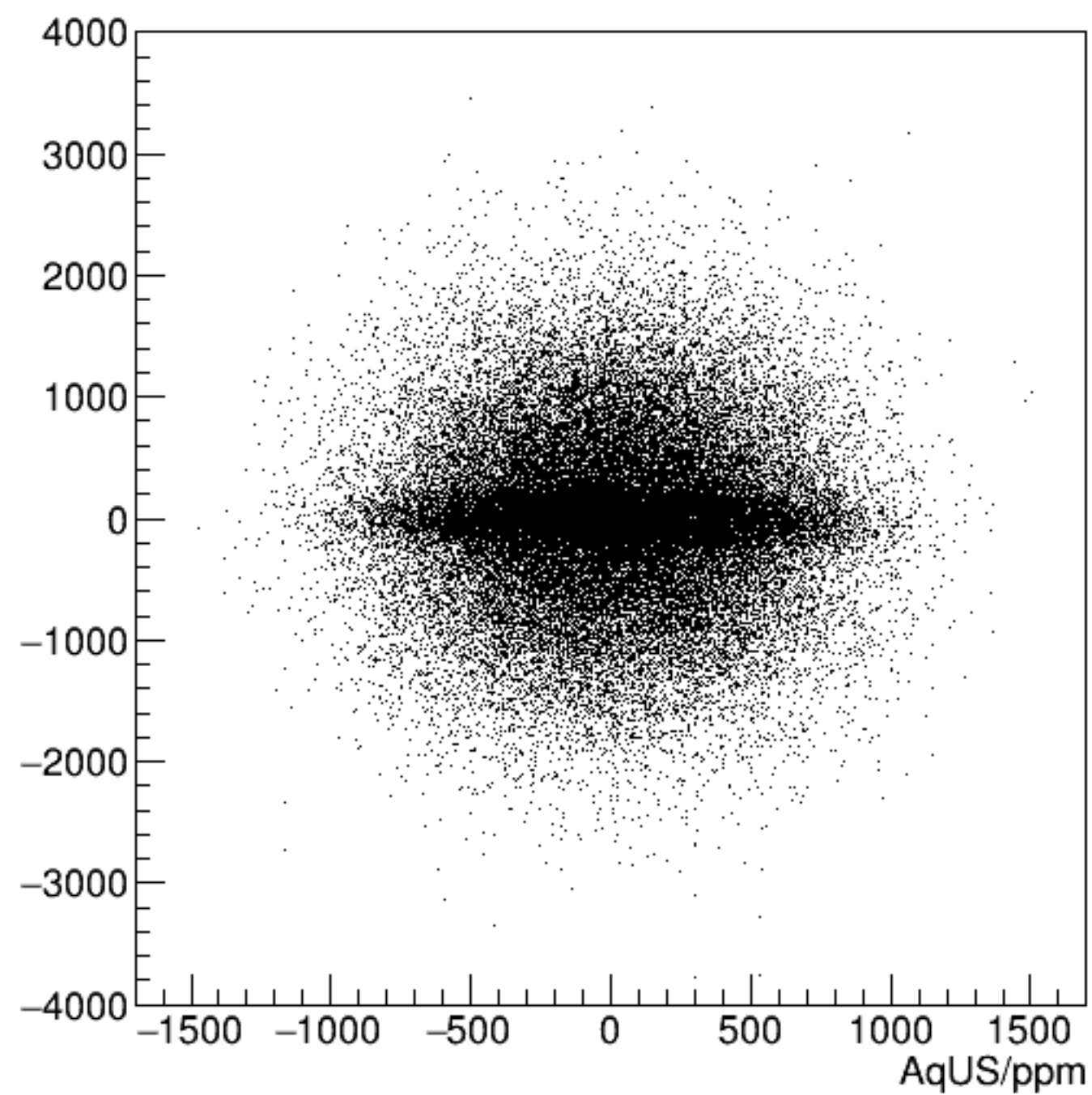
reg_asym_sam1/ppm:AqUS/ppm {ok_cut}
