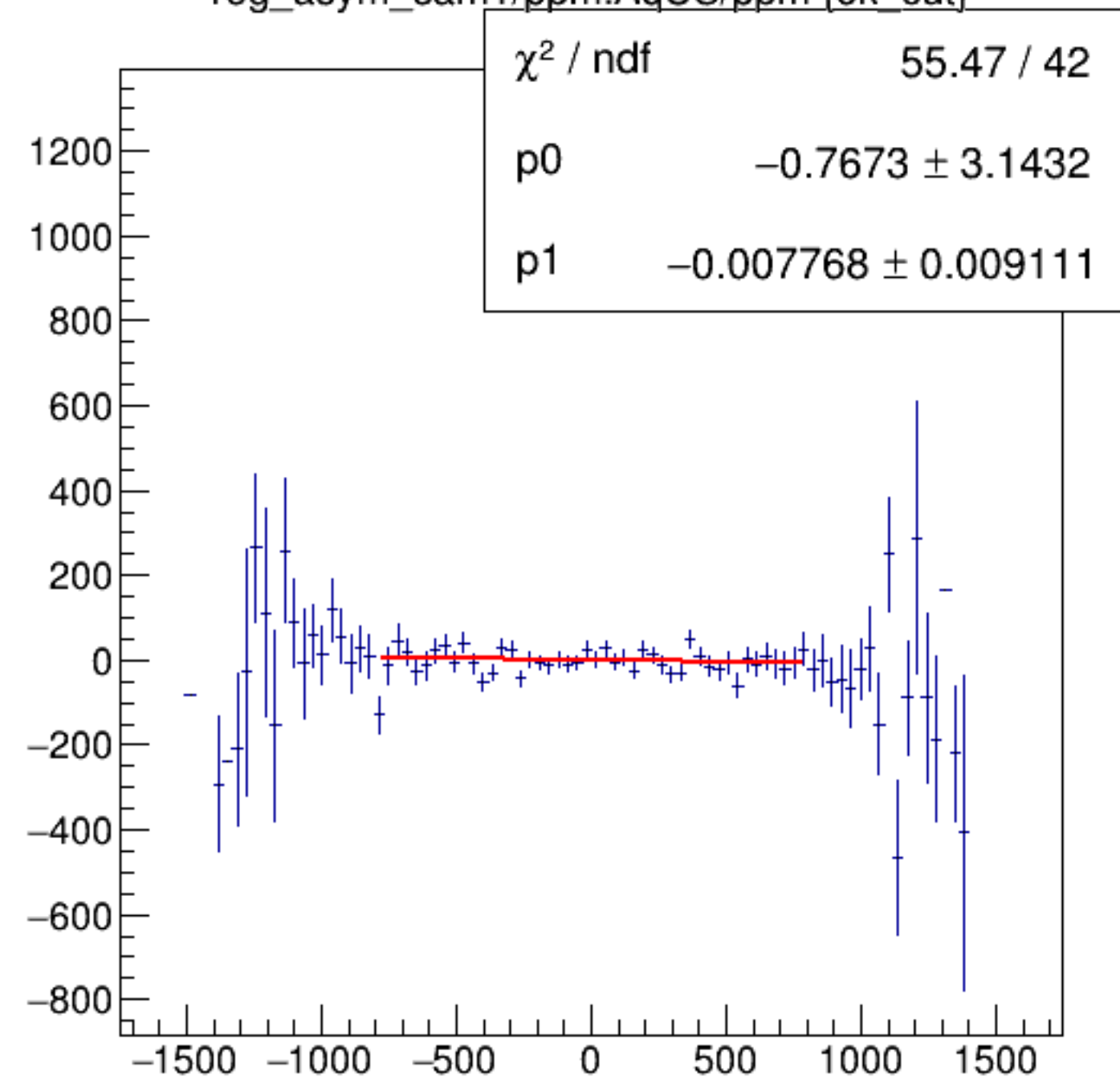
reg_asym_sam1/ppm:AqUS/ppm {ok_cut}
