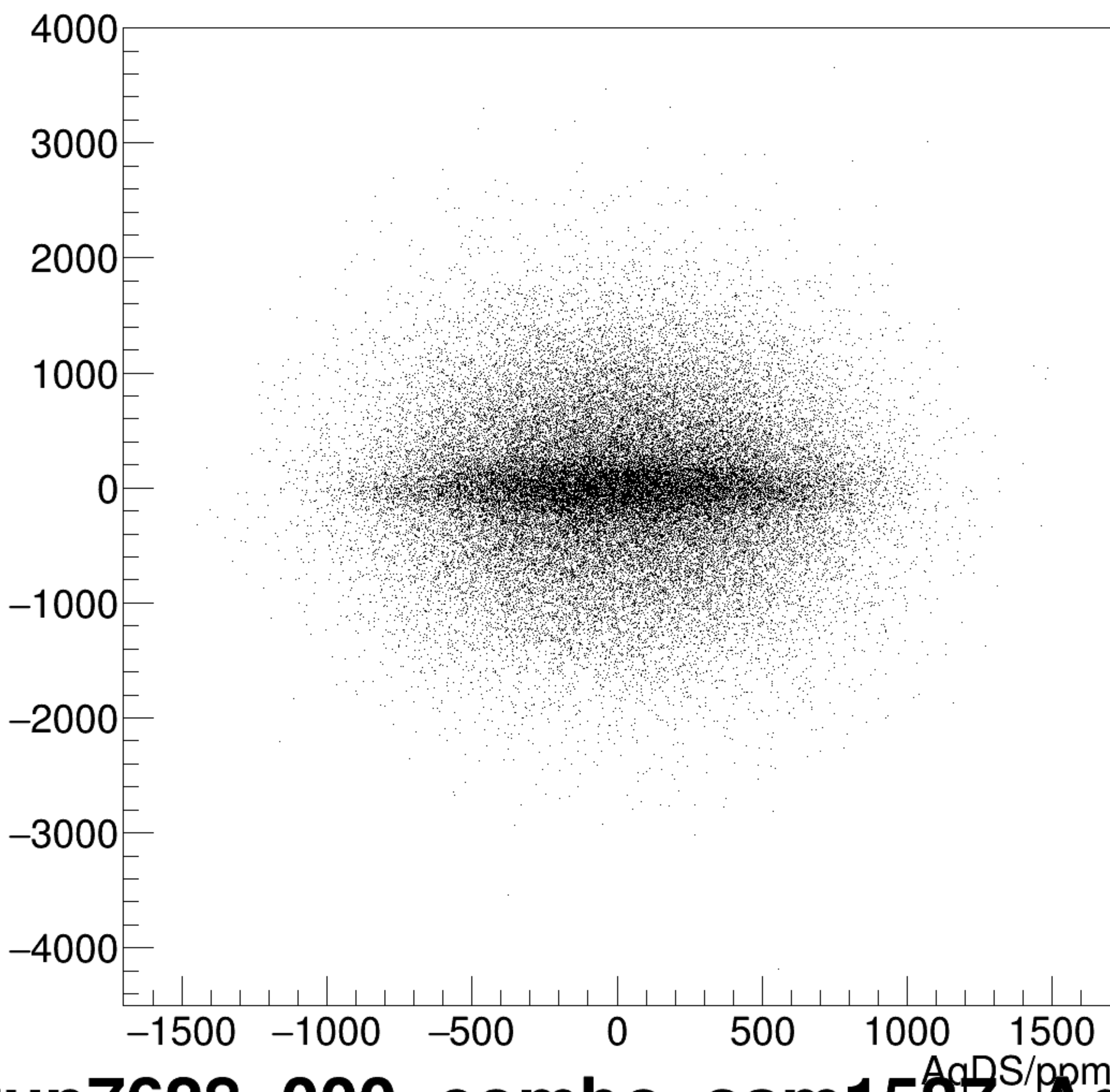
AverageLumi/ppm:AqDS/ppm {ok_cut}
