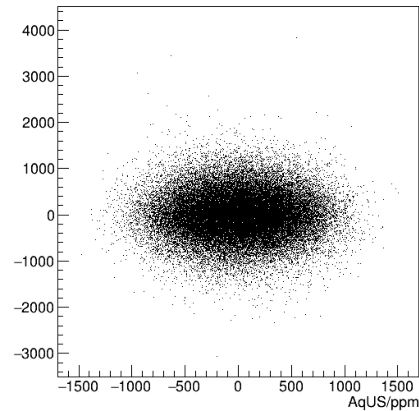
reg_asym_sam3/ppm:AqUS/ppm {ok_cut}
