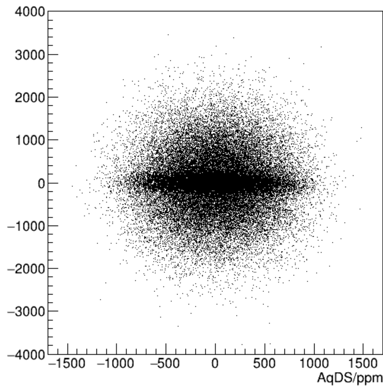
reg_asym_sam1/ppm:AqDS/ppm {ok_cut}
