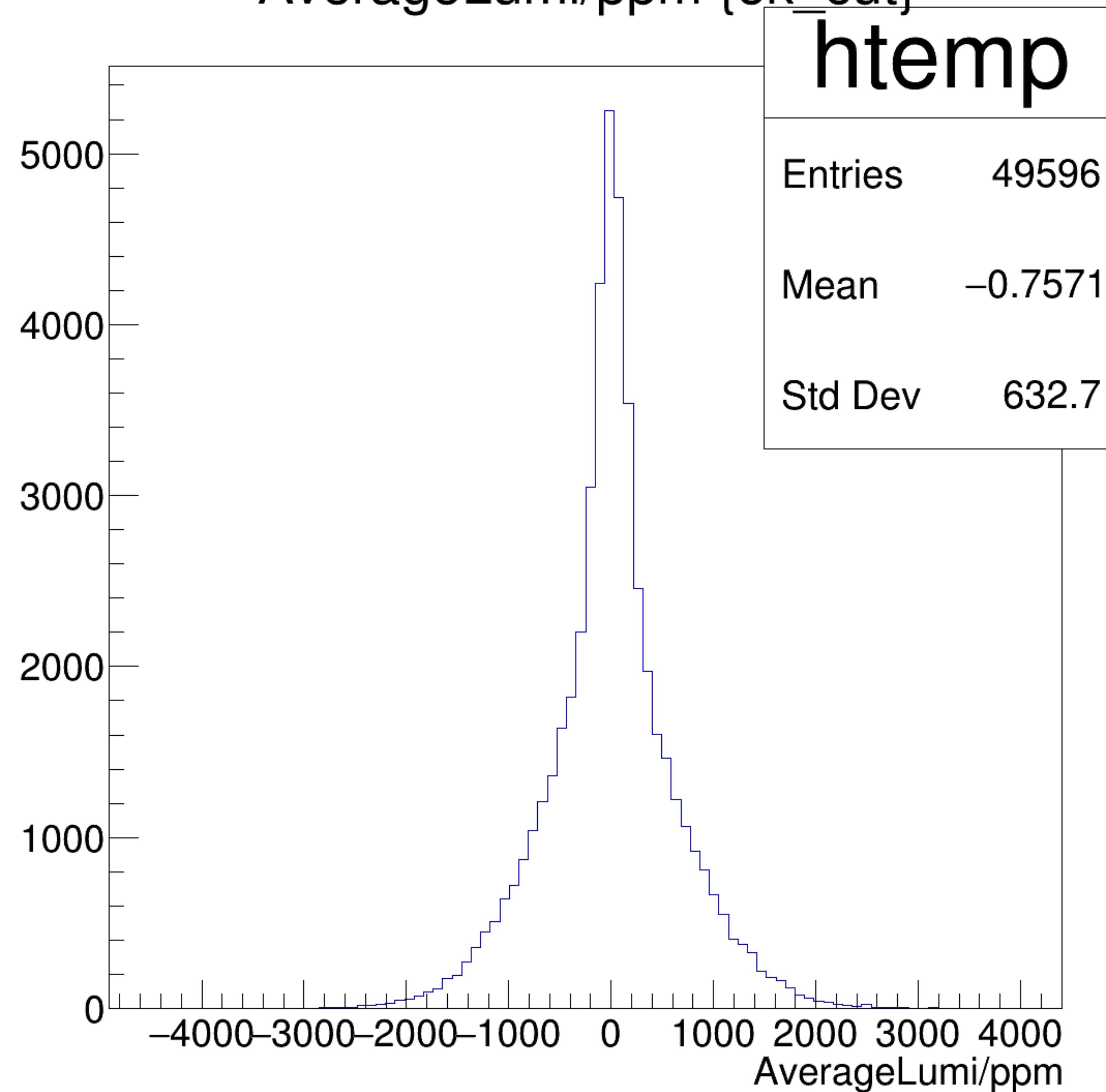
AverageLumi/ppm {ok_cut}
