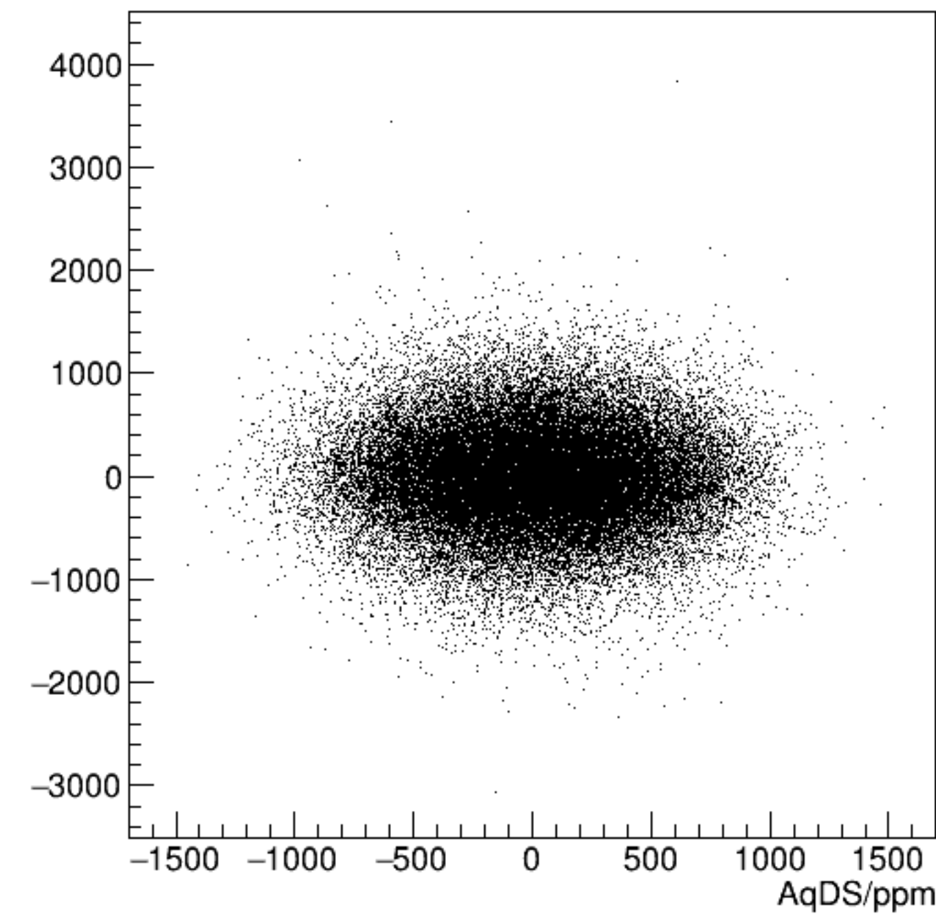
reg_asym_sam3/ppm:AqDS/ppm {ok_cut}
