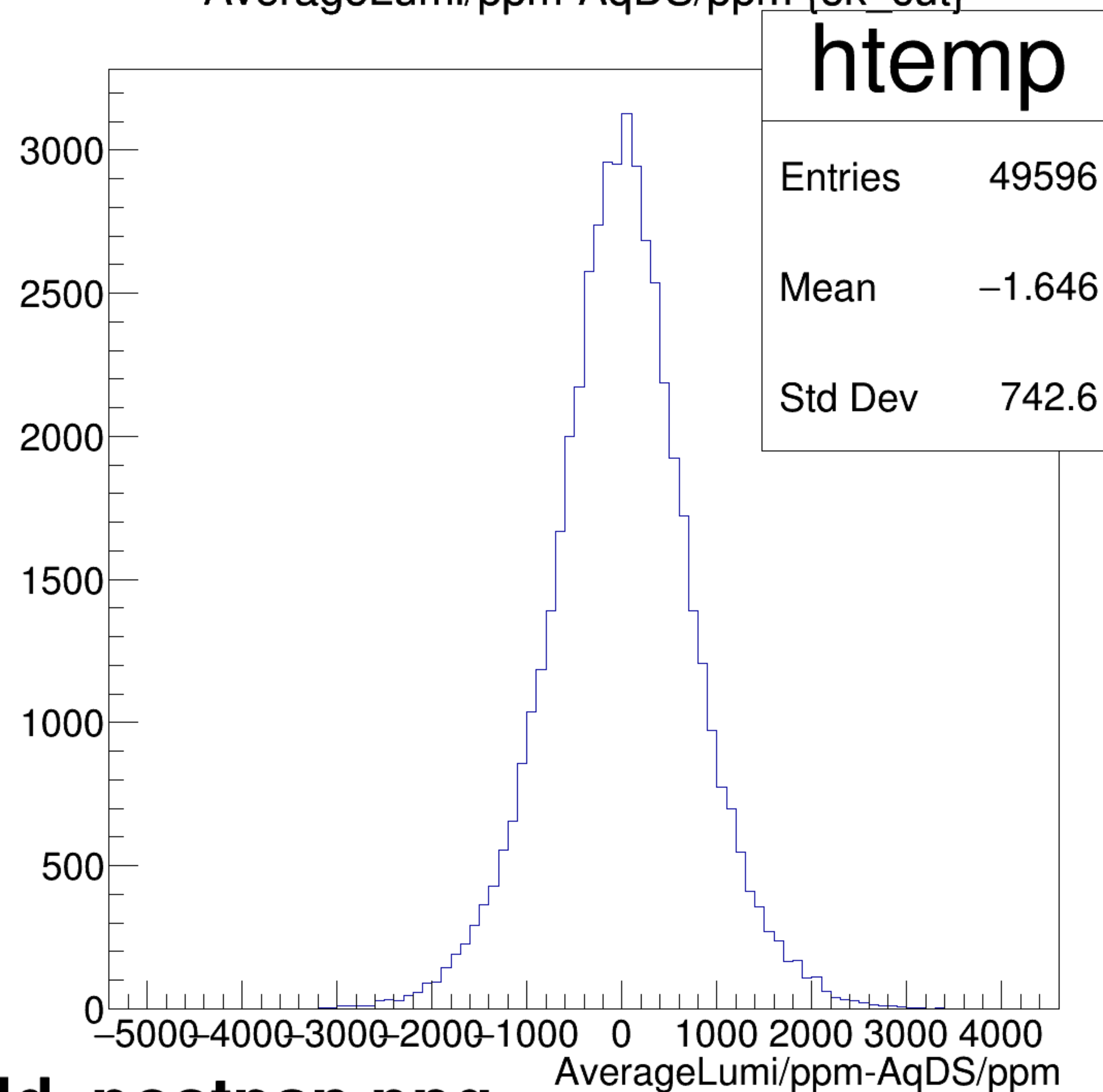
AverageLumi/ppm-AqDS/ppm {ok_cut}
