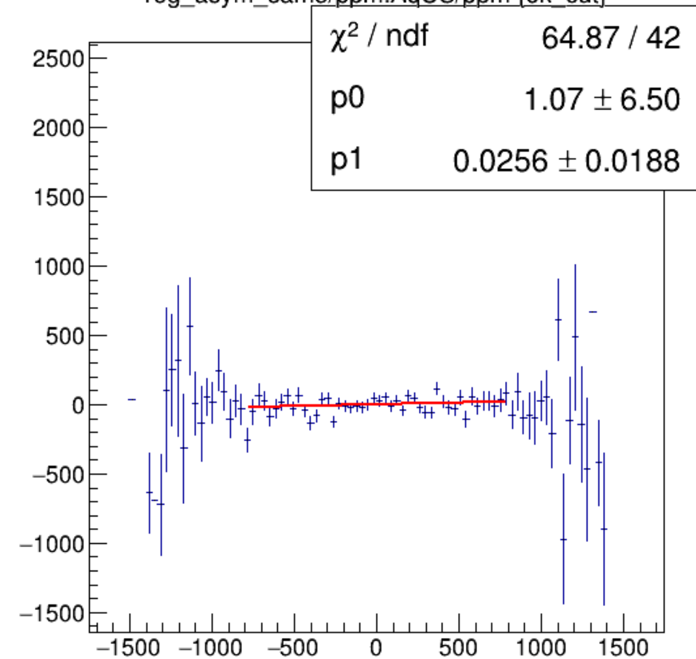
reg_asym_sam5/ppm:AqUS/ppm {ok_cut}
