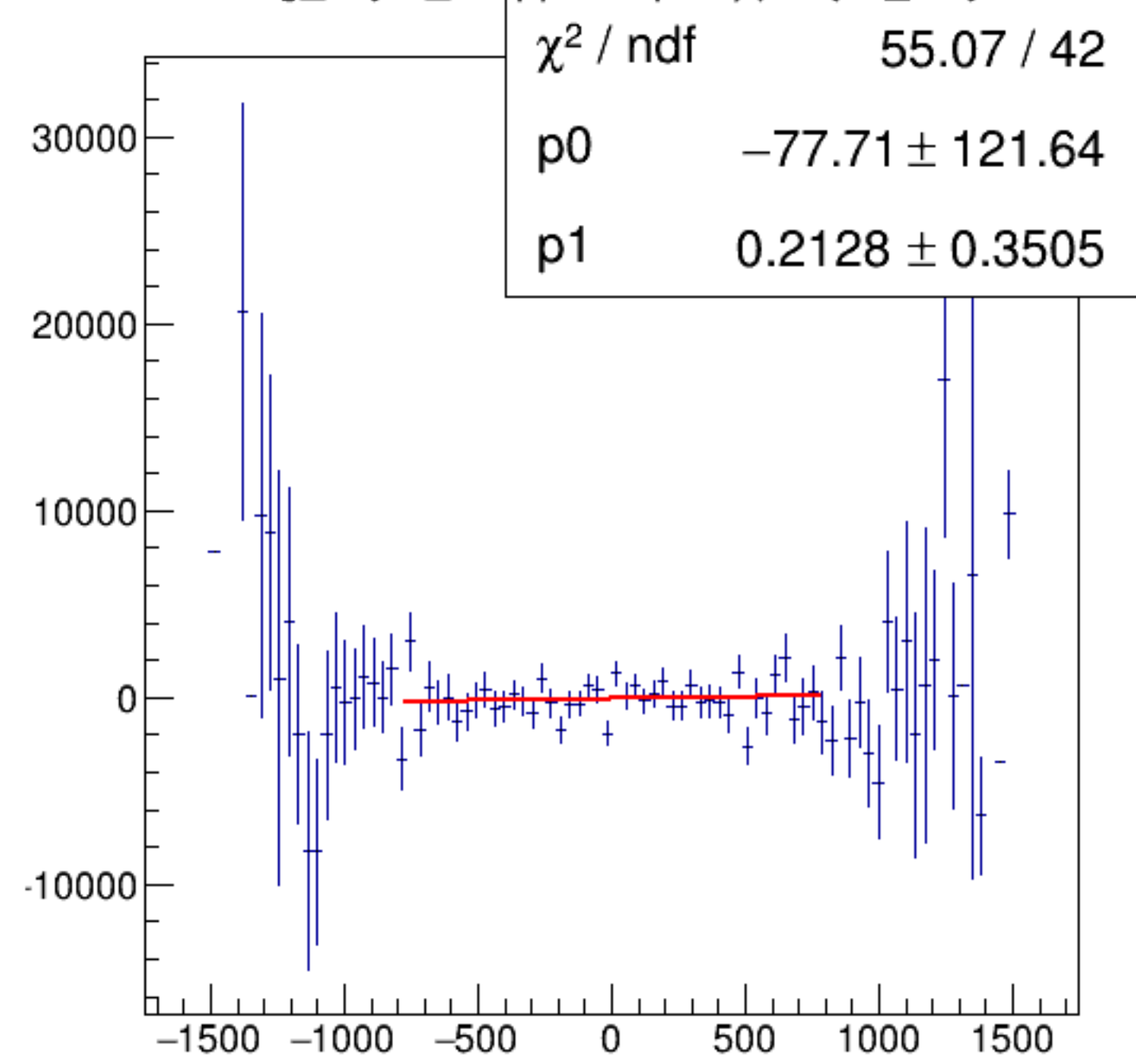
reg_asym_dsl/ppm:AqUS/ppm {ok_cut}
