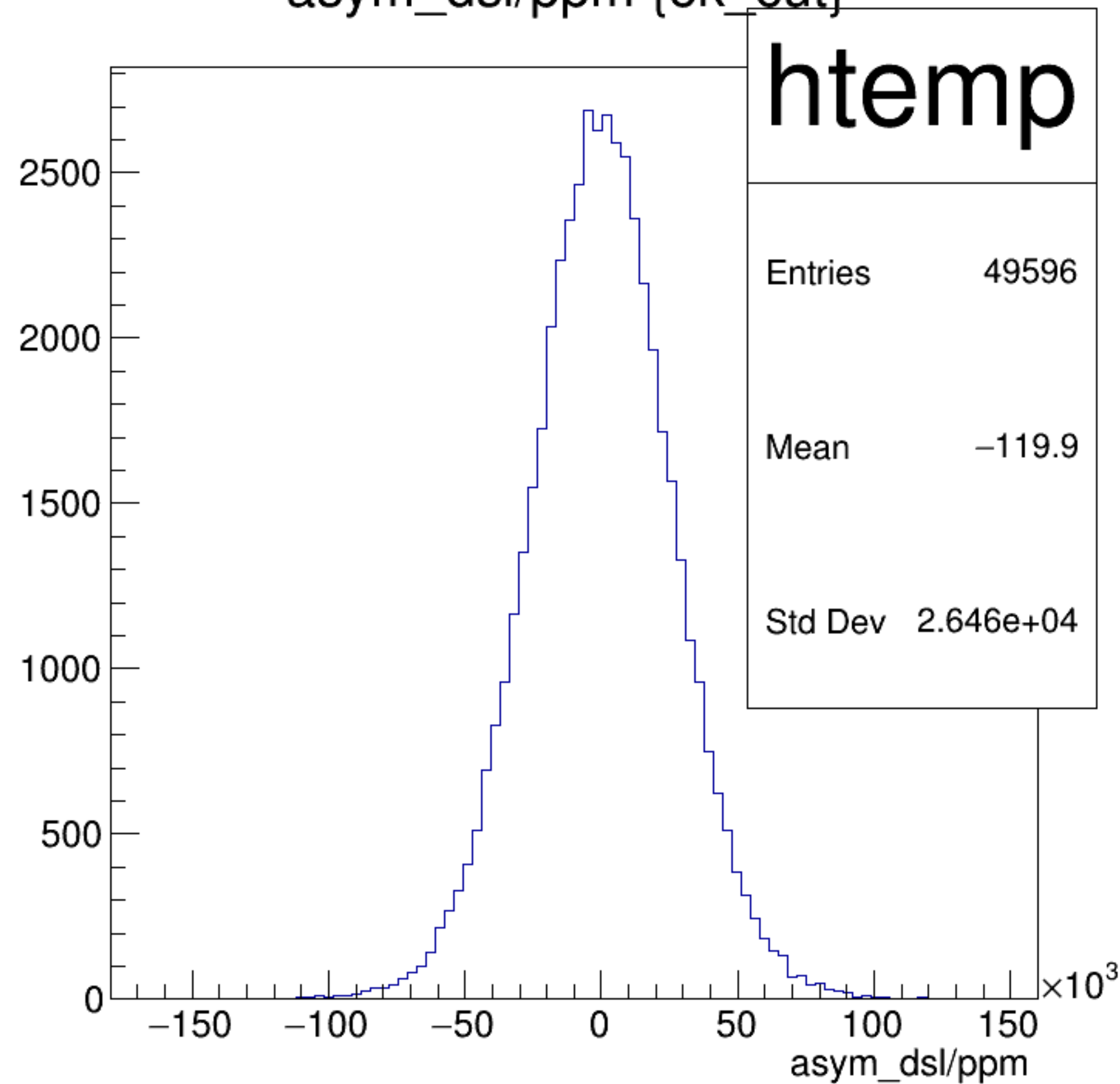
asym_dsl/ppm {ok_cut}
