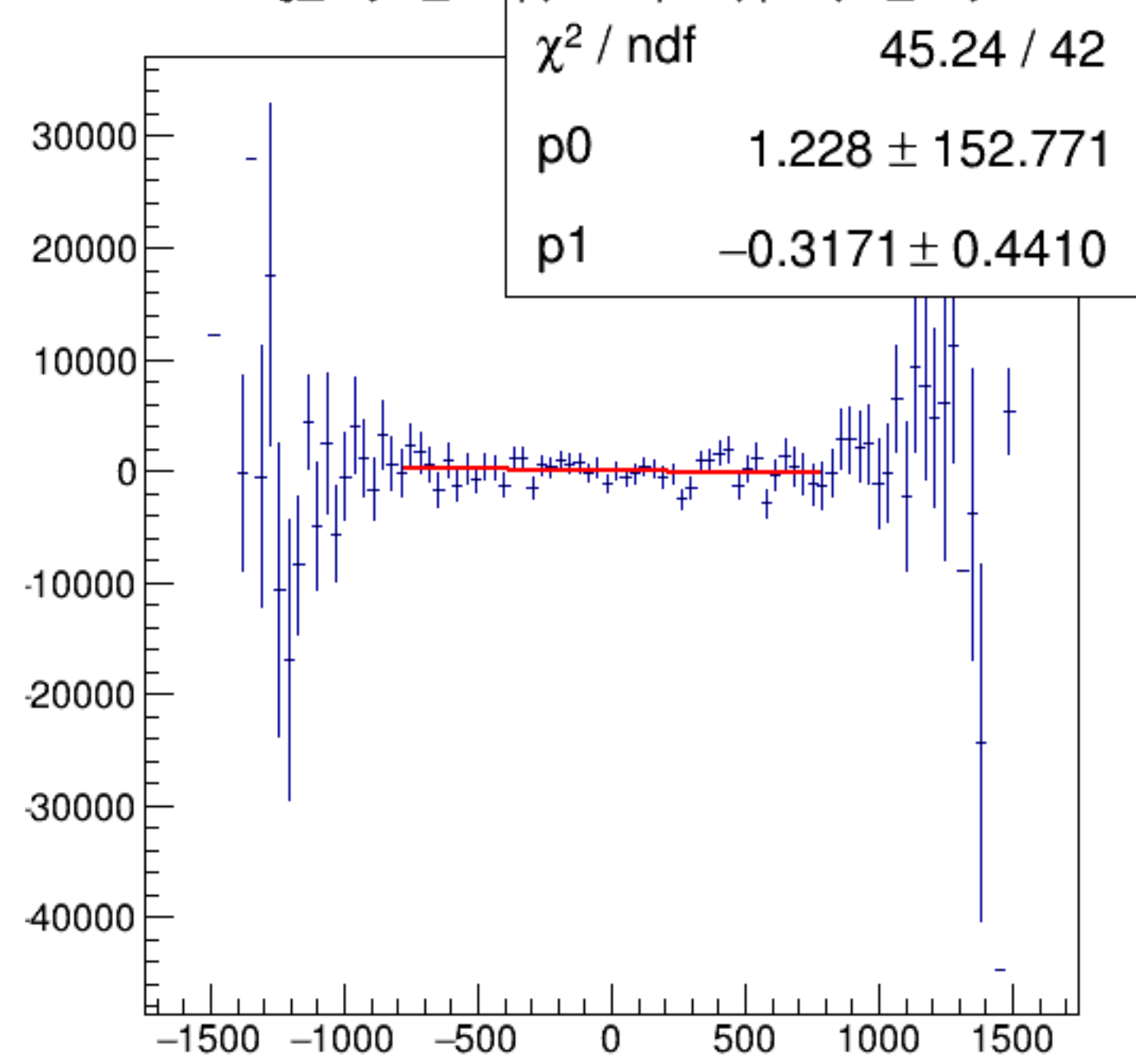
reg_asym_dsr/ppm:AqUS/ppm {ok_cut}
