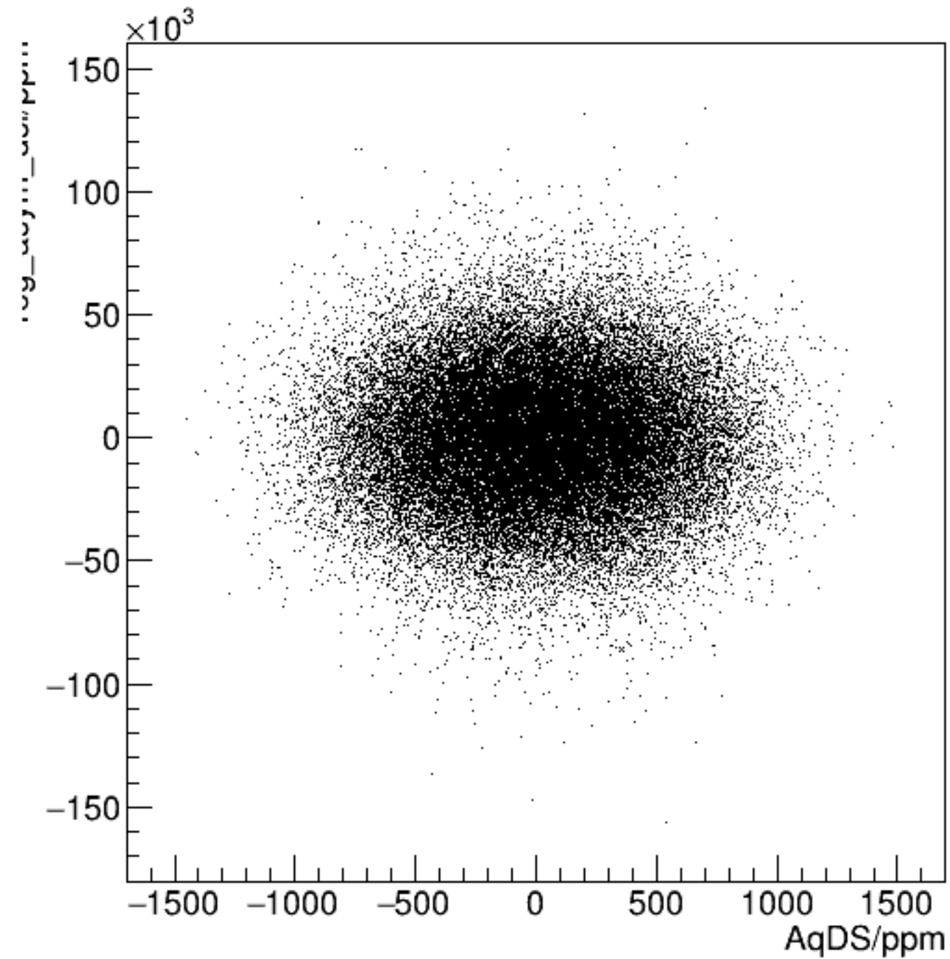
reg_asym_dsl/ppm:AqDS/ppm {ok_cut}
