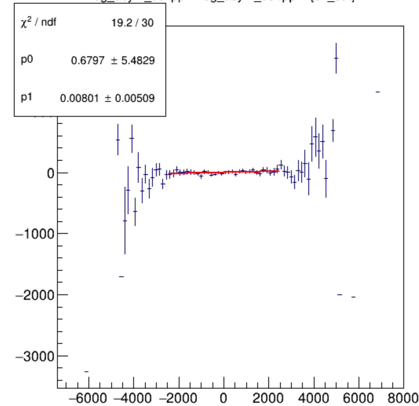
reg_asym_usl/ppm:reg_asym_usr/ppm {ok_cut}
