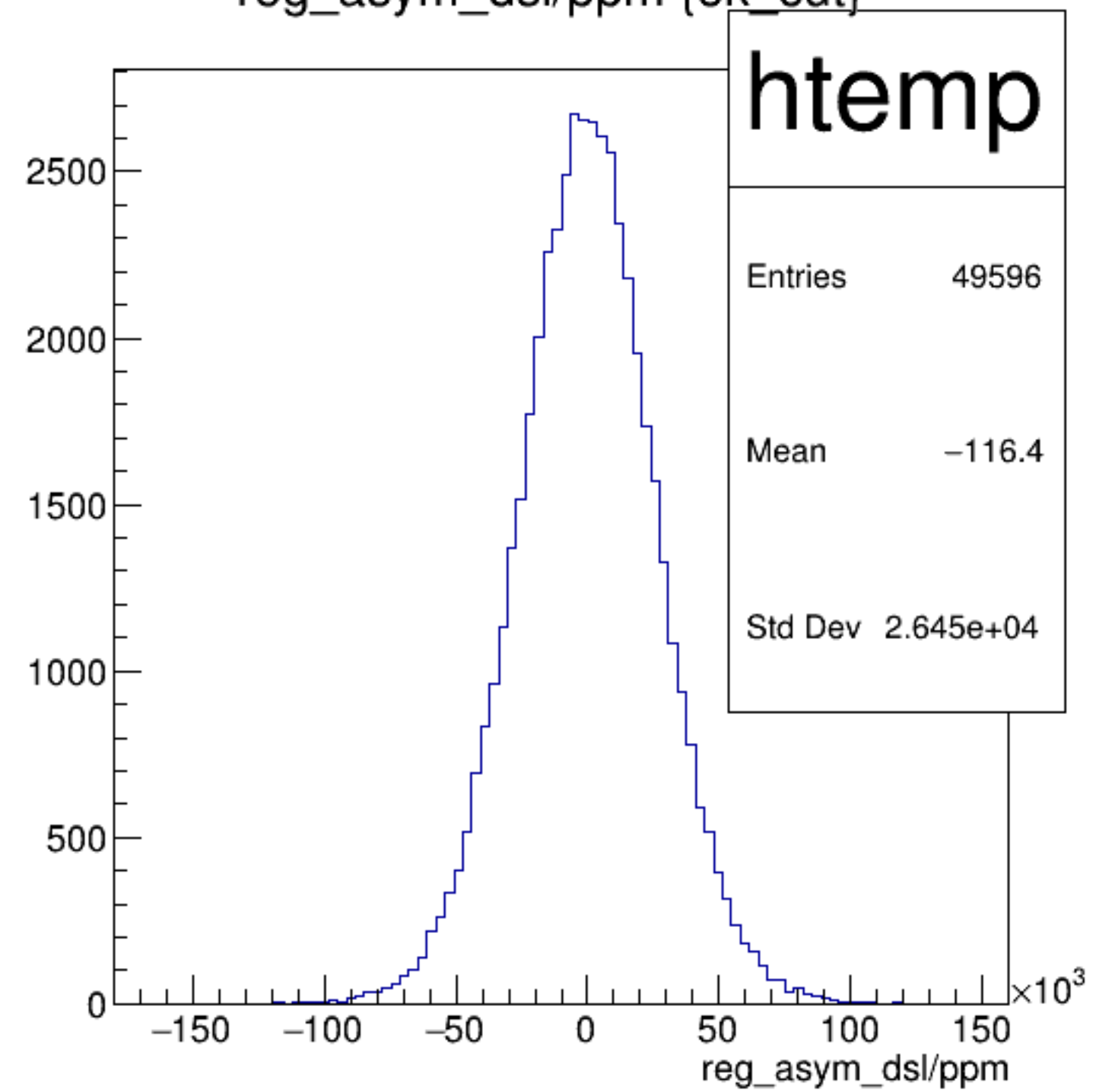
reg_asym_dsl/ppm {ok_cut}
