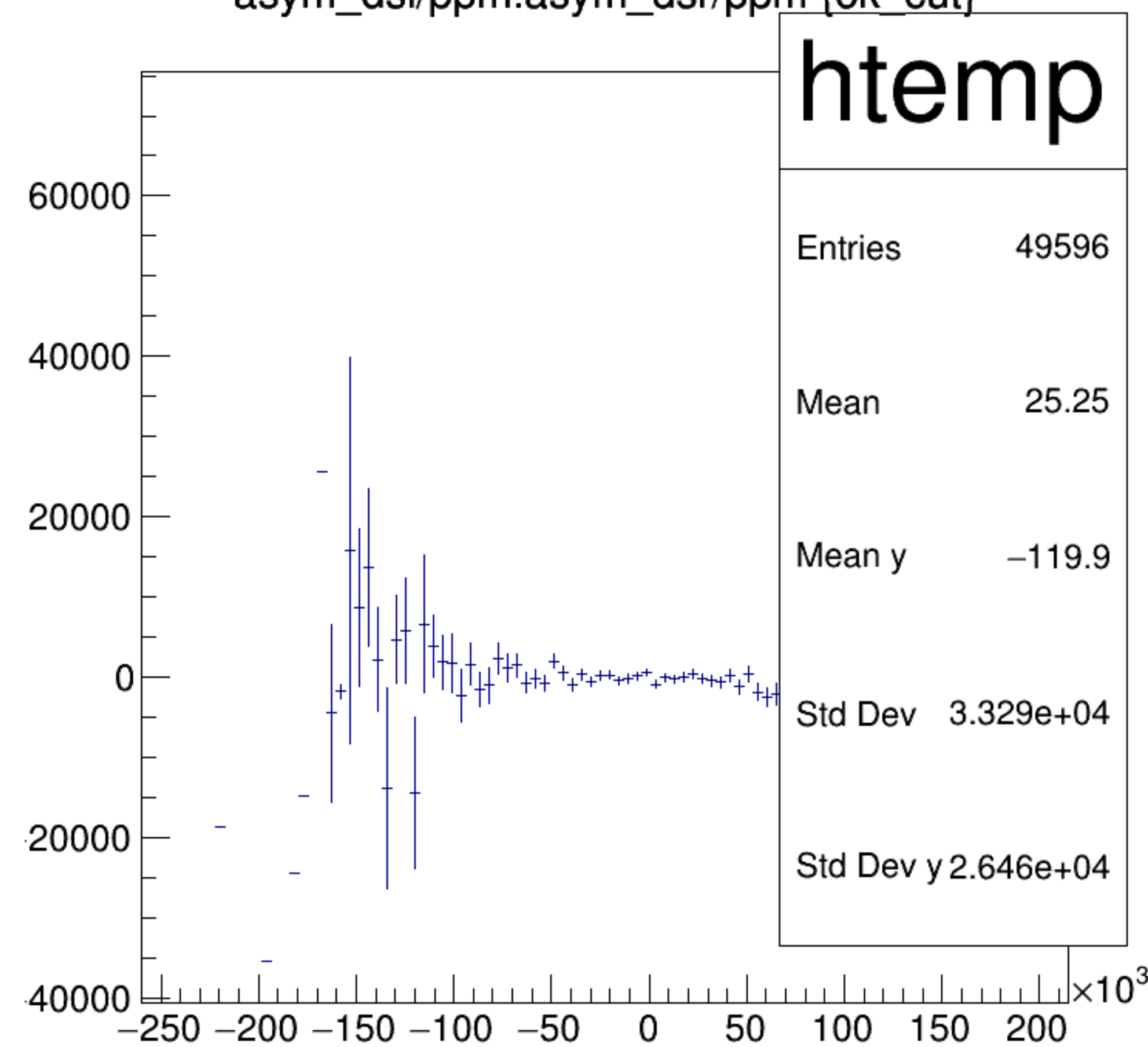
asym_dsl/ppm:asym_dsr/ppm {ok_cut}
