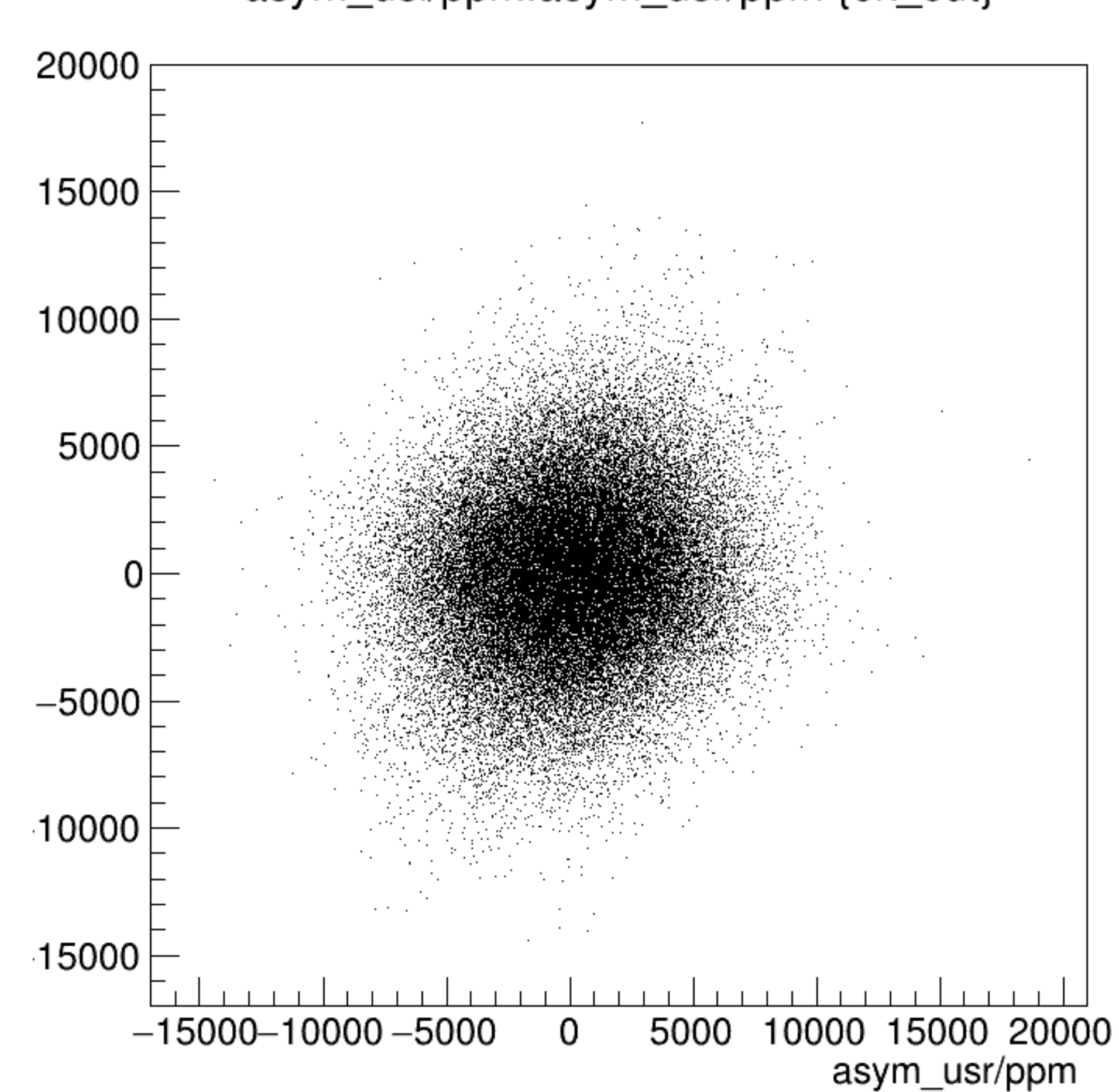
asym_usl/ppm:asym_usr/ppm {ok_cut}
