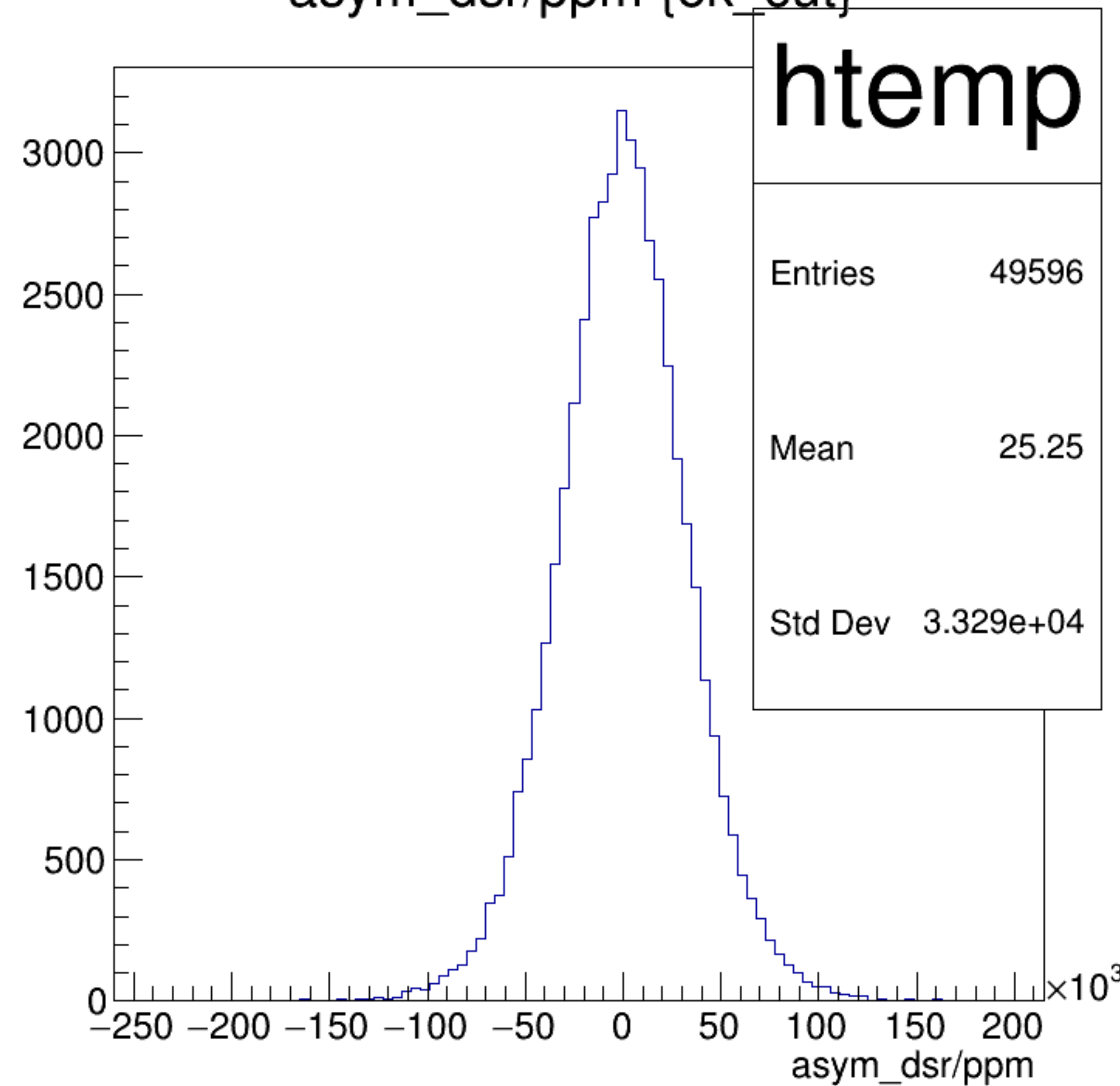
asym_dsr/ppm {ok_cut}
