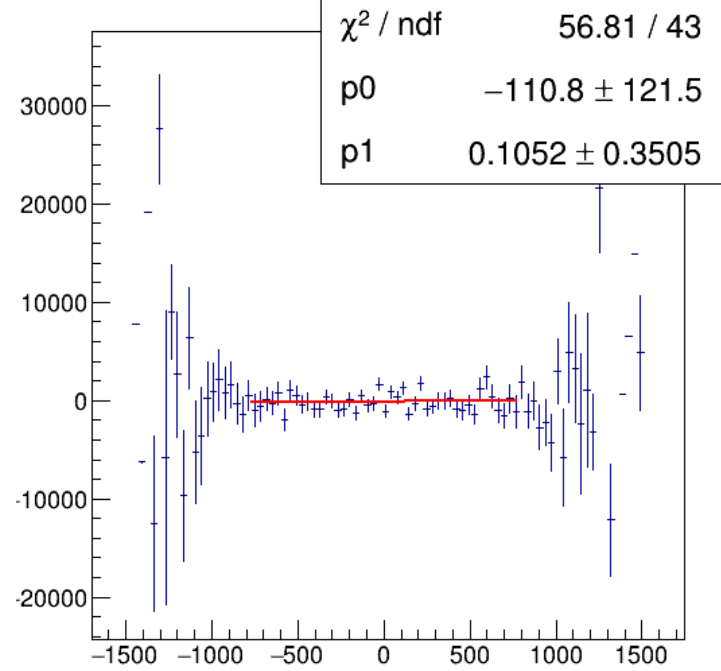
reg_asym_dsl/ppm:AqDS/ppm {ok_cut}
