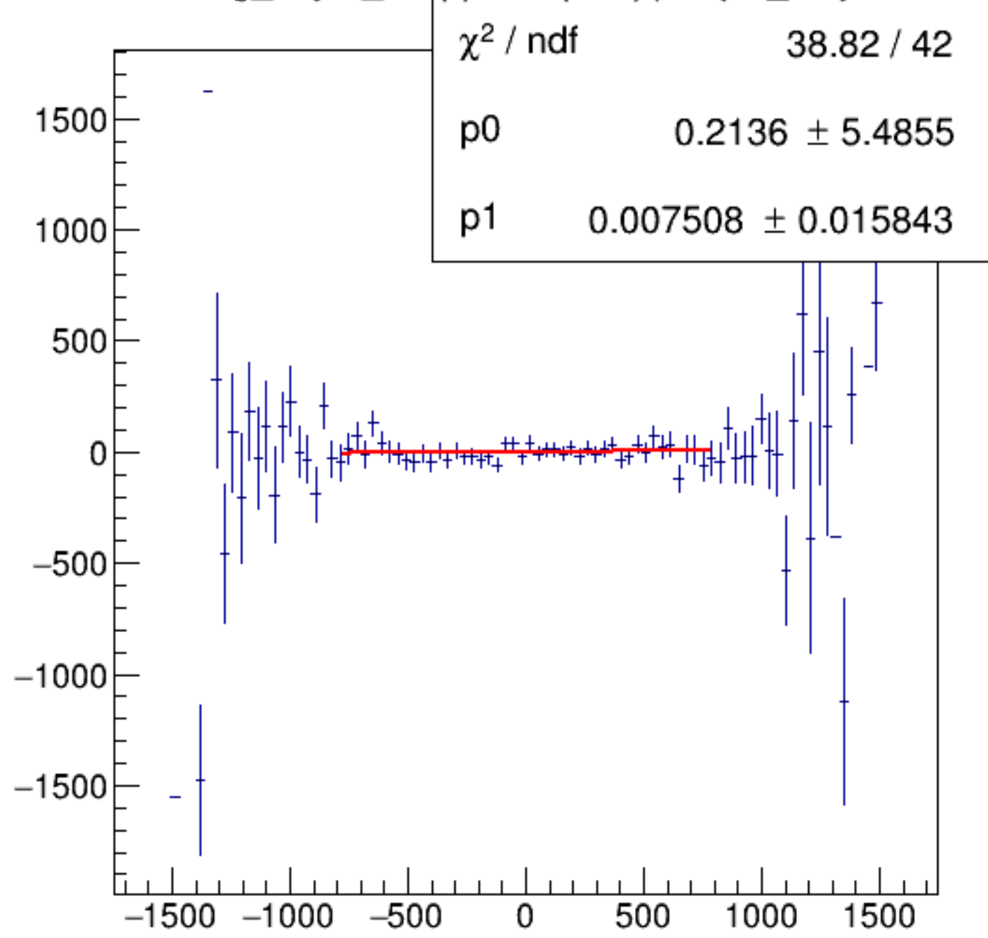
reg_asym_usl/ppm:AqUS/ppm {ok_cut}
