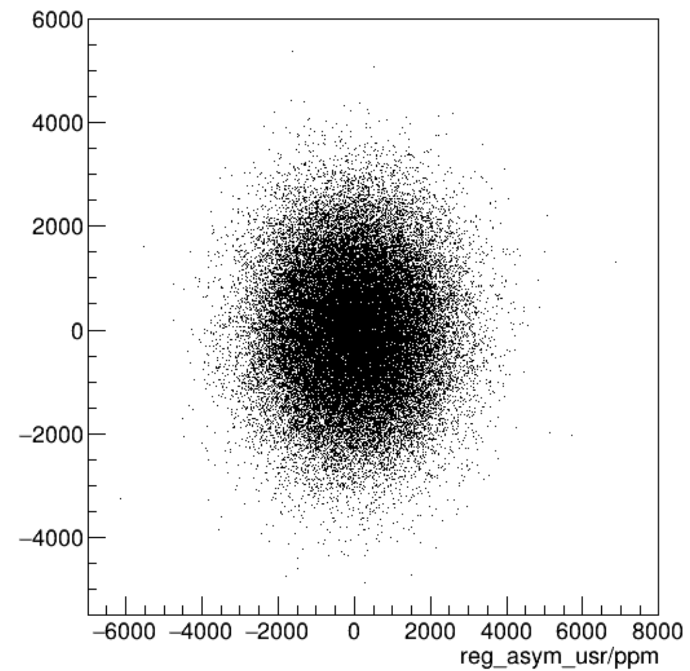
reg_asym_usl/ppm:reg_asym_usr/ppm {ok_cut}
