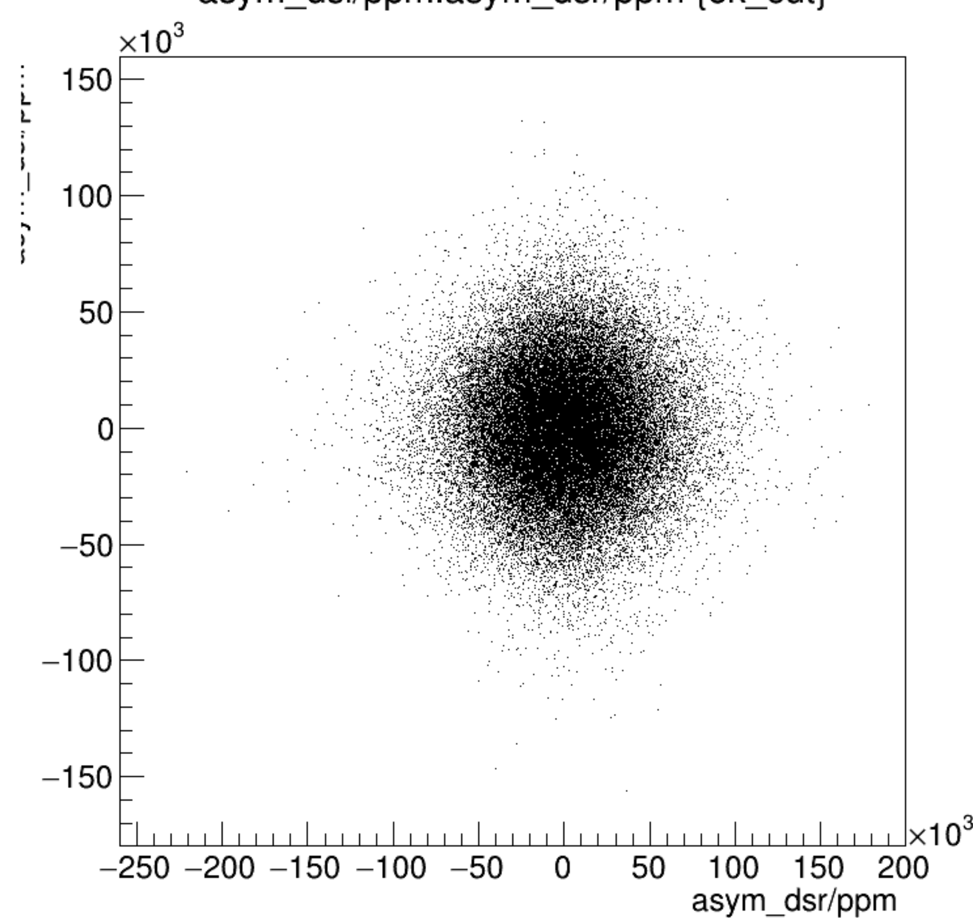
asym_dsl/ppm:asym_dsr/ppm {ok_cut}
