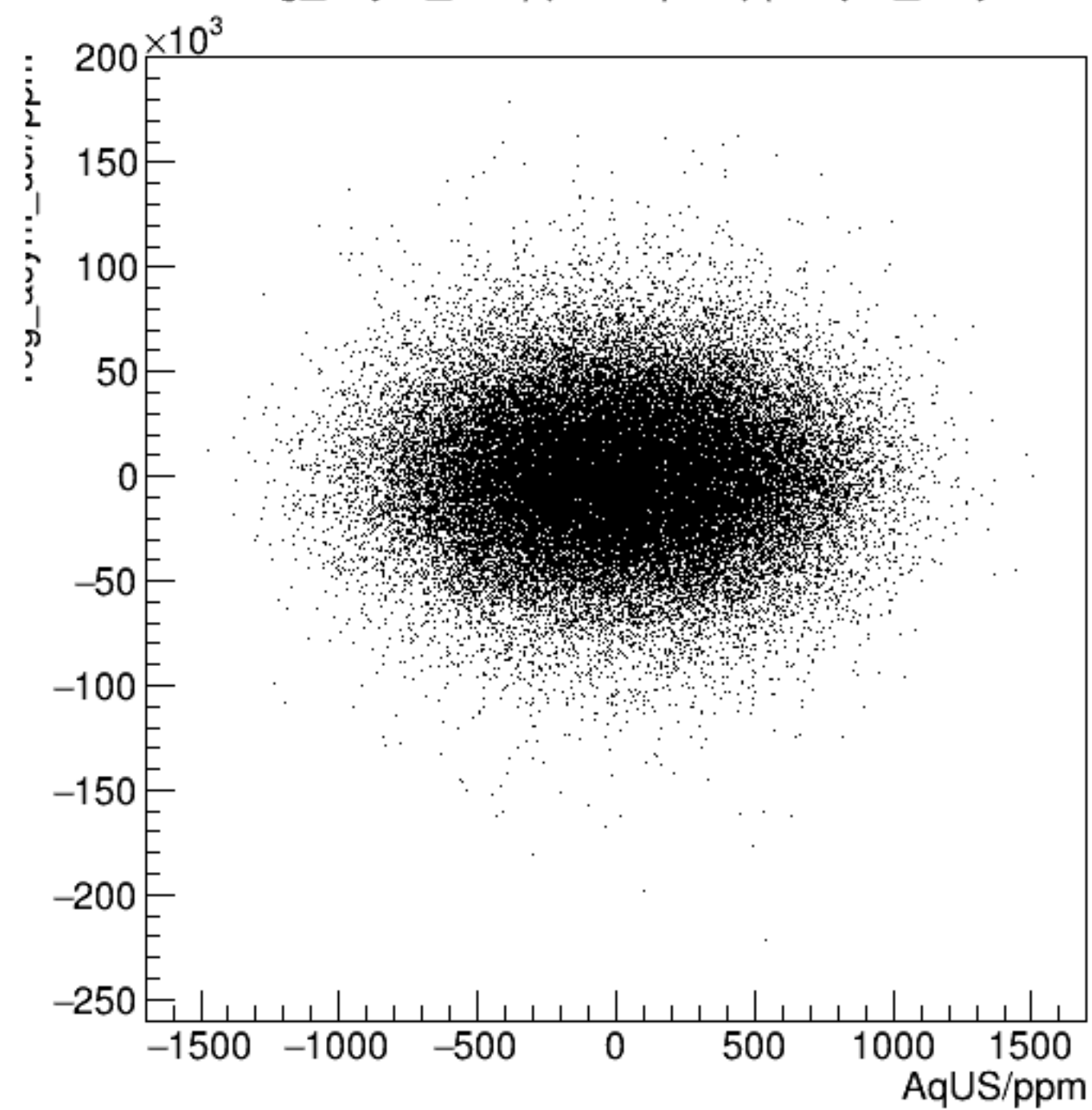
reg_asym_dsr/ppm:AqUS/ppm {ok_cut}
