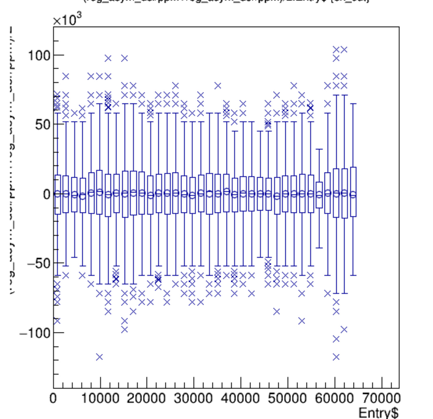
(reg_asym_dsl/ppm+reg_asym_dsr/ppm)/2:Entry$ {ok_cut}
