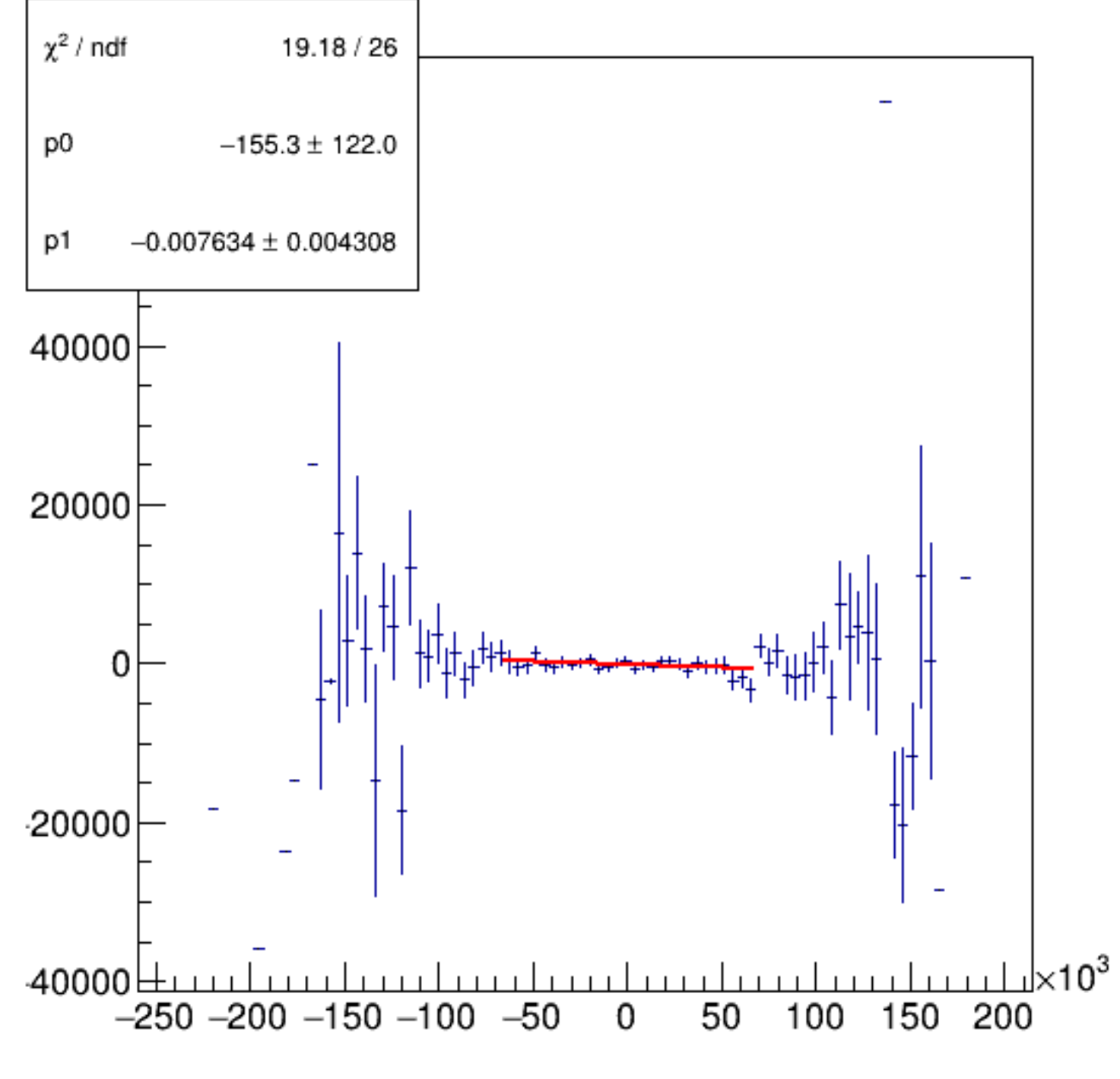
reg_asym_dsl/ppm:reg_asym_dsr/ppm {ok_cut}
