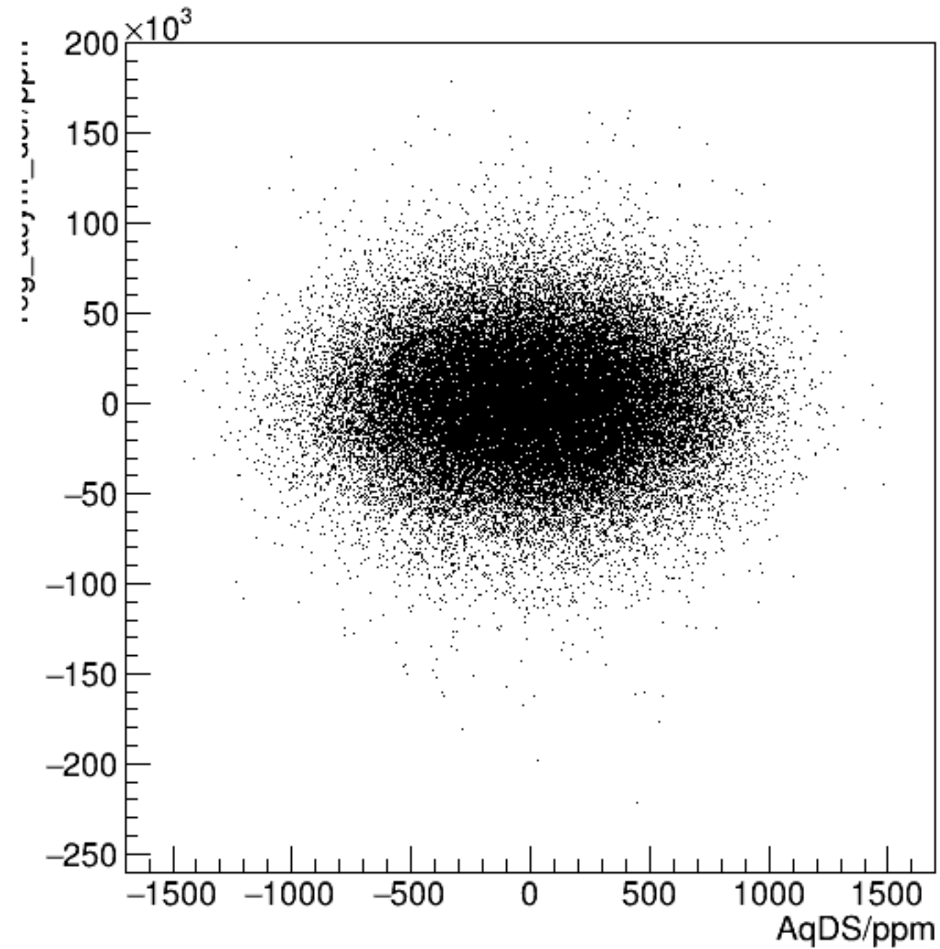
reg_asym_dsr/ppm:AqDS/ppm {ok_cut}
