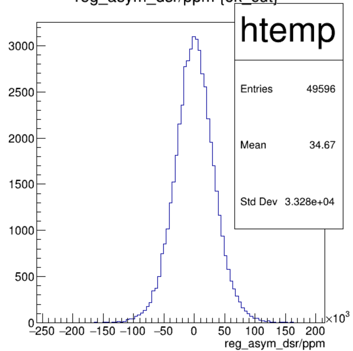
reg_asym_dsr/ppm {ok_cut}
