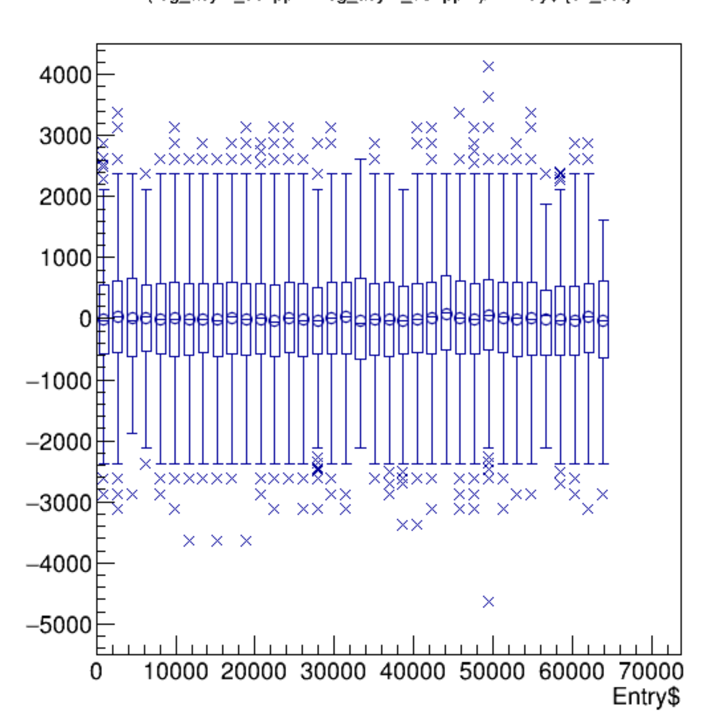
(reg_asym_usl/ppm+reg_asym_usr/ppm)/2:Entry$ {ok_cut}
