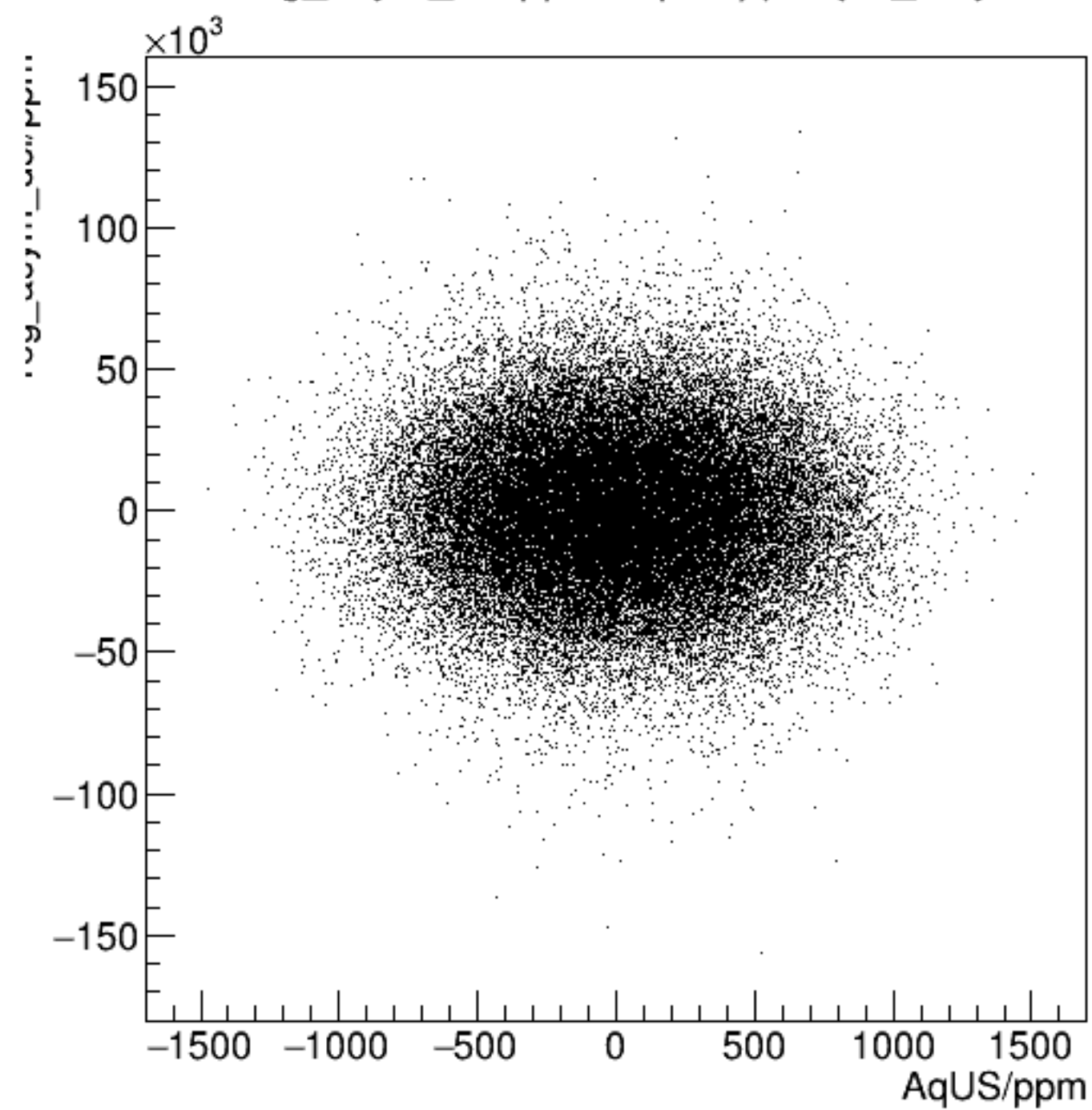
reg_asym_dsl/ppm:AqUS/ppm {ok_cut}
