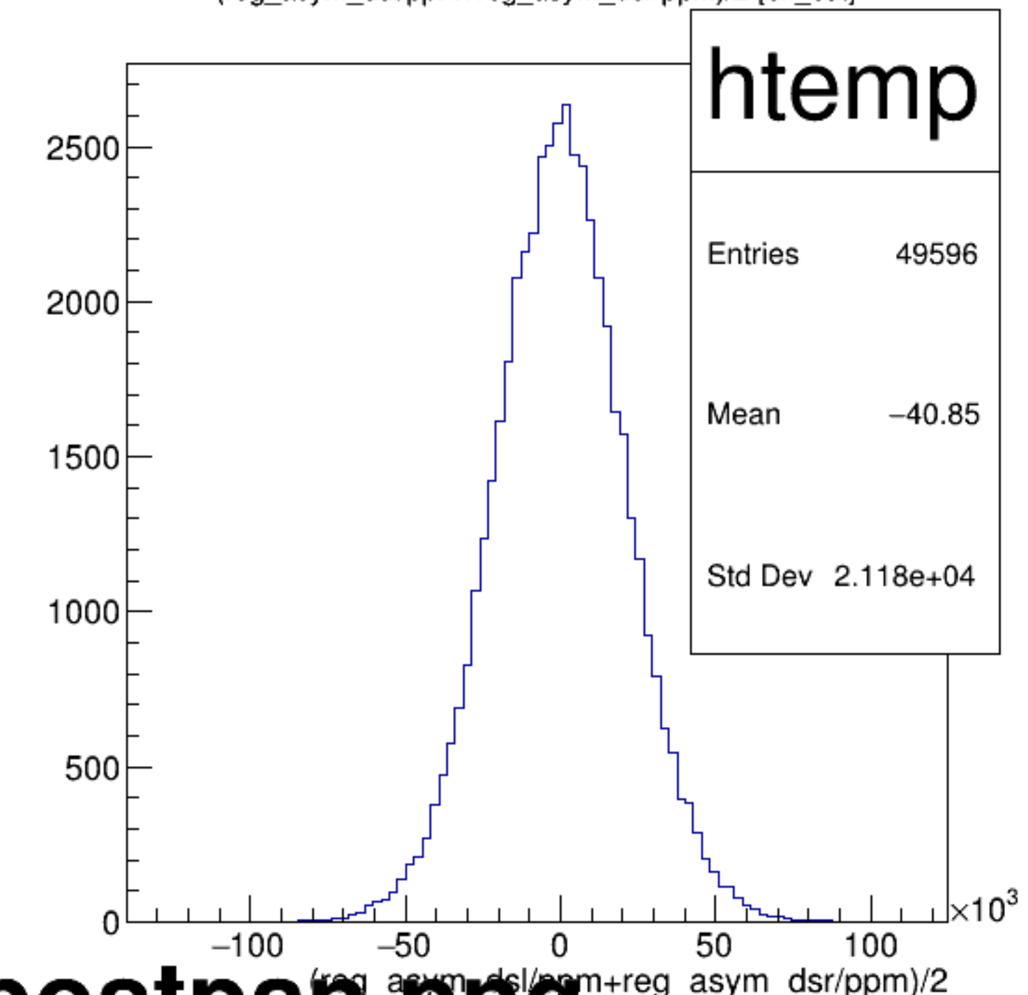
(reg_asym_dsl/ppm+reg_asym_dsr/ppm)/2 {ok_cut}
