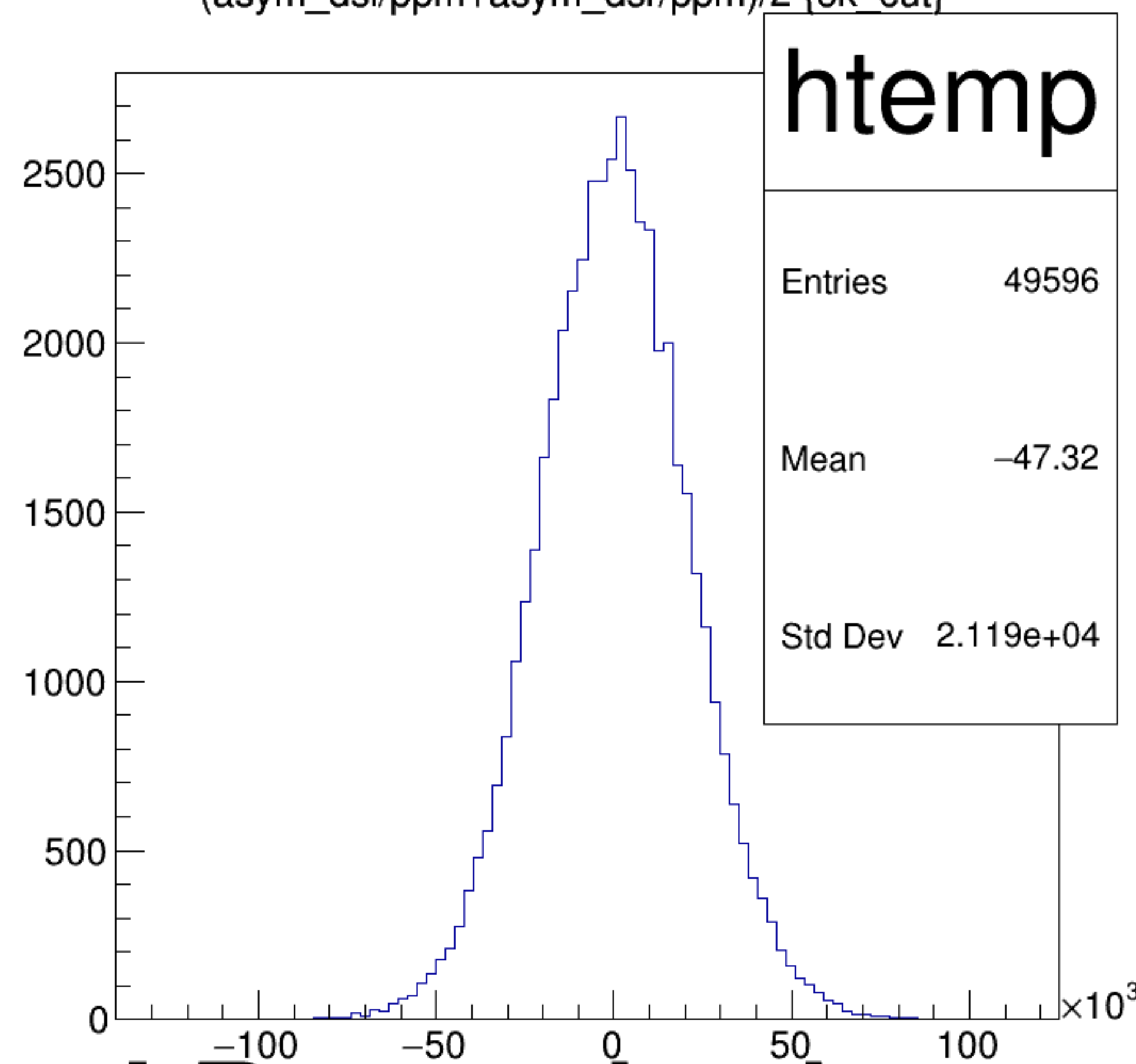
(asym_dsl/ppm+asym_dsr/ppm)/2 {ok_cut}
