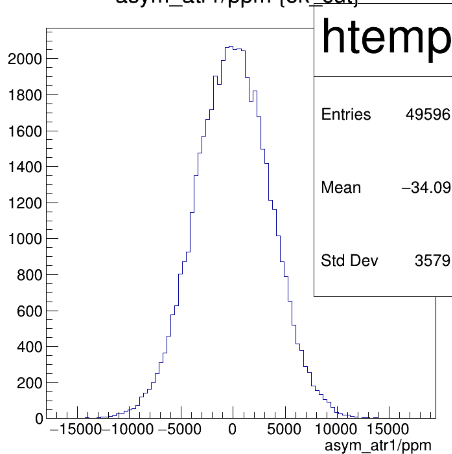
asym_atr1/ppm {ok_cut}
