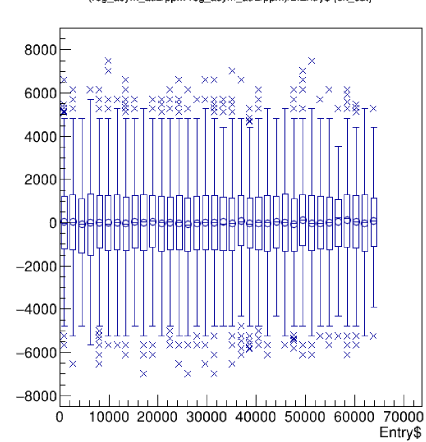
(reg_asym_atl2/ppm-reg_asym_atr2/ppm)/2:Entry$ {ok_cut}
