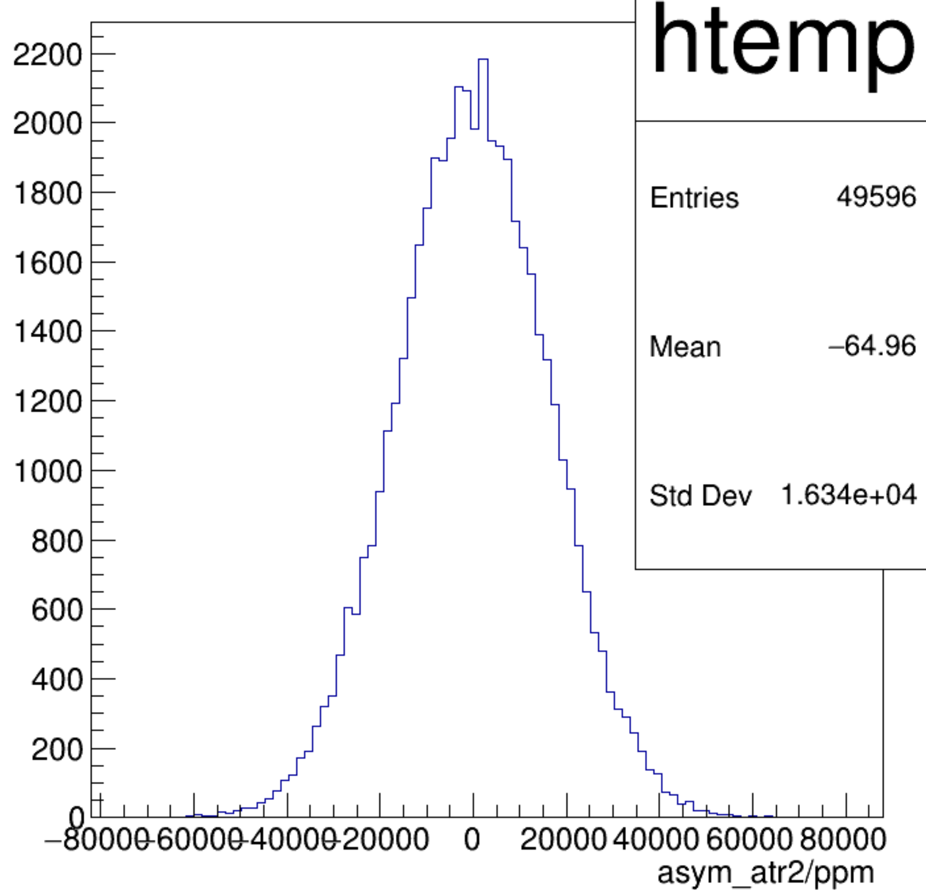
asym_atr2/ppm {ok_cut}
