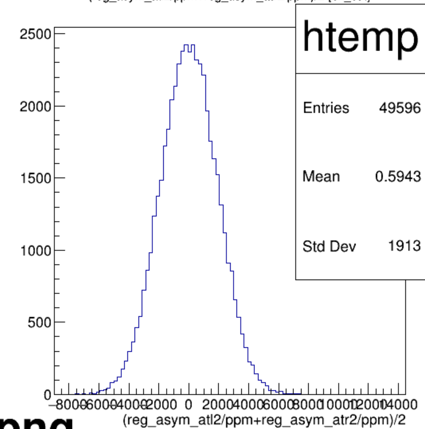
(reg_asym_atl2/ppm+reg_asym_atr2/ppm)/2 {ok_cut}
