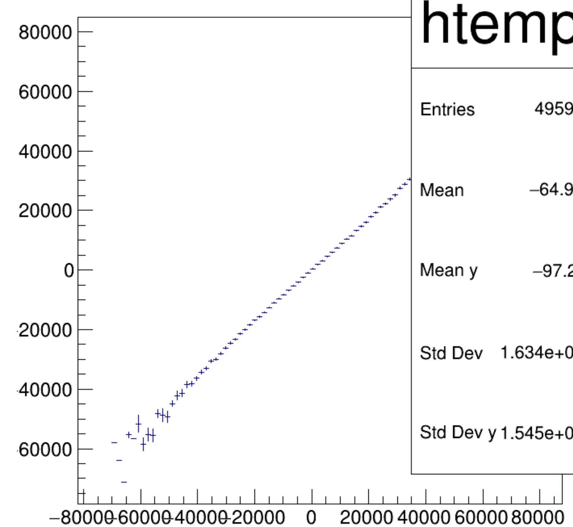
asym_atl2/ppm:asym_atr2/ppm {ok_cut}
