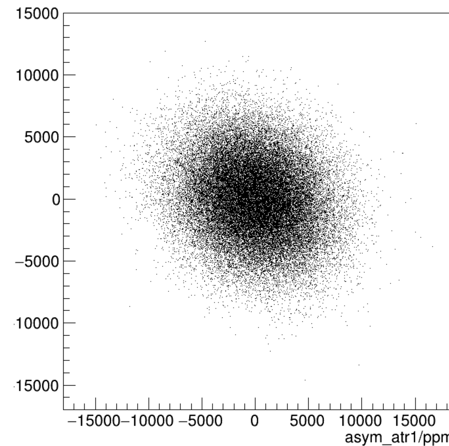
asym_atl1/ppm:asym_atr1/ppm {ok_cut}
