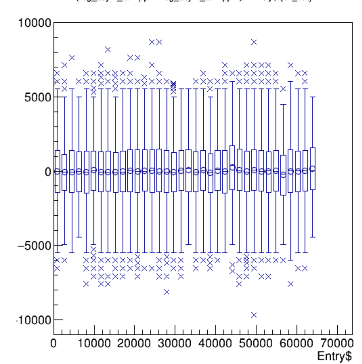
(reg_asym_atl1/ppm+reg_asym_atr1/ppm)/2:Entry$ {ok_cut}
