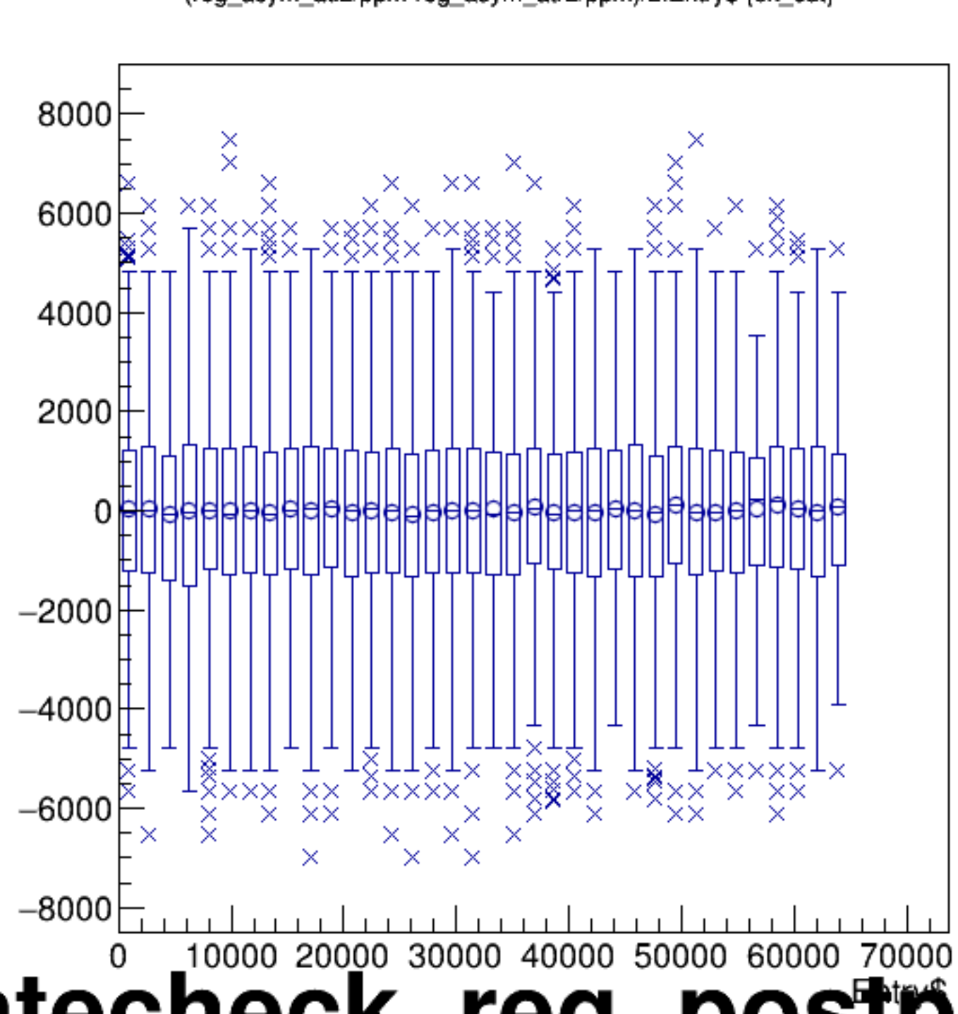
(reg_asym_atl2/ppm-reg_asym_atr2/ppm)/2:Entry$ {ok_cut}
