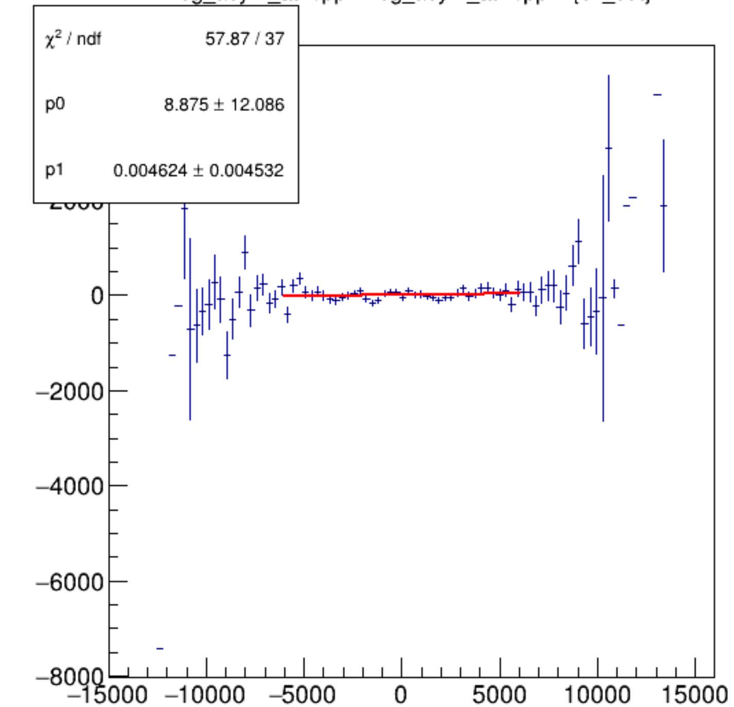
reg_asym_atl1/ppm:reg_asym_atr1/ppm {ok_cut}
