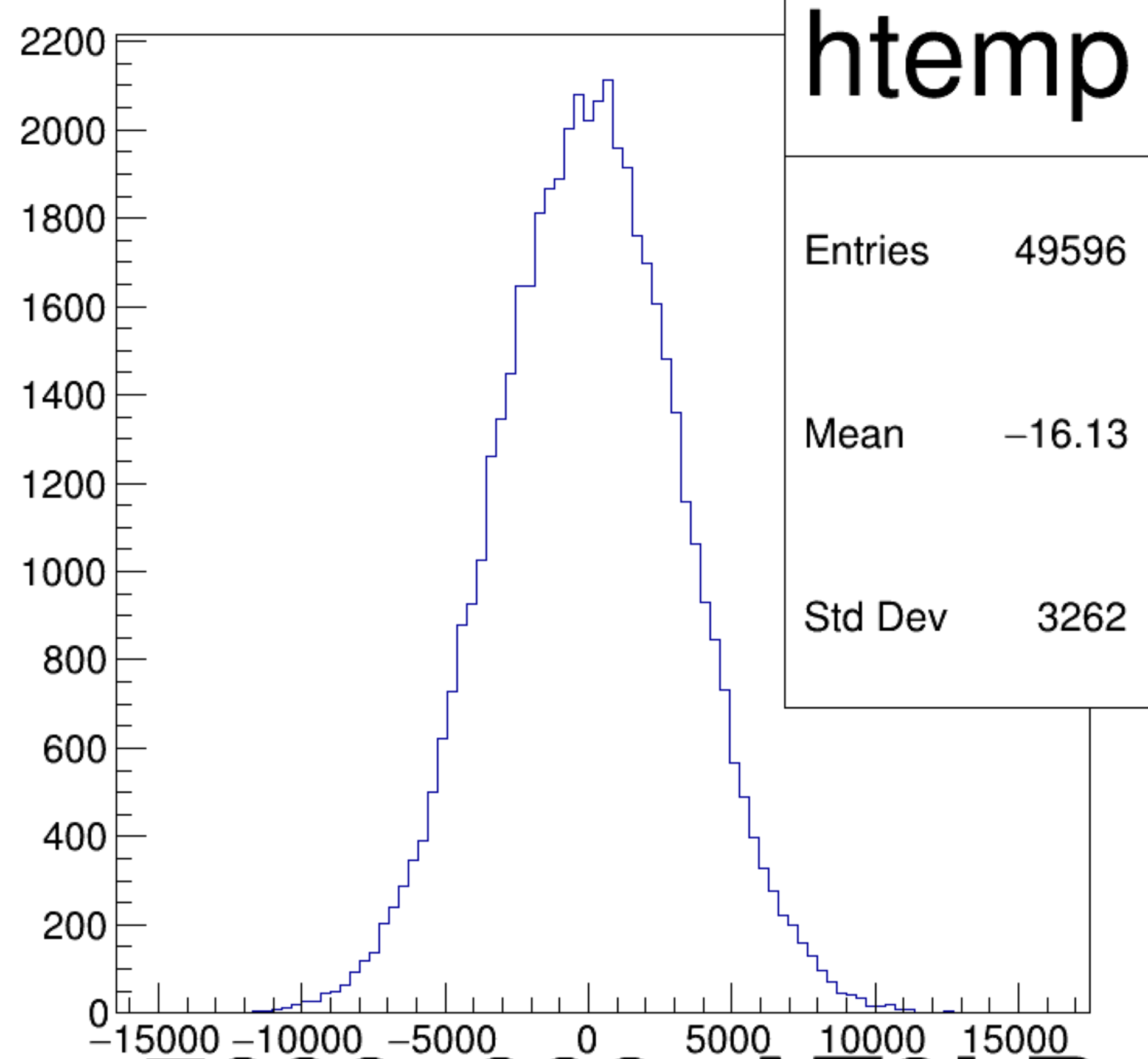
(asym_atl2/ppm-asym_atr2/ppm)/2 {ok_cut}
