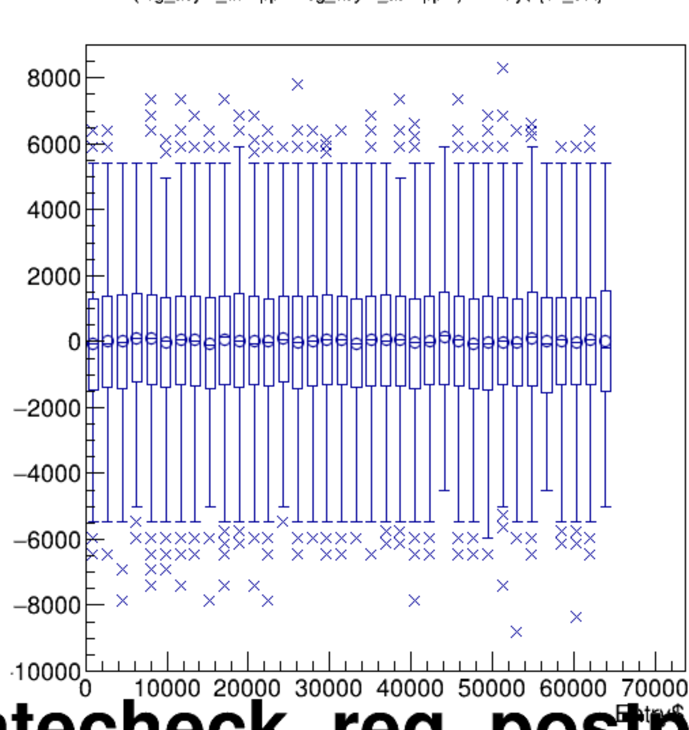
(reg_asym_atl1/ppm-reg_asym_atr1/ppm)/2:Entry$ {ok_cut}
