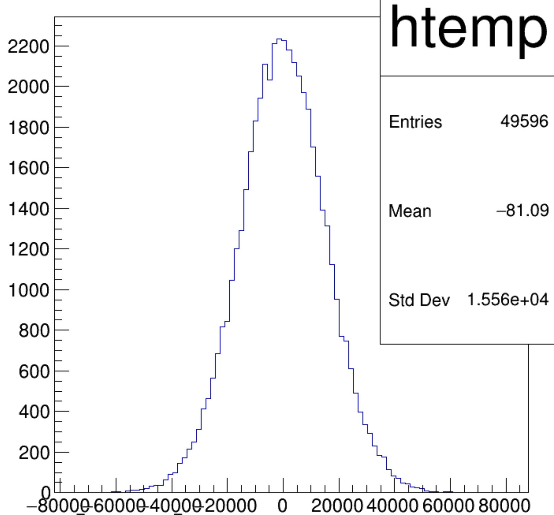
(asym_atl2/ppm+asym_atr2/ppm)/2 {ok_cut}
