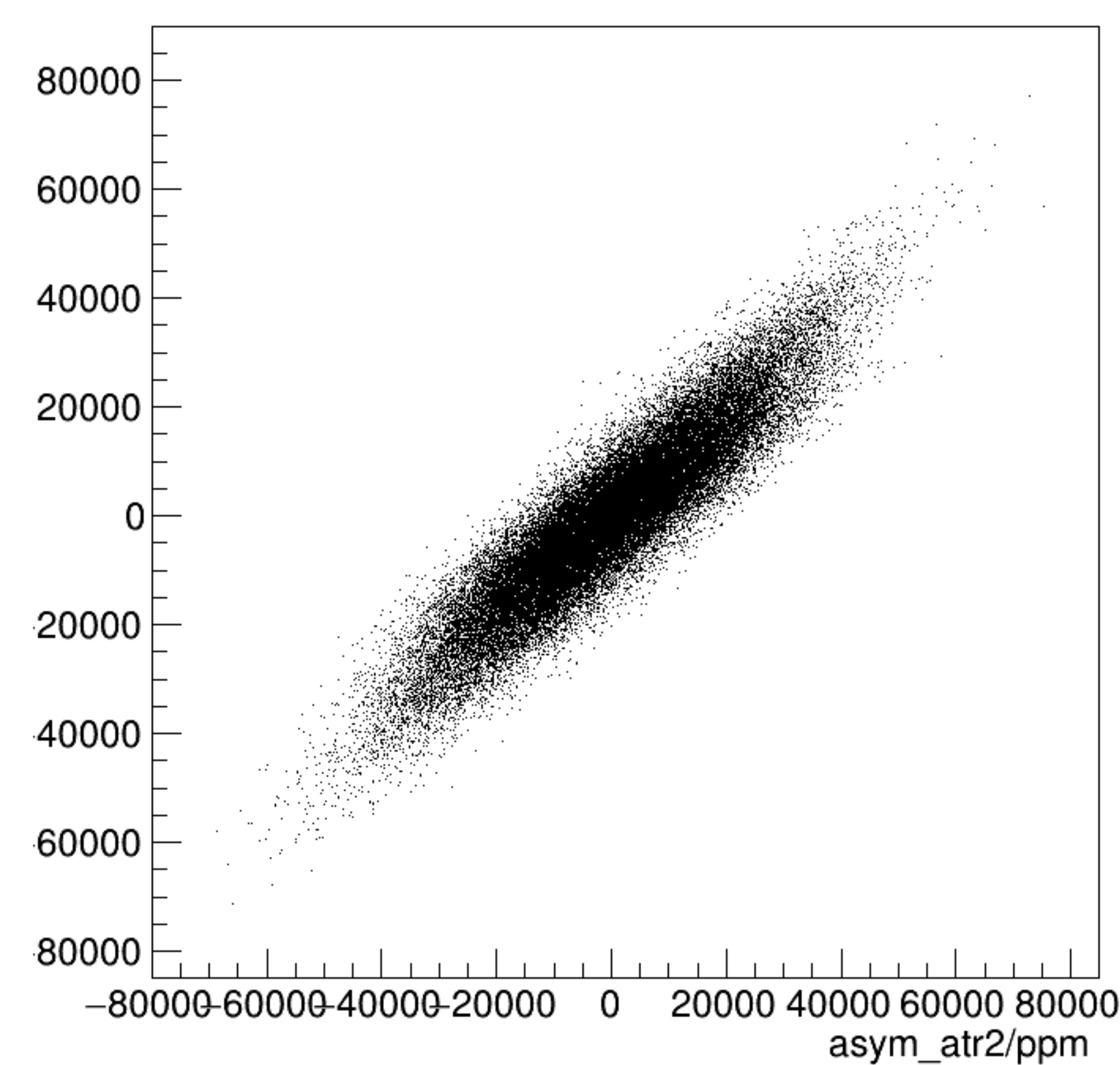
asym_atl2/ppm:asym_atr2/ppm {ok_cut}
