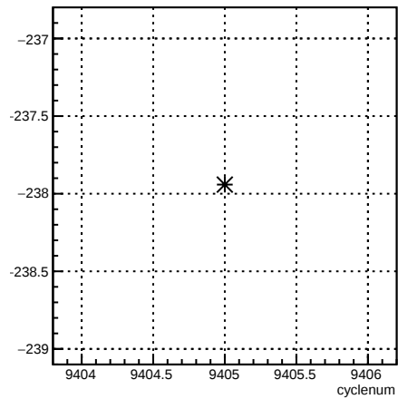
11X12X_coil6:cyclenum {run == 7789}
