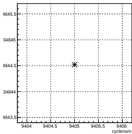
usr_coil7:cyclenum {run == 7789}
