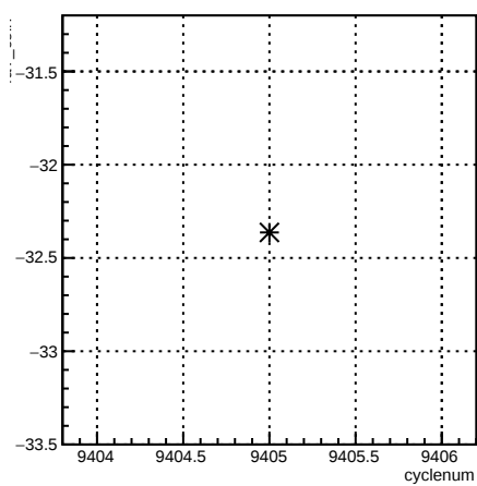
4aY_coil7:cyclenum {run == 7789}
