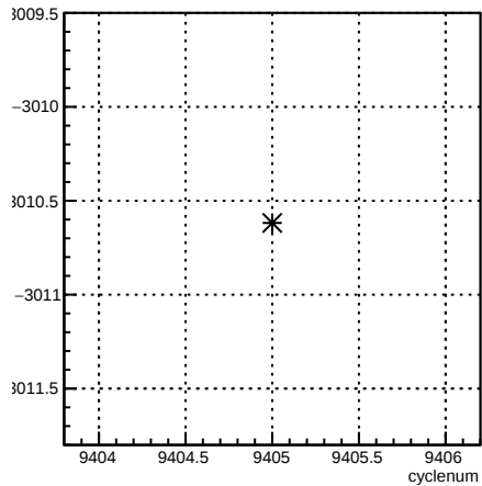
usr_coil6:cyclenum {run == 7789}
