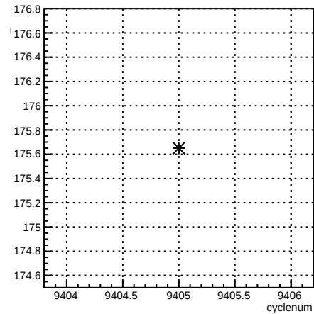
usr_4eX:cyclenum {run == 7789}
