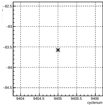
11X12X_coil7:cyclenum {run == 7789}
