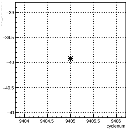
usl_11X12X:cyclenum {run == 7789}
