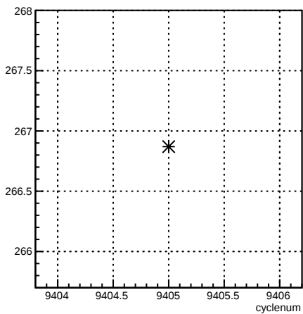
4eY_coil4:cyclenum {run == 7789}
