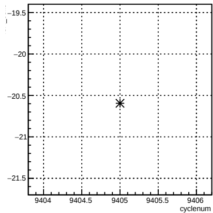
4eX_coil3:cyclenum {run == 7789}
