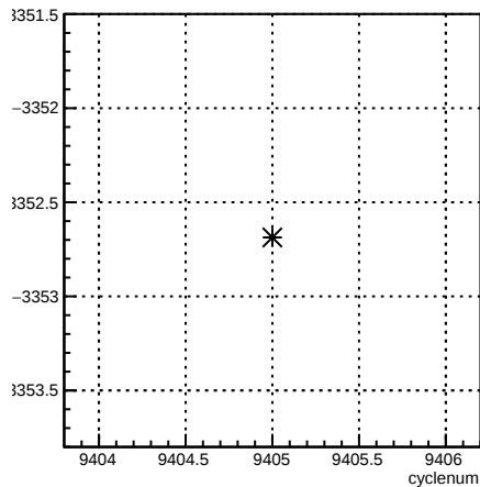
usl_coil6:cyclenum {run == 7789}
