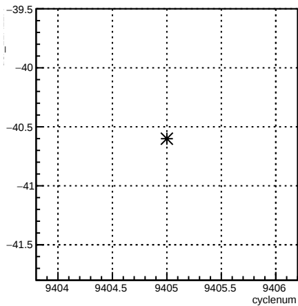
usr_11X12X:cyclenum {run == 7789}
