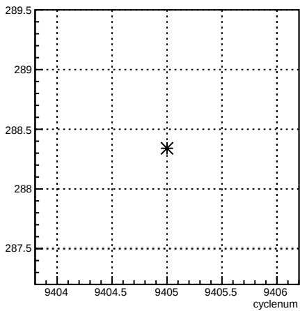
4aY_coil4:cyclenum {run == 7789}
