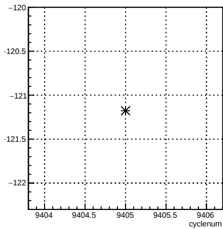
4aY_coil6:cyclenum {run == 7789}
