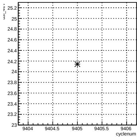
usl_4eY:cyclenum {run == 7789}
