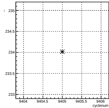
4eX_coil7:cyclenum {run == 7789}
