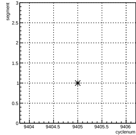
segment:cyclenum {run == 7789}
