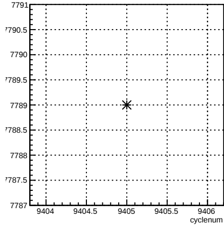
run:cyclenum {run == 7789}
