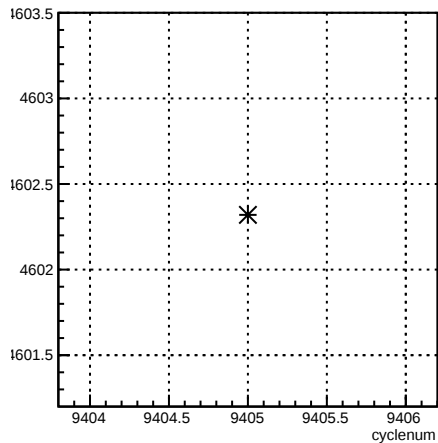
usl_coil7:cyclenum {run == 7789}
