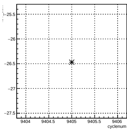
4eY_coil7:cyclenum {run == 7789}
