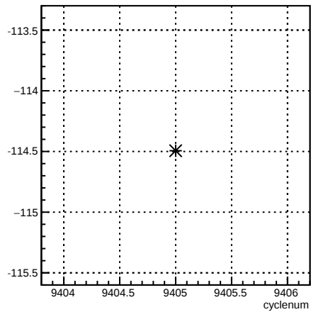
4eX_coil1:cyclenum {run == 7789}
