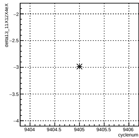
delta13_11X12X4eX:cyclenum {run == 7789}
