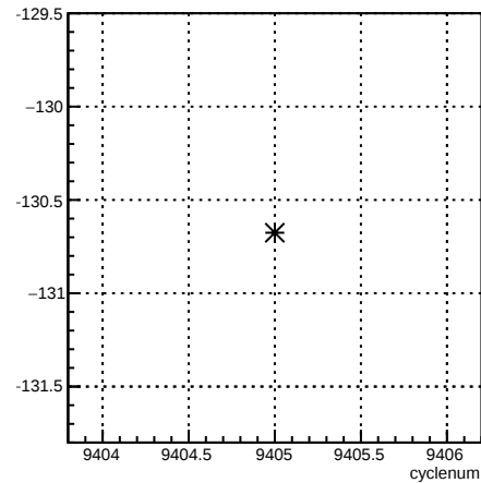
usr_4aX:cyclenum {run == 7789}
