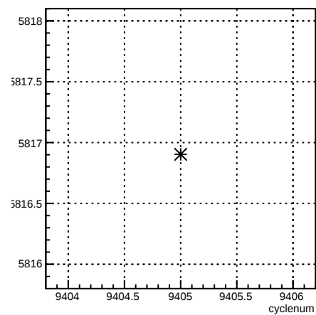
usl_coil4:cyclenum {run == 7789}
