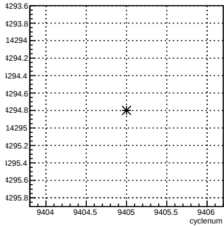
usr_coil1:cyclenum {run == 7789}
