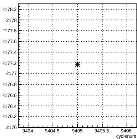
usl_coil3:cyclenum {run == 7789}
