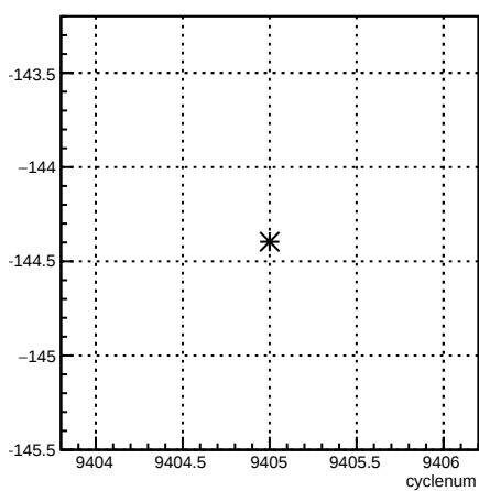
4eY_coil6:cyclenum {run == 7789}
