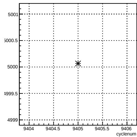
usr_coil4:cyclenum {run == 7789}
