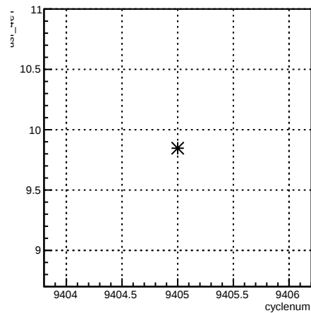
usr_4eY:cyclenum {run == 7789}
