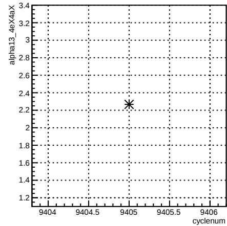
alpha13_4eX4aX:cyclenum {run == 7789}
