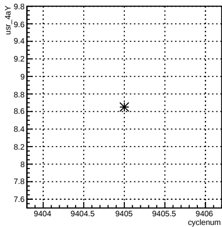
usr_4aY:cyclenum {run == 7789}
