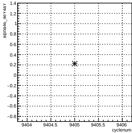
alpha46_4eY4aY:cyclenum {run == 7789}
