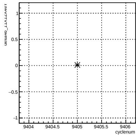
delta46_11X12X4eY:cyclenum {run == 7789}
