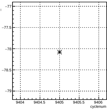
usl_4eY:cyclenum {run == 7789}
