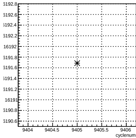
usl_coil1:cyclenum {run == 7789}
