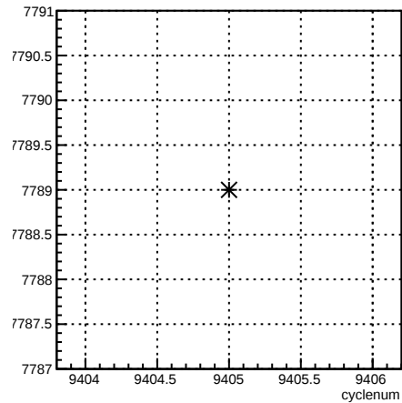
run:cyclenum {run == 7789}
