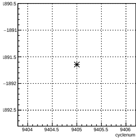
usr_coil3:cyclenum {run == 7789}
