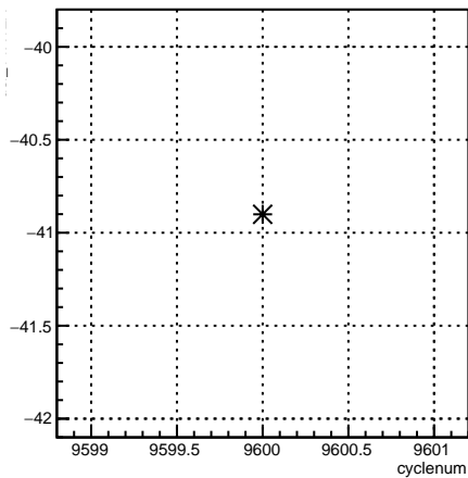
usl_11X12X:cyclenum {run == 7848}
