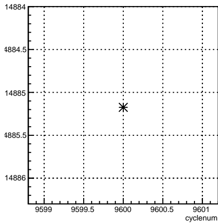
usr_coil1:cyclenum {run == 7848}
