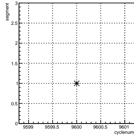
segment:cyclenum {run == 7848}
