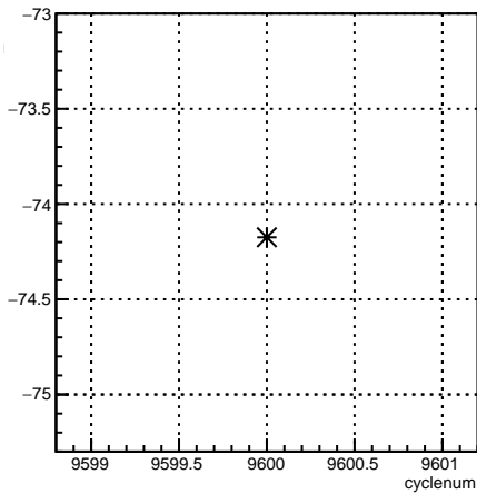
usl_4aX:cyclenum {run == 7848}
