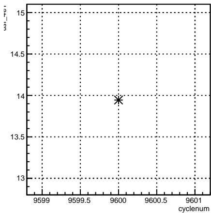
usr_4eY:cyclenum {run == 7848}
