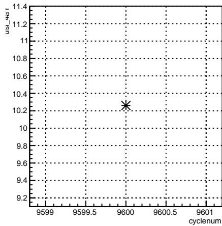
usl_4aY:cyclenum {run == 7848}
