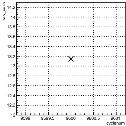
4eX_coil3:cyclenum {run == 7848}
