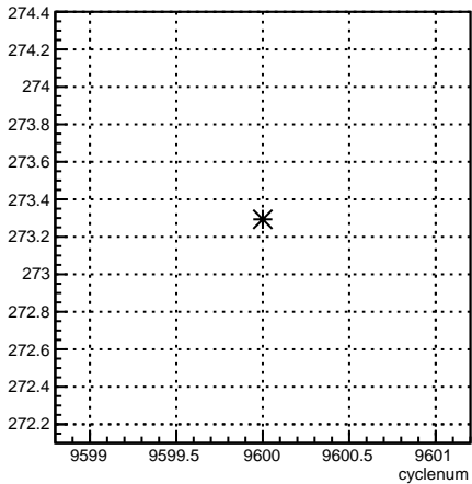
4eY_coil4:cyclenum {run == 7848}
