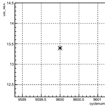
usl_4eX:cyclenum {run == 7848}
