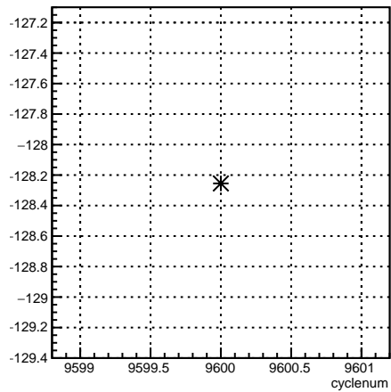
4eX_coil1:cyclenum {run == 7848}
