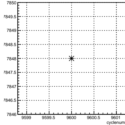
run:cyclenum {run == 7848}
