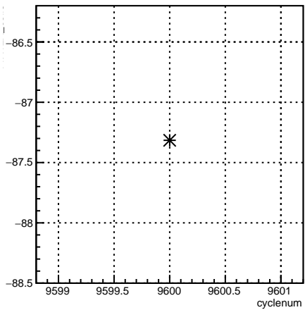
11X12X_coil7:cyclenum {run == 7848}
