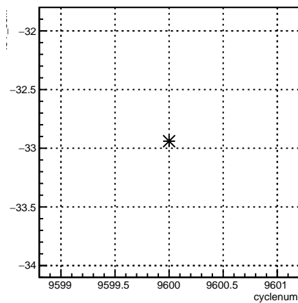
4eY_coil7:cyclenum {run == 7848}
