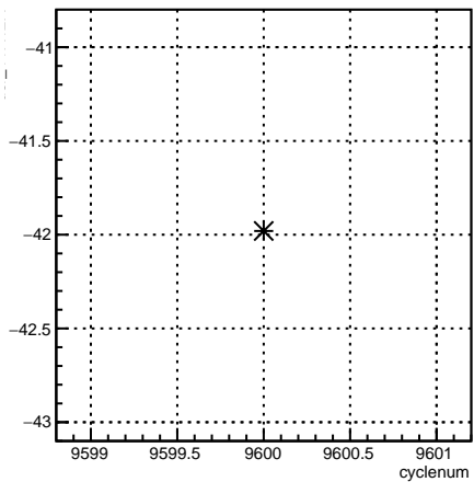
usr_11X12X:cyclenum {run == 7848}
