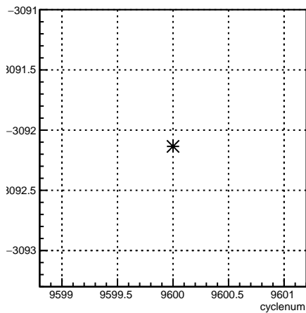
usr_coil6:cyclenum {run == 7848}
