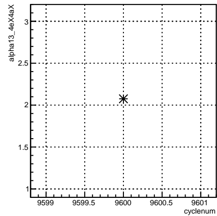
alpha13_4eX4aX:cyclenum {run == 7848}
