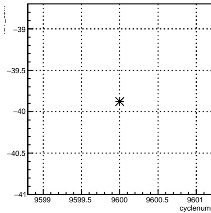
4eY_coil7:cyclenum {run == 7848}
