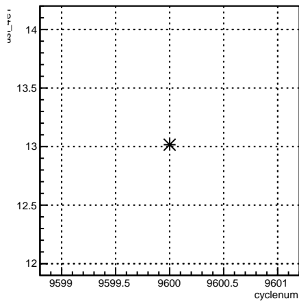
usl_4eY:cyclenum {run == 7848}
