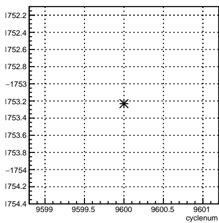
usr_coil3:cyclenum {run == 7848}
