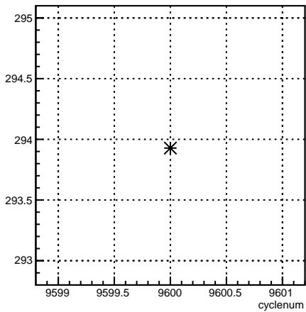
4eY_coil4:cyclenum {run == 7848}
