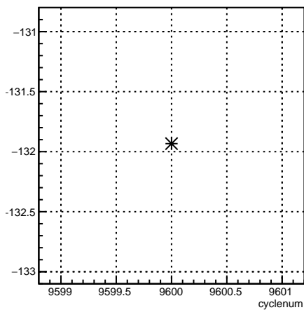
4eY_coil6:cyclenum {run == 7848}
