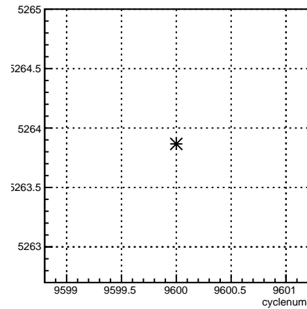
usr_coil4:cyclenum {run == 7848}
