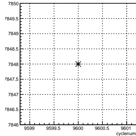
run:cyclenum {run == 7848}
