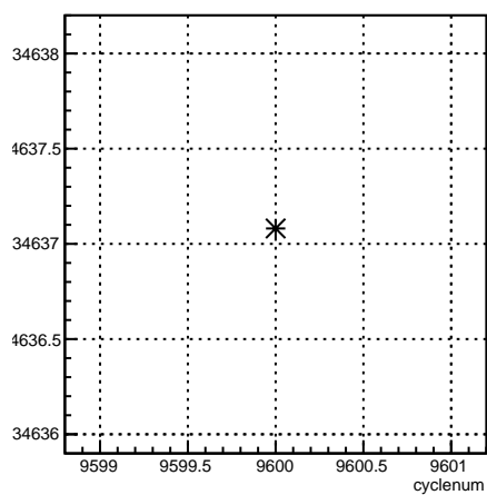
usr_coil7:cyclenum {run == 7848}
