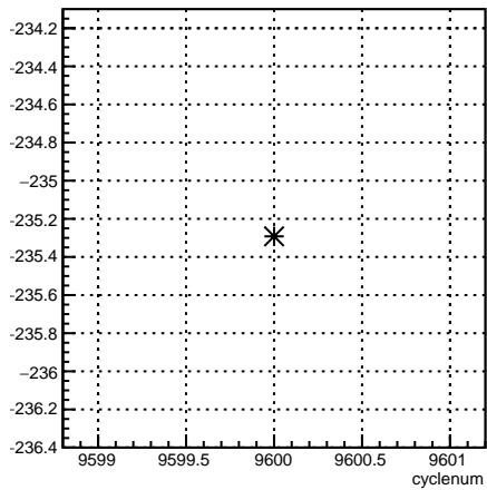
11X12X_coil6:cyclenum {run == 7848}
