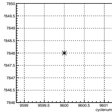
run:cyclenum {run == 7848}
