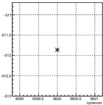
11X12X_coil7:cyclenum {run == 7848}
