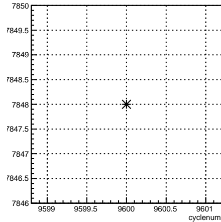
run:cyclenum {run == 7848}
