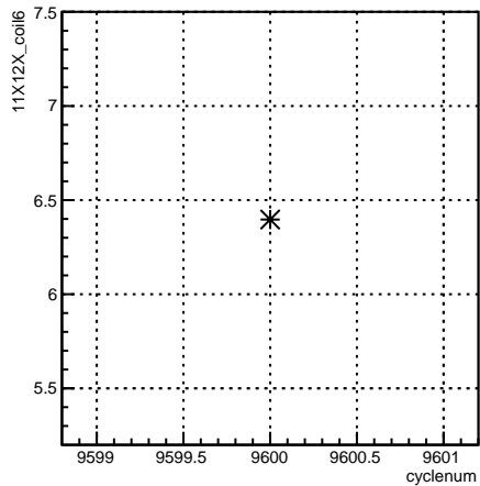
11X12X_coil6:cyclenum {run == 7848}
