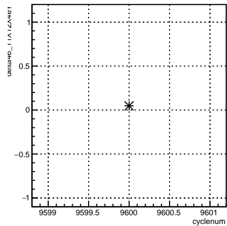
delta46_11X12X4eY:cyclenum {run == 7848}
