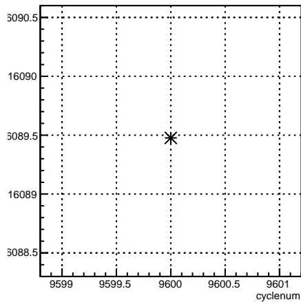
usl_coil6:cyclenum {run == 7848}
