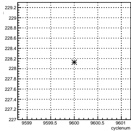
4eX_coil7:cyclenum {run == 7848}
