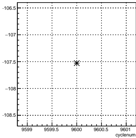
4eY_coil6:cyclenum {run == 7848}
