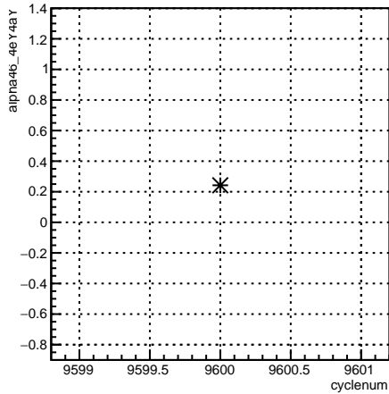
run:cyclenum {run == 7848}
