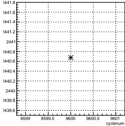
usl_coil7:cyclenum {run == 7848}
