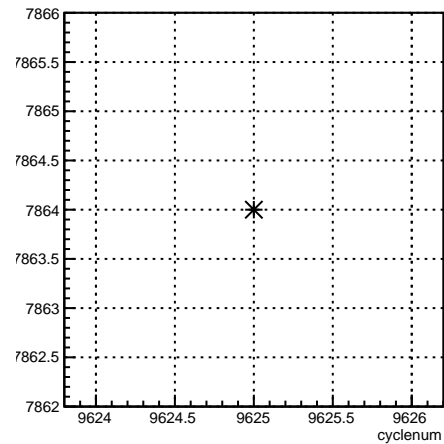
run:cyclenum {run == 7864}
