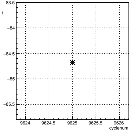
11X12X_coil3:cyclenum {run == 7864}
