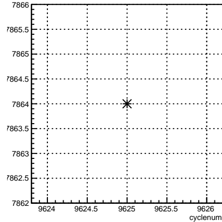
run:cyclenum {run == 7864}
