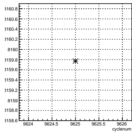
usr_coil4:cyclenum {run == 7864}
