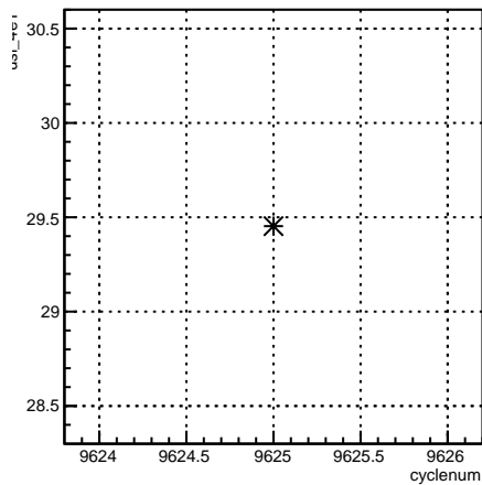
usl_4eY:cyclenum {run == 7864}
