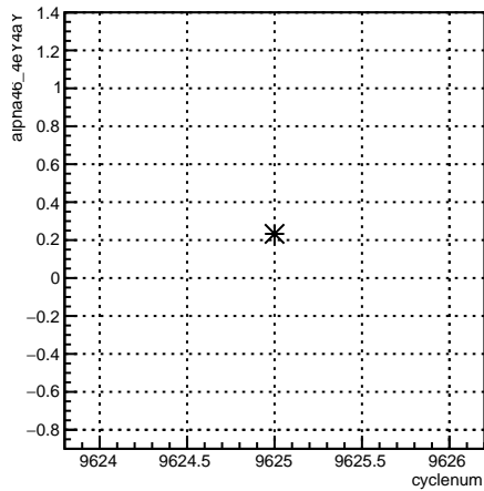
alpha46_4eY4aY:cyclenum {run == 7864}
