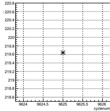
4aX_coil7:cyclenum {run == 7864}
