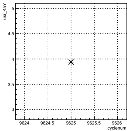
usr_4aY:cyclenum {run == 7864}
