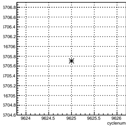
usl_coil6:cyclenum {run == 7864}
