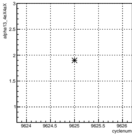
alpha13_4eX4aX:cyclenum {run == 7864}
