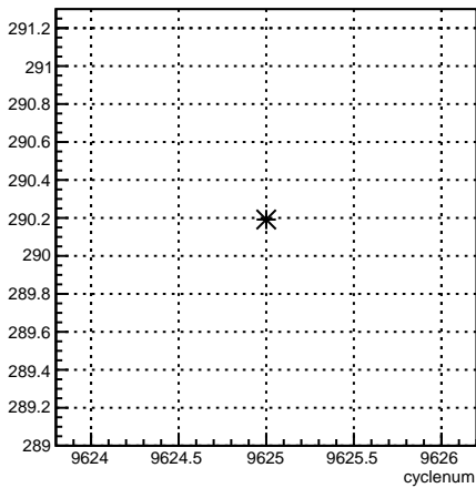
4eY_coil4:cyclenum {run == 7864}
