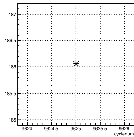
usr_4eX:cyclenum {run == 7864}
