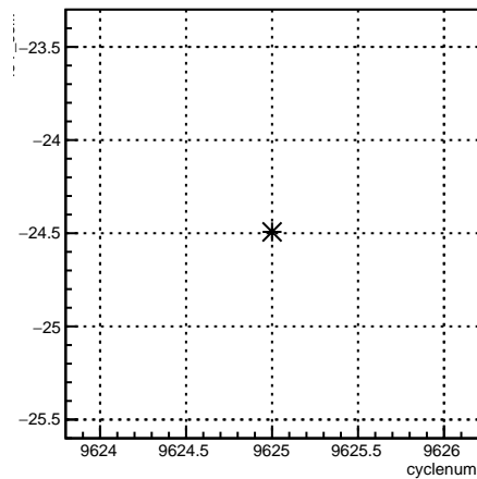
4eY_coil7:cyclenum {run == 7864}
