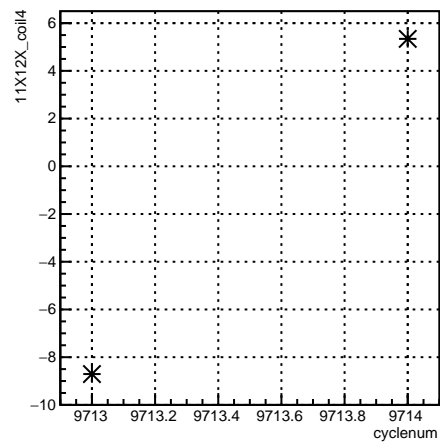
11X12X_coil4:cyclenum {run == 7895}
