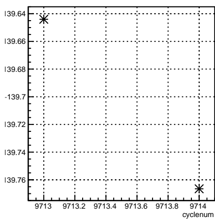
4eY_coil6:cyclenum {run == 7895}
