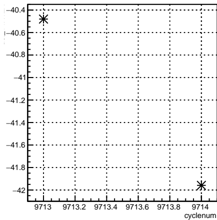
usl_11X12X:cyclenum {run == 7895}
