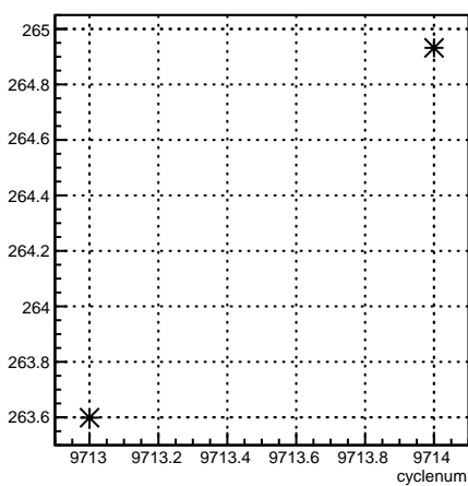
4eY_coil4:cyclenum {run == 7895}
