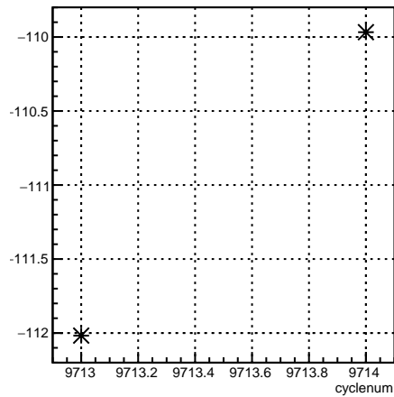
4eX_coil1:cyclenum {run == 7895}
