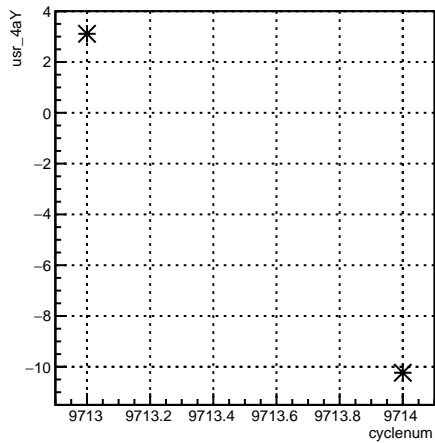
usr_4aY:cyclenum {run == 7895}
