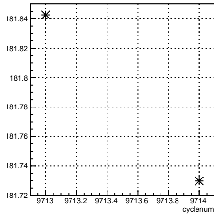
run:cyclenum {run == 7895}
