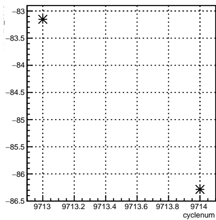
11X12X_coil3:cyclenum {run == 7895}
