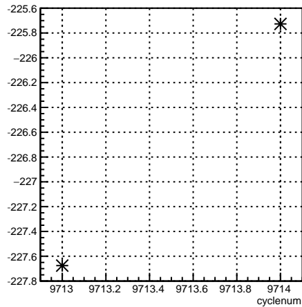
4eX_coil1:cyclenum {run == 7895}
