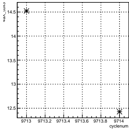
4eX_coil3:cyclenum {run == 7895}
