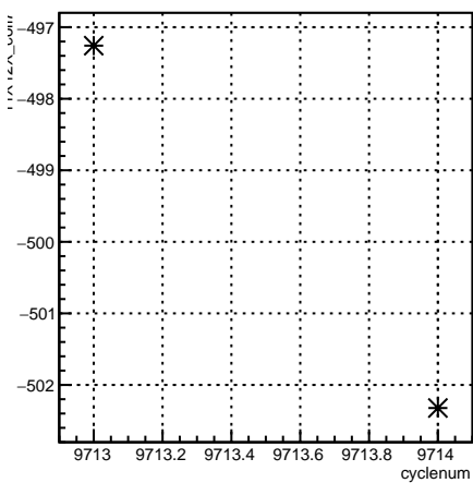
11X12X_coil7:cyclenum {run == 7895}
