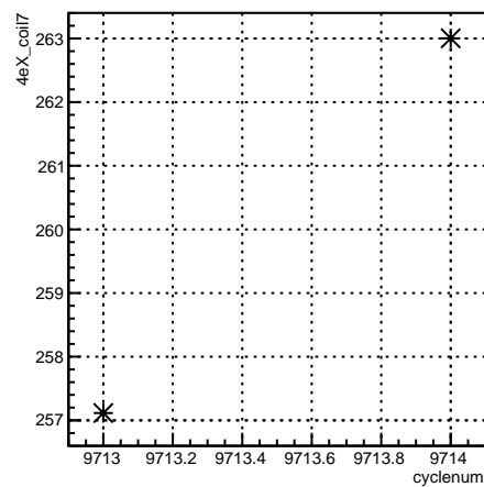
4eX_coil7:cyclenum {run == 7895}
