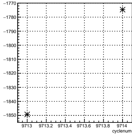
usr_coil3:cyclenum {run == 7895}
