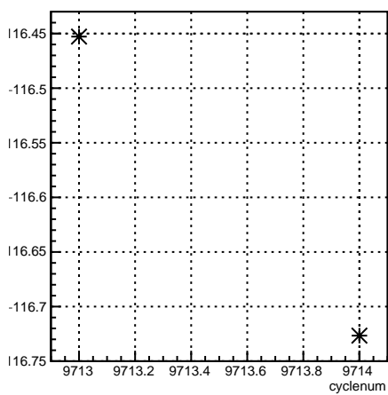
4aY_coil6:cyclenum {run == 7895}
