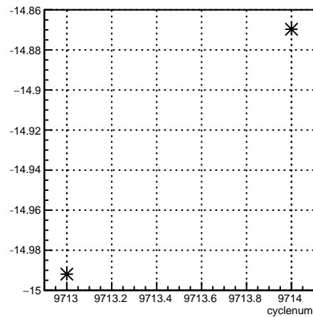
4eY_coil7:cyclenum {run == 7895}
