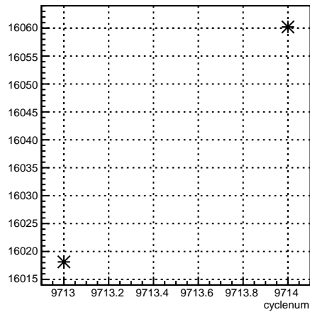
usl_coil6:cyclenum {run == 7895}
