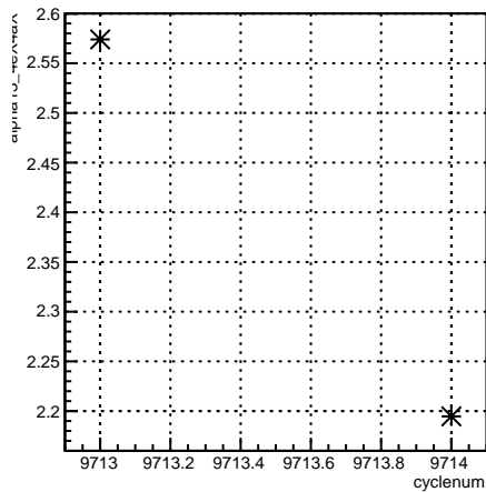
alpha13_4eX4aX:cyclenum {run == 7895}
