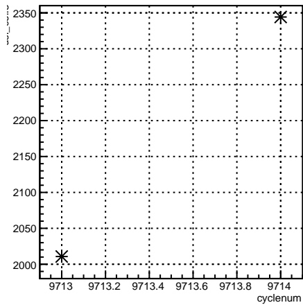
usl_coil7:cyclenum {run == 7895}
