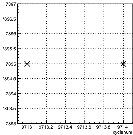
run:cyclenum {run == 7895}
