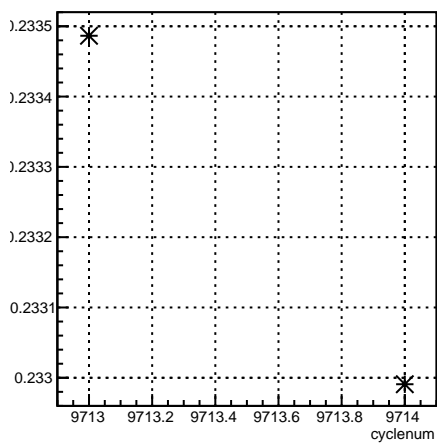
alpha46_4eY4aY:cyclenum {run == 7895}
