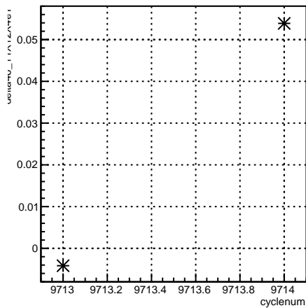
delta46_11X12X4eY:cyclenum {run == 7895}
