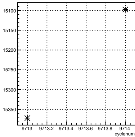
usr_coil6:cyclenum {run == 7895}
