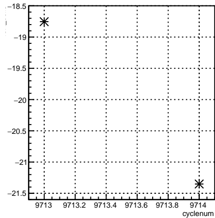
4eX_coil3:cyclenum {run == 7895}
