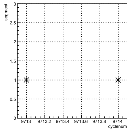
segment:cyclenum {run == 7895}
