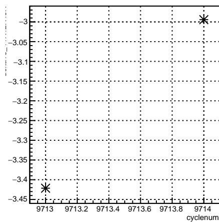
delta13_11X12X4eX:cyclenum {run == 7895}
