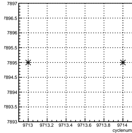
run:cyclenum {run == 7895}
