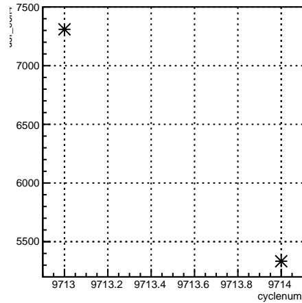
usr_coil4:cyclenum {run == 7895}
