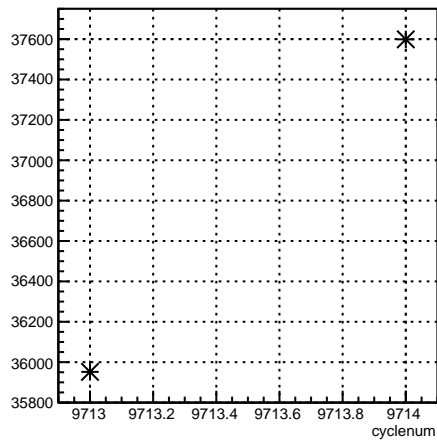
usr_coil7:cyclenum {run == 7895}
