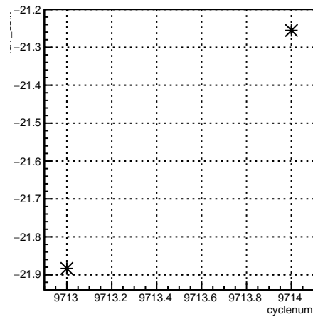
4aY_coil7:cyclenum {run == 7895}
