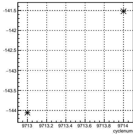
usr_4eY:cyclenum {run == 7895}
