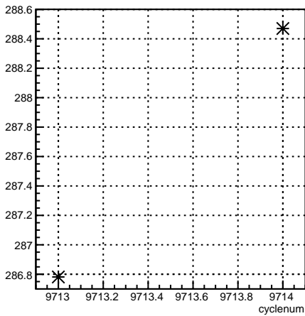
4aY_coil4:cyclenum {run == 7895}
