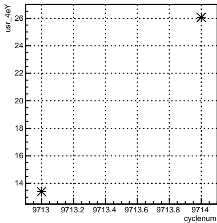
usr_4eY:cyclenum {run == 7895}
