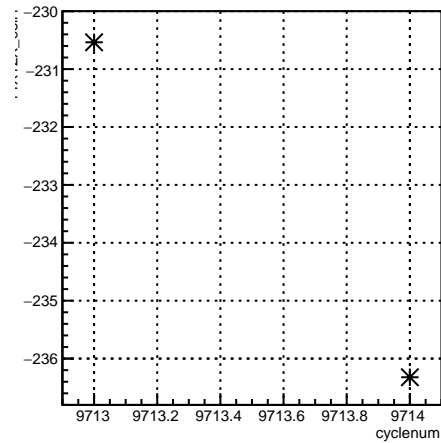
11X12X_coil1:cyclenum {run == 7895}
