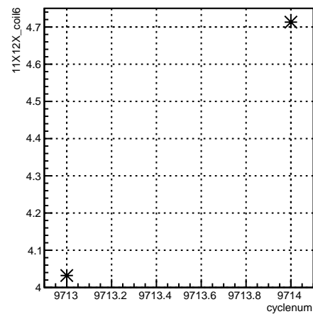
11X12X_coil6:cyclenum {run == 7895}
