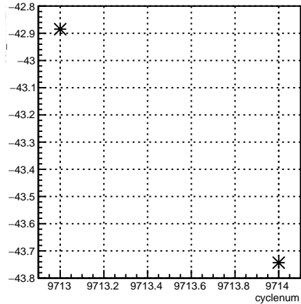
usr_11X12X:cyclenum {run == 7895}
