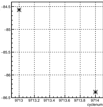
usl_4eY:cyclenum {run == 7895}
