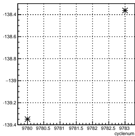
4eY_coil6:cyclenum {run == 7910}
