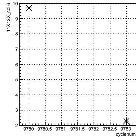
11X12X_coil6:cyclenum {run == 7910}
