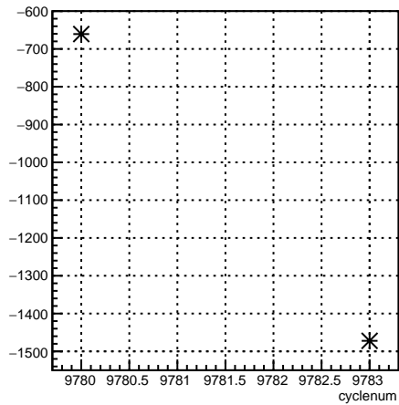
usr_coil3:cyclenum {run == 7910}
