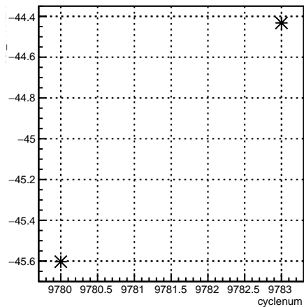
usr_11X12X:cyclenum {run == 7910}
