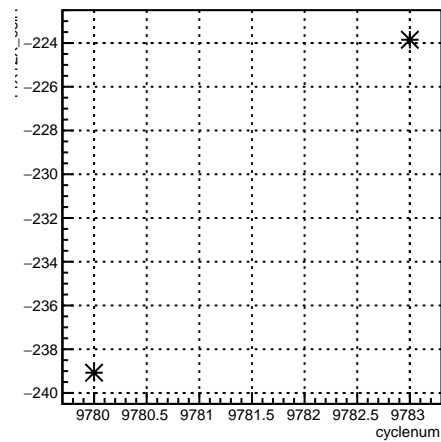
11X12X_coil1:cyclenum {run == 7910}
