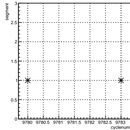
segment:cyclenum {run == 7910}
