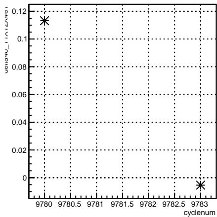
delta46_11X12X4eY:cyclenum {run == 7910}
