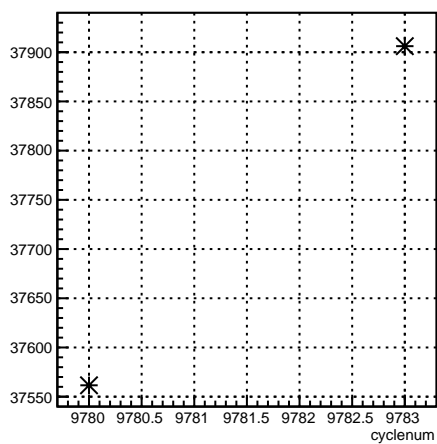
usr_coil7:cyclenum {run == 7910}
