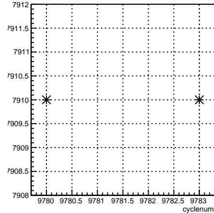
run:cyclenum {run == 7910}
