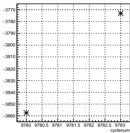
usr_coil6:cyclenum {run == 7910}
