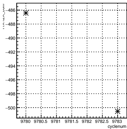
11X12X_coil7:cyclenum {run == 7910}
