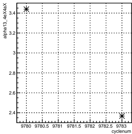
alpha13_4eX4aX:cyclenum {run == 7910}
