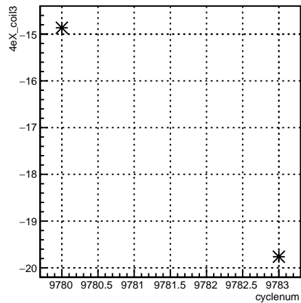
4eX_coil3:cyclenum {run == 7910}
