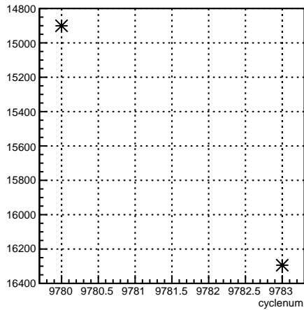
usr_coil1:cyclenum {run == 7910}
