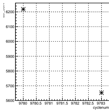
usr_coil4:cyclenum {run == 7910}
