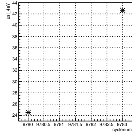
usl_4eY:cyclenum {run == 7910}
