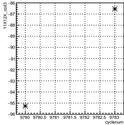
11X12X_coil3:cyclenum {run == 7910}
