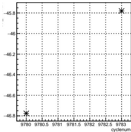
usl_11X12X:cyclenum {run == 7910}
