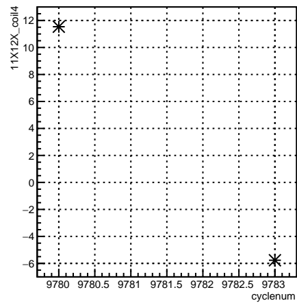
11X12X_coil4:cyclenum {run == 7910}
