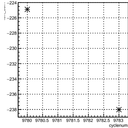
4eX_coil1:cyclenum {run == 7910}
