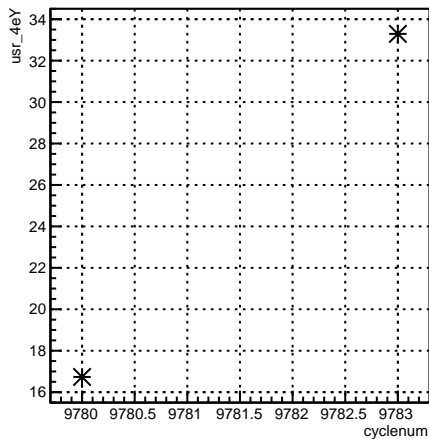
usr_4eY:cyclenum {run == 7910}
