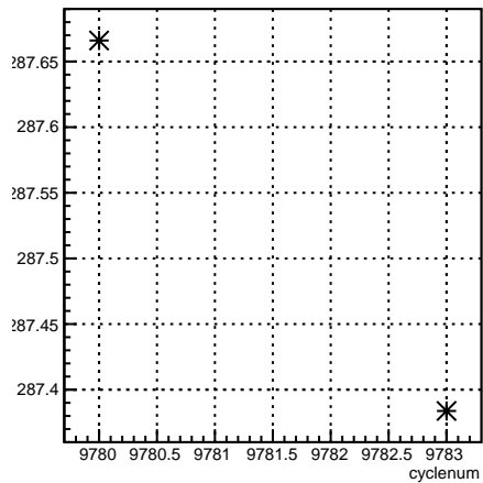
4eY_coil4:cyclenum {run == 7910}
