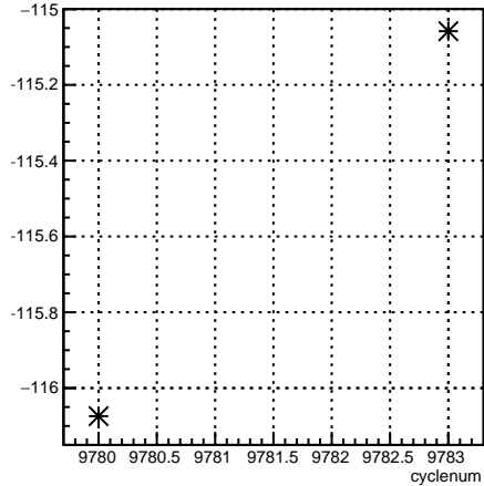
4eY_coil6:cyclenum {run == 7910}
