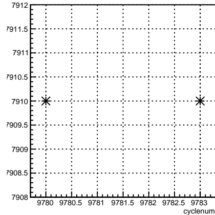
run:cyclenum {run == 7910}
