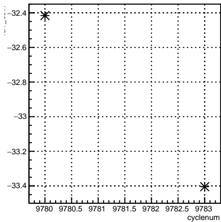
4eY_coil7:cyclenum {run == 7910}
