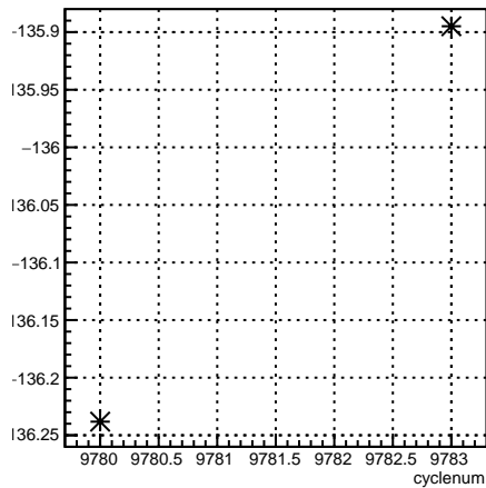
usr_4eY:cyclenum {run == 7910}
