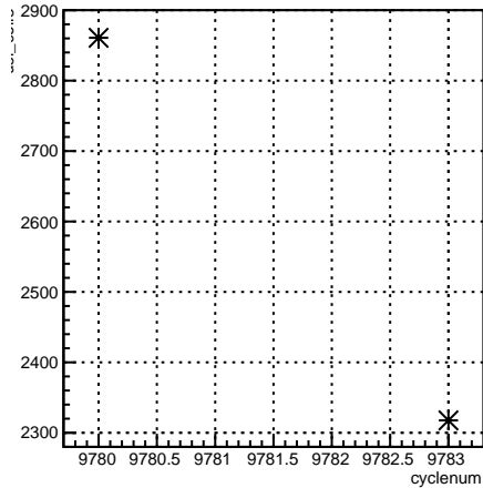
usl_coil7:cyclenum {run == 7910}
