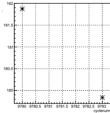
usr_4eX:cyclenum {run == 7910}
