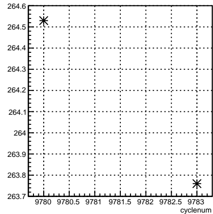
4eY_coil4:cyclenum {run == 7910}
