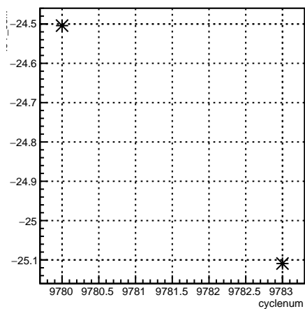
4eY_coil7:cyclenum {run == 7910}
