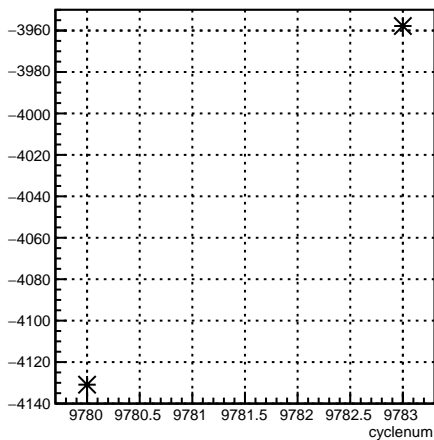
usl_coil6:cyclenum {run == 7910}
