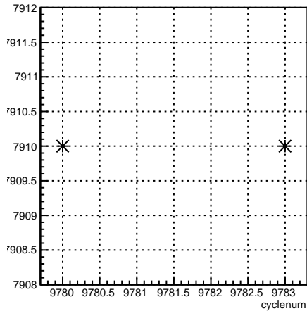
run:cyclenum {run == 7910}
