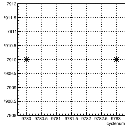
run:cyclenum {run == 7910}
