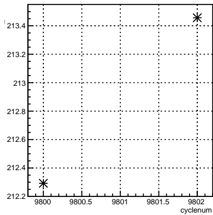
4eX_coil7:cyclenum {run == 7914}
