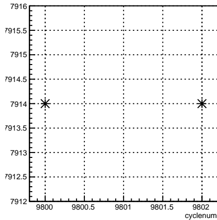
run:cyclenum {run == 7914}
