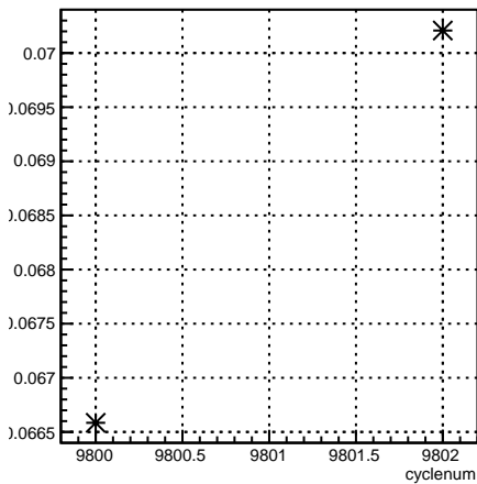
delta46_11X12X4eY:cyclenum {run == 7914}
