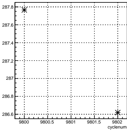
4eY_coil4:cyclenum {run == 7914}
