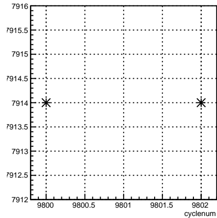
run:cyclenum {run == 7914}
