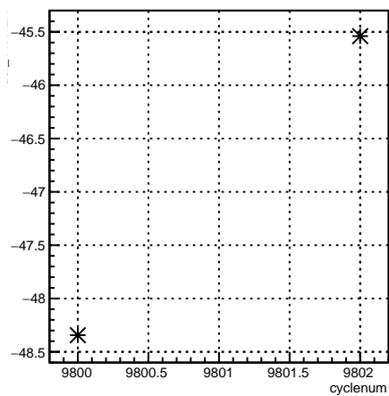
usr_11X12X:cyclenum {run == 7914}
