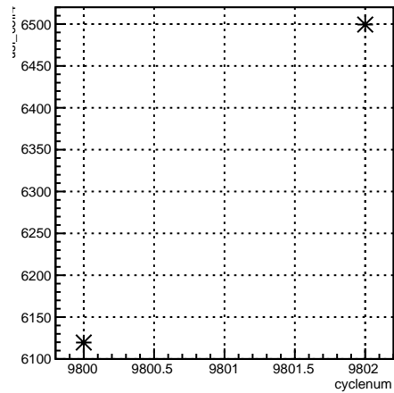
run:cyclenum {run == 7914}
