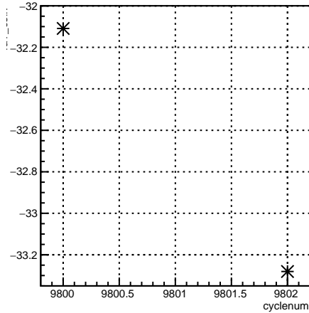
4eY_coil7:cyclenum {run == 7914}
