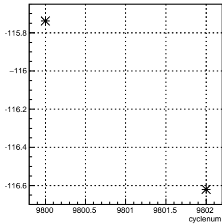
4eY_coil6:cyclenum {run == 7914}
