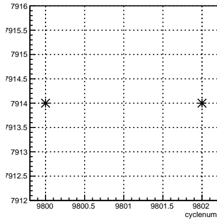
run:cyclenum {run == 7914}
