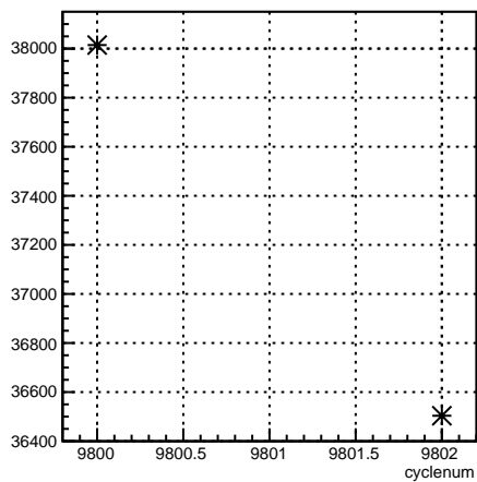
usr_coil7:cyclenum {run == 7914}
