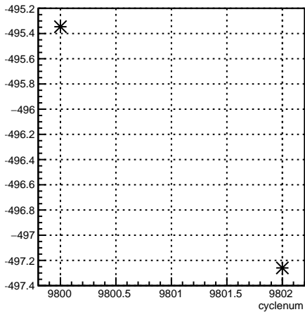
11X12X_coil7:cyclenum {run == 7914}
