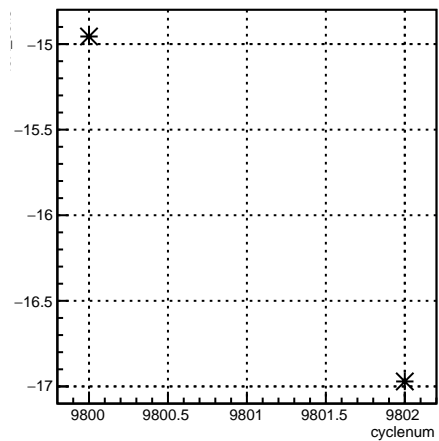
4eX_coil3:cyclenum {run == 7914}
