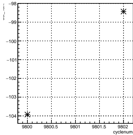
usl_4aX:cyclenum {run == 7914}
