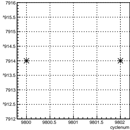
run:cyclenum {run == 7914}
