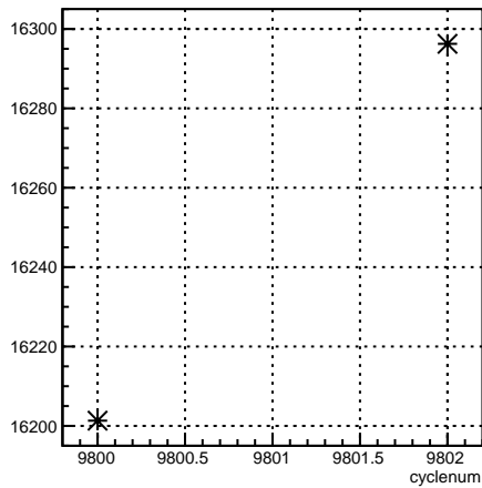
usl_coil6:cyclenum {run == 7914}
