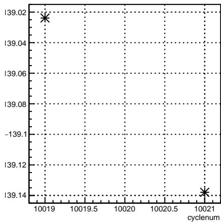
4eY_coil6:cyclenum {run == 7962}
