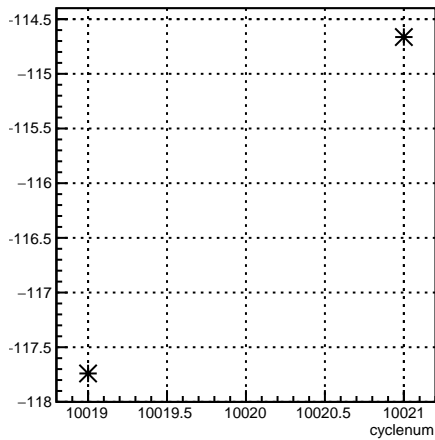
4eX_coil1:cyclenum {run == 7962}
