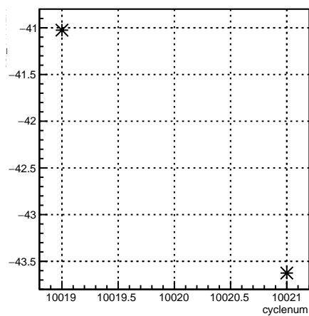
usr_11X12X:cyclenum {run == 7962}
