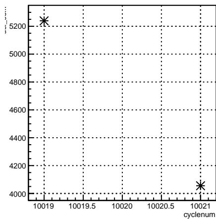
usl_coil7:cyclenum {run == 7962}
