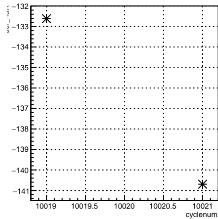
usr_4aX:cyclenum {run == 7962}
