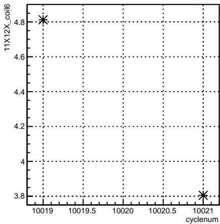
11X12X_coil6:cyclenum {run == 7962}
