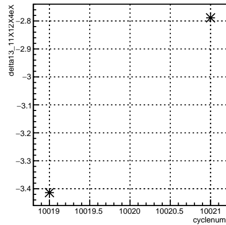
segment:cyclenum {run == 7962}
