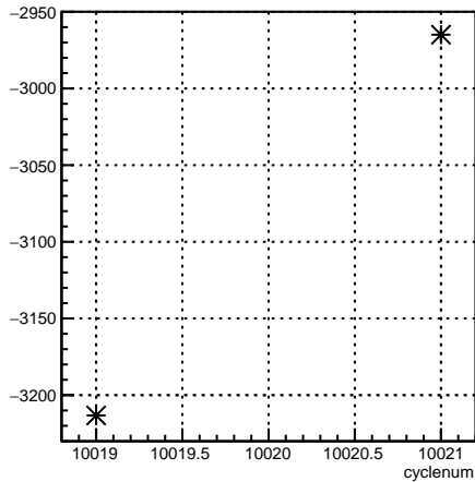
usl_coil6:cyclenum {run == 7962}
