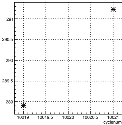
4eY_coil4:cyclenum {run == 7962}
