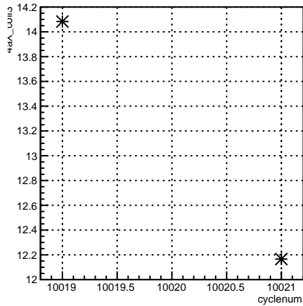
4eX_coil3:cyclenum {run == 7962}
