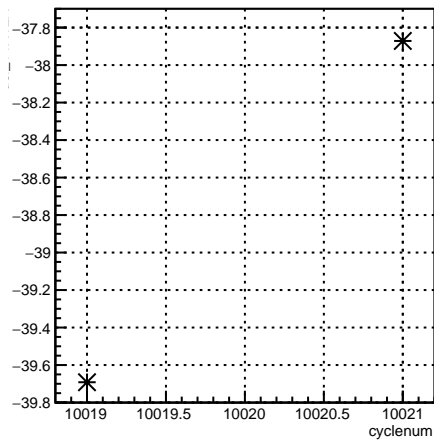
usl_11X12X:cyclenum {run == 7962}
