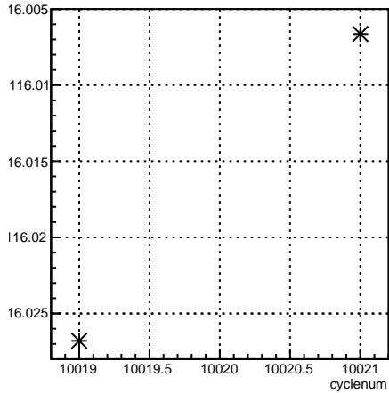
4aY_coil6:cyclenum {run == 7962}
