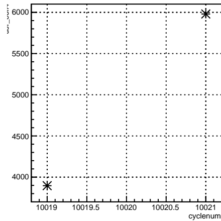
run:cyclenum {run == 7962}
