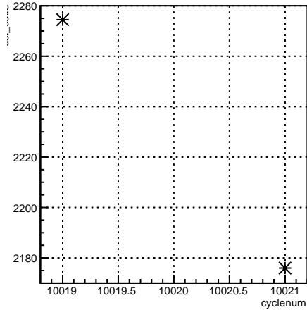
usl_coil7:cyclenum {run == 7962}
