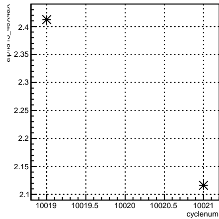
alpha13_4eX4aX:cyclenum {run == 7962}
