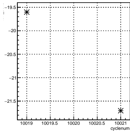
4eX_coil3:cyclenum {run == 7962}
