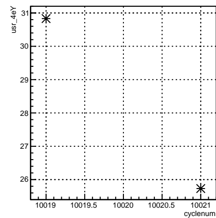
usr_4eY:cyclenum {run == 7962}
