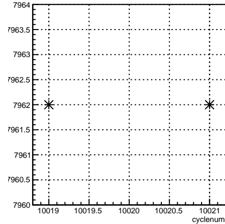
run:cyclenum {run == 7962}
