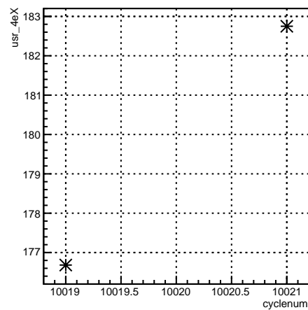
usr_4eX:cyclenum {run == 7962}
