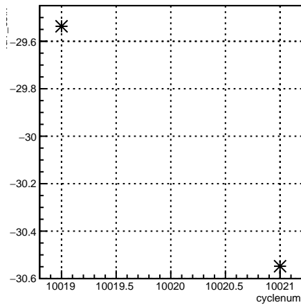
4eY_coil7:cyclenum {run == 7962}
