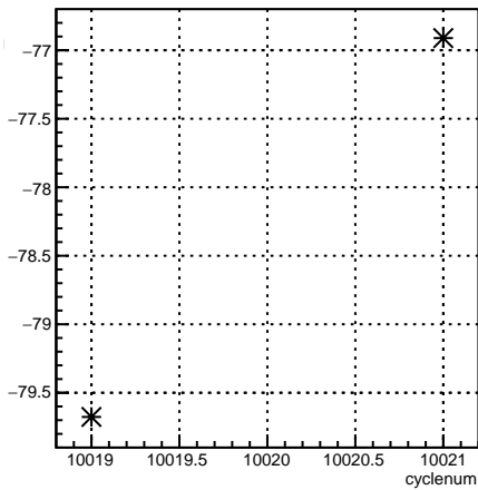
usl_4eY:cyclenum {run == 7962}
