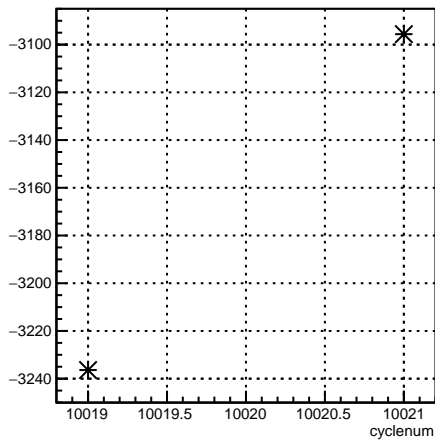
usr_coil6:cyclenum {run == 7962}
