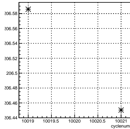
4eX_coil7:cyclenum {run == 7962}
