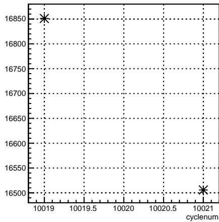
usl_coil6:cyclenum {run == 7962}
