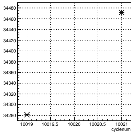
usr_coil7:cyclenum {run == 7962}
