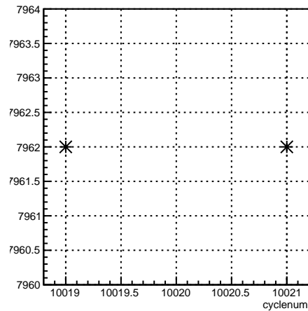
run:cyclenum {run == 7962}
