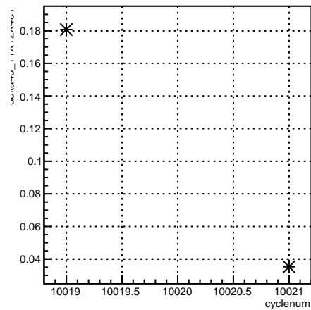
delta46_11X12X4eY:cyclenum {run == 7962}
