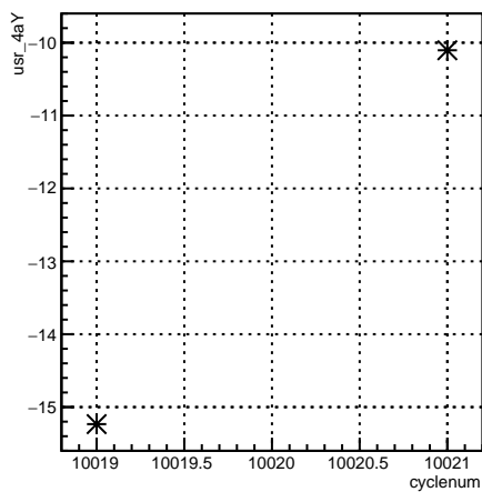
usr_4aY:cyclenum {run == 7962}
