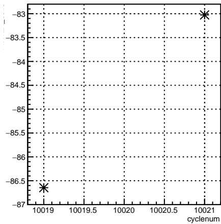
11X12X_coil7:cyclenum {run == 7962}
