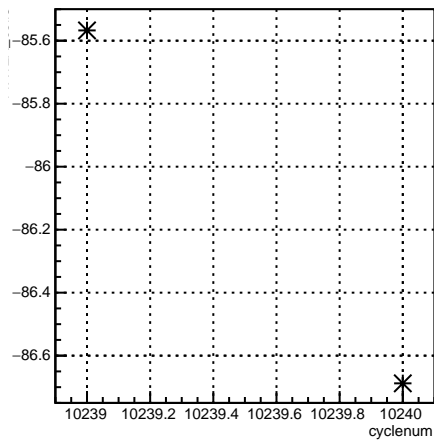
11X12X_coil3:cyclenum {run == 8037}
