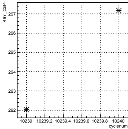
4eY_coil4:cyclenum {run == 8037}
