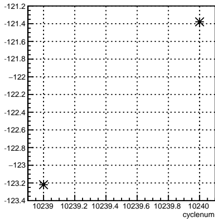
usr_4aX:cyclenum {run == 8037}
