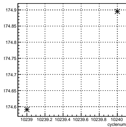
usr_4eX:cyclenum {run == 8037}
