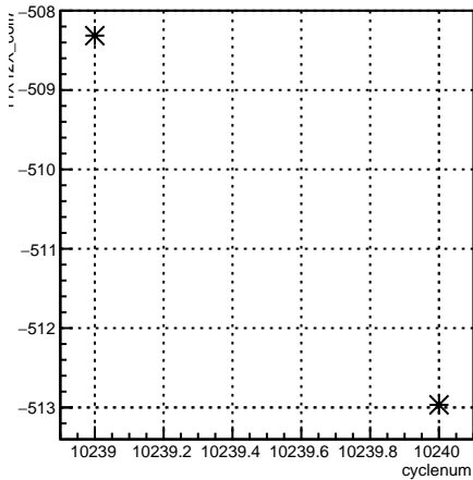
11X12X_coil7:cyclenum {run == 8037}
