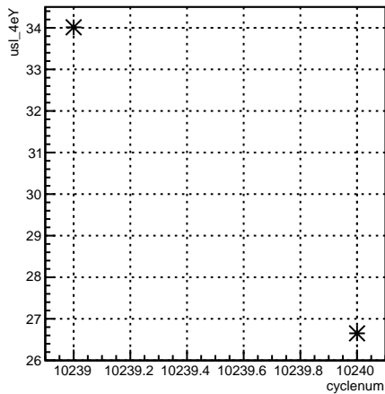
usl_4eY:cyclenum {run == 8037}
