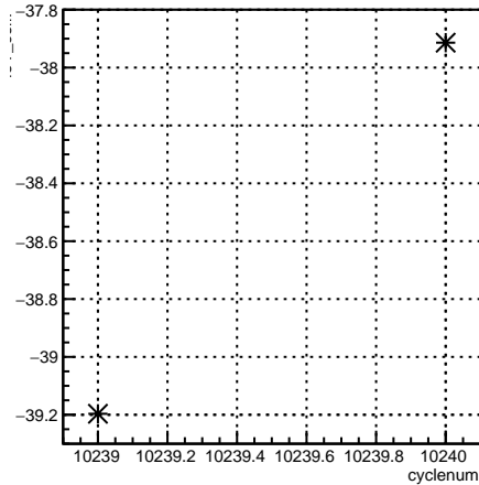
4eY_coil7:cyclenum {run == 8037}
