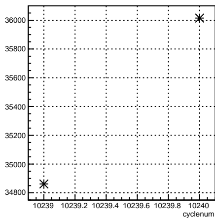
usr_coil7:cyclenum {run == 8037}
