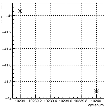
usr_11X12X:cyclenum {run == 8037}
