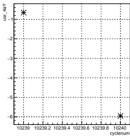
usr_4aY:cyclenum {run == 8037}
