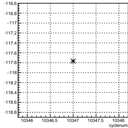
usr_4aX:cyclenum {run == 8105}
