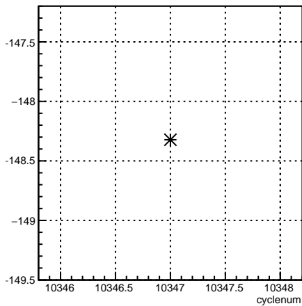
4eY_coil6:cyclenum {run == 8105}
