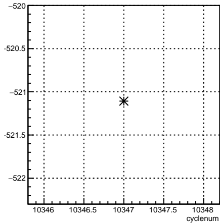
11X12X_coil7:cyclenum {run == 8105}
