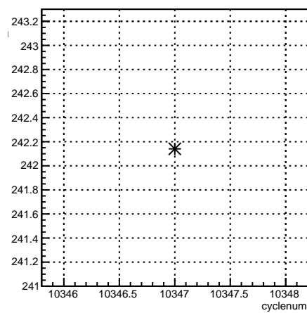
4aX_coil7:cyclenum {run == 8105}
