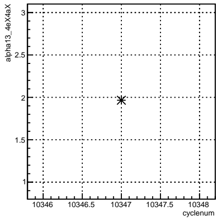
alpha13_4eX4aX:cyclenum {run == 8105}
