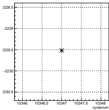
usr_coil3:cyclenum {run == 8105}
