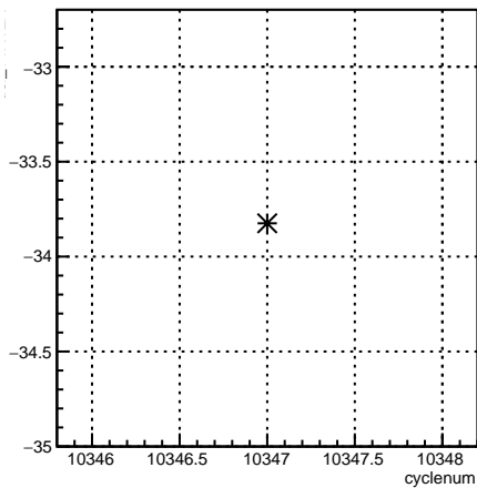
usl_11X12X:cyclenum {run == 8105}
