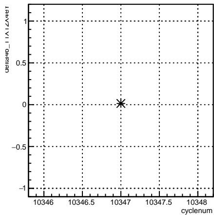
delta46_11X12X4eY:cyclenum {run == 8105}
