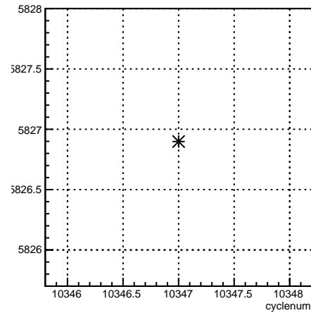
usr_coil4:cyclenum {run == 8105}
