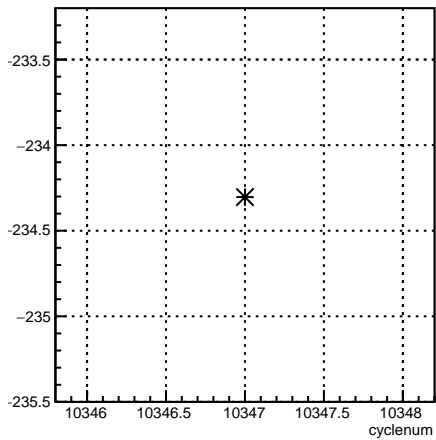
11X12X_coil6:cyclenum {run == 8105}
