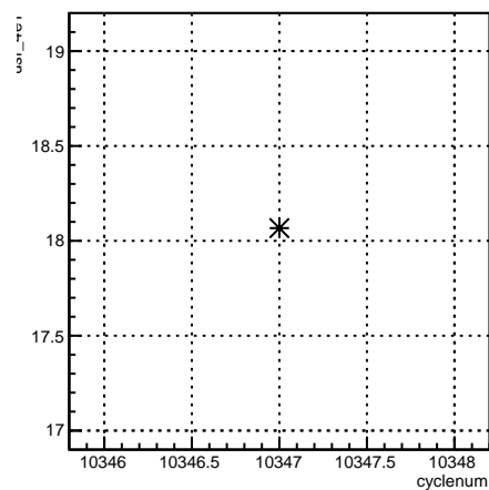
usr_4eY:cyclenum {run == 8105}
