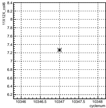
11X12X_coil6:cyclenum {run == 8105}
