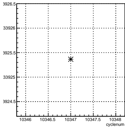
usr_coil7:cyclenum {run == 8105}
