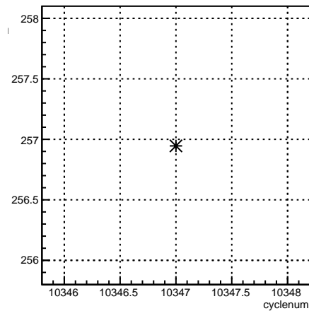
4eX_coil7:cyclenum {run == 8105}
