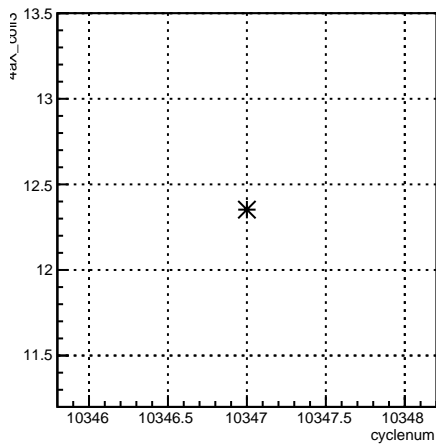
4aX_coil3:cyclenum {run == 8105}
