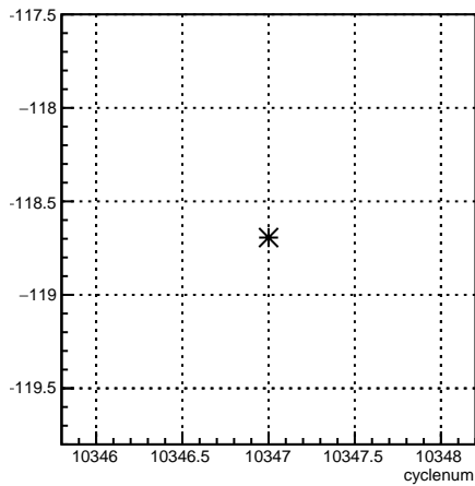
4aX_coil1:cyclenum {run == 8105}
