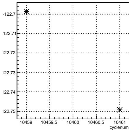
4eY_coil6:cyclenum {run == 8133}
