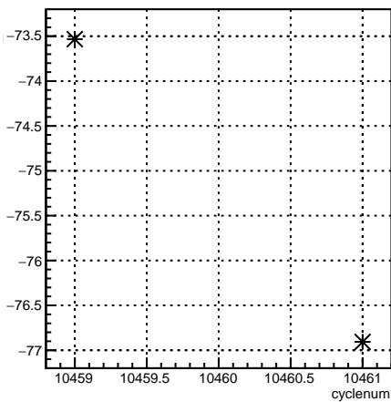
usl_4aX:cyclenum {run == 8133}
