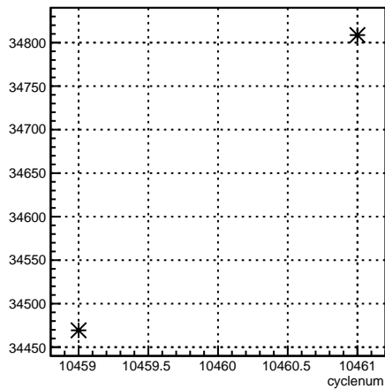
usr_coil7:cyclenum {run == 8133}
