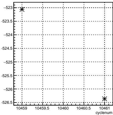
11X12X_coil7:cyclenum {run == 8133}
