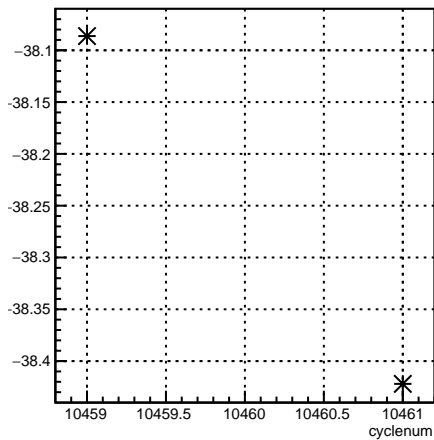
usl_11X12X:cyclenum {run == 8133}
