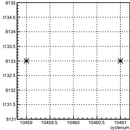
run:cyclenum {run == 8133}
