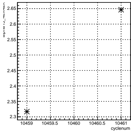
alpha13_4eX4aX:cyclenum {run == 8133}
