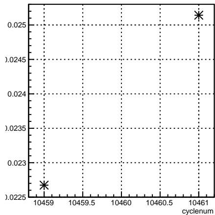
delta46_11X12X4eY:cyclenum {run == 8133}
