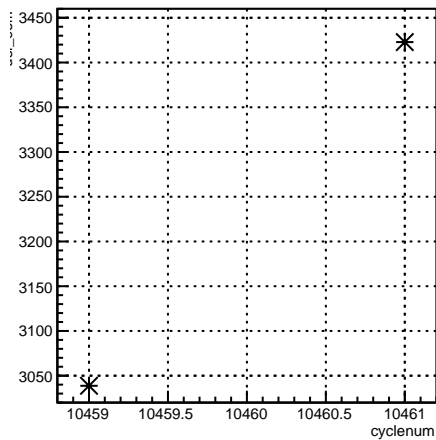
usl_coil7:cyclenum {run == 8133}
