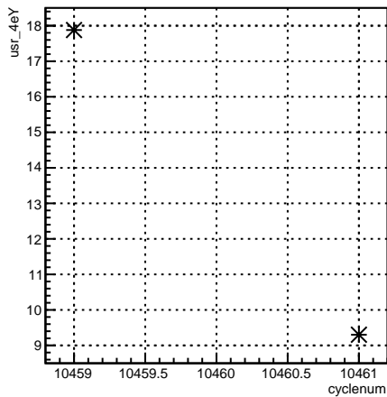
usr_4eY:cyclenum {run == 8133}
