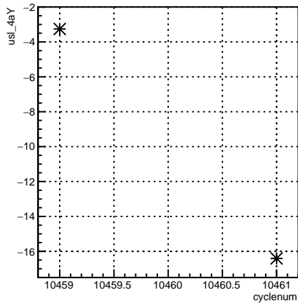
usl_4aY:cyclenum {run == 8133}
