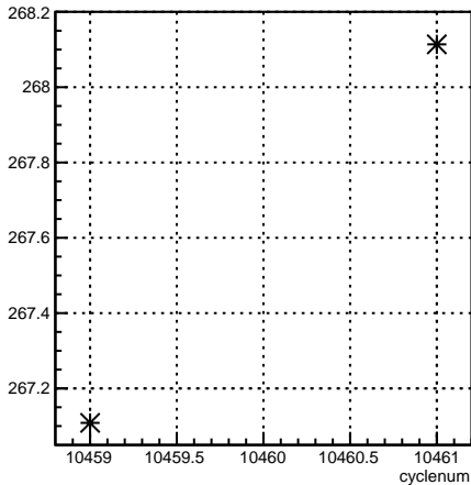
4eY_coil4:cyclenum {run == 8133}
