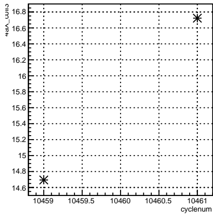
4eX_coil3:cyclenum {run == 8133}
