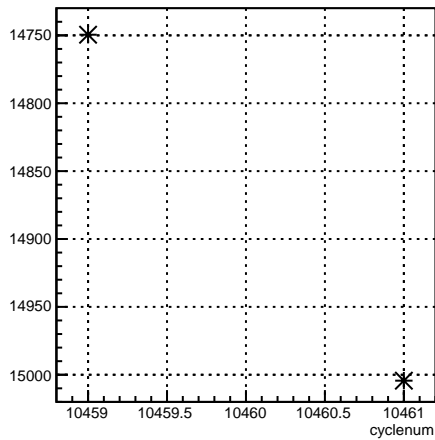
usr_coil6:cyclenum {run == 8133}
