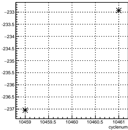
11X12X_coil6:cyclenum {run == 8133}
