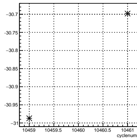
4eY_coil7:cyclenum {run == 8133}
