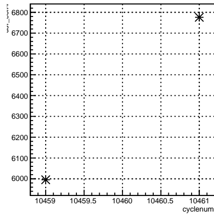
run:cyclenum {run == 8133}
