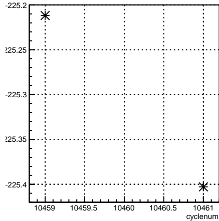
4eX_coil1:cyclenum {run == 8133}
