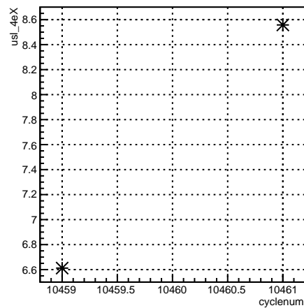
usl_4eX:cyclenum {run == 8133}
