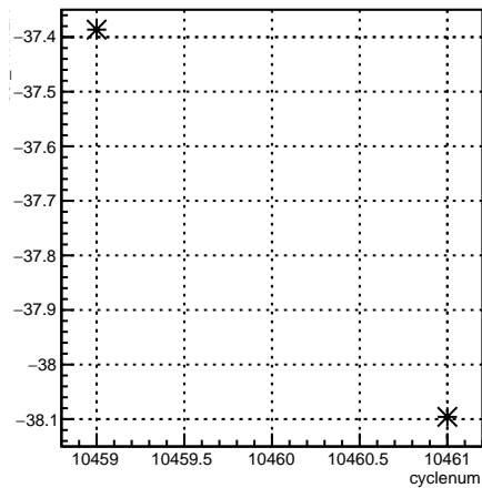
usr_11X12X:cyclenum {run == 8133}
