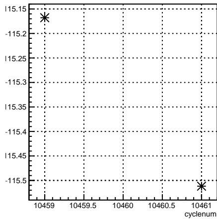
usr_4eY:cyclenum {run == 8133}
