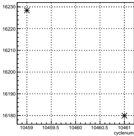
usl_coil6:cyclenum {run == 8133}
