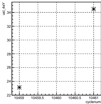
usl_4eY:cyclenum {run == 8133}
