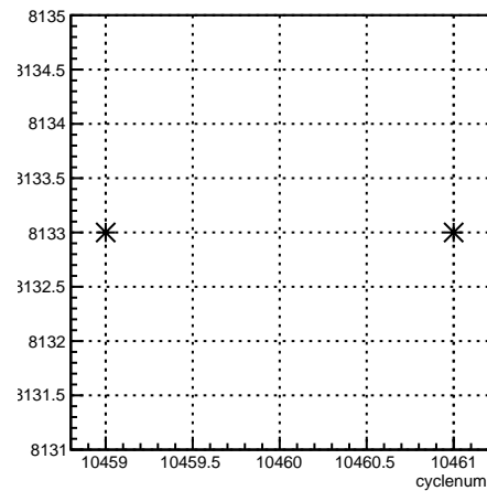
run:cyclenum {run == 8133}
