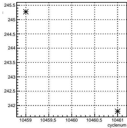
4eX_coil7:cyclenum {run == 8133}
