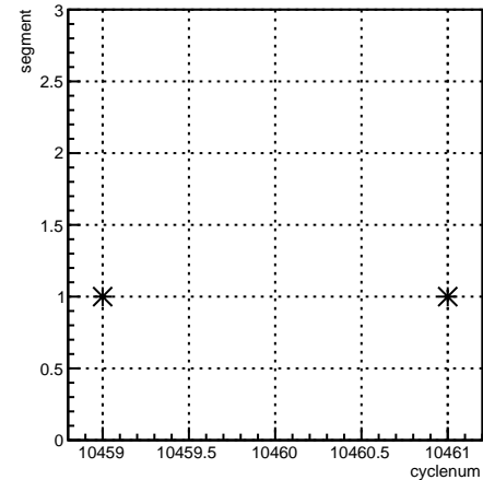
segment:cyclenum {run == 8133}
