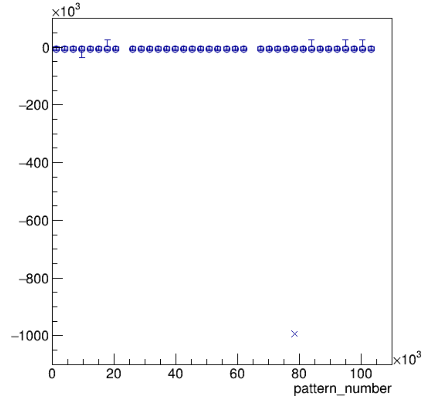
asym_atl1/ppm:pattern_number {ErrorFlag==0}
