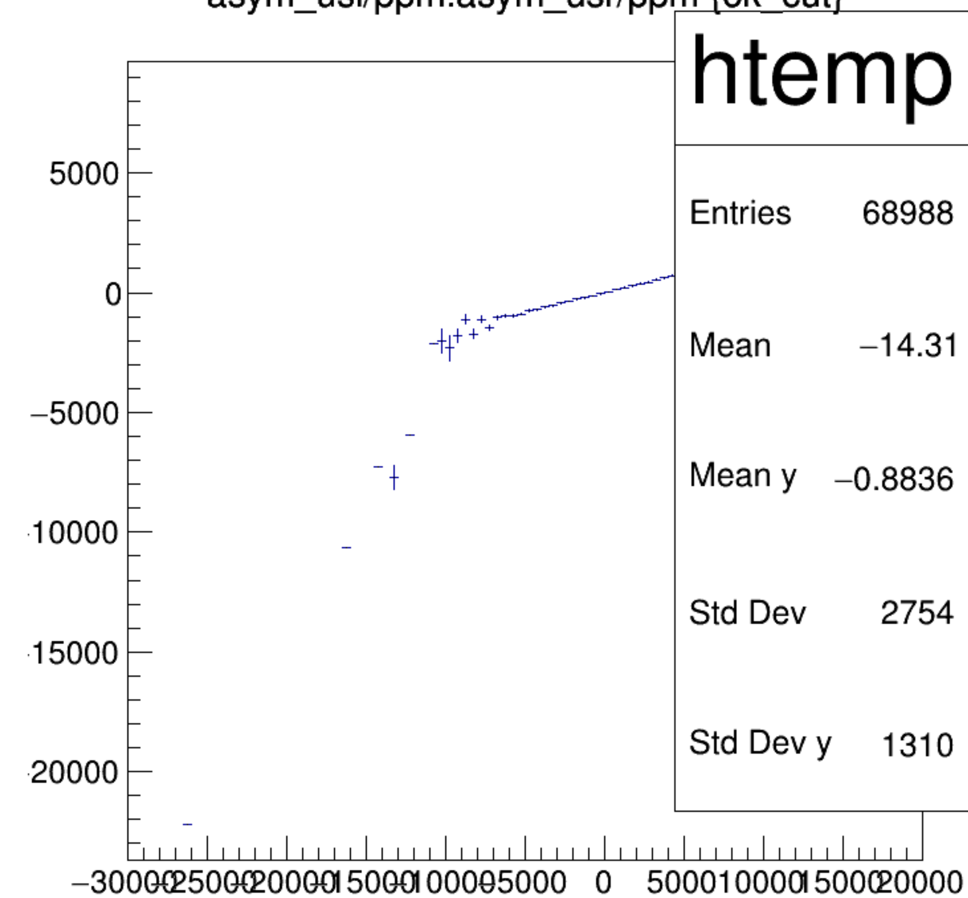
asym_usl/ppm:asym_usr/ppm {ok_cut}
