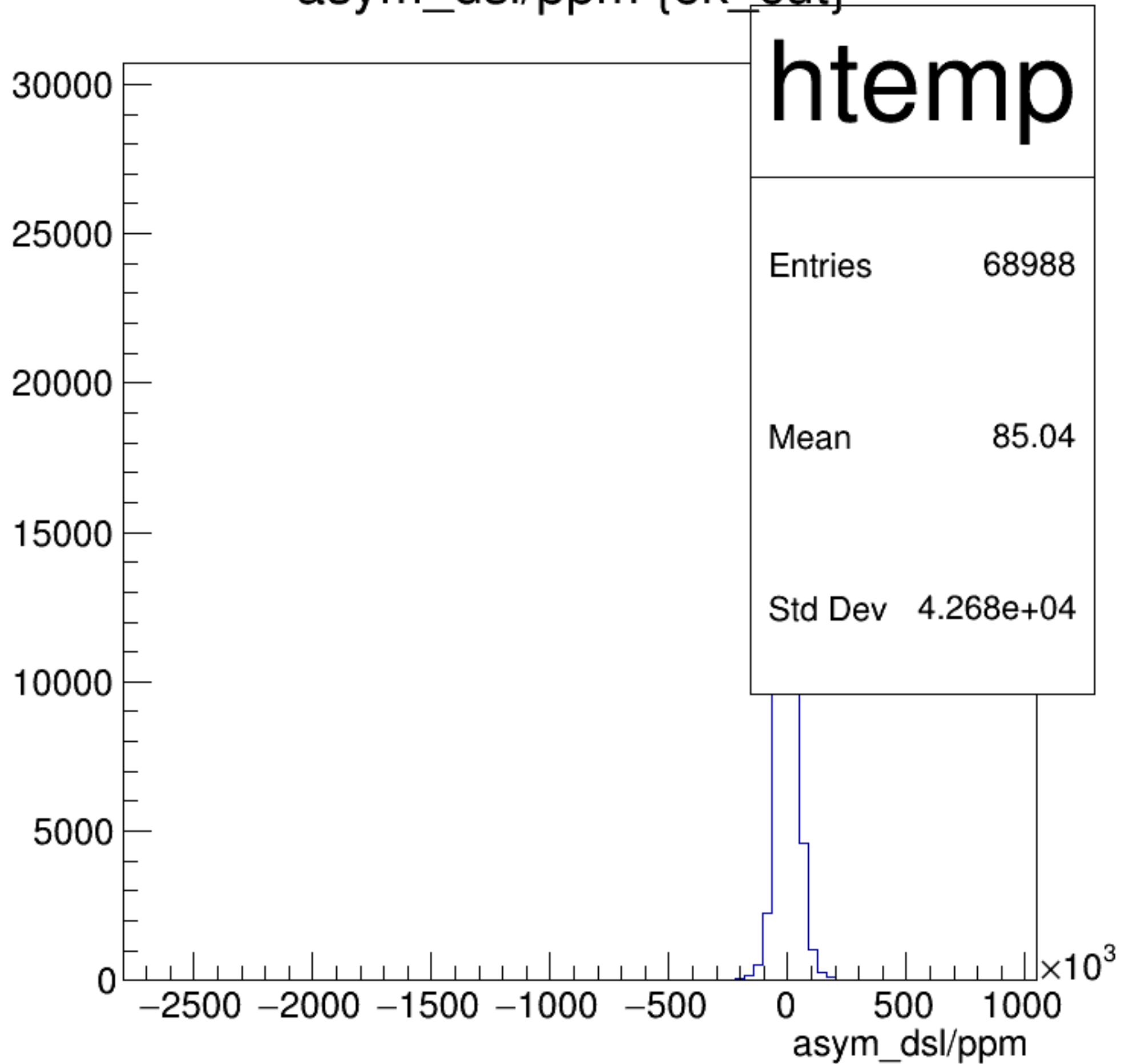
asym_dsl/ppm {ok_cut}
