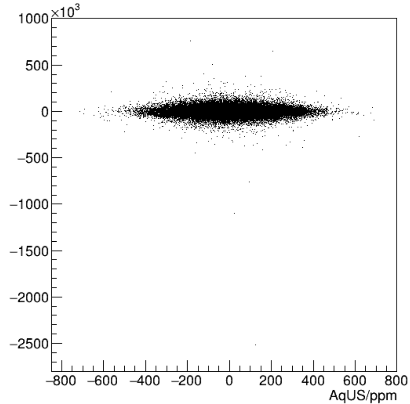
reg_asym_dsl/ppm:AqUS/ppm {ok_cut}
