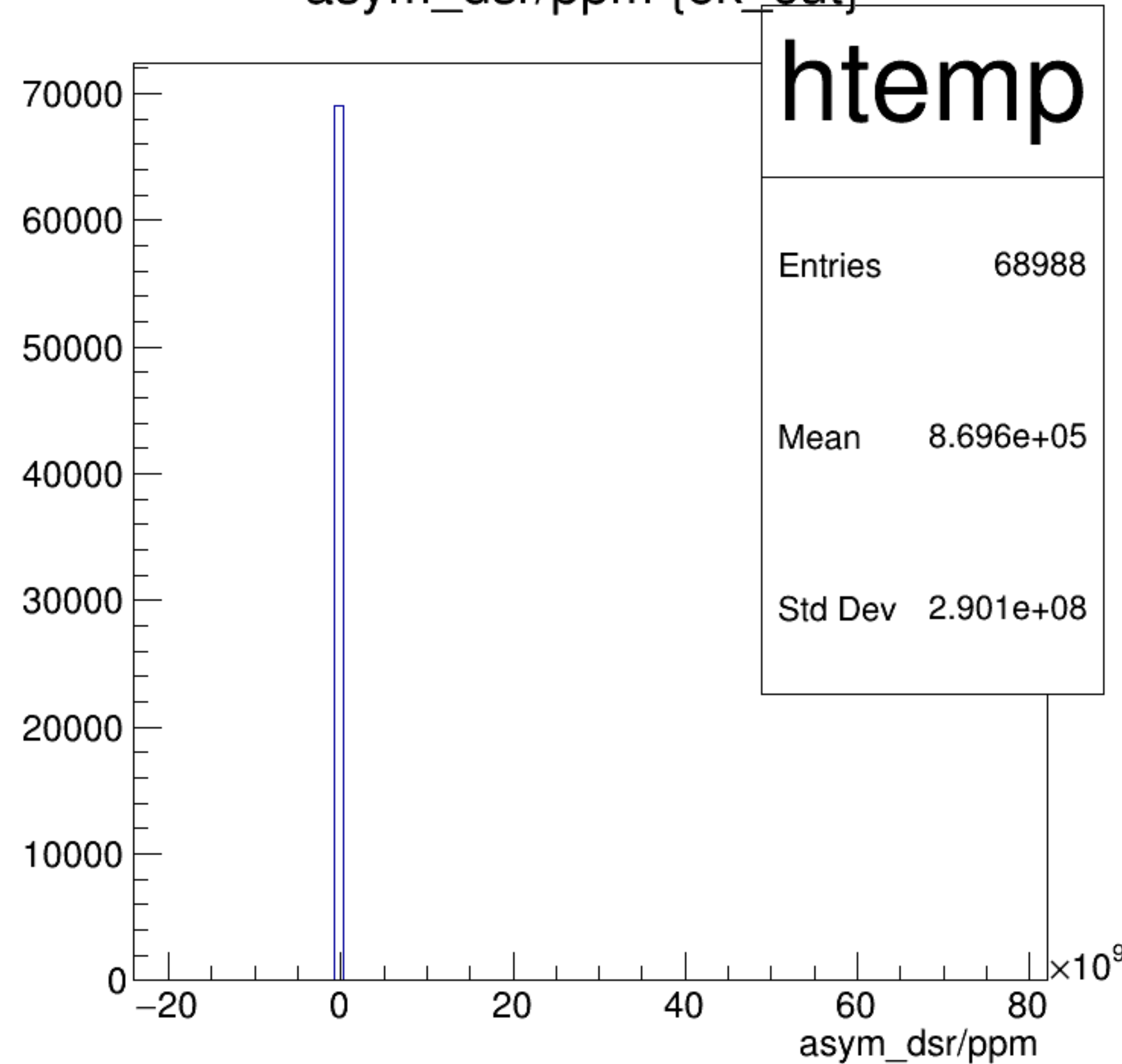
asym_dsr/ppm {ok_cut}
