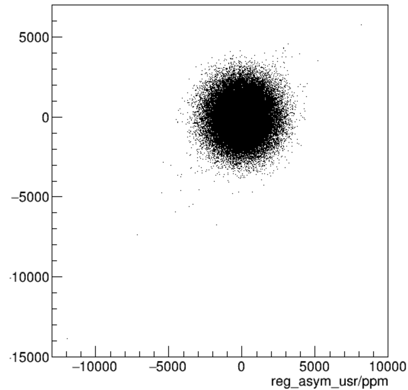
reg_asym_usl/ppm:reg_asym_usr/ppm {ok_cut}
