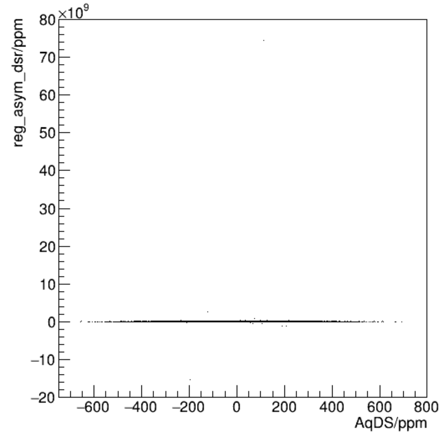
reg_asym_dsr/ppm:AqDS/ppm {ok_cut}
