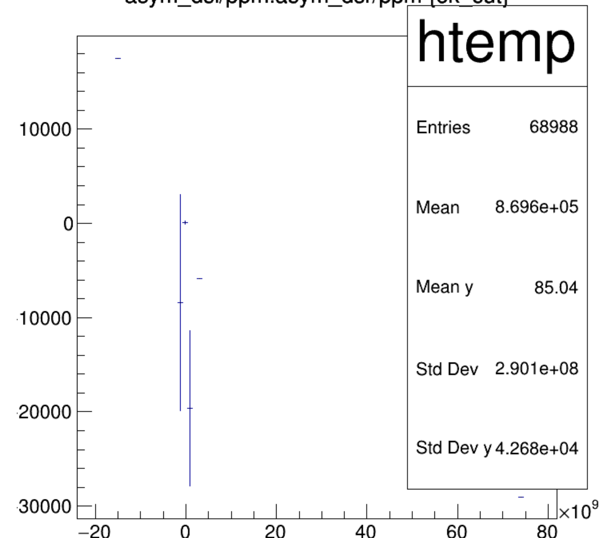
asym_dsl/ppm:asym_dsr/ppm {ok_cut}
