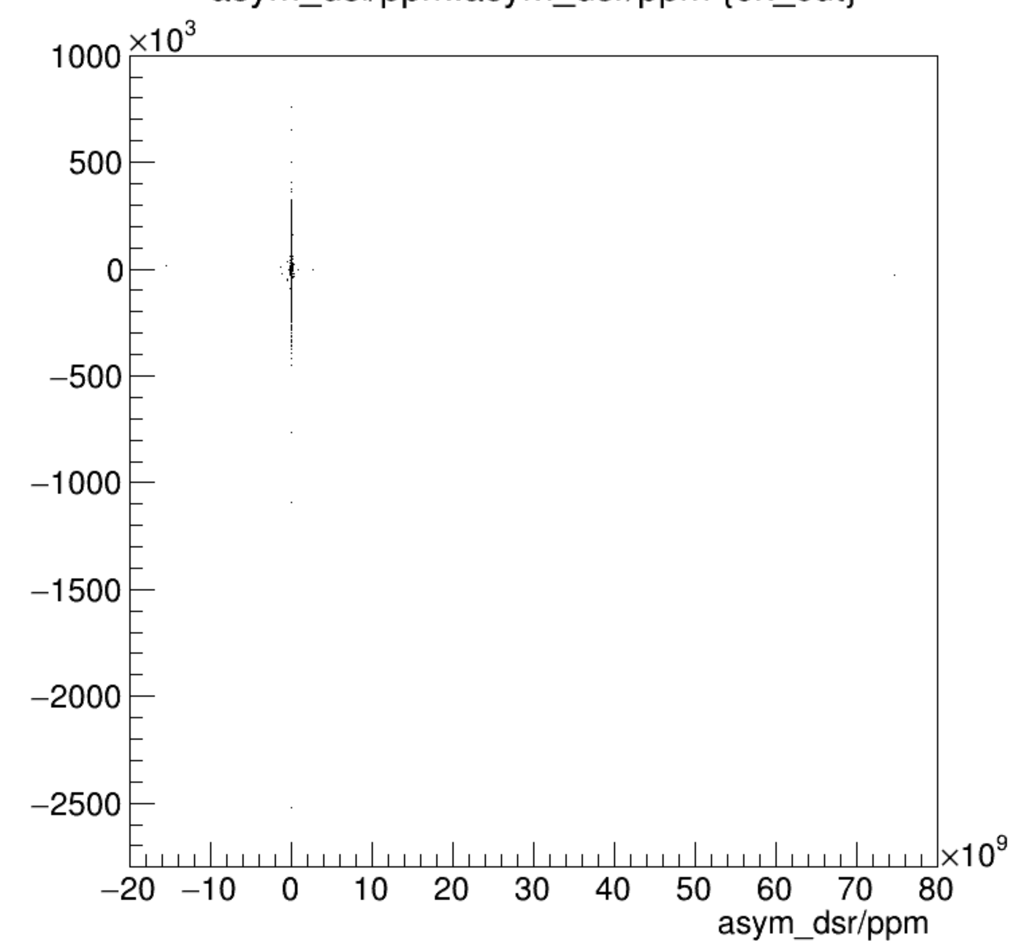
asym_dsl/ppm:asym_dsr/ppm {ok_cut}
