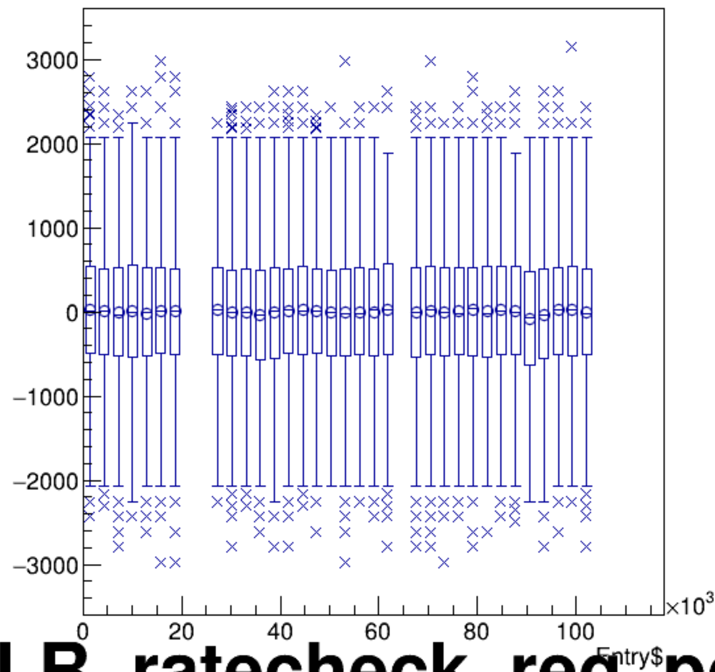
(reg_asym_usl/ppm-reg_asym_usr/ppm)/2:Entry$ {ok_cut}
