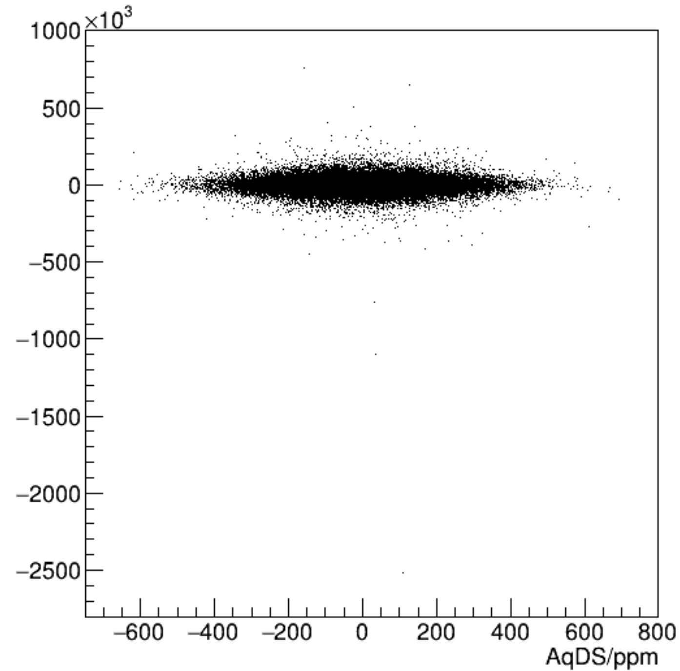
reg_asym_dsl/ppm:AqDS/ppm {ok_cut}
