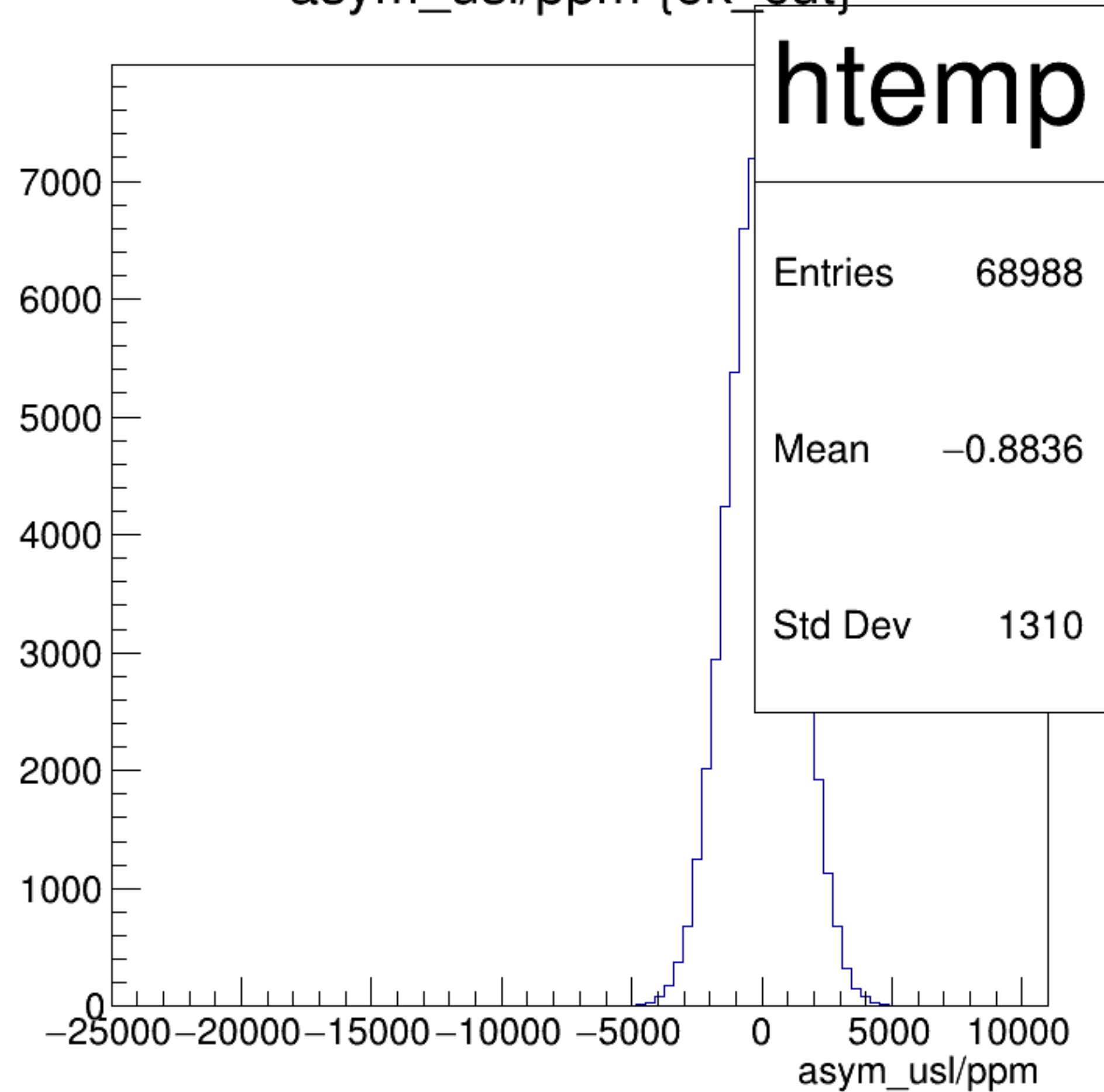
asym_usl/ppm {ok_cut}
