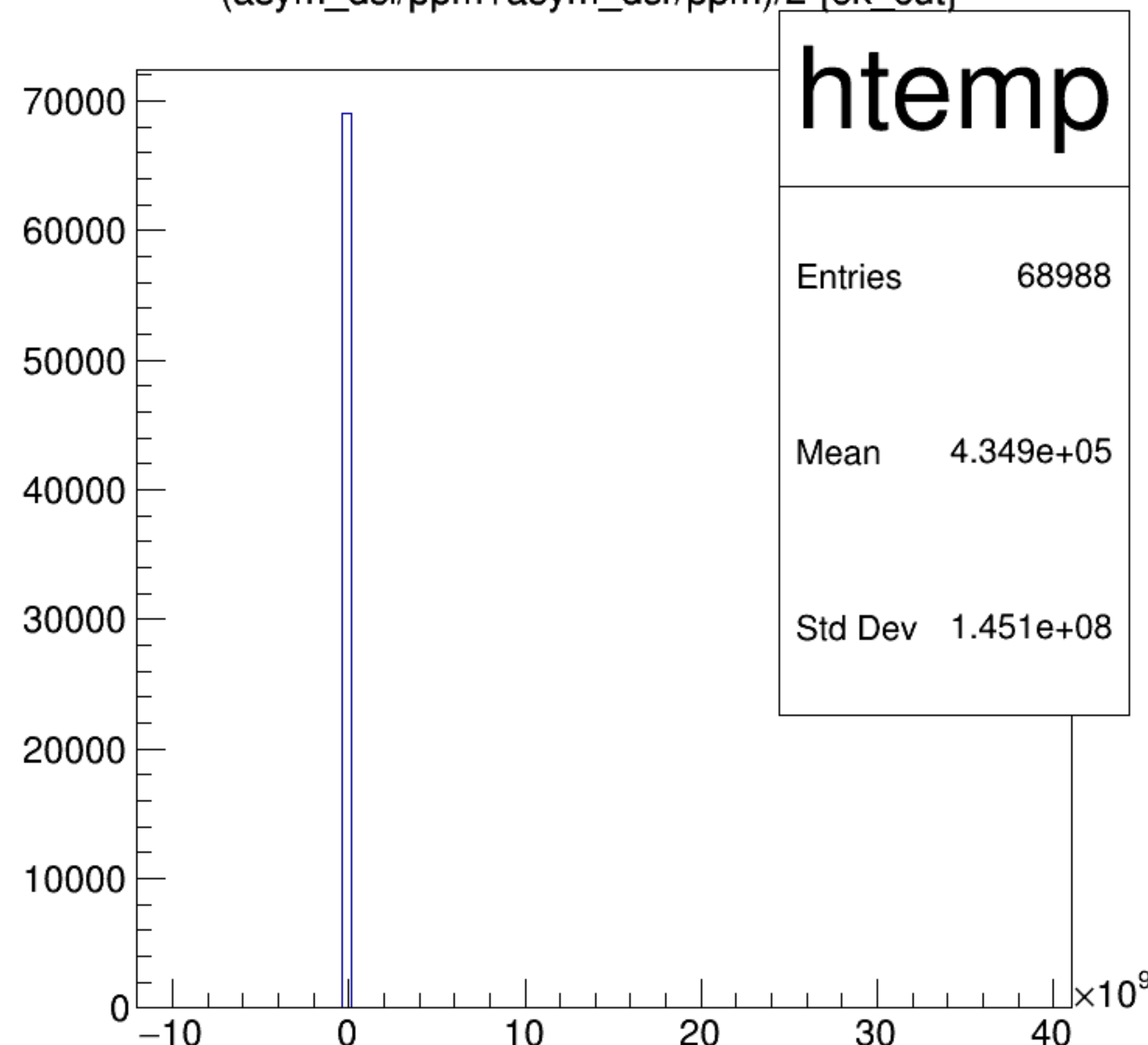
(asym_dsl/ppm+asym_dsr/ppm)/2 {ok_cut}
