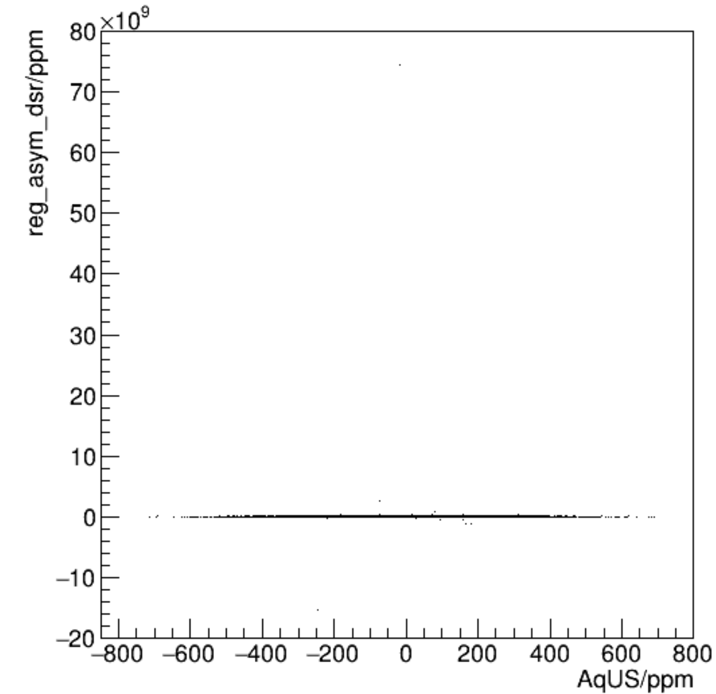
reg_asym_dsr/ppm:AqUS/ppm {ok_cut}
