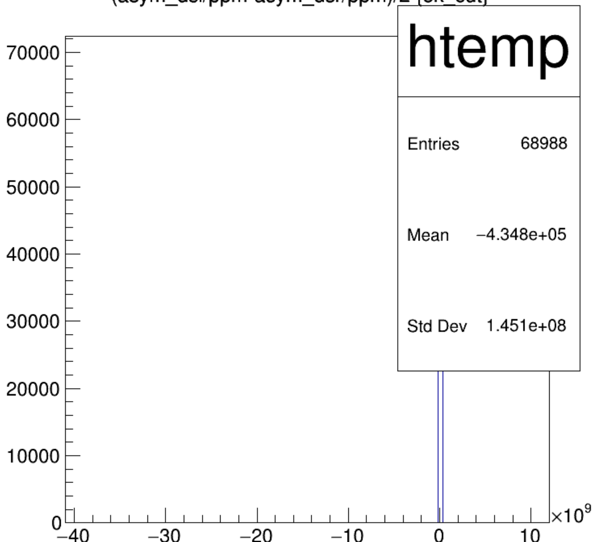
(asym_dsl/ppm-asym_dsr/ppm)/2 {ok_cut}
