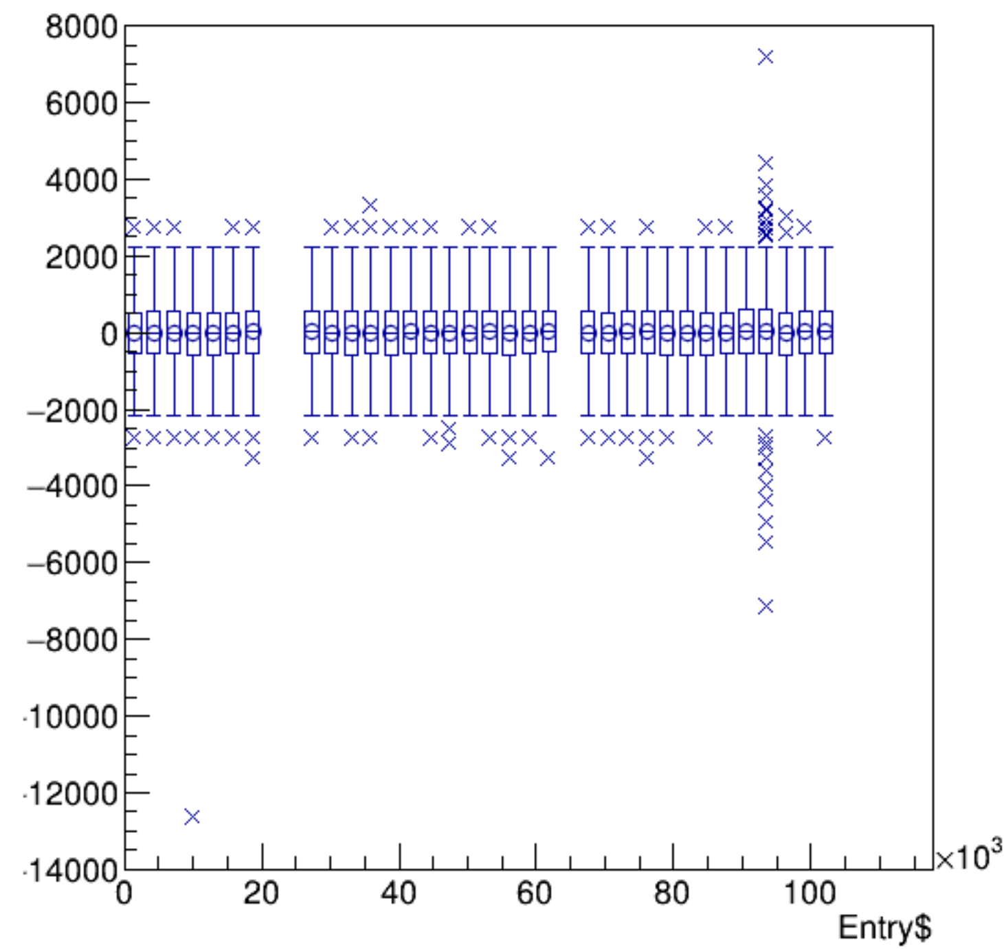
(reg_asym_usl/ppm+reg_asym_usr/ppm)/2:Entry$ {ok_cut}
