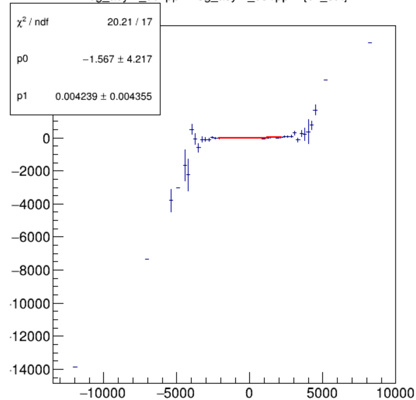
reg_asym_usl/ppm:reg_asym_usr/ppm {ok_cut}
