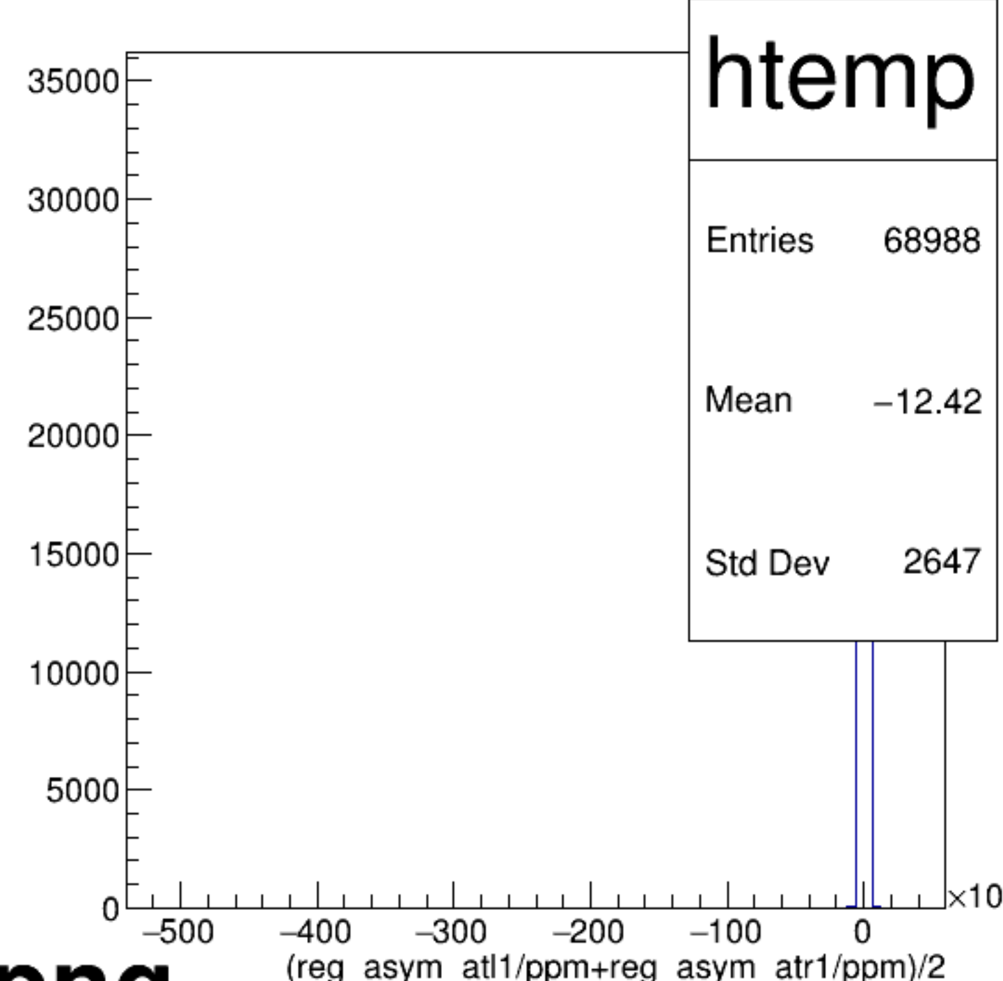
(reg_asym_atl1/ppm+reg_asym_atr1/ppm)/2 {ok_cut}
