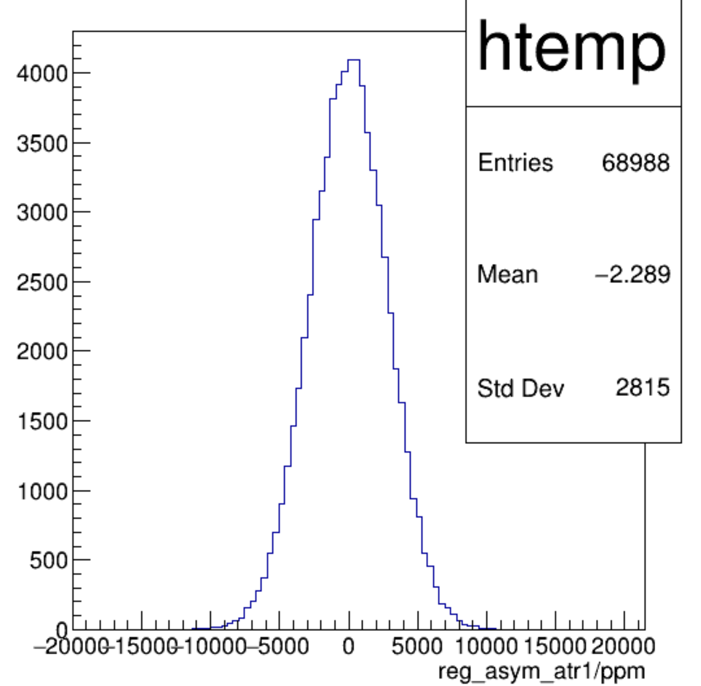
reg_asym_atr1/ppm {ok_cut}
