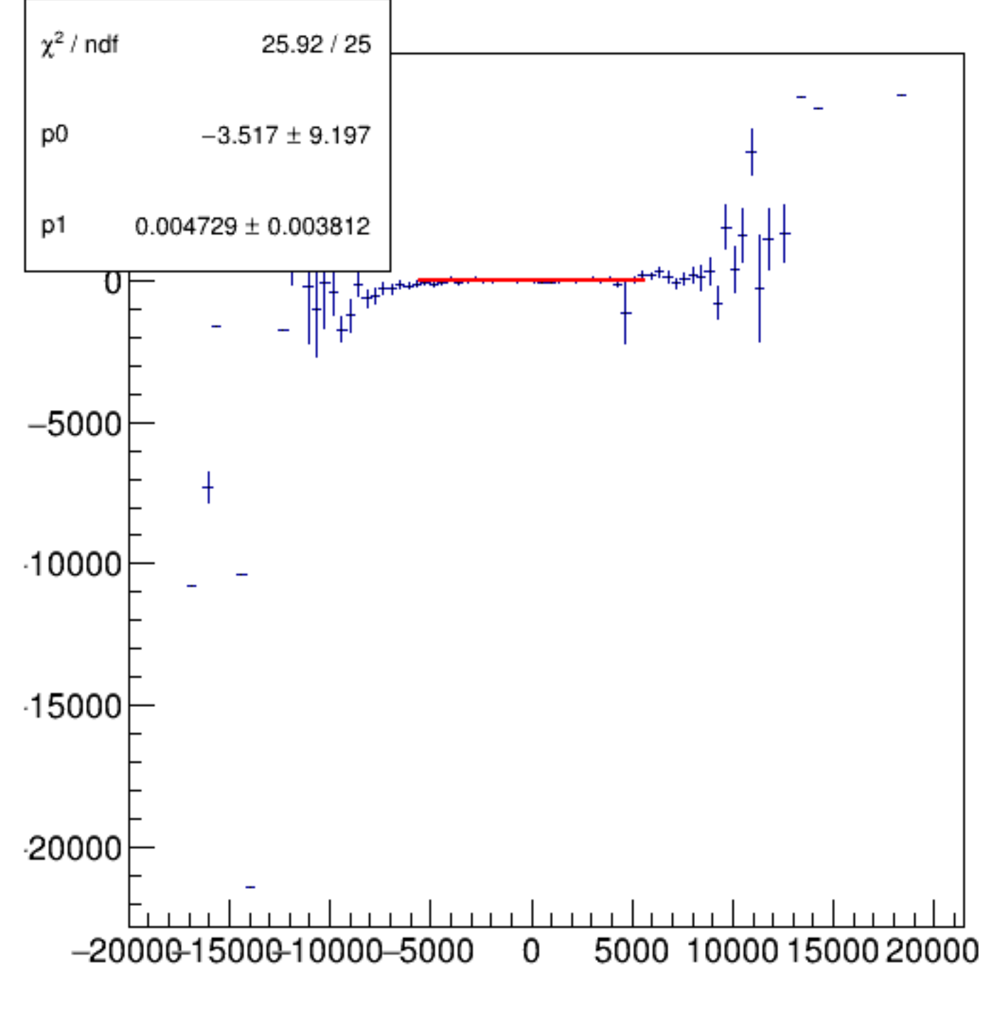
reg_asym_atl1/ppm:reg_asym_atr1/ppm {ok_cut}
