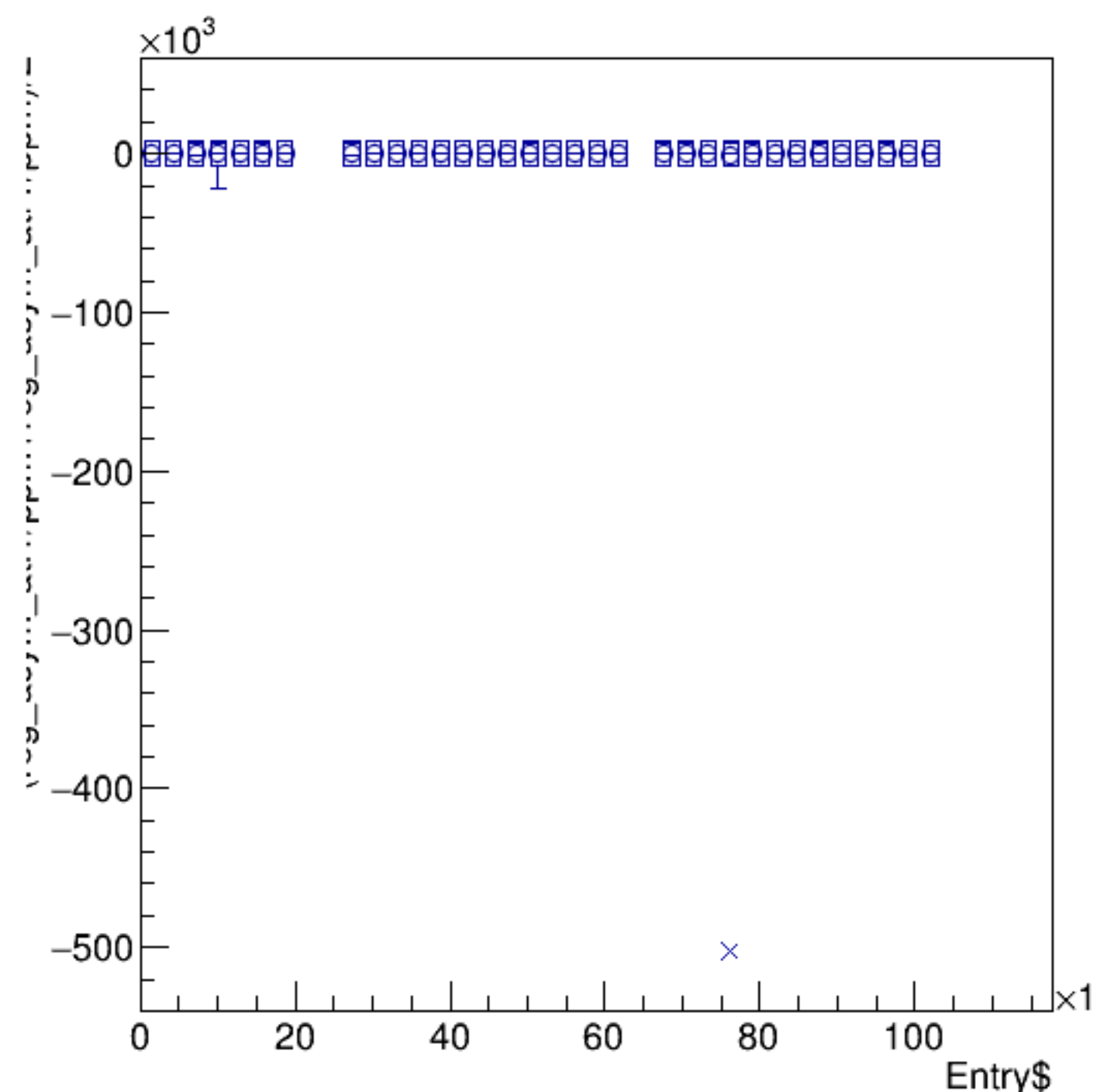
(reg_asym_atl1/ppm+reg_asym_atr1/ppm)/2:Entry$ {ok_cut}
