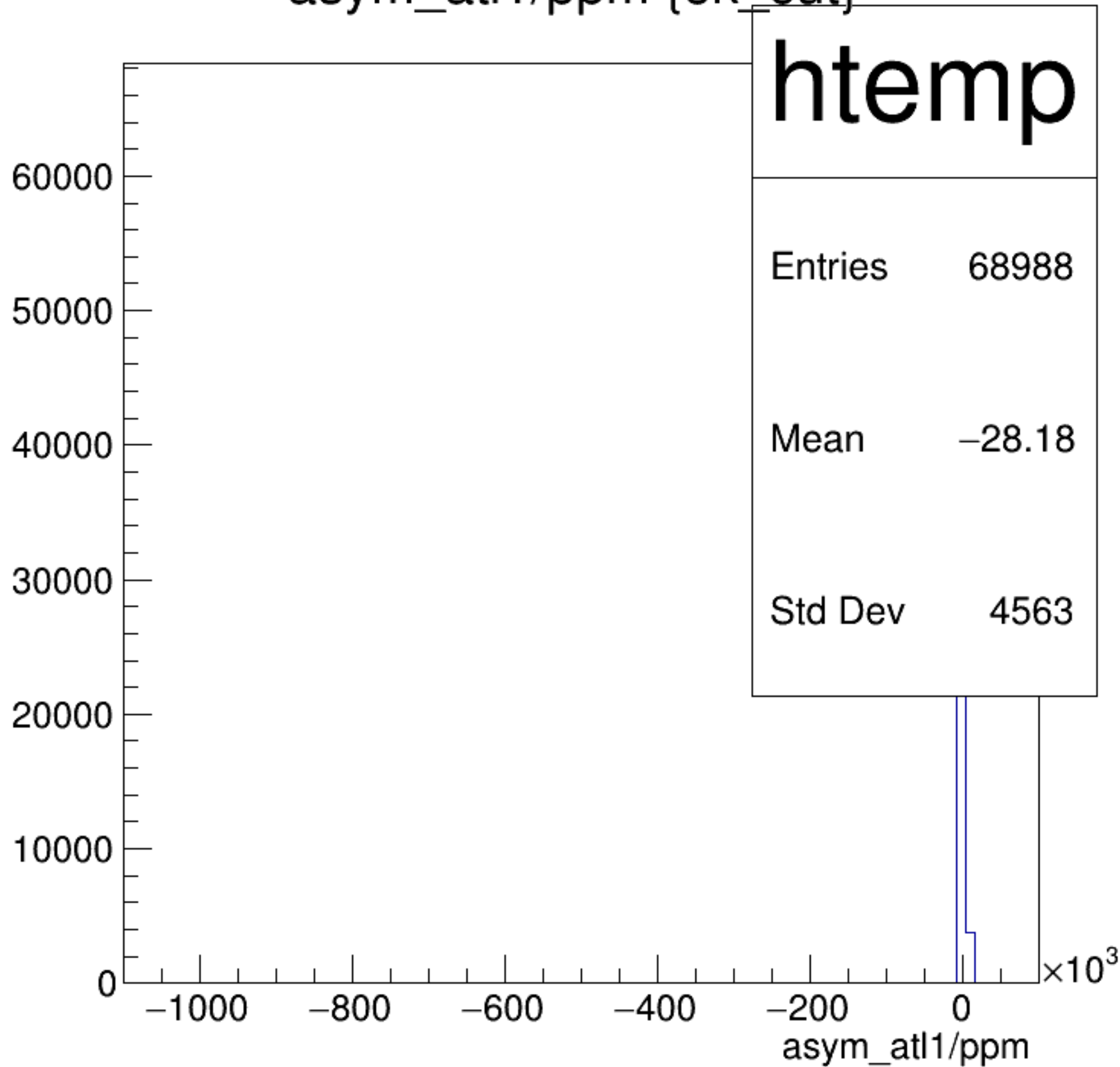
asym_atl1/ppm {ok_cut}
