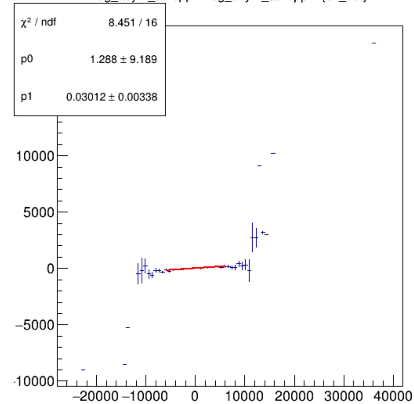
reg_asym_atl2/ppm:reg_asym_atr2/ppm {ok_cut}
