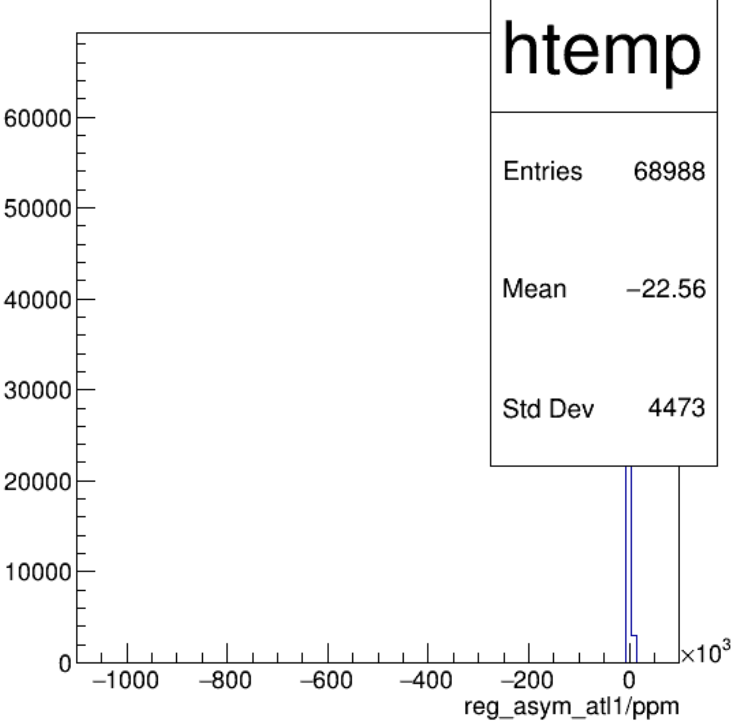
reg_asym_atl1/ppm {ok_cut}
