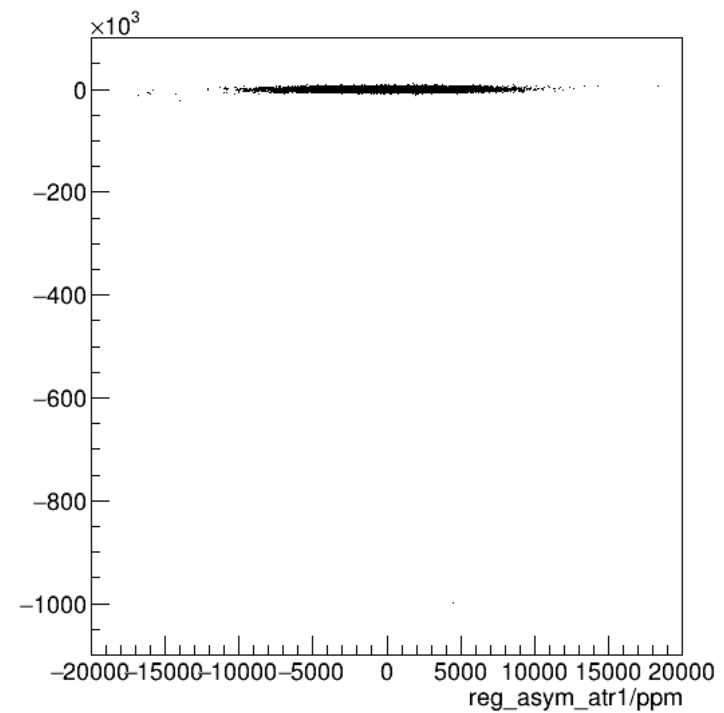
reg_asym_atl1/ppm:reg_asym_atr1/ppm {ok_cut}
