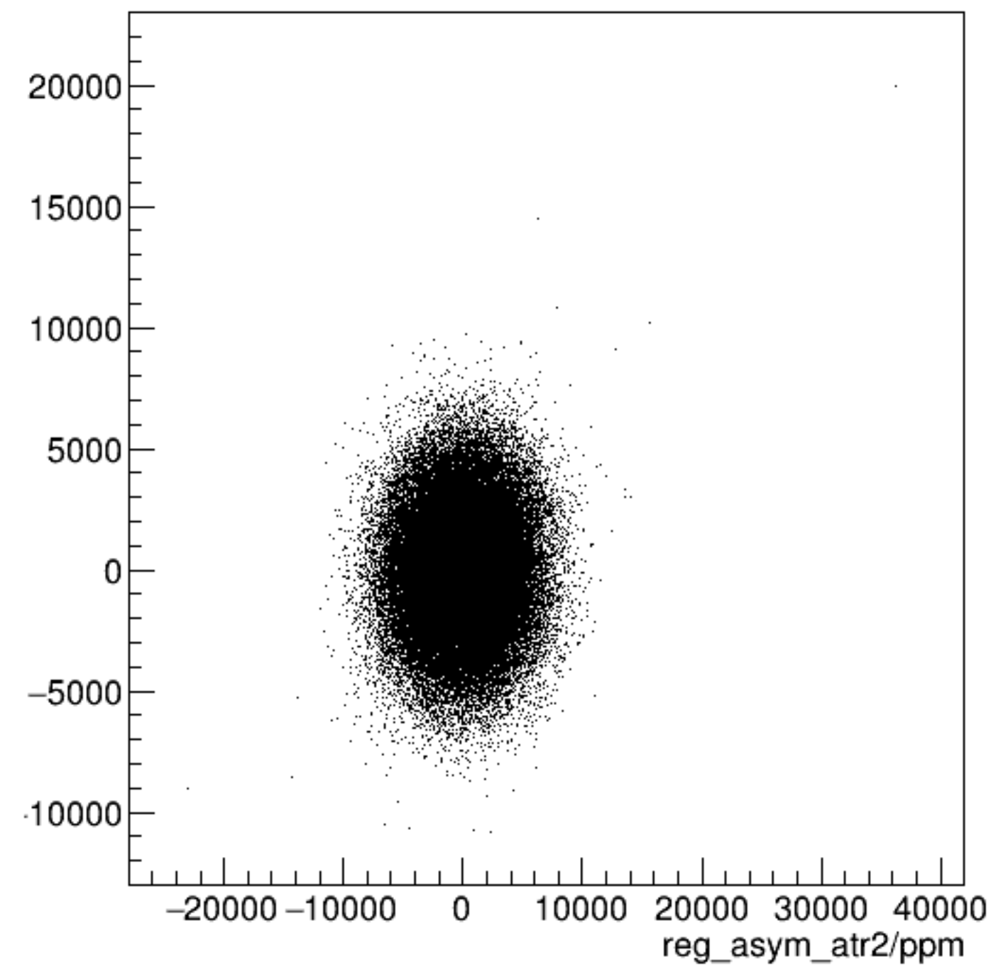
reg_asym_atl2/ppm:reg_asym_atr2/ppm {ok_cut}
