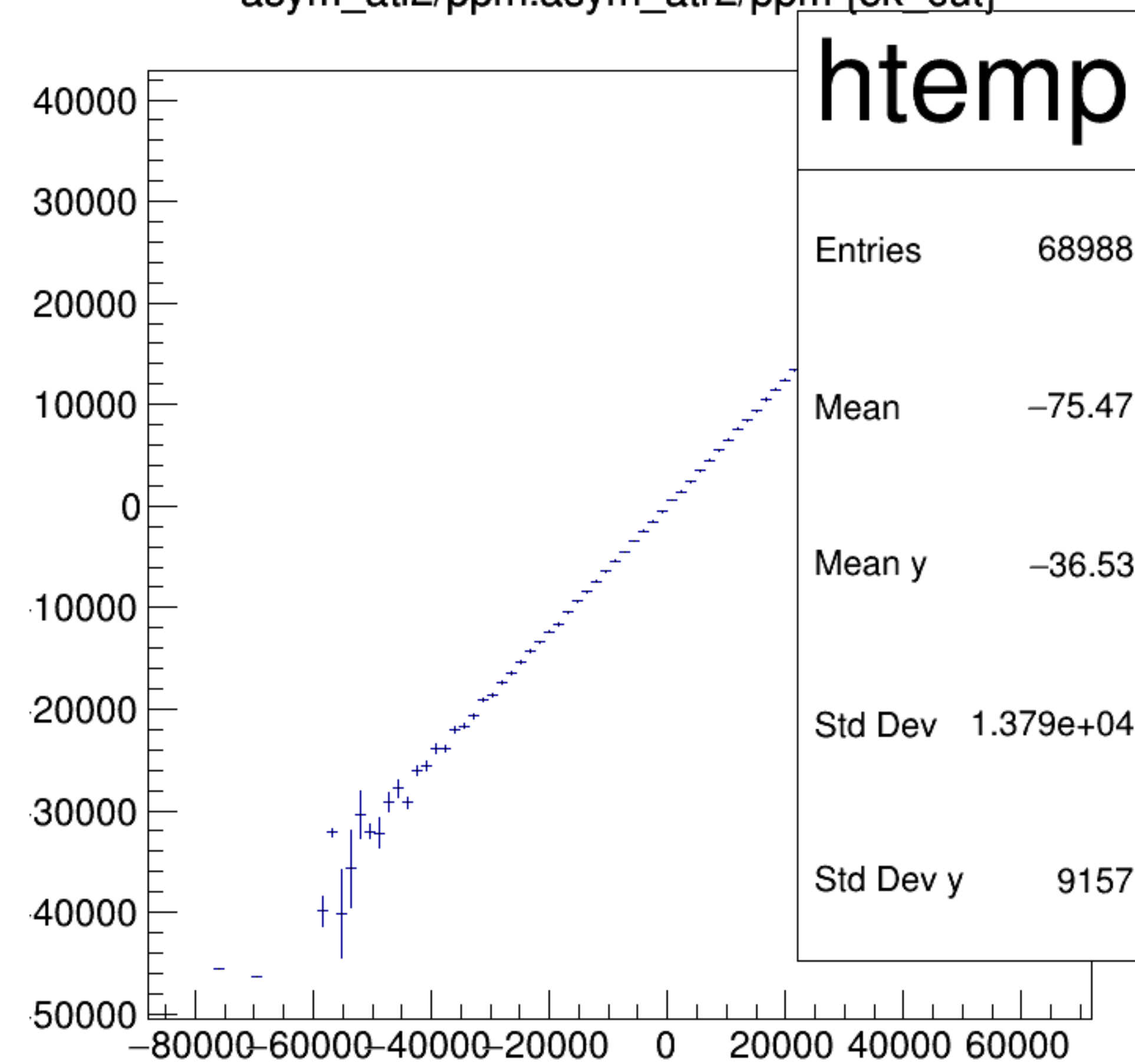
asym_atl2/ppm:asym_atr2/ppm {ok_cut}
