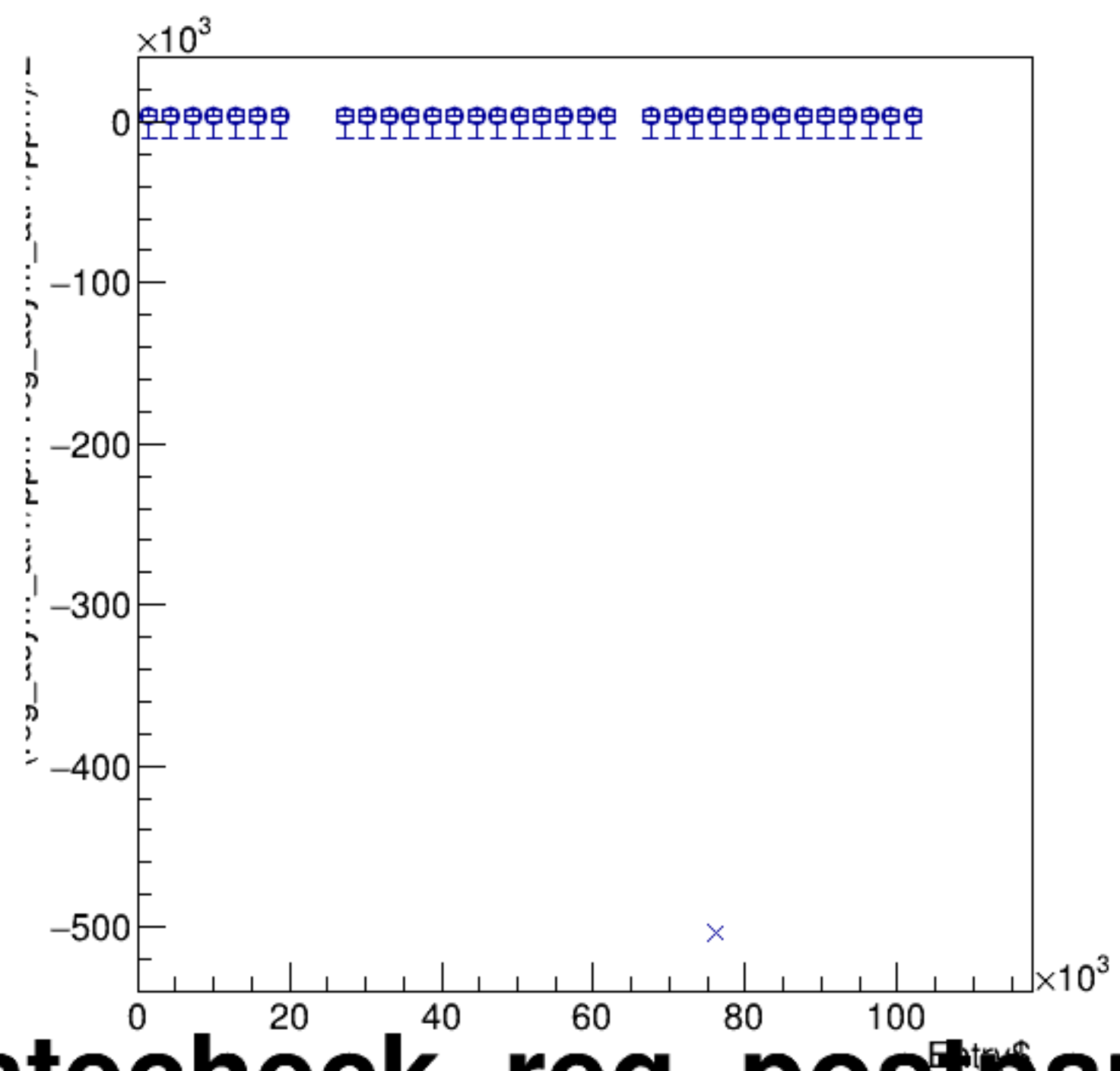
(reg_asym_atl1/ppm-reg_asym_atr1/ppm)/2:Entry$ {ok_cut}
