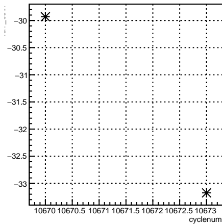
4eY_coil7:cyclenum {run == 8190}
