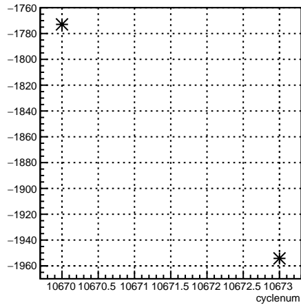
usr_coil3:cyclenum {run == 8190}
