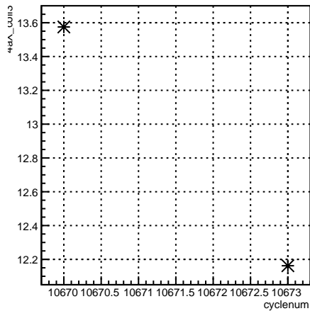
4eX_coil3:cyclenum {run == 8190}
