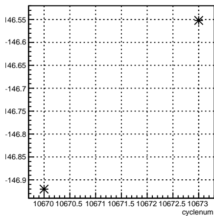
4eY_coil6:cyclenum {run == 8190}
