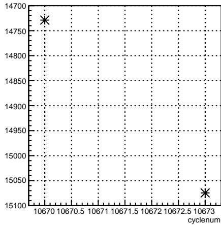
usr_coil1:cyclenum {run == 8190}
