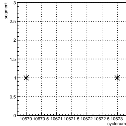
segment:cyclenum {run == 8190}
