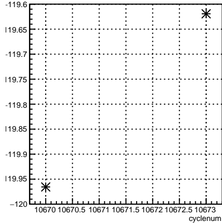
4eY_coil6:cyclenum {run == 8190}
