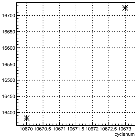
usl_coil6:cyclenum {run == 8190}
