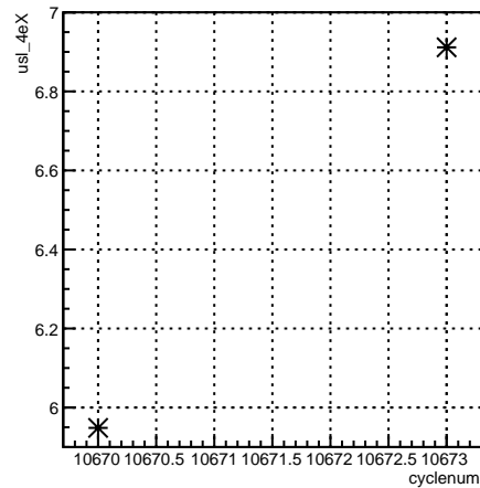
usl_4eX:cyclenum {run == 8190}
