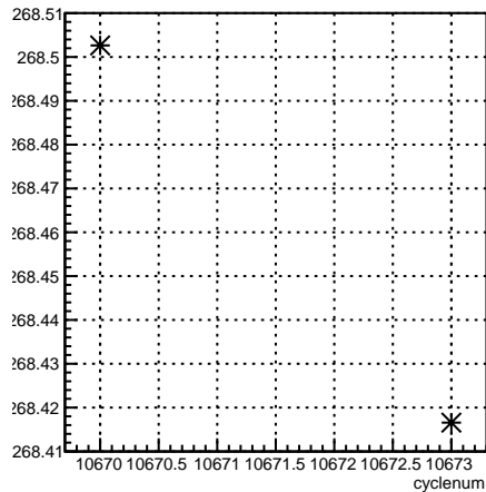
4eY_coil4:cyclenum {run == 8190}
