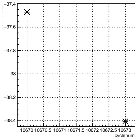
usl_11X12X:cyclenum {run == 8190}
