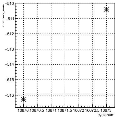
11X12X_coil7:cyclenum {run == 8190}
