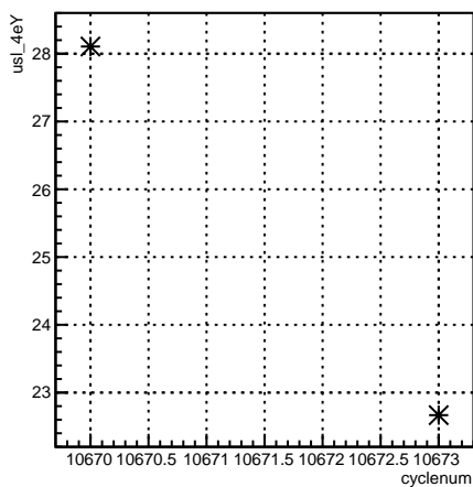
usl_4eY:cyclenum {run == 8190}
