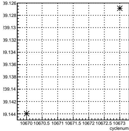
11X12X_coil1:cyclenum {run == 8190}
