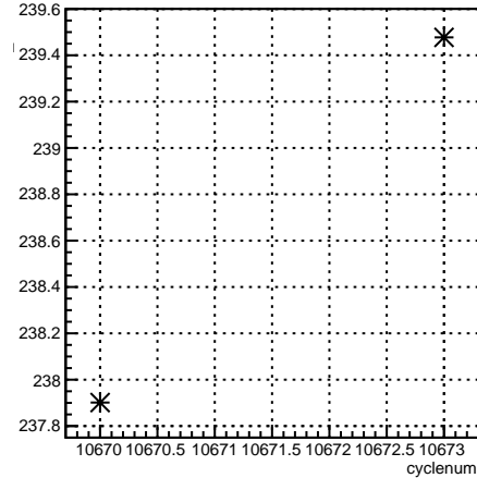
4eX_coil7:cyclenum {run == 8190}
