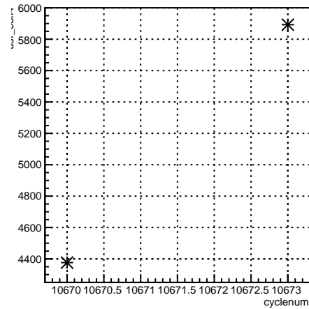
usr_coil4:cyclenum {run == 8190}
