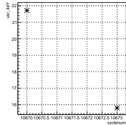
usr_4eY:cyclenum {run == 8190}
