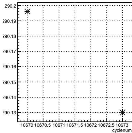
4eY_coil4:cyclenum {run == 8190}
