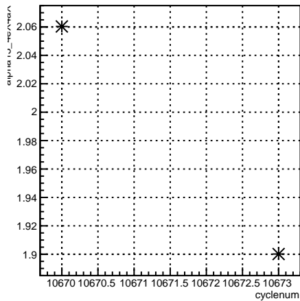
alpha13_4eX4aX:cyclenum {run == 8190}
