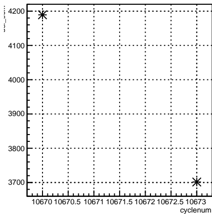
usl_coil7:cyclenum {run == 8190}
