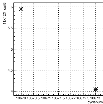
11X12X_coil6:cyclenum {run == 8190}
