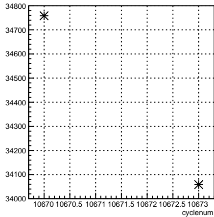
usr_coil7:cyclenum {run == 8190}
