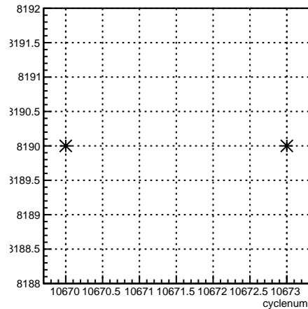
run:cyclenum {run == 8190}
