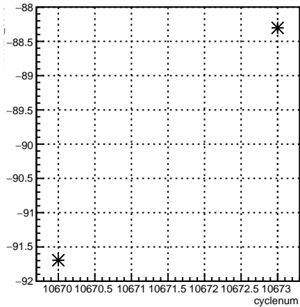
11X12X_coil3:cyclenum {run == 8190}
