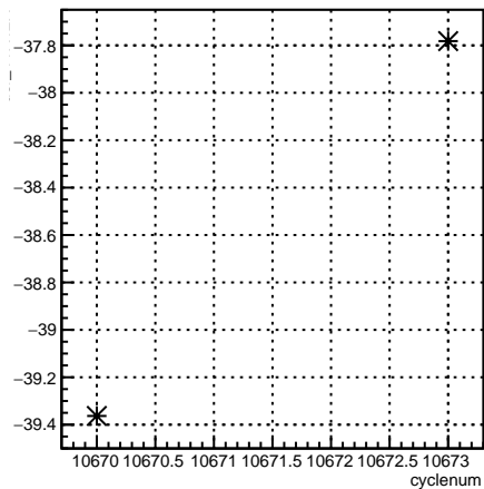
usr_11X12X:cyclenum {run == 8190}
