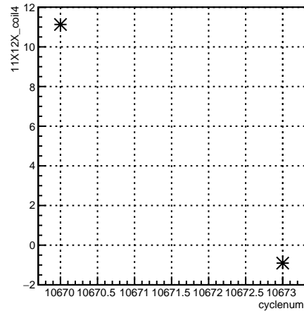
11X12X_coil4:cyclenum {run == 8190}
