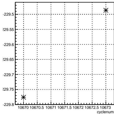
4eX_coil1:cyclenum {run == 8190}
