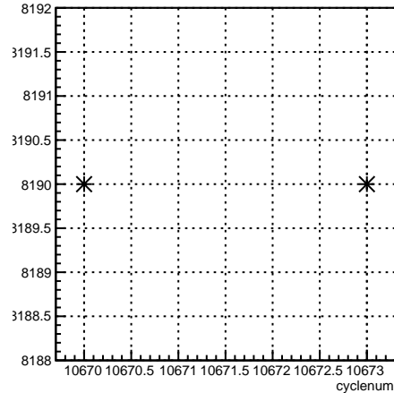
run:cyclenum {run == 8190}
