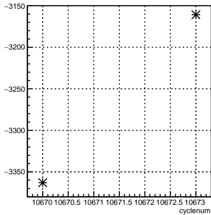
usr_coil6:cyclenum {run == 8190}
