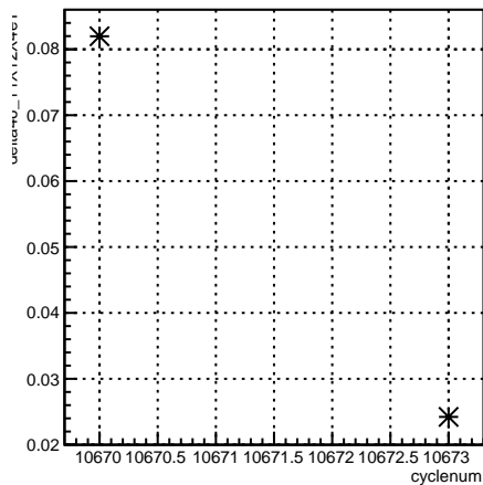
delta46_11X12X4eY:cyclenum {run == 8190}
