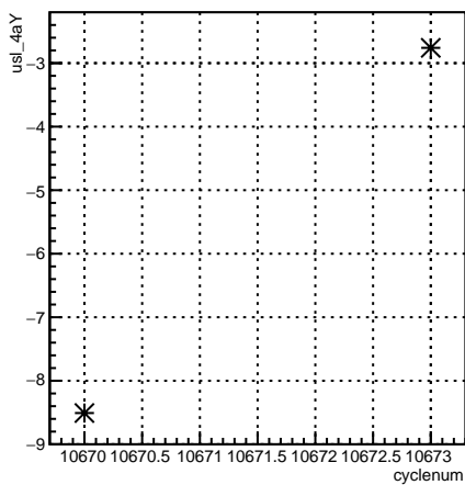
usl_4aY:cyclenum {run == 8190}
