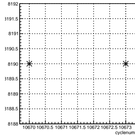
run:cyclenum {run == 8190}
