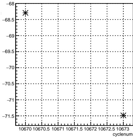
usl_4aX:cyclenum {run == 8190}
