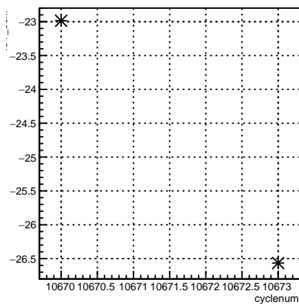
4eY_coil7:cyclenum {run == 8190}
