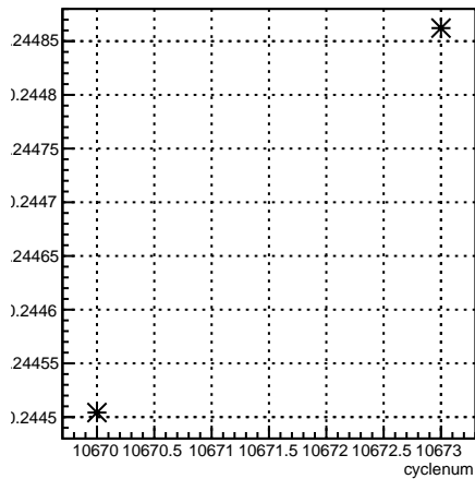
run:cyclenum {run == 8190}
