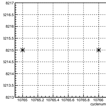
run:cyclenum {run == 8215}
