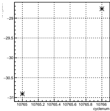
4eY_coil7:cyclenum {run == 8215}
