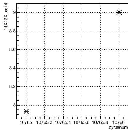
11X12X_coil4:cyclenum {run == 8215}
