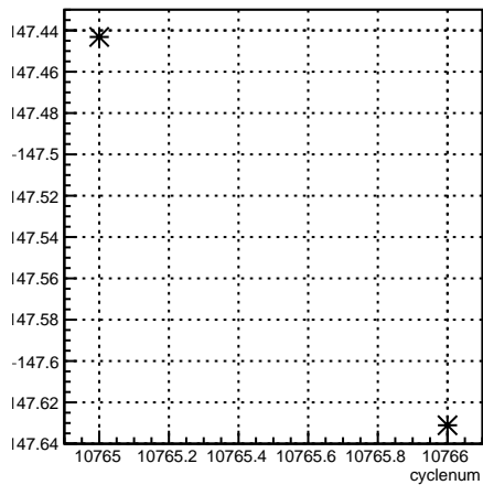
4eY_coil6:cyclenum {run == 8215}
