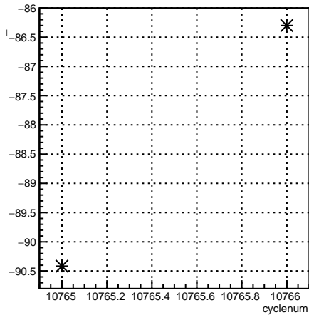
11X12X_coil3:cyclenum {run == 8215}
