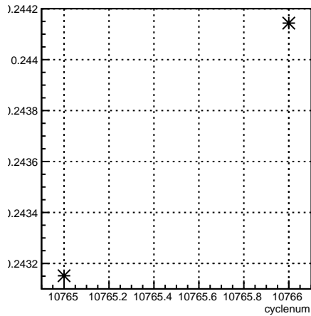
alpha46_4eY4aY:cyclenum {run == 8215}
