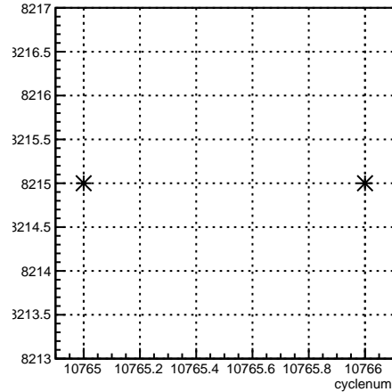
run:cyclenum {run == 8215}
