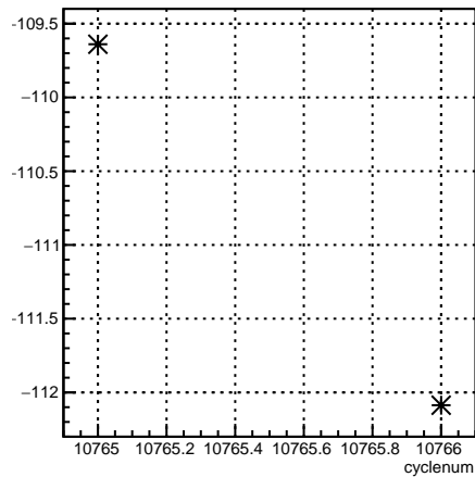
usr_4eY:cyclenum {run == 8215}
