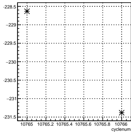
4eX_coil1:cyclenum {run == 8215}
