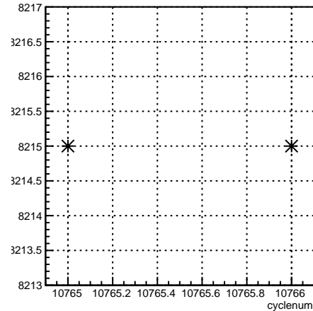
run:cyclenum {run == 8215}
