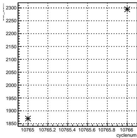
usl_coil7:cyclenum {run == 8215}
