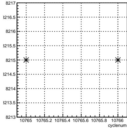
run:cyclenum {run == 8215}
