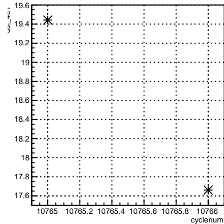
usl_4eY:cyclenum {run == 8215}
