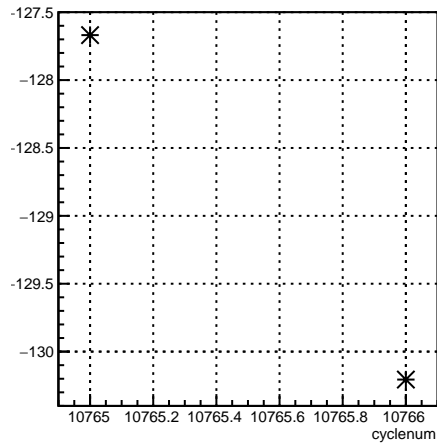
4aX_coil1:cyclenum {run == 8215}
