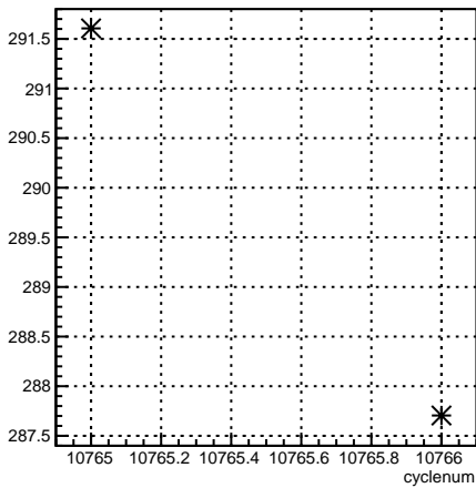
4eY_coil4:cyclenum {run == 8215}
