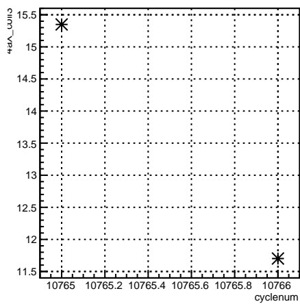
4aX_coil3:cyclenum {run == 8215}
