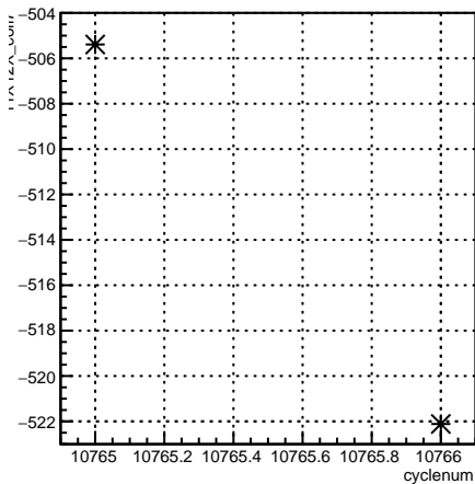
11X12X_coil7:cyclenum {run == 8215}
