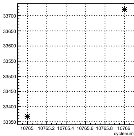
usr_coil7:cyclenum {run == 8215}
