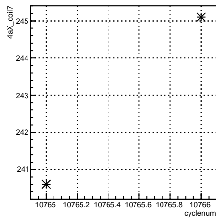
4aX_coil7:cyclenum {run == 8215}
