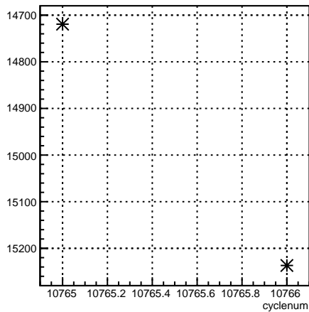
usr_coil6:cyclenum {run == 8215}
