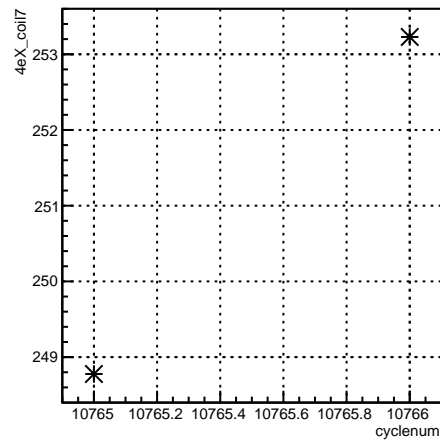
4eX_coil7:cyclenum {run == 8215}
