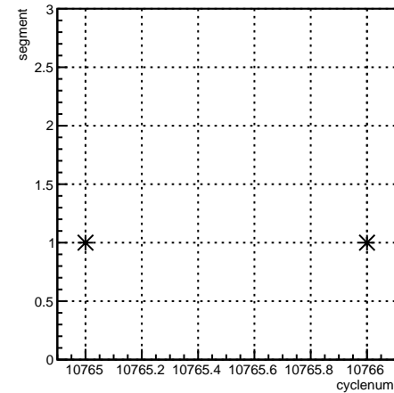
segment:cyclenum {run == 8215}
