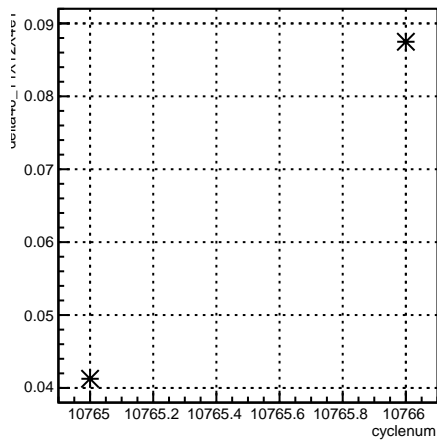
delta46_11X12X4eY:cyclenum {run == 8215}
