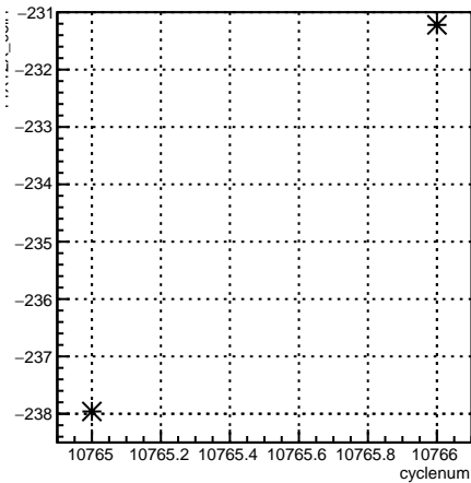
11X12X_coil1:cyclenum {run == 8215}
