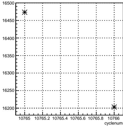
usl_coil6:cyclenum {run == 8215}
