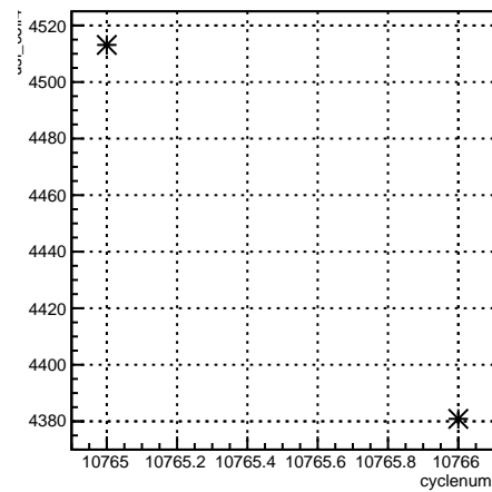
run:cyclenum {run == 8215}
