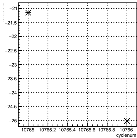
4eX_coil3:cyclenum {run == 8215}
