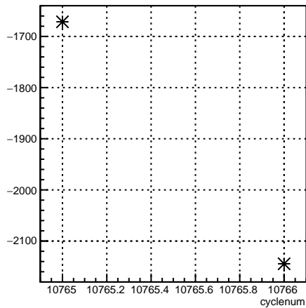
usr_coil7:cyclenum {run == 8215}
