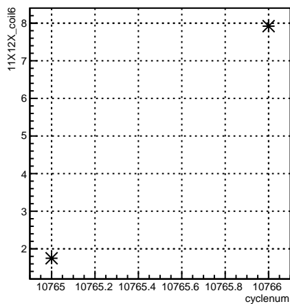
11X12X_coil6:cyclenum {run == 8215}
