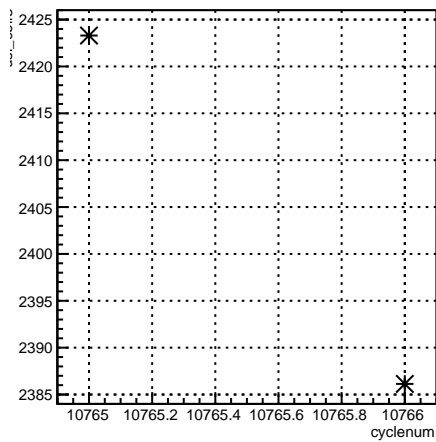
usl_coil7:cyclenum {run == 8215}
