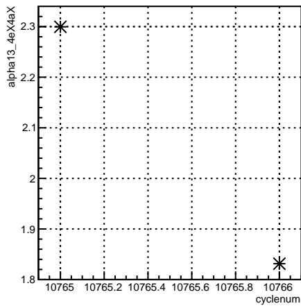
alpha13_4eX4aX:cyclenum {run == 8215}
