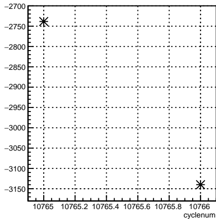
usr_coil6:cyclenum {run == 8215}
