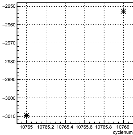
usl_coil6:cyclenum {run == 8215}
