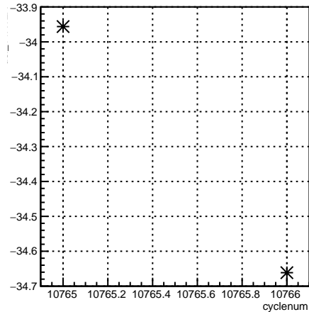
usl_11X12X:cyclenum {run == 8215}
