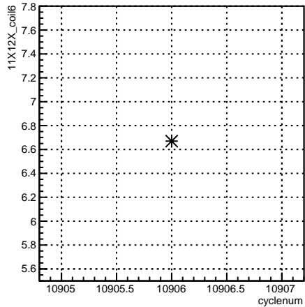
11X12X_coil6:cyclenum {run == 8244}
