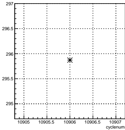
4aY_coil4:cyclenum {run == 8244}
