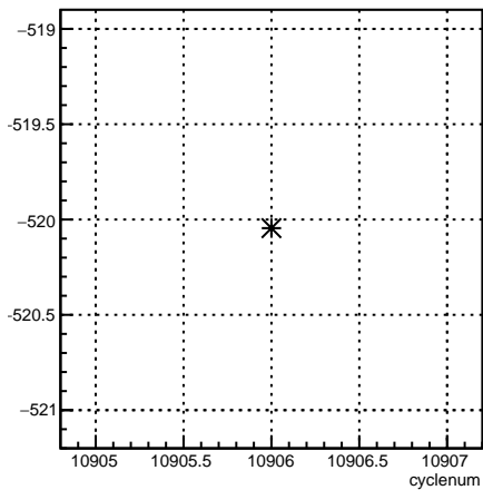
11X12X_coil7:cyclenum {run == 8244}
