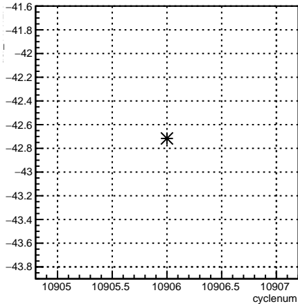
usr_11X12X:cyclenum {run == 8244}
