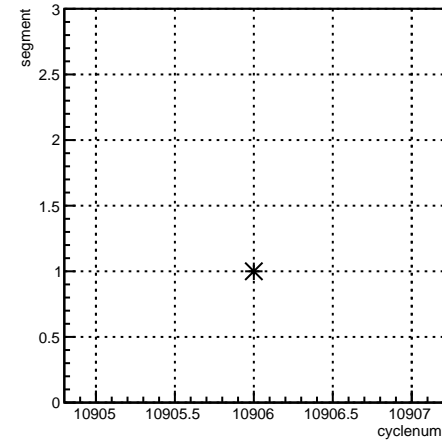
segment:cyclenum {run == 8244}
