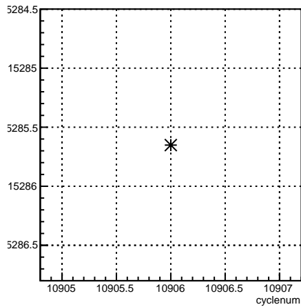
usr_coil1:cyclenum {run == 8244}
