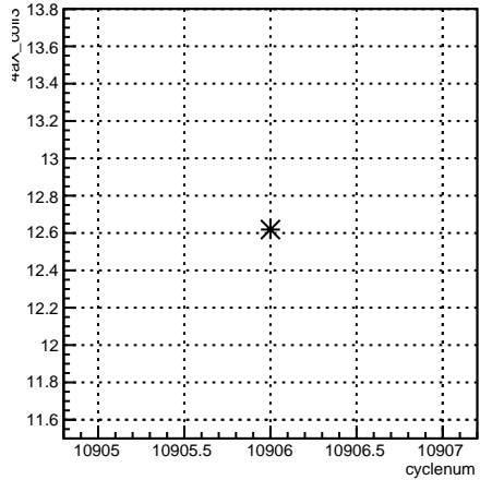
4eX_coil3:cyclenum {run == 8244}
