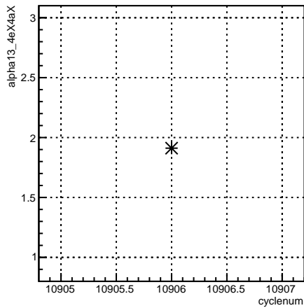
alpha13_4eX4aX:cyclenum {run == 8244}
