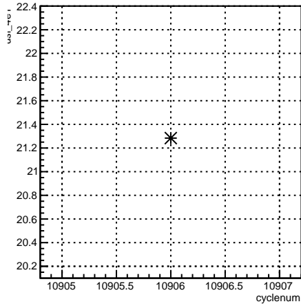
usl_4eY:cyclenum {run == 8244}
