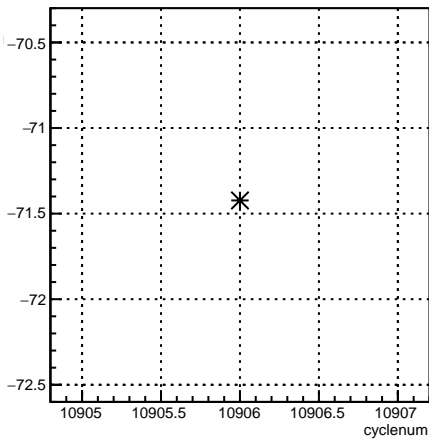
usl_4eY:cyclenum {run == 8244}
