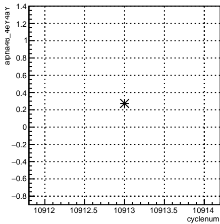
alpha46_4eY4aY:cyclenum {run == 8245}
