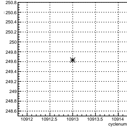
4eX_coil7:cyclenum {run == 8245}
