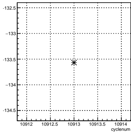
4eY_coil6:cyclenum {run == 8245}
