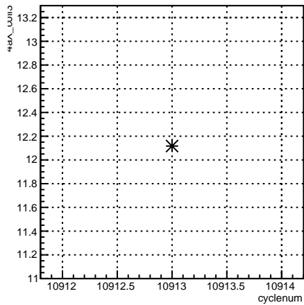
4eX_coil3:cyclenum {run == 8245}
