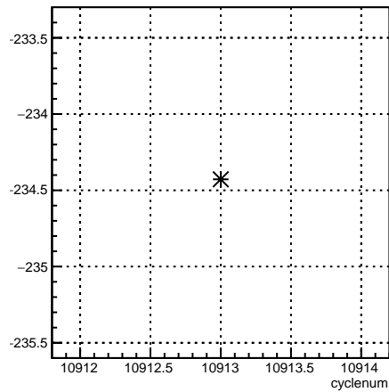
11X12X_coil6:cyclenum {run == 8245}
