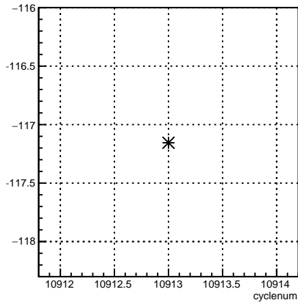
usr_4aX:cyclenum {run == 8245}
