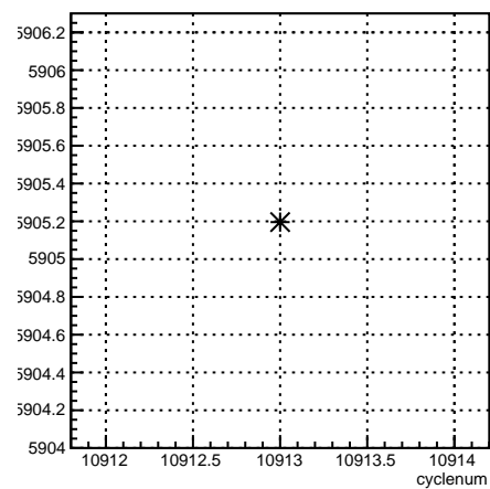
usl_coil4:cyclenum {run == 8245}
