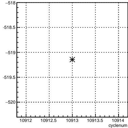
11X12X_coil7:cyclenum {run == 8245}
