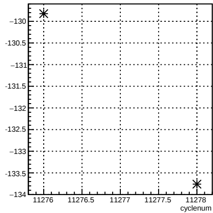
4eX_coil1:cyclenum {run == 8344}
