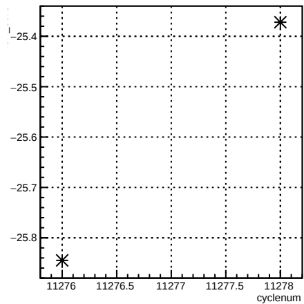
4eX_coil3:cyclenum {run == 8344}
