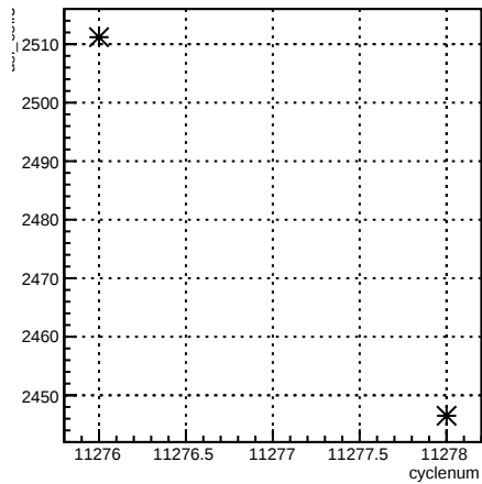
usl_coil7:cyclenum {run == 8344}
