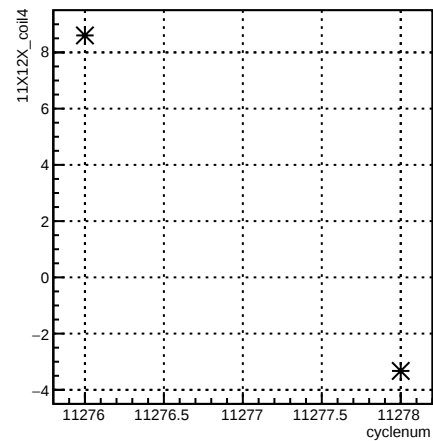
11X12X_coil4:cyclenum {run == 8344}
