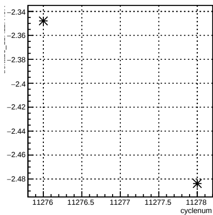
delta13_11X12X4eX:cyclenum {run == 8344}
