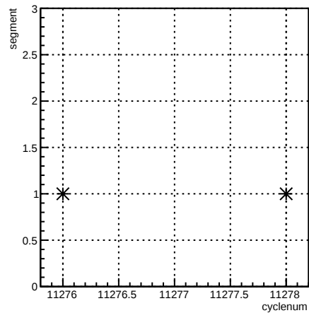
segment:cyclenum {run == 8344}
