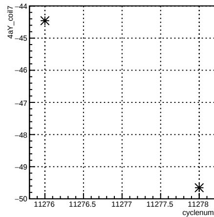
4aY_coil7:cyclenum {run == 8344}
