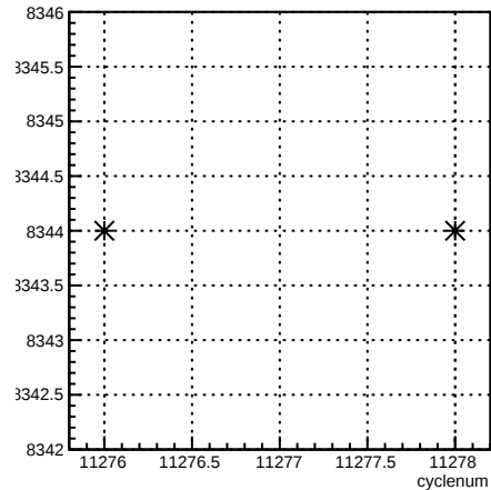
run:cyclenum {run == 8344}
