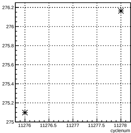
4eY_coil4:cyclenum {run == 8344}
