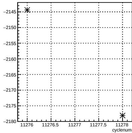
usr_coil7:cyclenum {run == 8344}
