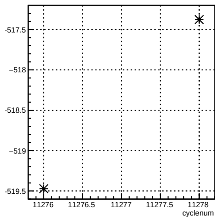
11X12X_coil7:cyclenum {run == 8344}
