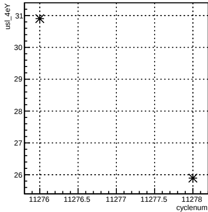
usl_4eY:cyclenum {run == 8344}
