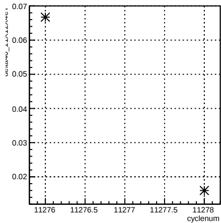
delta46_11X12X4eY:cyclenum {run == 8344}
