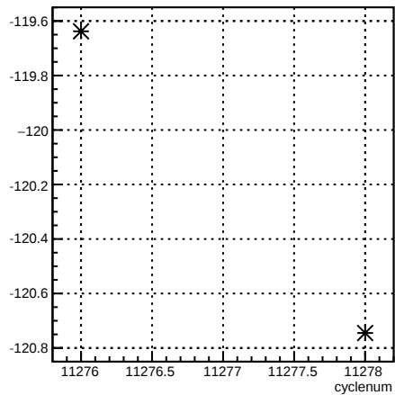
usr_4eY:cyclenum {run == 8344}
