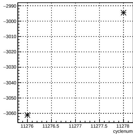
usr_coil6:cyclenum {run == 8344}
