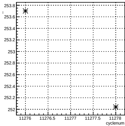
4eX_coil7:cyclenum {run == 8344}
