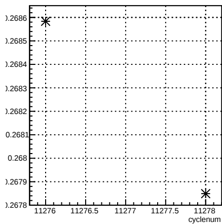
alpha46_4eY4aY:cyclenum {run == 8344}
