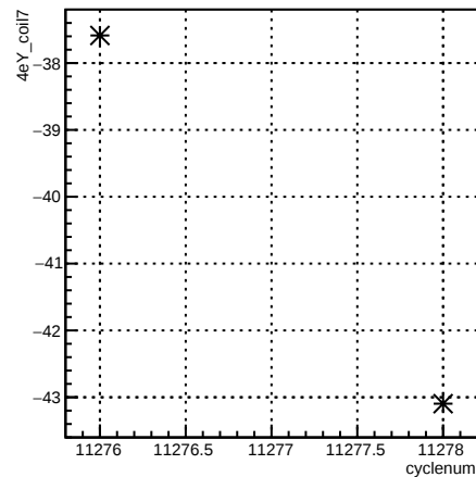
4eY_coil7:cyclenum {run == 8344}
