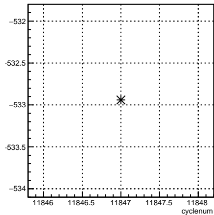
11X12X_coil7:cyclenum {run == 8532}
