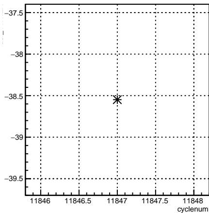
usr_11X12X:cyclenum {run == 8532}
