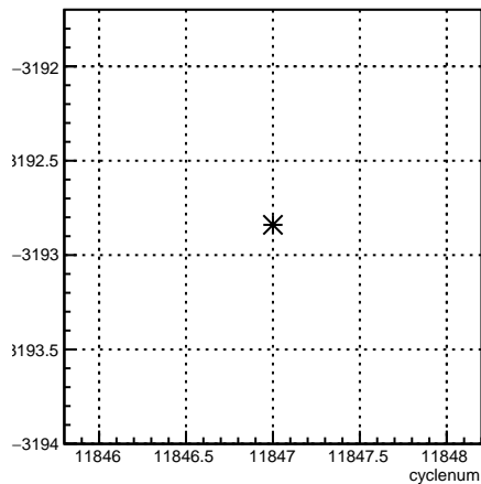
usl_coil6:cyclenum {run == 8532}
