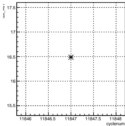
usl_4eY:cyclenum {run == 8532}
