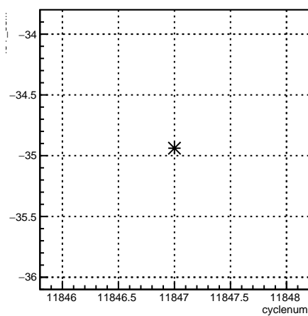
4eY_coil7:cyclenum {run == 8532}
