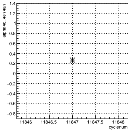
alpha46_4eY4aY:cyclenum {run == 8532}
