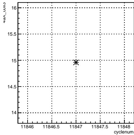
4eX_coil3:cyclenum {run == 8532}
