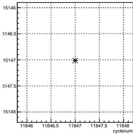
usr_coil6:cyclenum {run == 8532}
