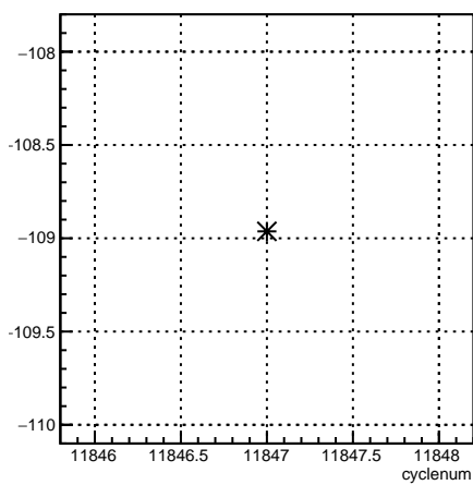
4aY_coil6:cyclenum {run == 8532}
