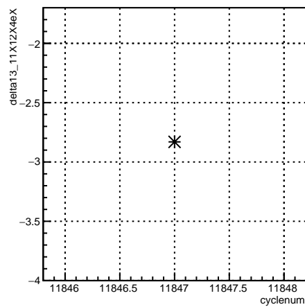
delta13_11X12X4eX:cyclenum {run == 8532}
