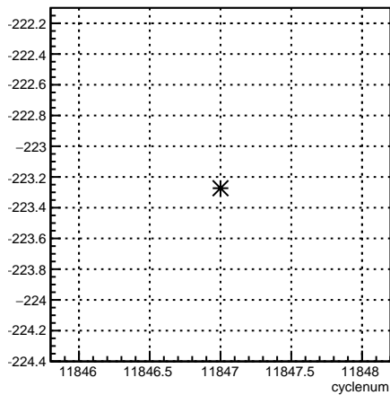
4eX_coil1:cyclenum {run == 8532}
