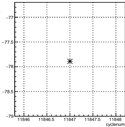
usl_4eY:cyclenum {run == 8532}
