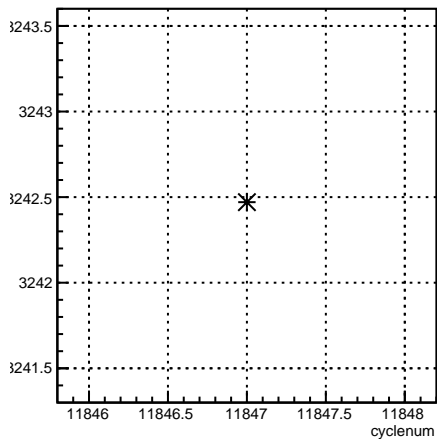
usl_coil7:cyclenum {run == 8532}
