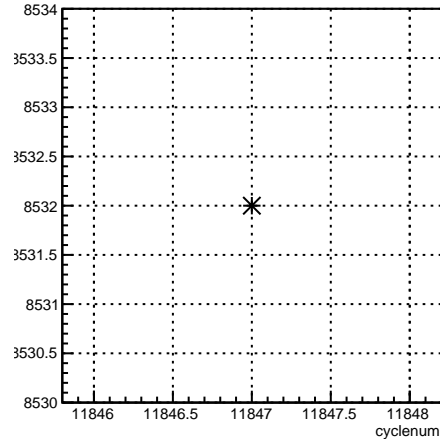
run:cyclenum {run == 8532}
