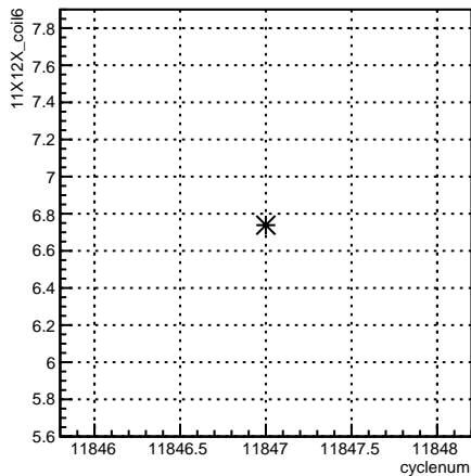
11X12X_coil6:cyclenum {run == 8532}
