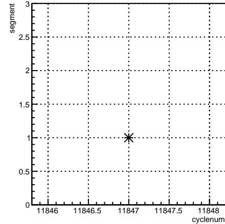
segment:cyclenum {run == 8532}
