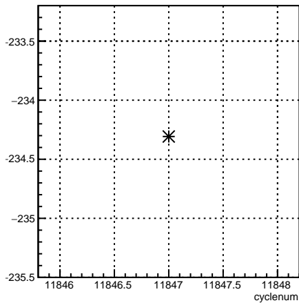
11X12X_coil1:cyclenum {run == 8532}
