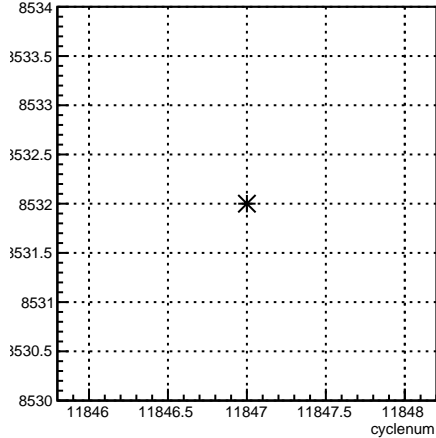
run:cyclenum {run == 8532}
