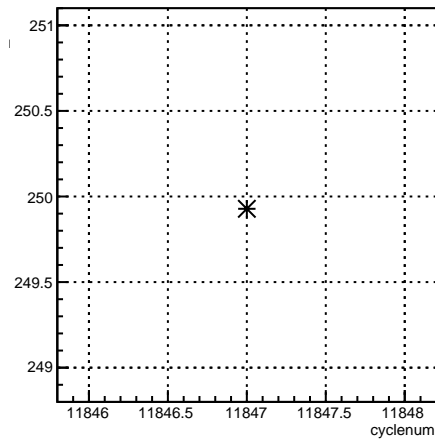
4eX_coil7:cyclenum {run == 8532}
