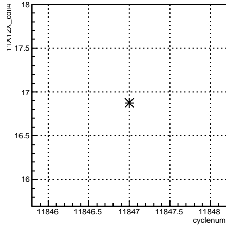
11X12X_coil4:cyclenum {run == 8532}
