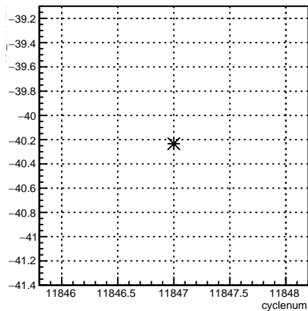
usl_11X12X:cyclenum {run == 8532}
