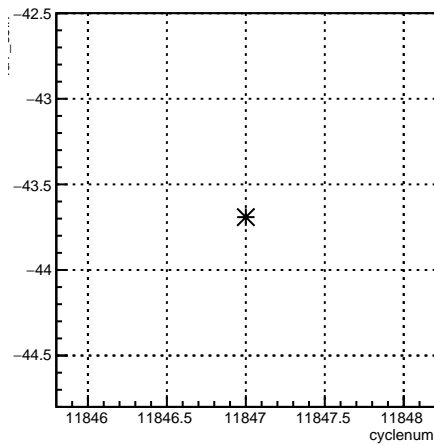
4aY_coil7:cyclenum {run == 8532}
