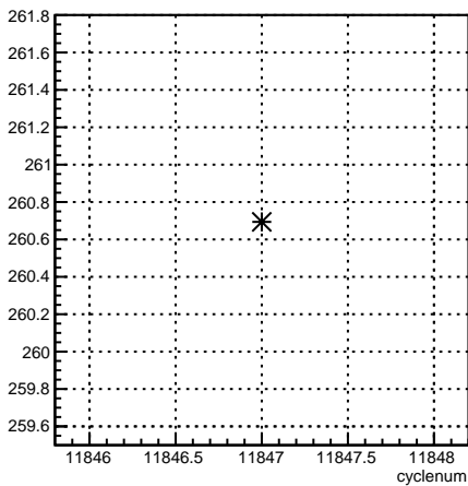
4eY_coil4:cyclenum {run == 8532}
