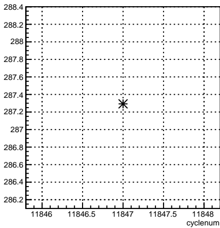
4aY_coil4:cyclenum {run == 8532}
