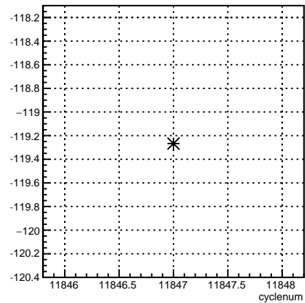
usr_4eY:cyclenum {run == 8532}
