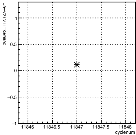
delta46_11X12X4eY:cyclenum {run == 8532}
