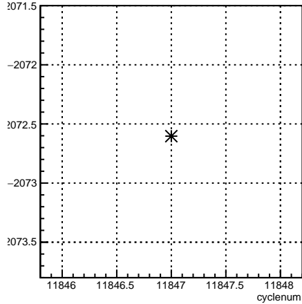
usr_coil7:cyclenum {run == 8532}
