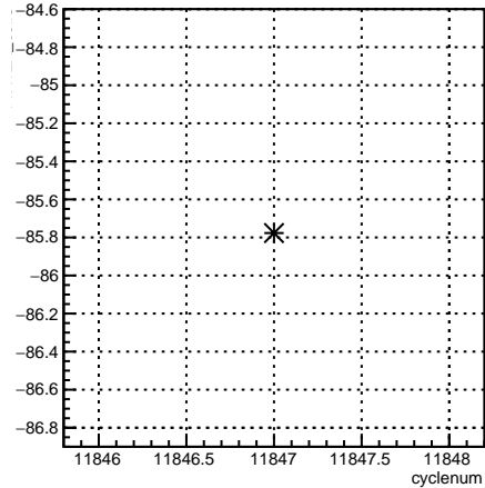
11X12X_coil3:cyclenum {run == 8532}
