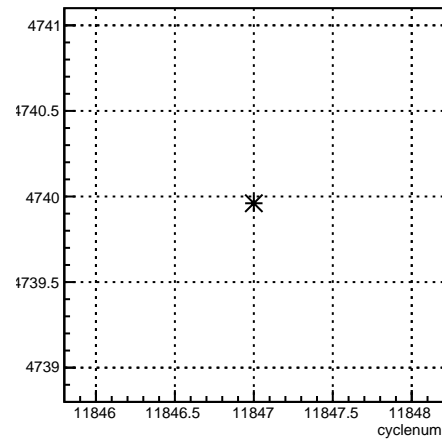
run:cyclenum {run == 8532}
