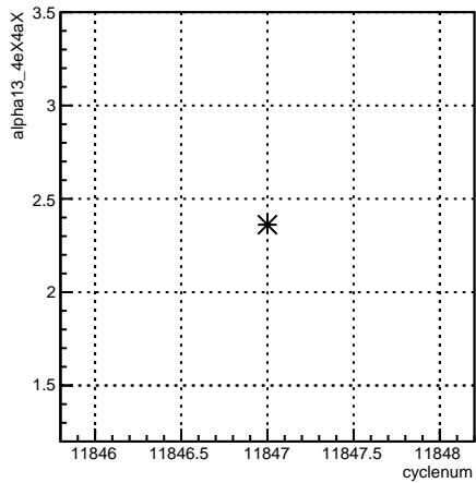
alpha13_4eX4aX:cyclenum {run == 8532}
