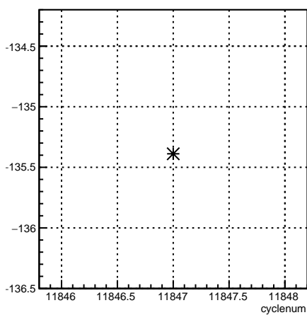
4eY_coil6:cyclenum {run == 8532}
