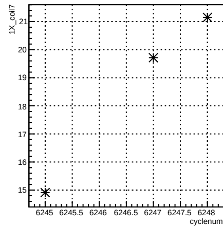
1X_coil7:cyclenum
