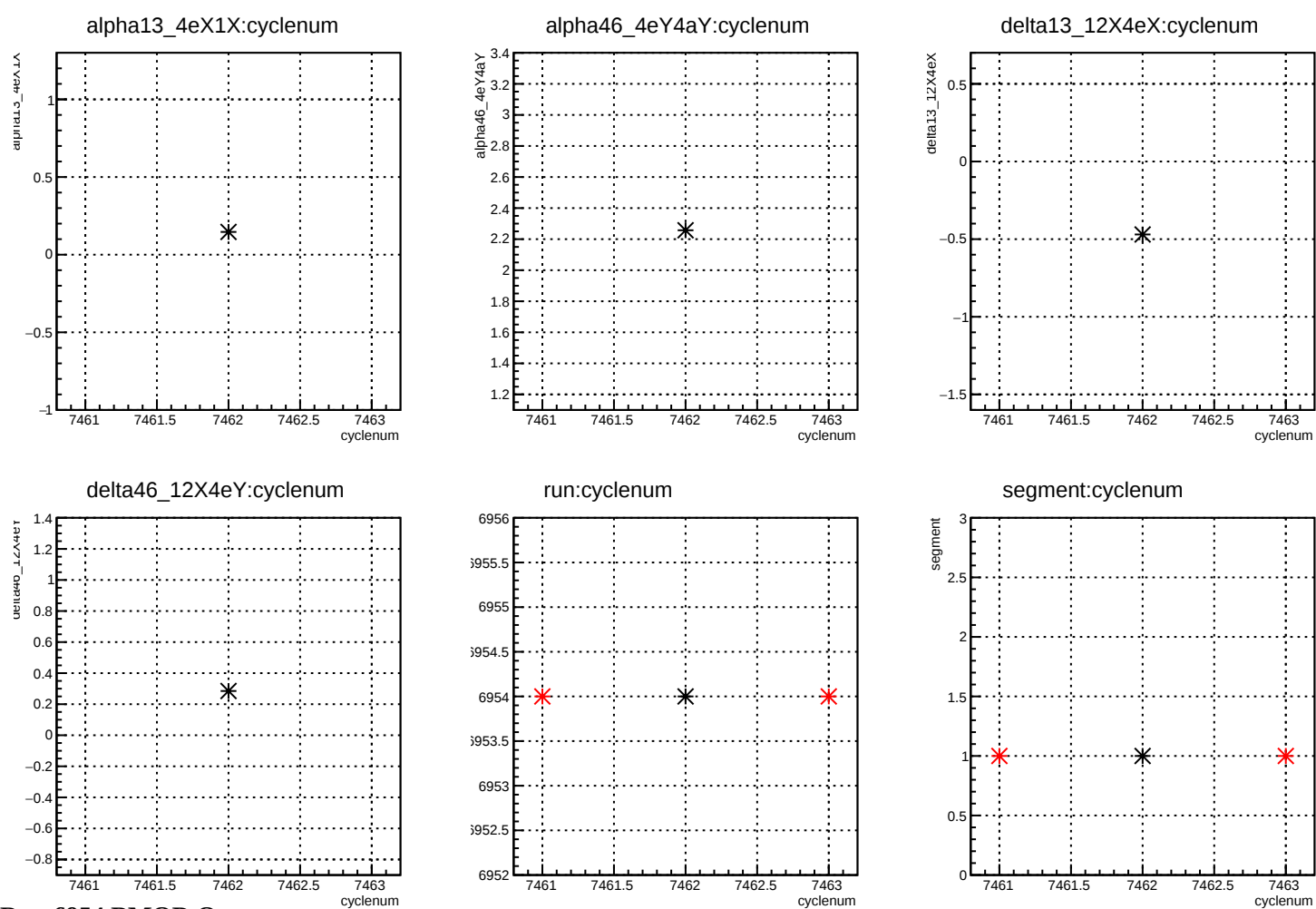
Run 6954 BMOD Outputs
