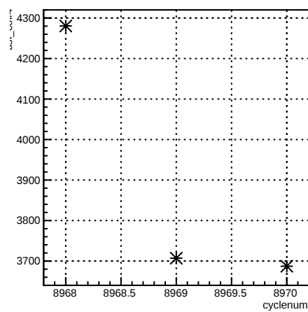
usl_coil4:cyclenum
