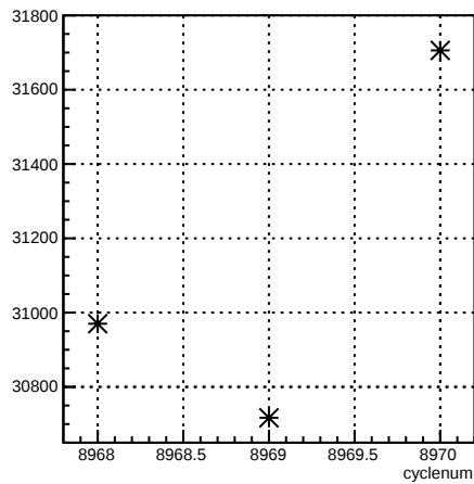
usl_coil1:cyclenum
