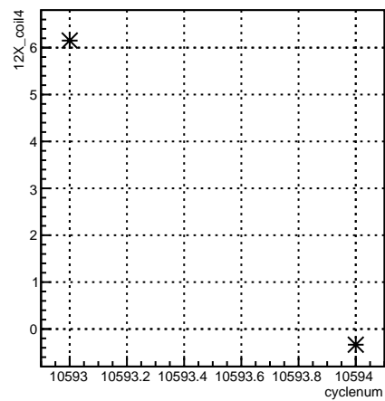
12X_coil4:cyclenum
