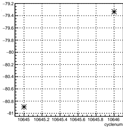
usl_1X:cyclenum
