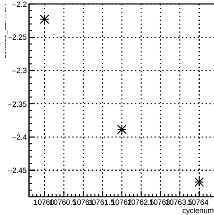
delta13_12X4eX:cyclenum
