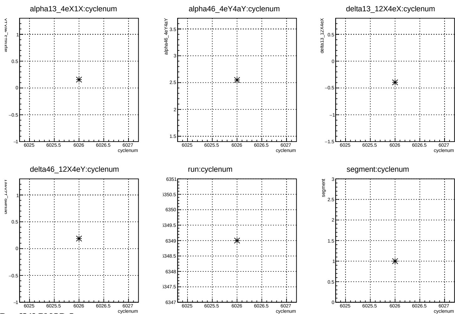
Run 6349 BMOD Outputs
