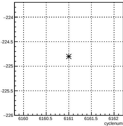
usr_1X:cyclenum
