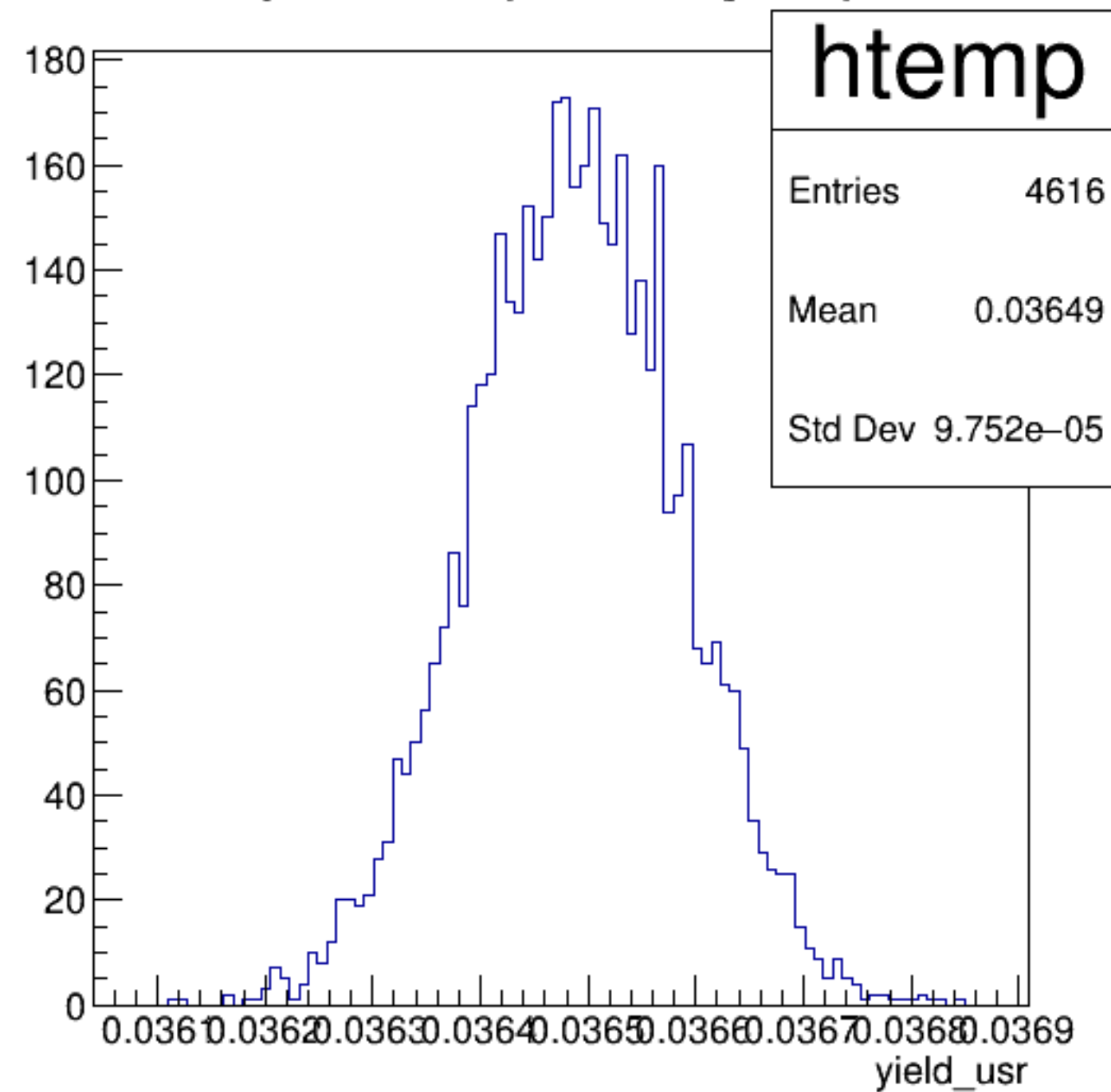
yield_usr {ErrorFlag==0}
