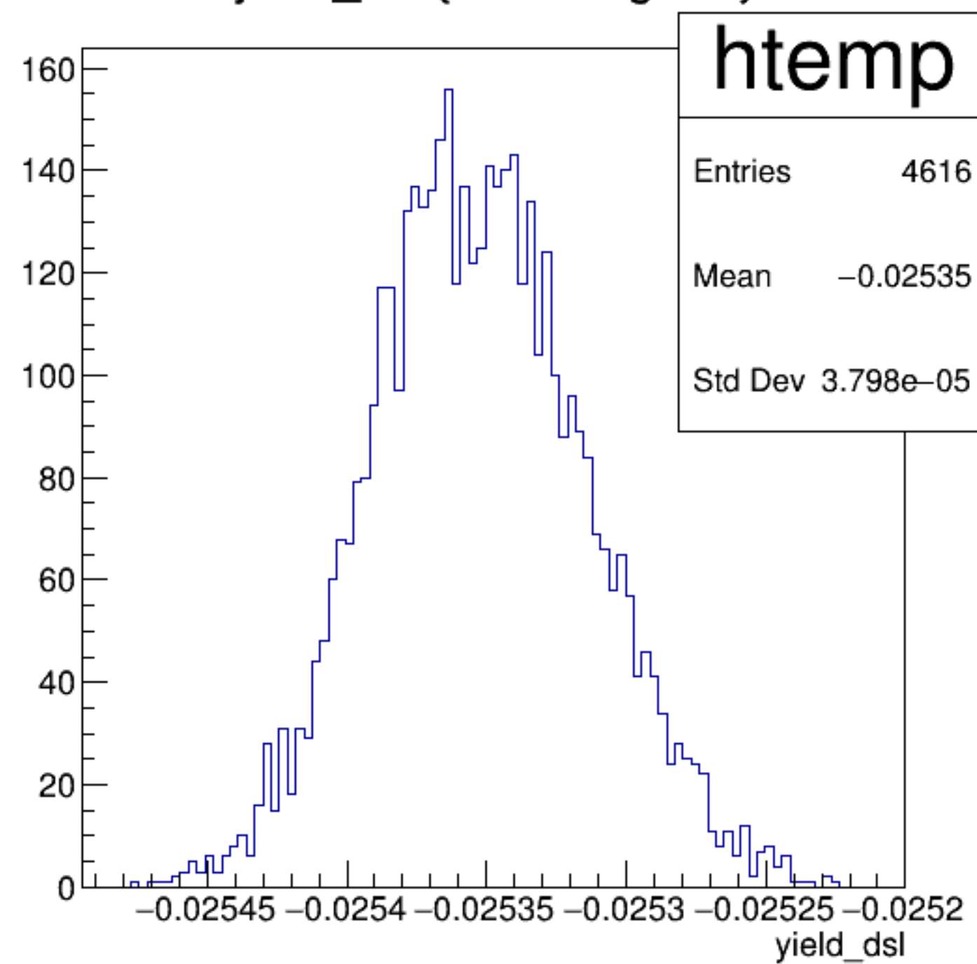
yield_dsl {ErrorFlag==0}
