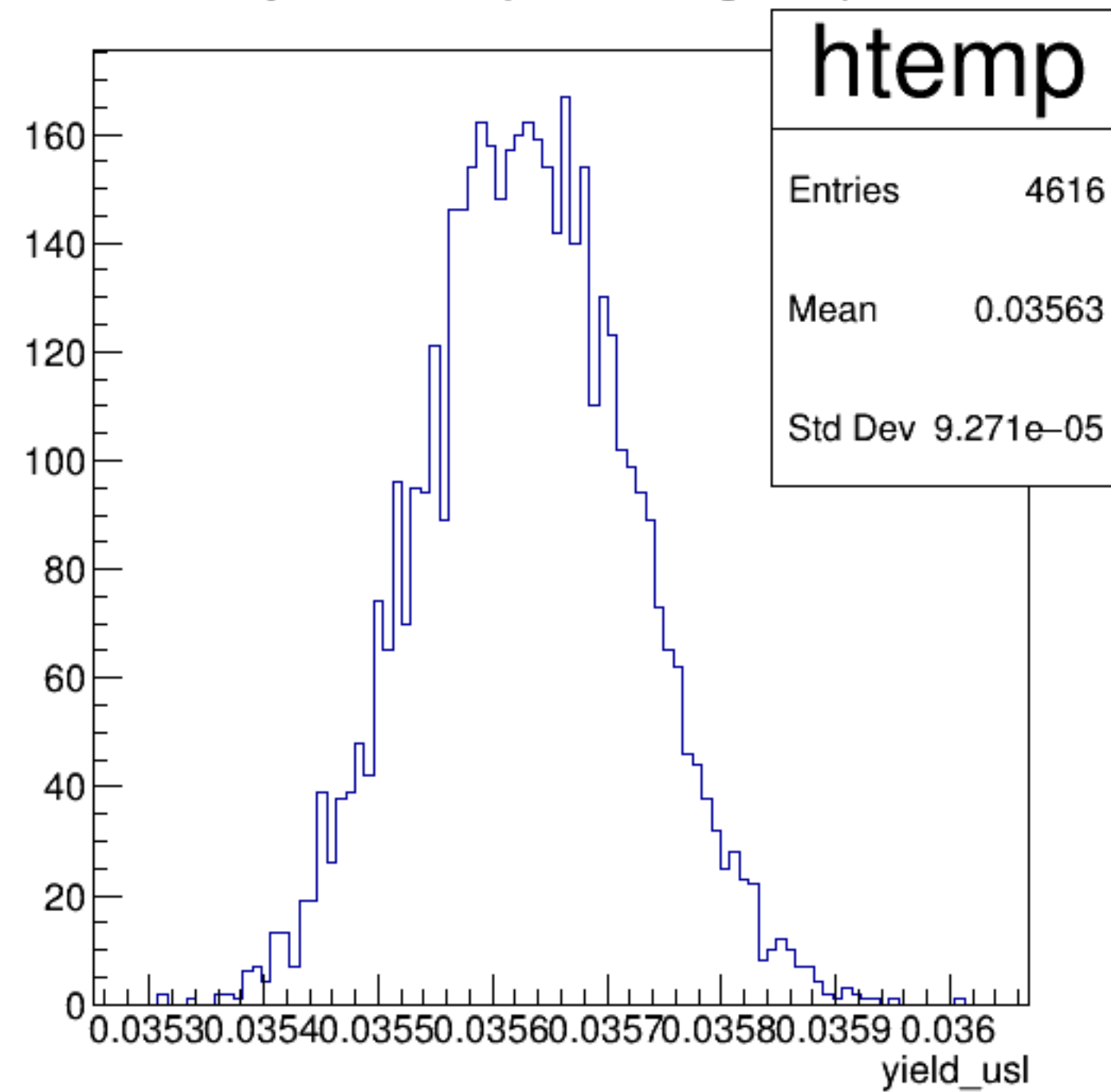
yield_usl {ErrorFlag==0}
