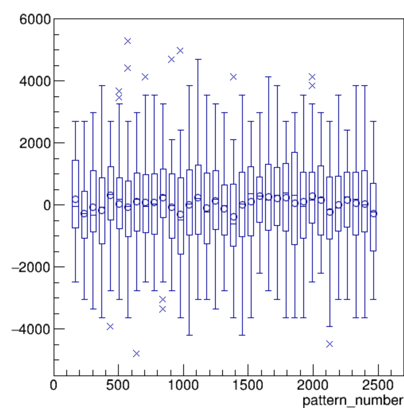
asym_usr/ppm:pattern_number {ErrorFlag==0}
