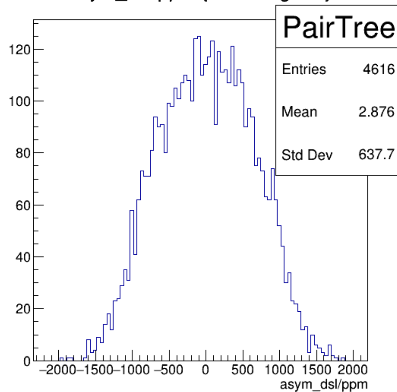
asym_dsl/ppm {ErrorFlag==0}
