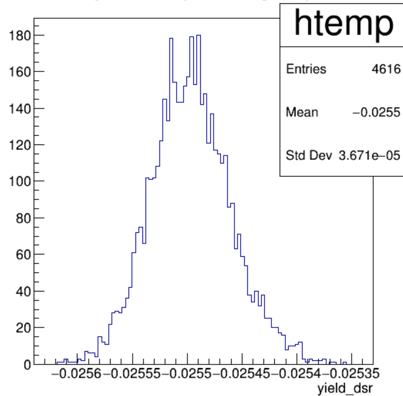
yield_dsr {ErrorFlag==0}
