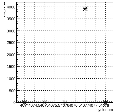
run:cyclenum {run == 5442}
