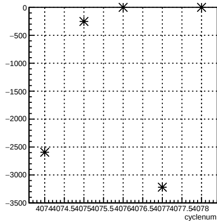
usr_coil6:cyclenum {run == 5442}
