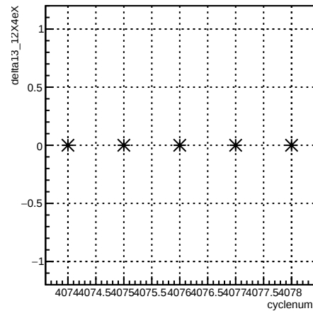
delta13_12X4eX:cyclenum {run == 5442}
