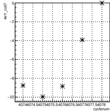
4eY_coil7:cyclenum {run == 5442}
