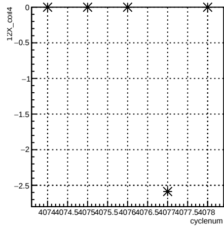
12X_coil4:cyclenum {run == 5442}
