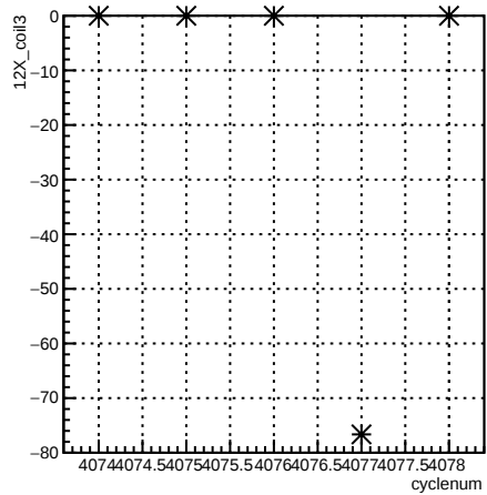
12X_coil3:cyclenum {run == 5442}
