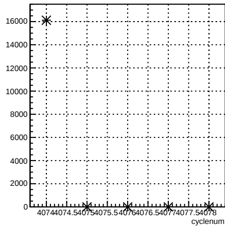
usl_coil6:cyclenum {run == 5442}
