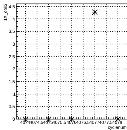
1X_coil3:cyclenum {run == 5442}
