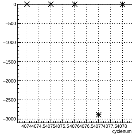
usr_coil3:cyclenum {run == 5442}
