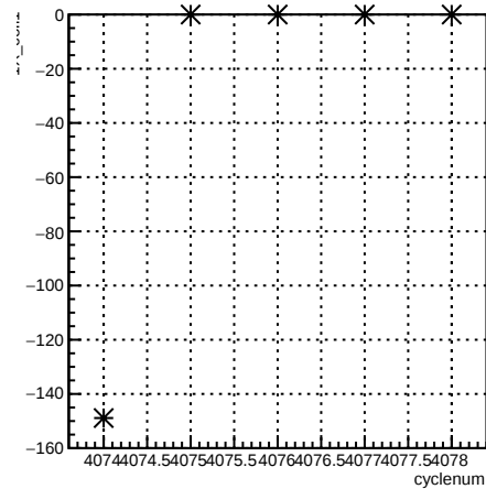
1X_coil1:cyclenum {run == 5442}
