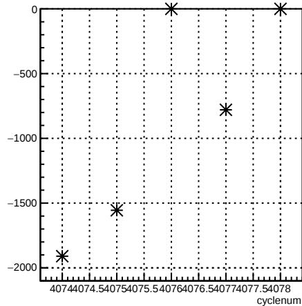
usl_coil6:cyclenum {run == 5442}
