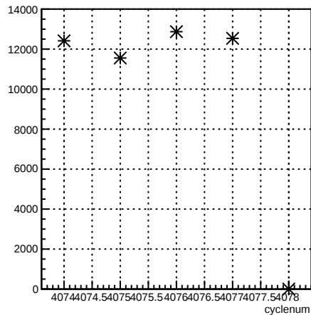
usl_coil7:cyclenum {run == 5442}
