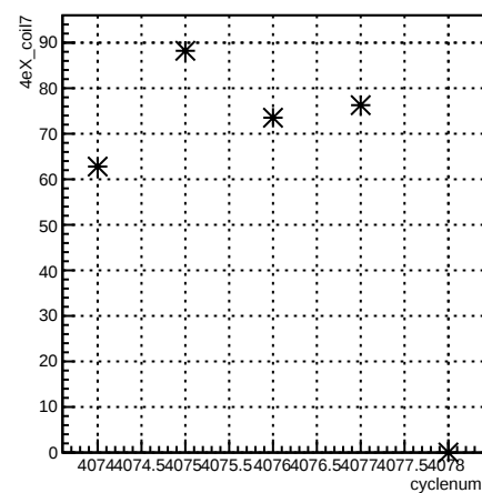
4eX_coil7:cyclenum {run == 5442}
