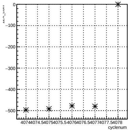
12X_coil7:cyclenum {run == 5442}
