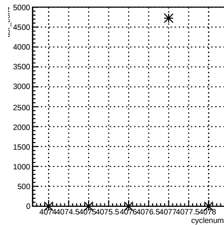
usr_coil4:cyclenum {run == 5442}
