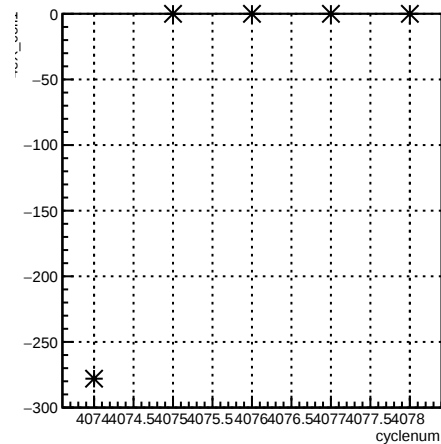
4eX_coil1:cyclenum {run == 5442}
