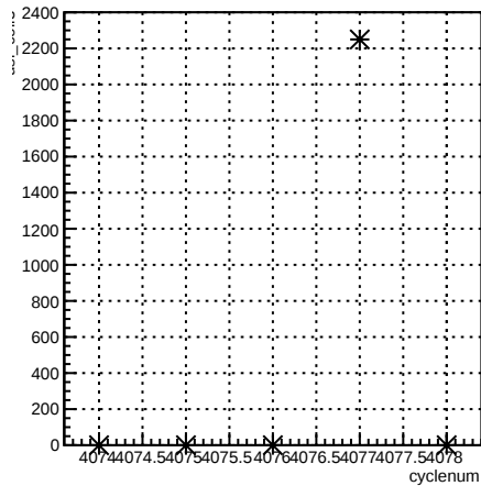
usl_coil3:cyclenum {run == 5442}
