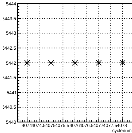
run:cyclenum {run == 5442}
