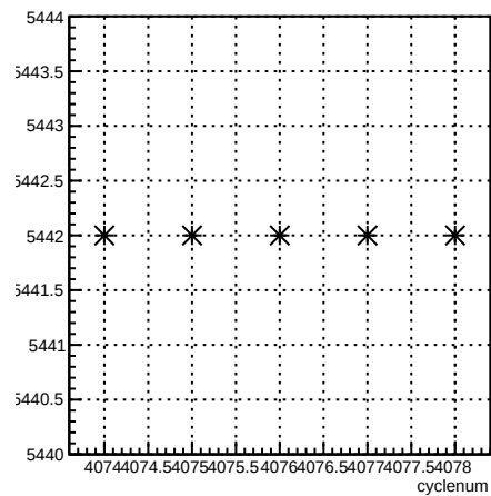
run:cyclenum {run == 5442}
