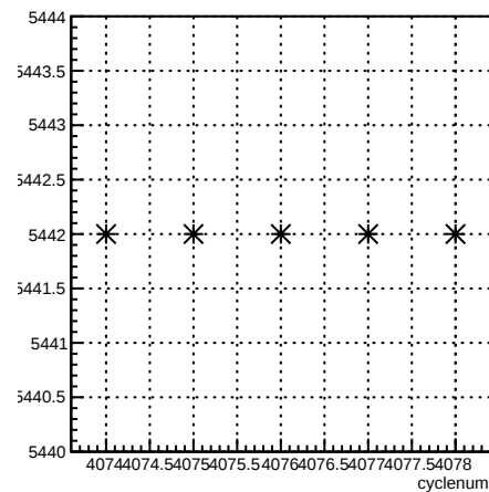
run:cyclenum {run == 5442}
