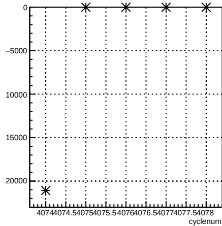
usr_coil1:cyclenum {run == 5442}
