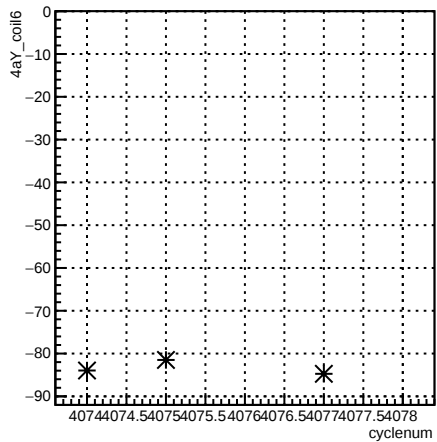
4aY_coil6:cyclenum {run == 5442}
