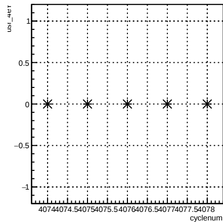
usr_4eY:cyclenum {run == 5442}
