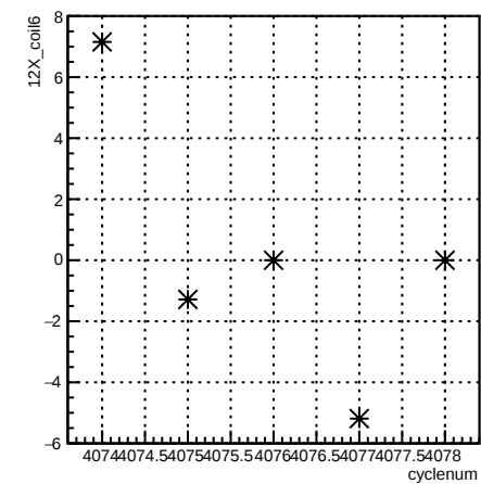
12X_coil6:cyclenum {run == 5442}
