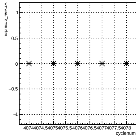
alpha13_4eX1X:cyclenum {run == 5442}
