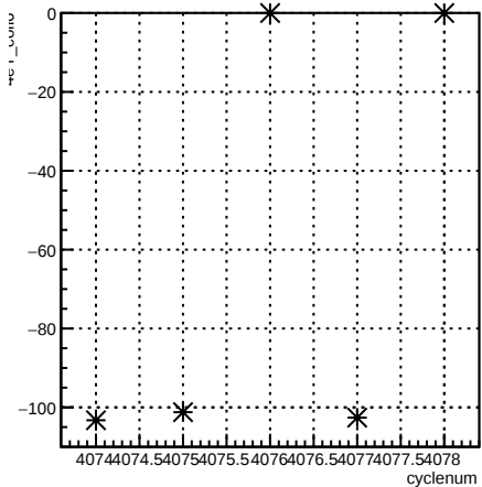
4eY_coil6:cyclenum {run == 5442}
