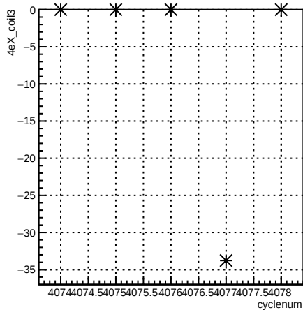
4eX_coil3:cyclenum {run == 5442}
