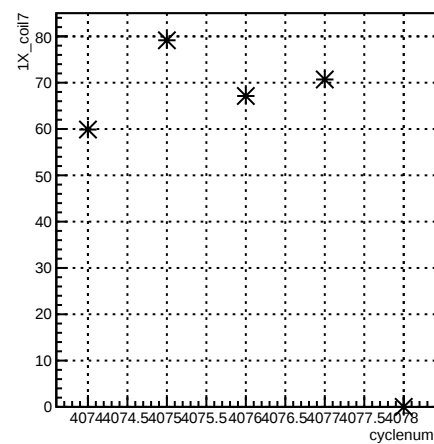
1X_coil7:cyclenum {run == 5442}
