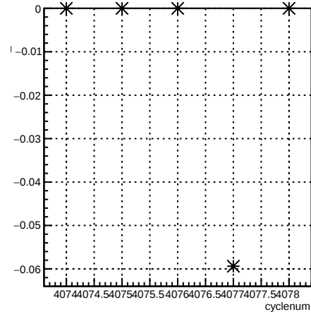
delta46_12X4eY:cyclenum {run == 5442}
