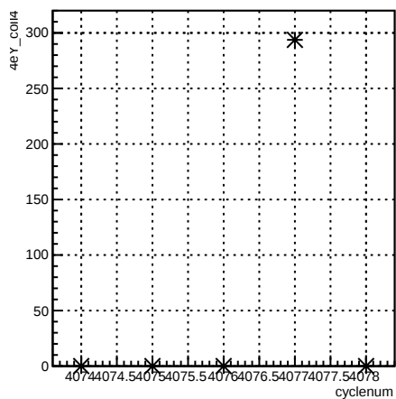
4eY_coil4:cyclenum {run == 5442}
