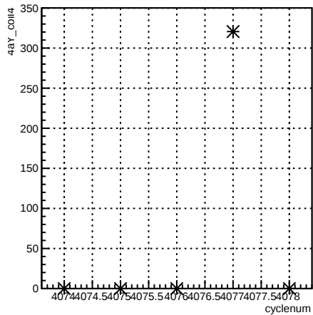
4aY_coil4:cyclenum {run == 5442}
