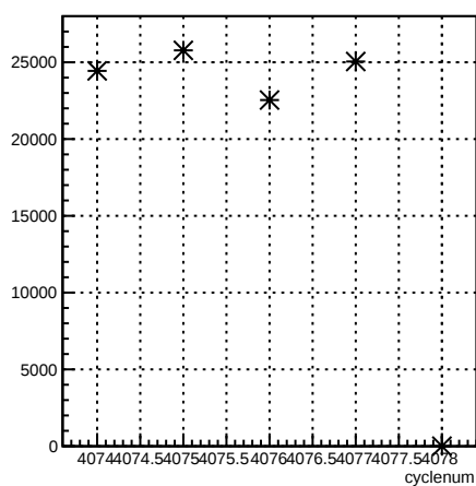
usr_coil7:cyclenum {run == 5442}
