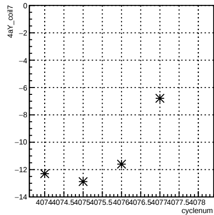
4aY_coil7:cyclenum {run == 5442}
