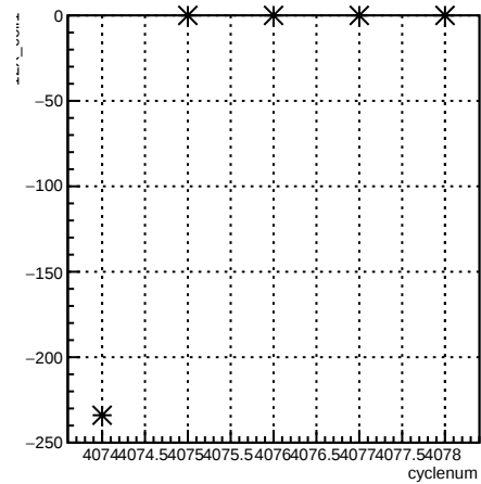
12X_coil1:cyclenum {run == 5442}
