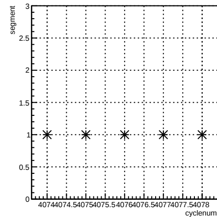
segment:cyclenum {run == 5442}
