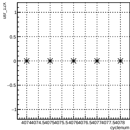
usr_12X:cyclenum {run == 5442}
