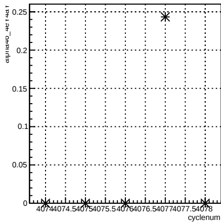
alpha46_4eY4aY:cyclenum {run == 5442}
