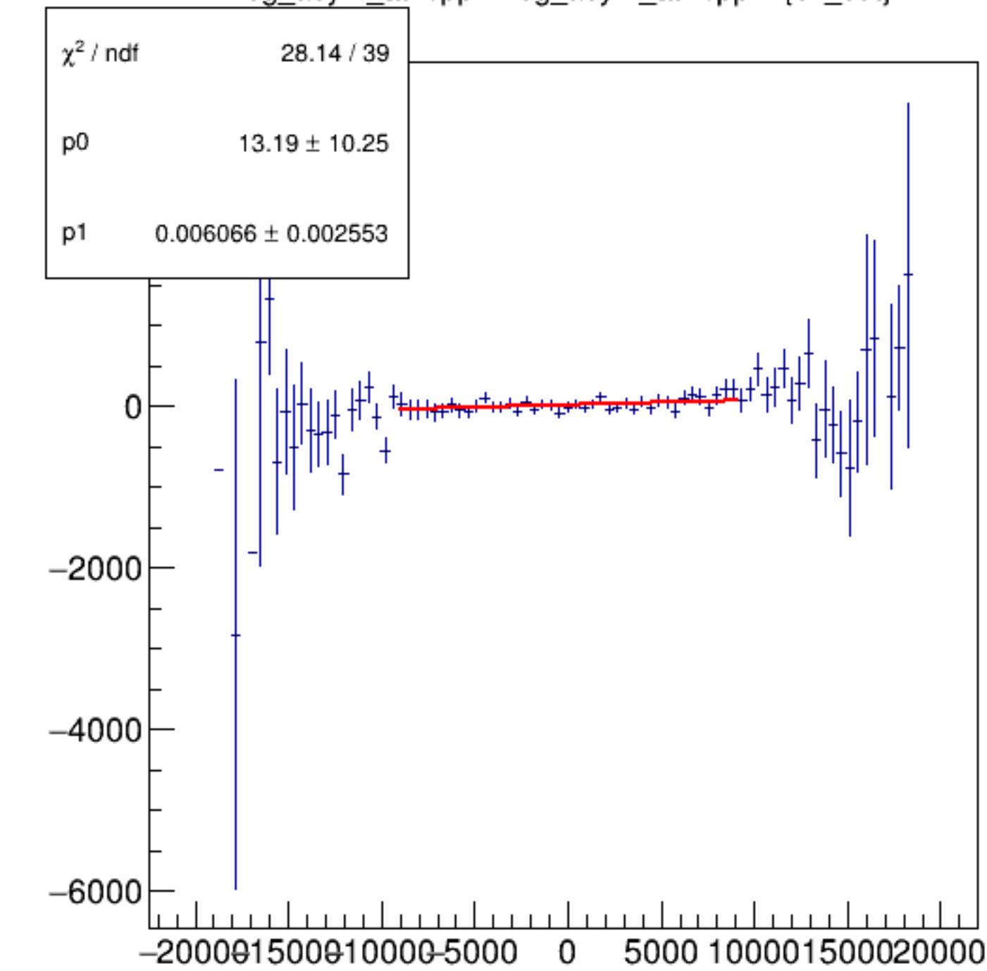
reg_asym_atl2/ppm:reg_asym_atr2/ppm {ok_cut}
