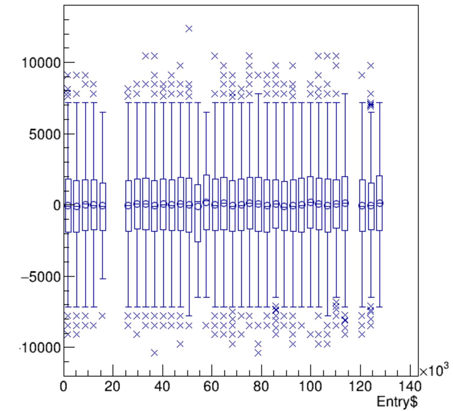
(reg_asym_atl2/ppm-reg_asym_atr2/ppm)/2:Entry$ {ok_cut}
