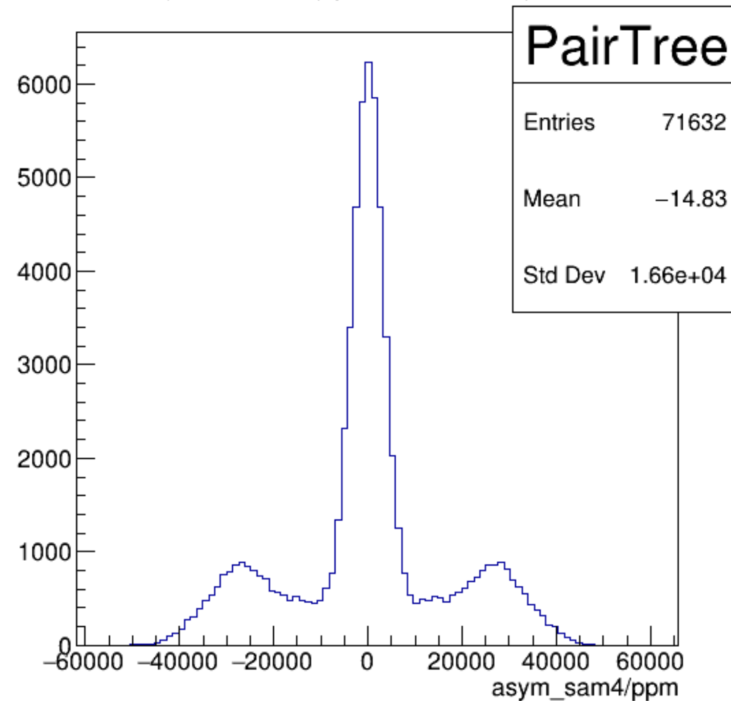
asym_sam4/ppm {ErrorFlag==0}
