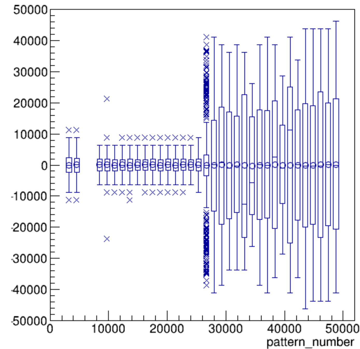
asym_sam3/ppm:pattern_number {ErrorFlag==0}
