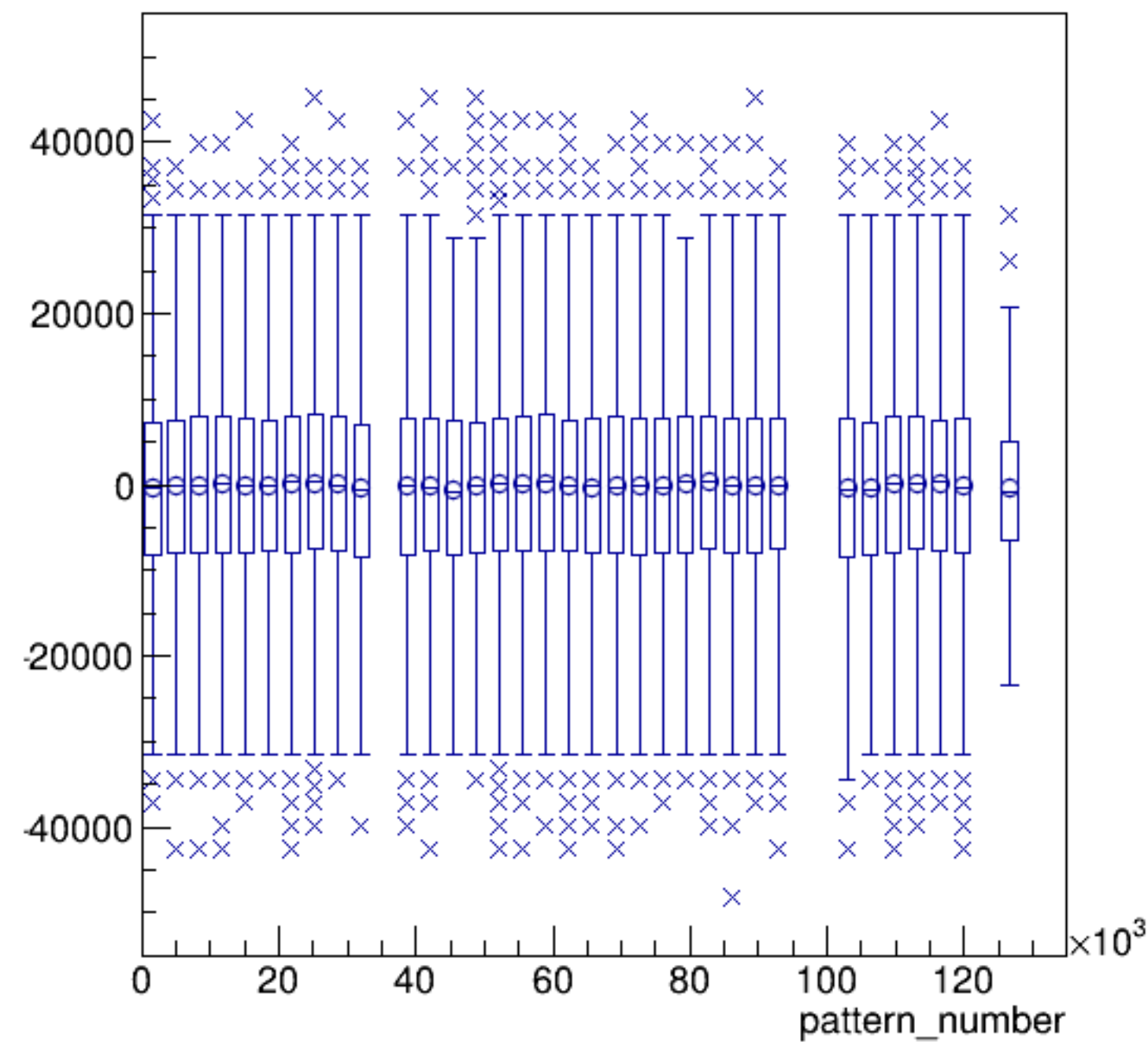
asym_atr1/ppm:pattern_number {ErrorFlag==0}
