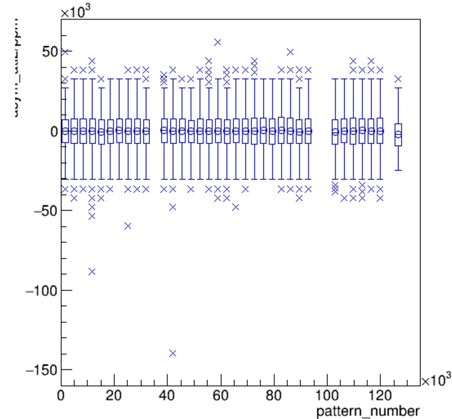
asym_atl2/ppm:pattern_number {ErrorFlag==0}
